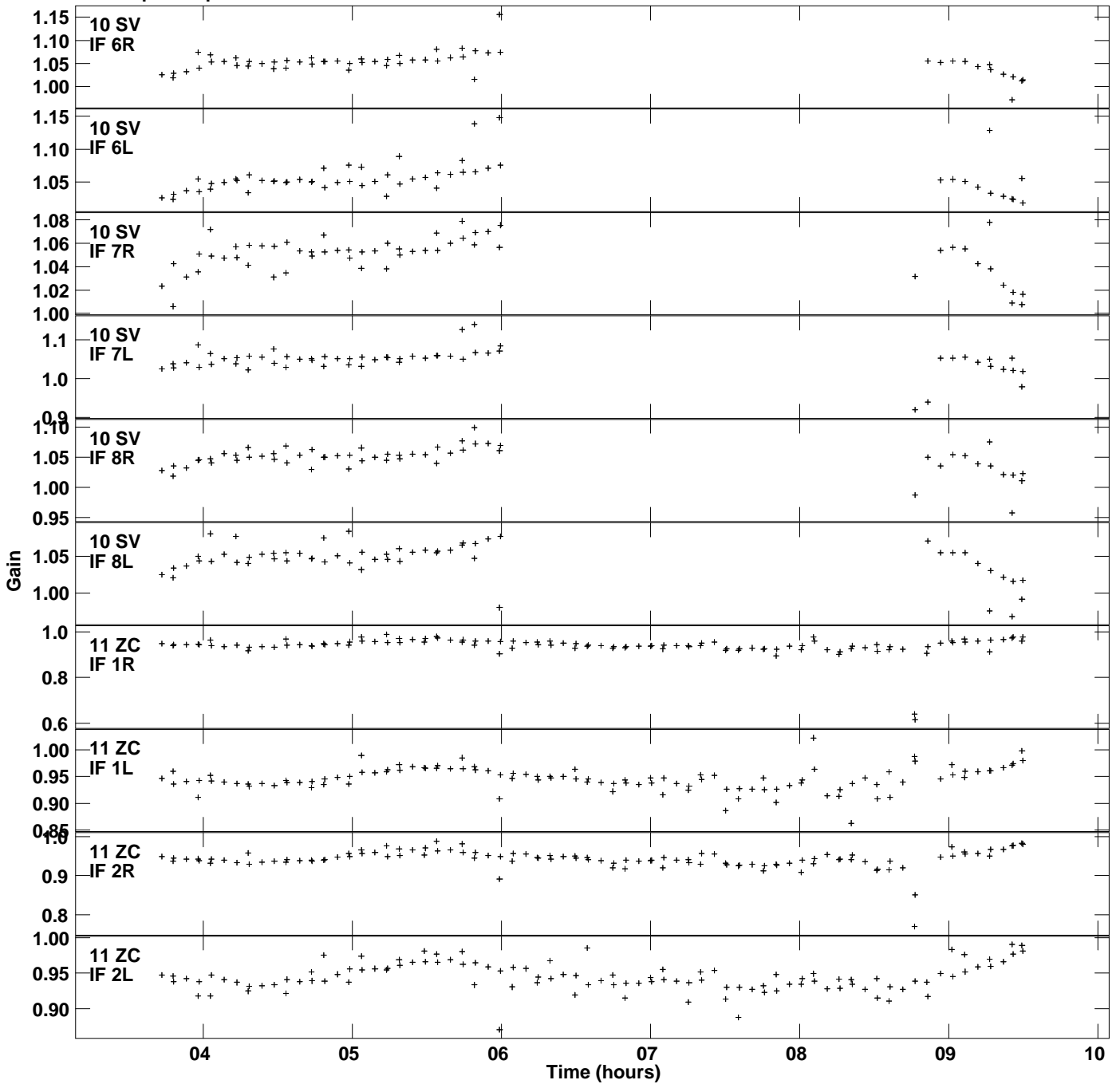
Plot file version 13 created 25-MAR-2014 11:53:36 Gain amp vs UTC time for J1128+5925.MULTI.1 SN 4 Rpol & Lpol IF 1 - 8
