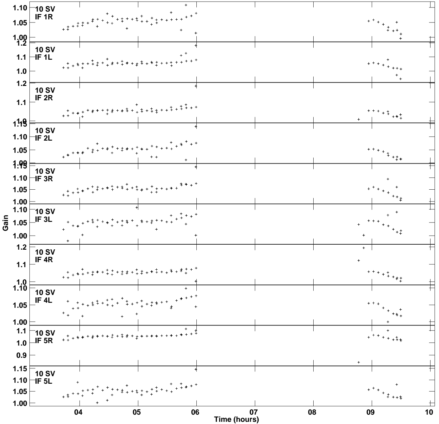
Plot file version 12 created 25-MAR-2014 11:53:36 Gain amp vs UTC time for J1128+5925.MULTI.1 SN 4 Rpol & Lpol IF 1 - 8
