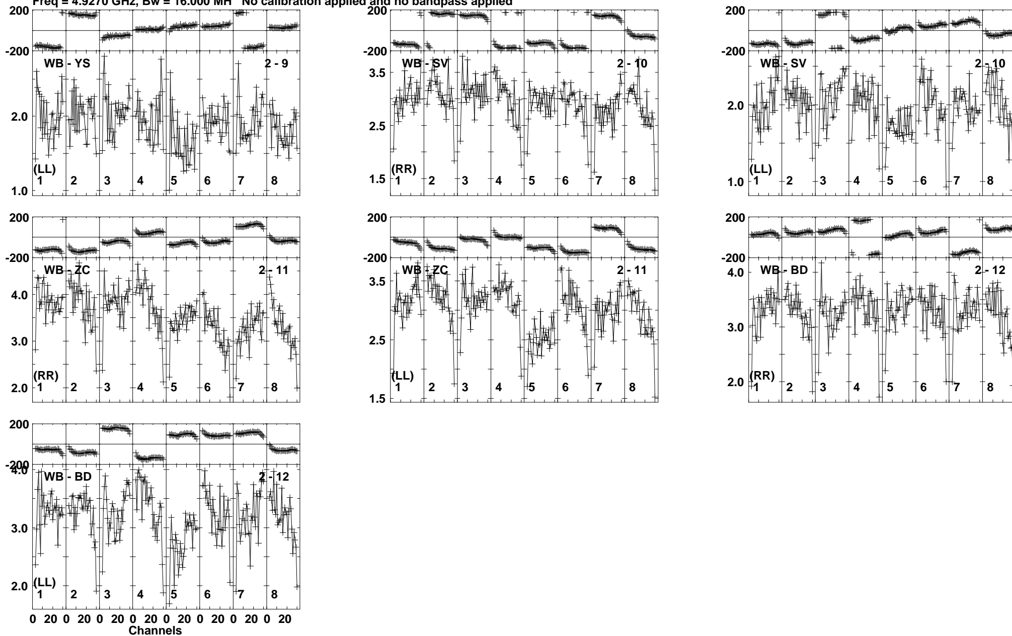
Lower frame: Milli Ampl Jy Top frame: Phas deg Vector averaged cross-power spectrum Baseline: WB (02) - YS (09) Timerange: 00/03:47:25 to 00/03:48:19
