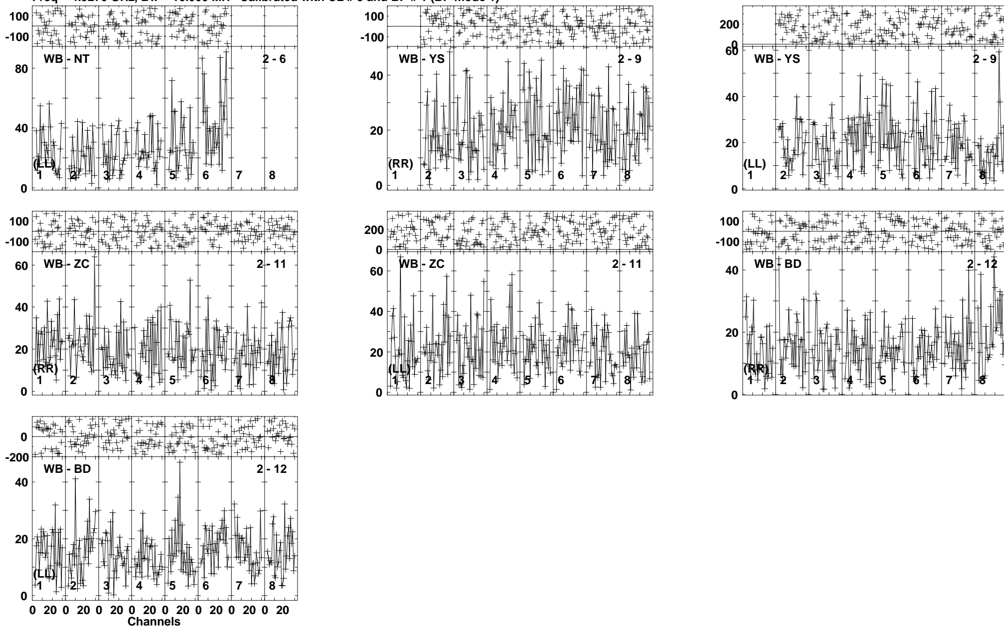
Lower frame: Milli Ampl Jy Top frame: Phas deg Vector averaged cross-power spectrum Baseline: WB (02) - NT (06) Timerange: 00/06:45:25 to 00/06:49:19
