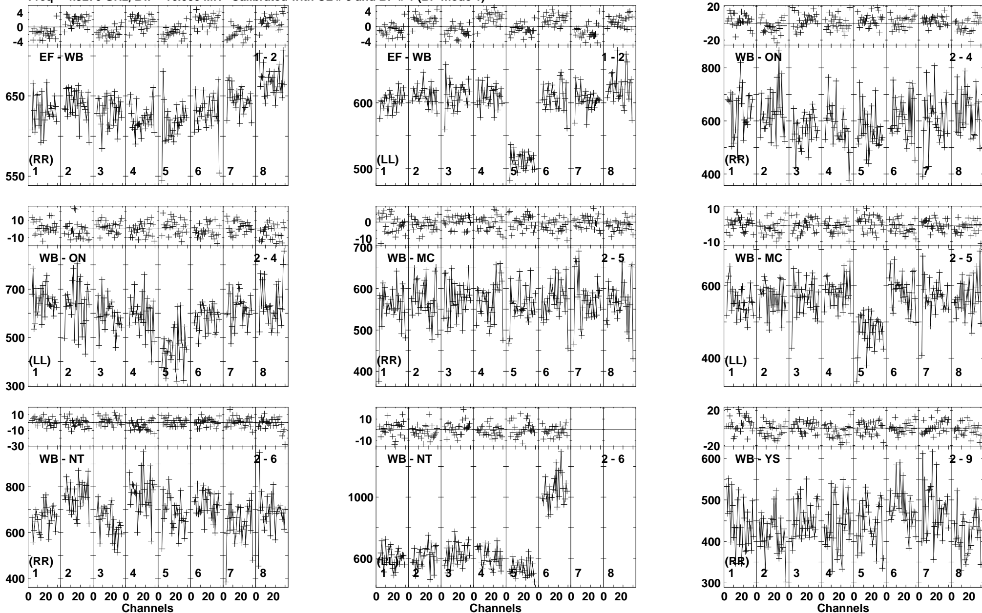
Lower frame: Milli Ampl Jy Top frame: Phas deg Vector averaged cross-power spectrum Baseline: EF (01) - WB (02) Timerange: 00/06:39:51 to 00/06:40:19
