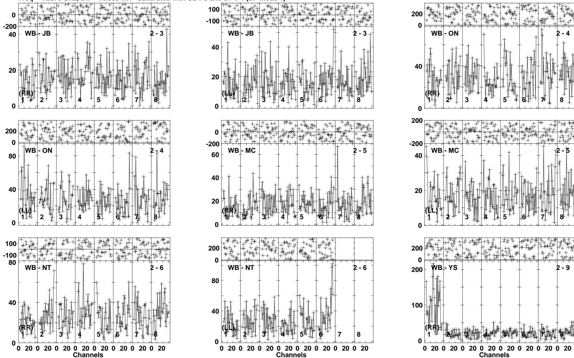
Lower frame: Milli Ampl Jy Top frame: Phas deg Vector averaged cross-power spectrum Baseline: WB (02) - JB (03) Timerange: 00/08:36:33 to 00/08:40:29
