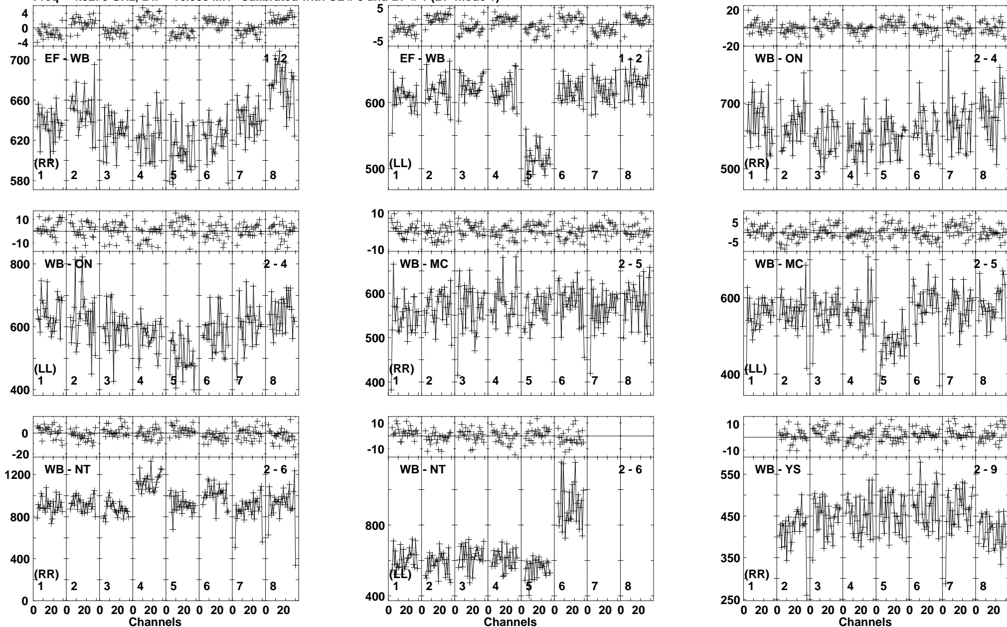
Lower frame: Milli Ampl Jy Top frame: Phas deg Vector averaged cross-power spectrum Baseline: EF (01) - WB (02) Timerange: 00/05:48:45 to 00/05:49:39
