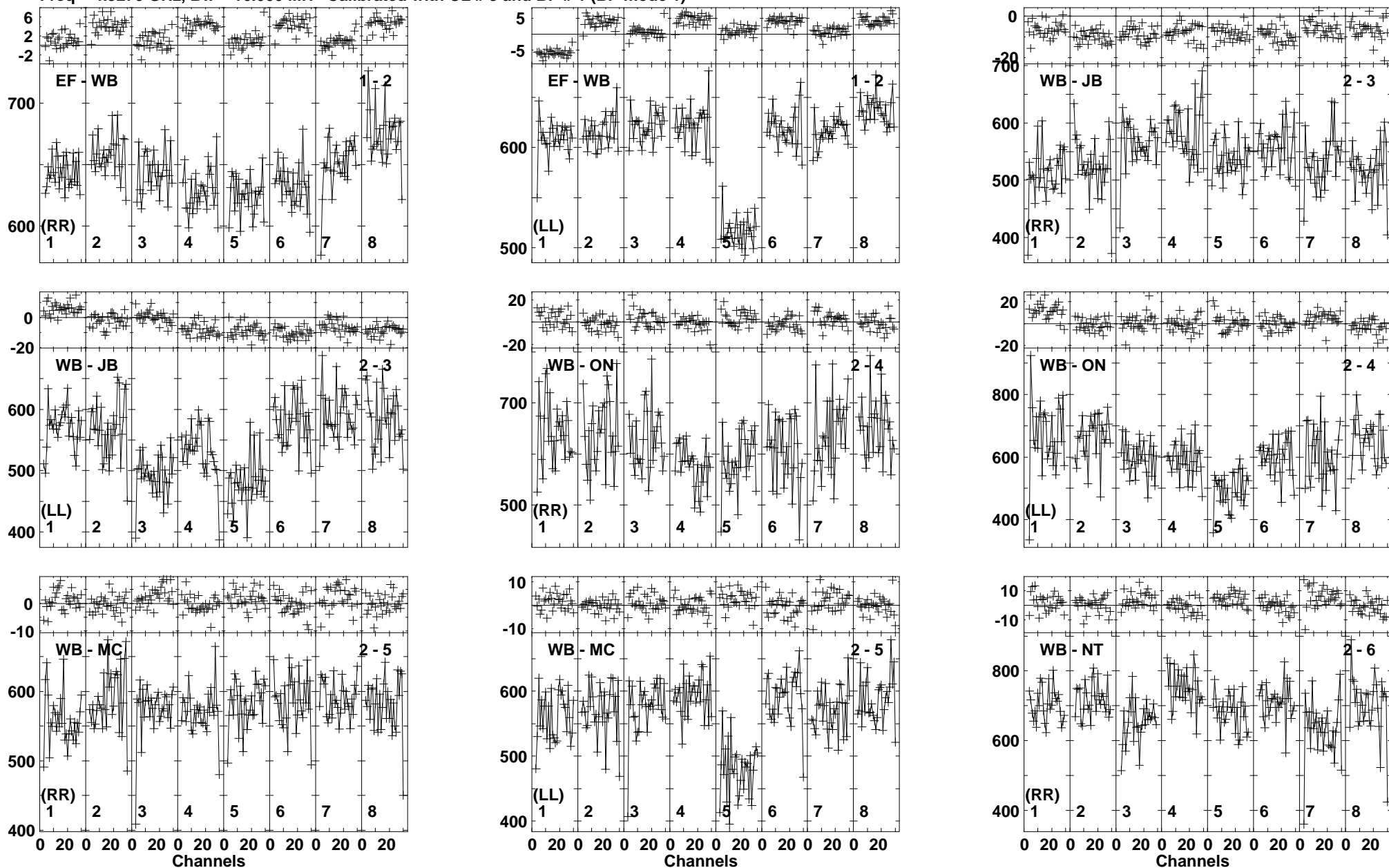
Lower frame: Milli Ampl Jy Top frame: Phas deg Vector averaged cross-power spectrum Baseline: EF (01) - WB (02) Timerange: 00/07:14:45 to 00/07:15:39
