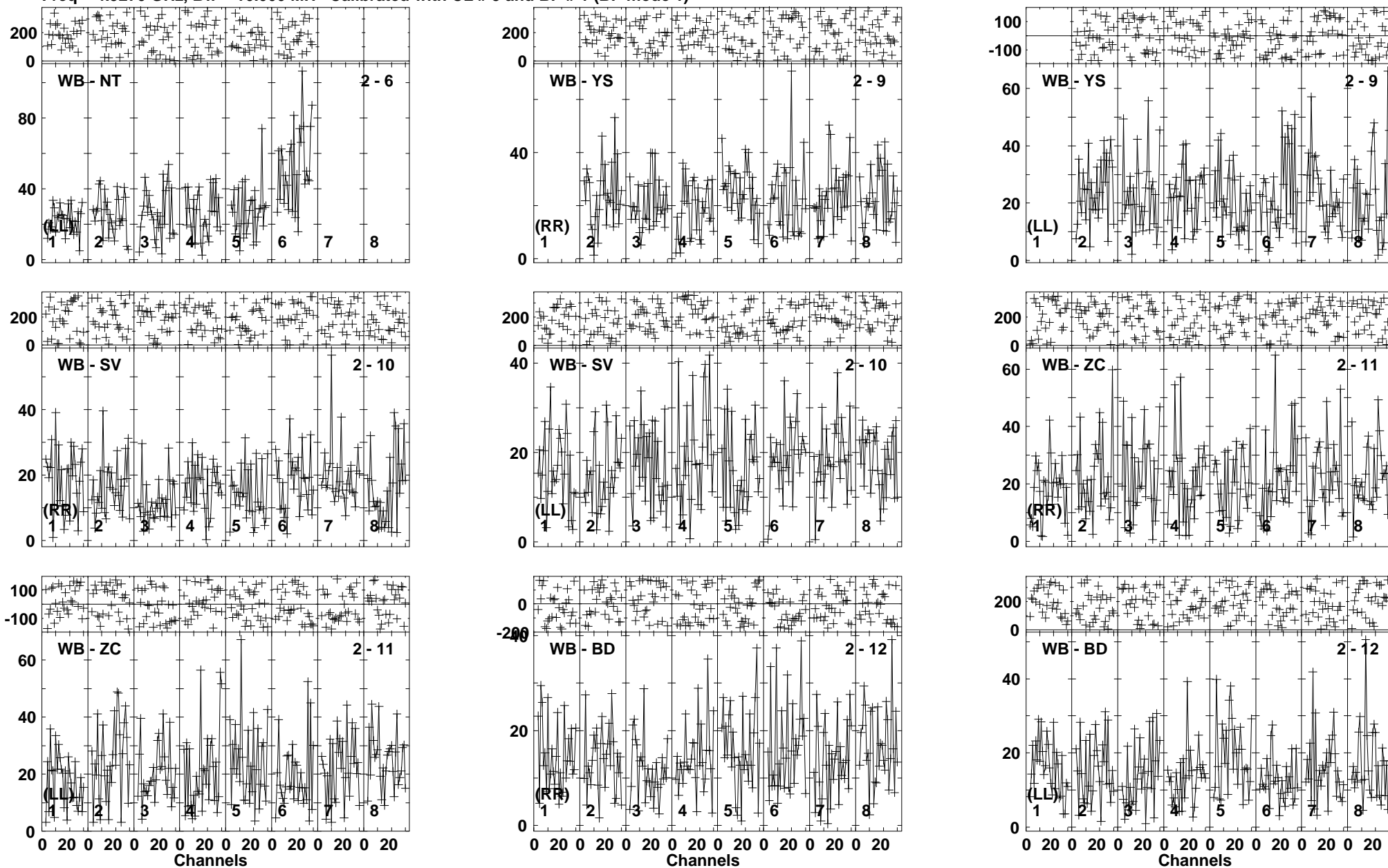
Lower frame: Milli Ampl Jy Top frame: Phas deg Vector averaged cross-power spectrum Baseline: WB (02) - NT (06) Timerange: 00/03:43:35 to 00/03:47:19
