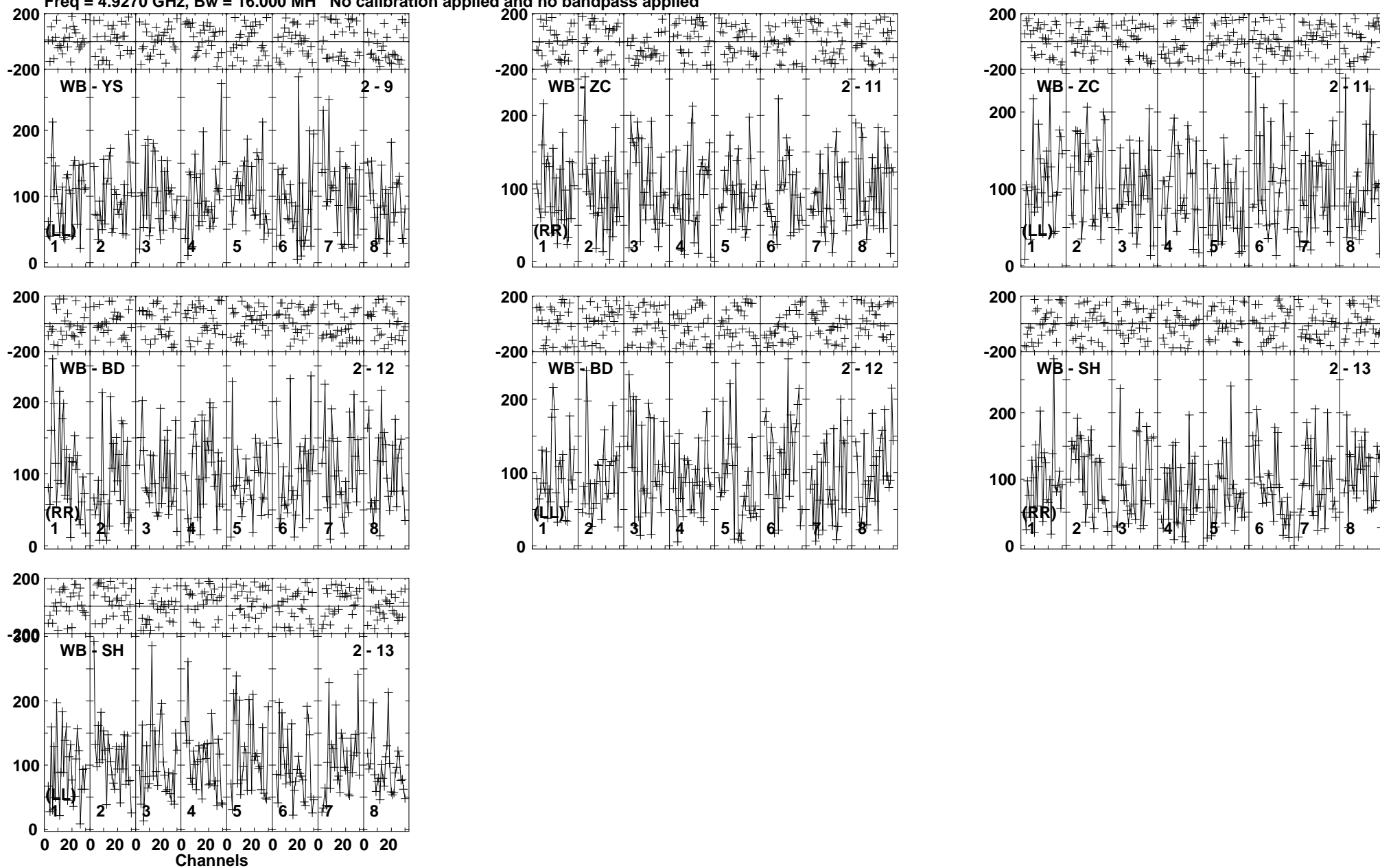
Lower frame: Micro Ampl Jy Top frame: Phas deg Vector averaged cross-power spectrum Baseline: WB (02) - YS (09) Timerange: 00/07:25:55 to 00/07:29:49
