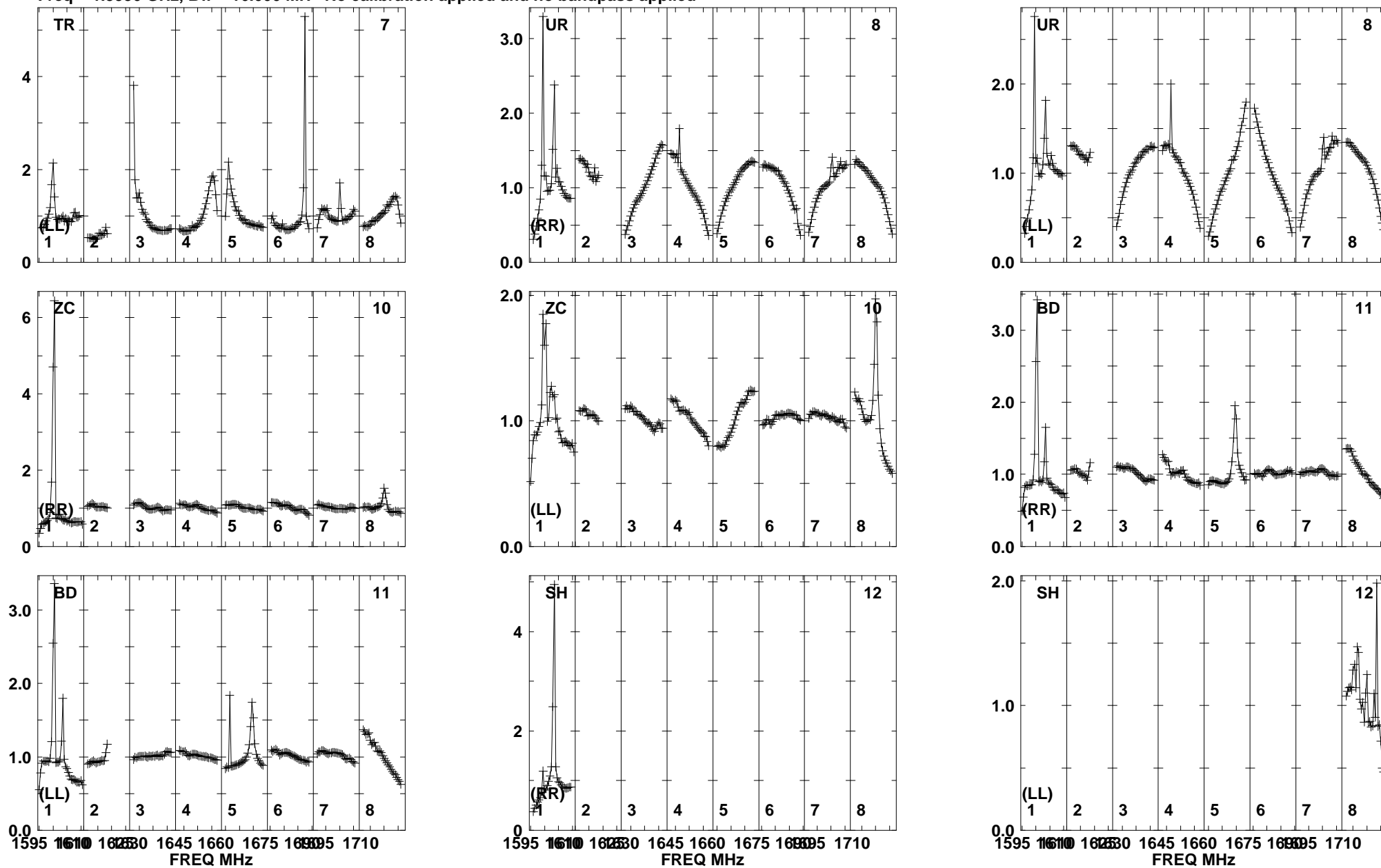
Lower frame: Real Jy Total-power spectrum Antenna: TR (07) Timerange: 00/08:32:21 to 00/08:36:49
