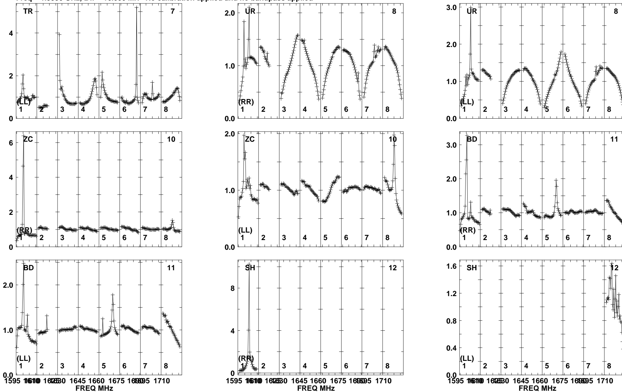
Lower frame: Real Jy Total-power spectrum Antenna: TR (07) Timerange: 00/08:31:25 to 00/08:32:19
