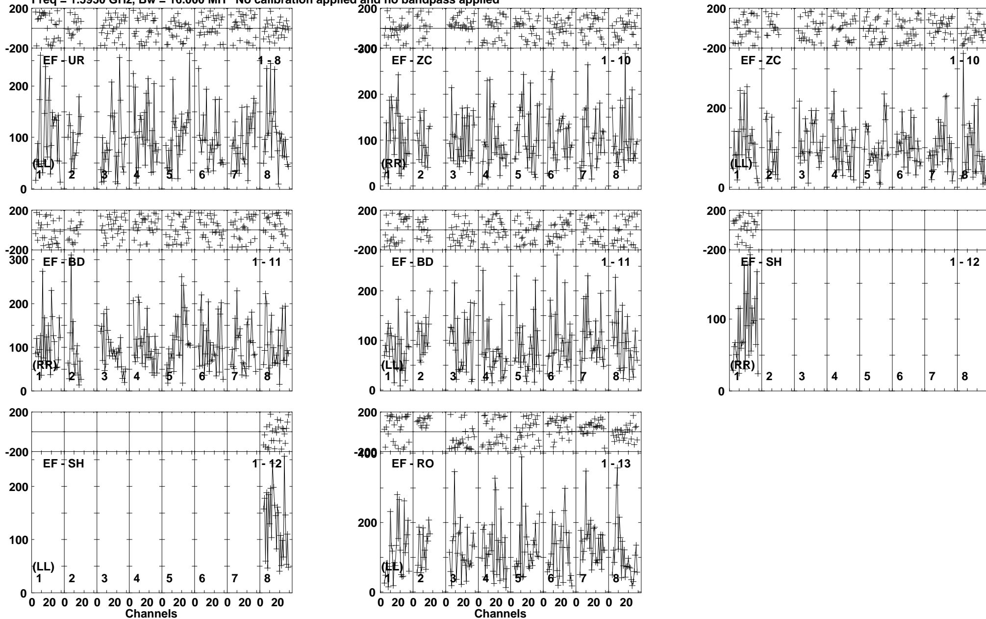
Lower frame: Micro Ampl Jy Top frame: Phas deg Vector averaged cross-power spectrum Baseline: EF (01) - UR (08) Timerange: 00/08:32:21 to 00/08:36:49
