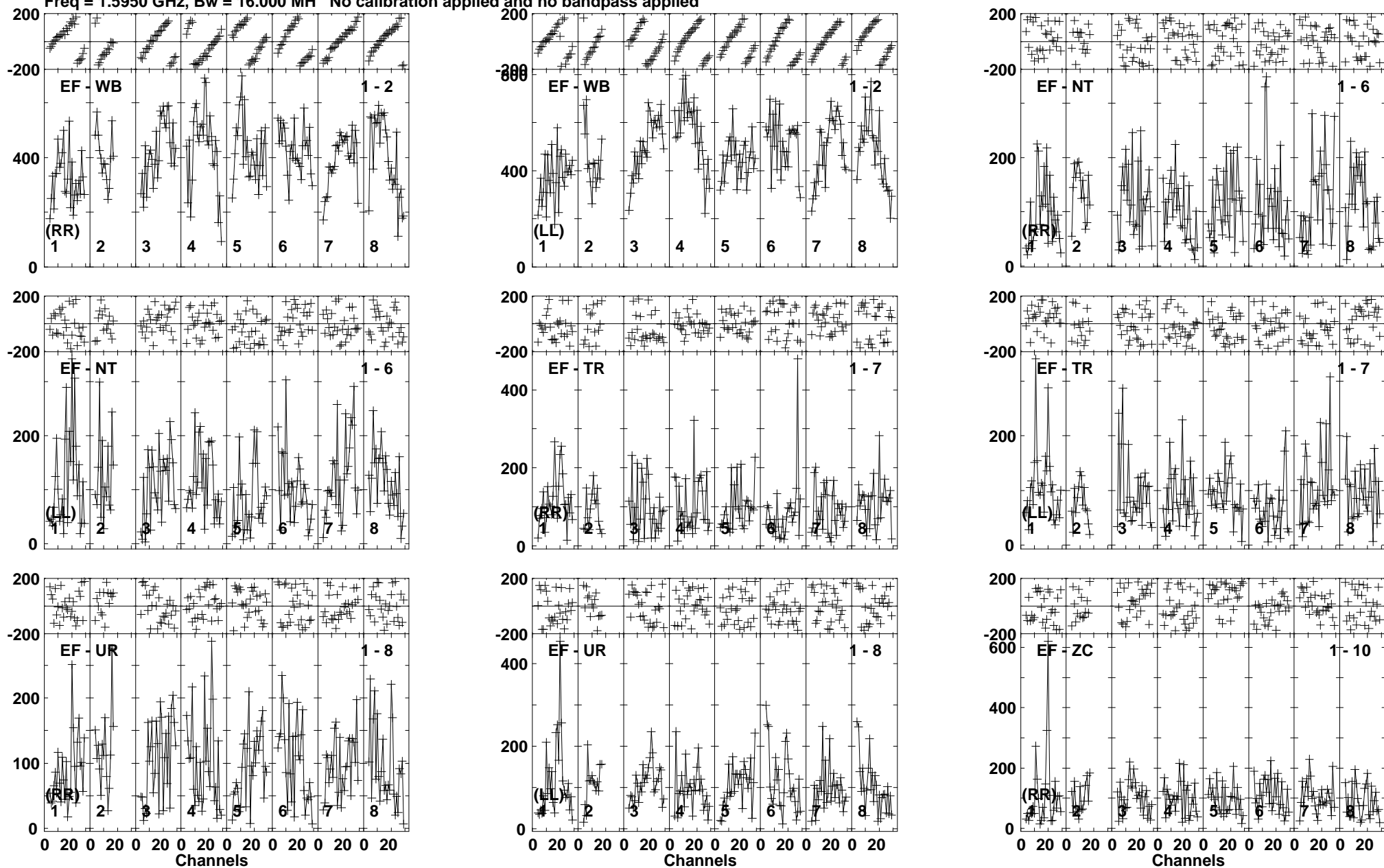
Lower frame: Micro Ampl Jy Top frame: Phas deg Vector averaged cross-power spectrum Baseline: EF (01) - WB (02) Timerange: 00/03:22:25 to 00/03:26:49
