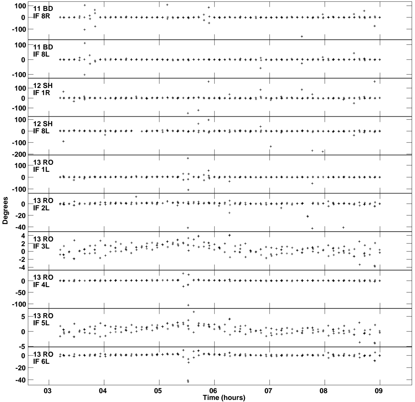
Plot file version 13 created 25-MAR-2014 18:13:04 Gain phs vs UTC time for J1128+5925.MULTI.1 SN 3 Rpol & Lpol IF 1 - 8
