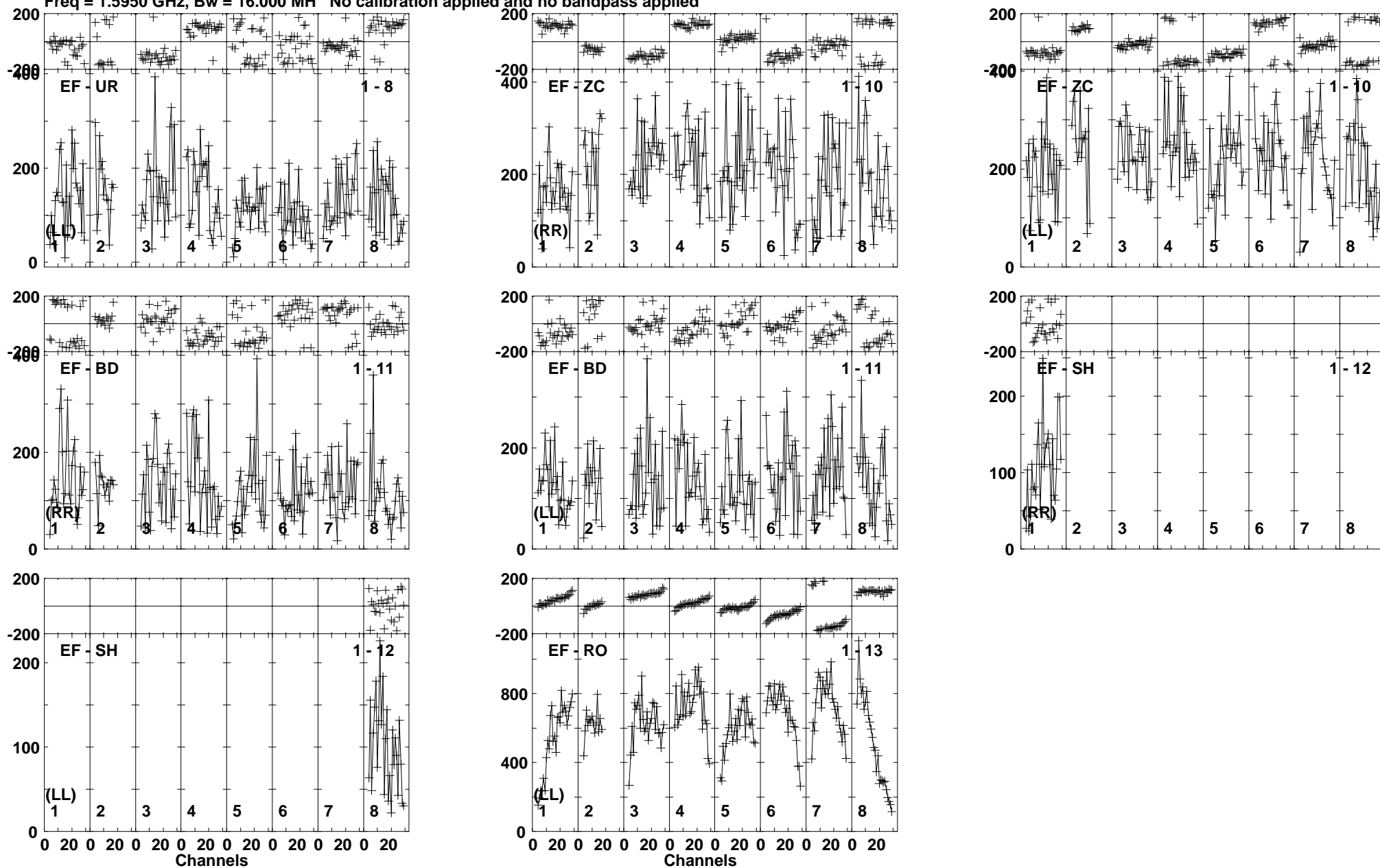
Lower frame: Micro Ampl Jy Top frame: Phas deg Vector averaged cross-power spectrum Baseline: EF (01) - UR (08) Timerange: 00/04:07:25 to 00/04:11:49
