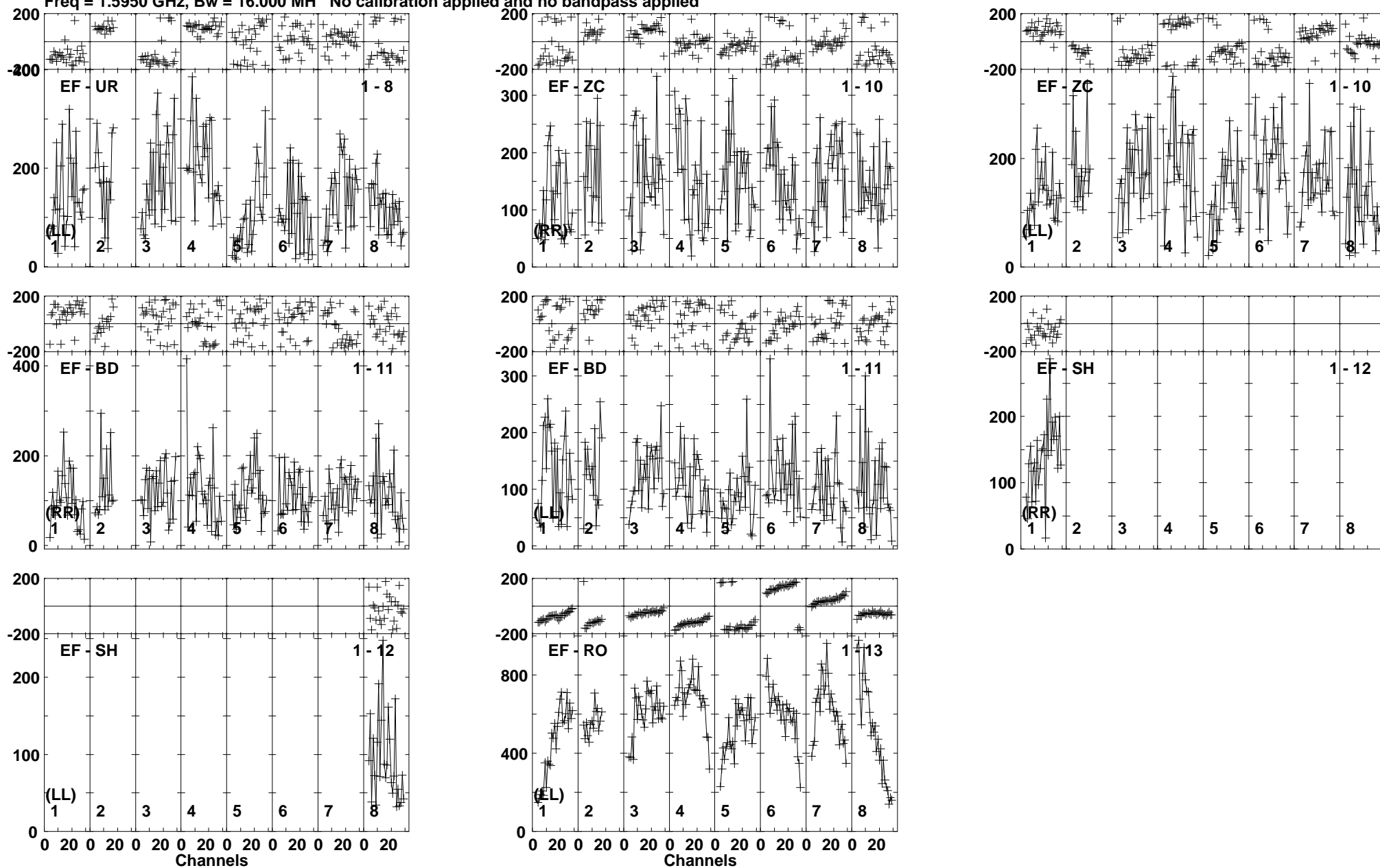
Lower frame: Micro Ampl Jy Top frame: Phas deg Vector averaged cross-power spectrum Baseline: EF (01) - UR (08) Timerange: 00/06:11:35 to 00/06:15:59
