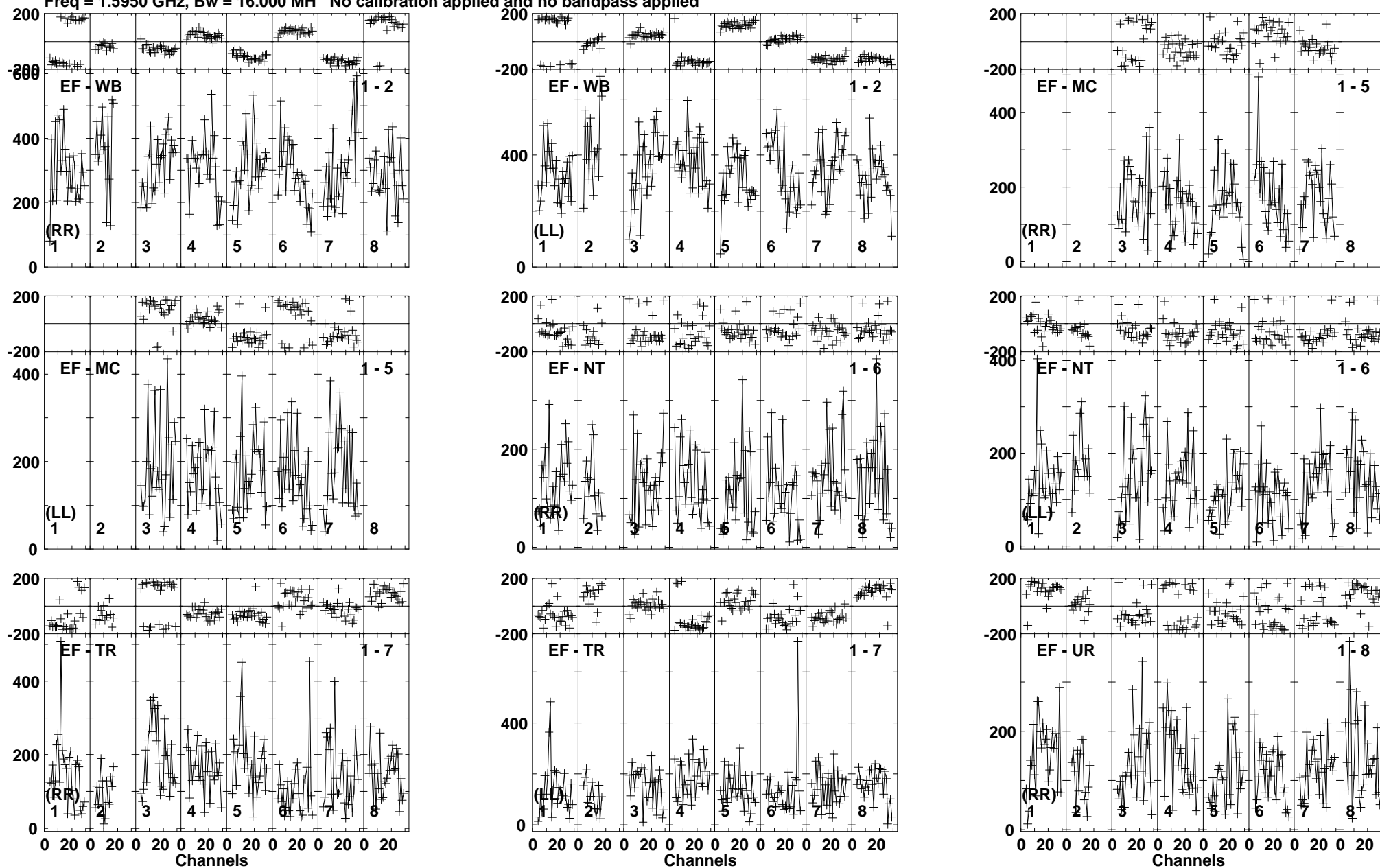
Lower frame: Micro Ampl Jy Top frame: Phas deg Vector averaged cross-power spectrum Baseline: EF (01) - WB (02) Timerange: 00/04:30:05 to 00/04:34:29
