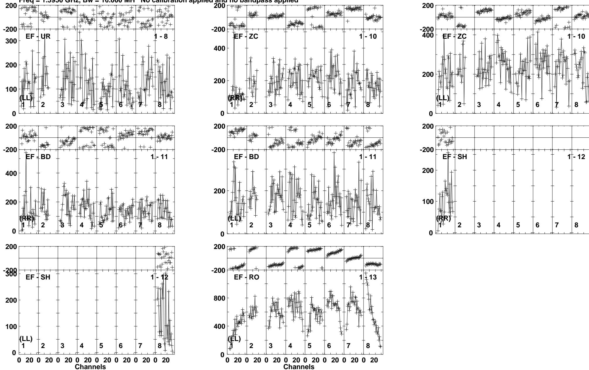
Lower frame: Micro Ampl Jy Top frame: Phas deg Vector averaged cross-power spectrum Baseline: EF (01) - UR (08) Timerange: 00/04:35:31 to 00/04:39:59
