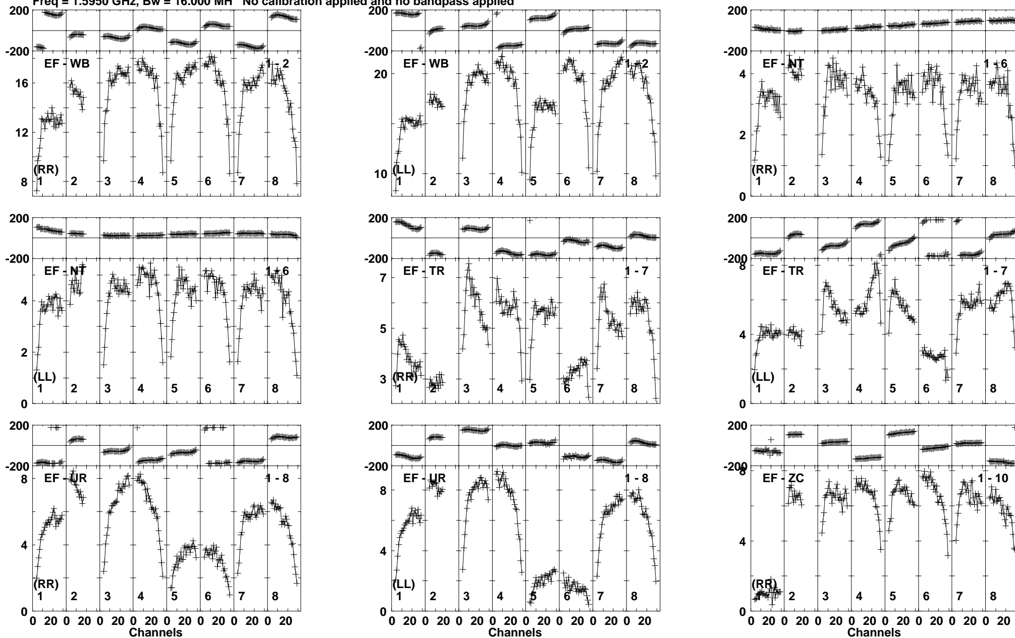
Lower frame: Milli Ampl Jy Top frame: Phas deg Vector averaged cross-power spectrum Baseline: EF (01) - WB (02) Timerange: 00/03:26:55 to 00/03:27:49
