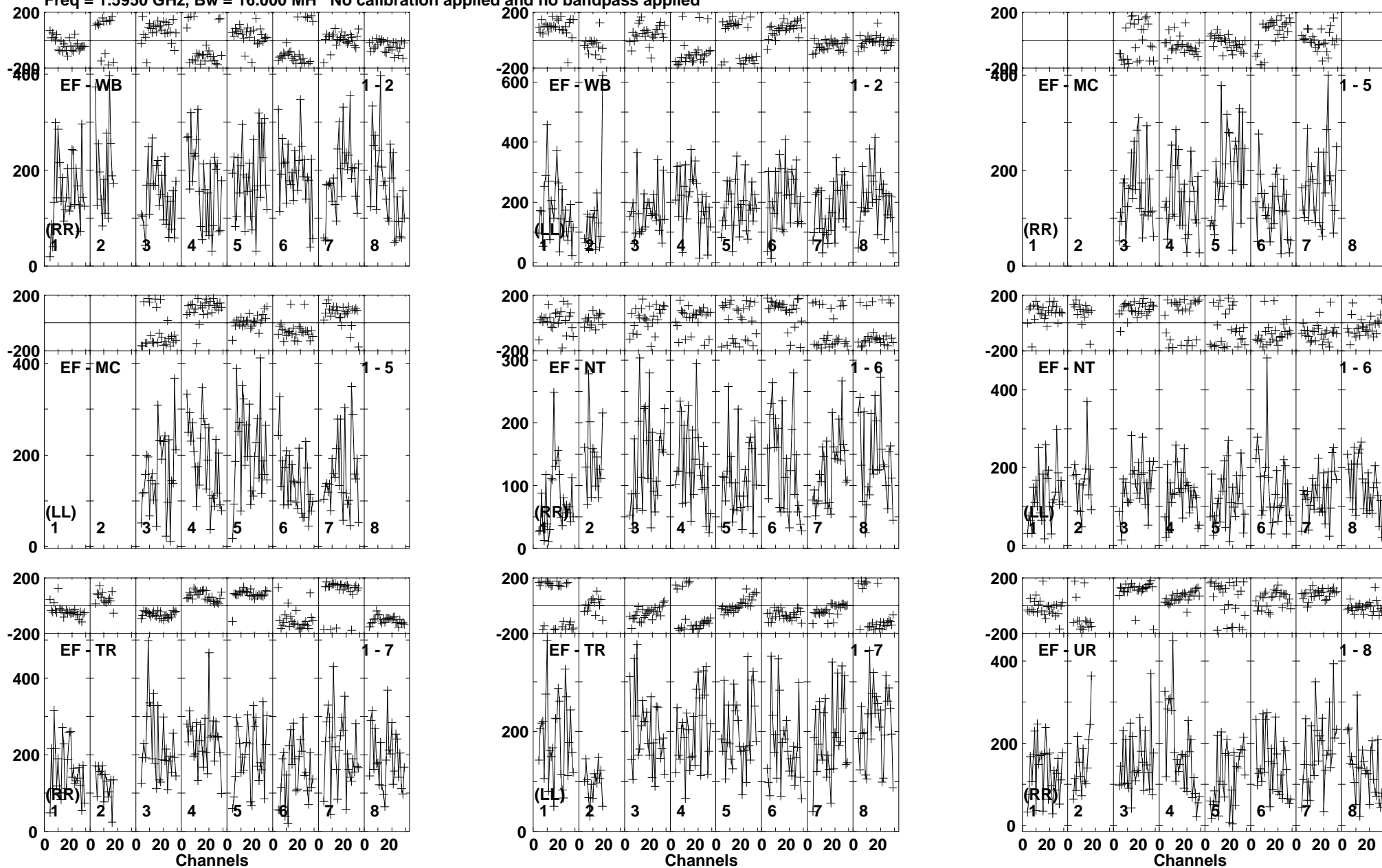
Lower frame: Micro Ampl Jy Top frame: Phas deg Vector averaged cross-power spectrum Baseline: EF (01) - WB (02) Timerange: 00/08:38:05 to 00/08:42:29
