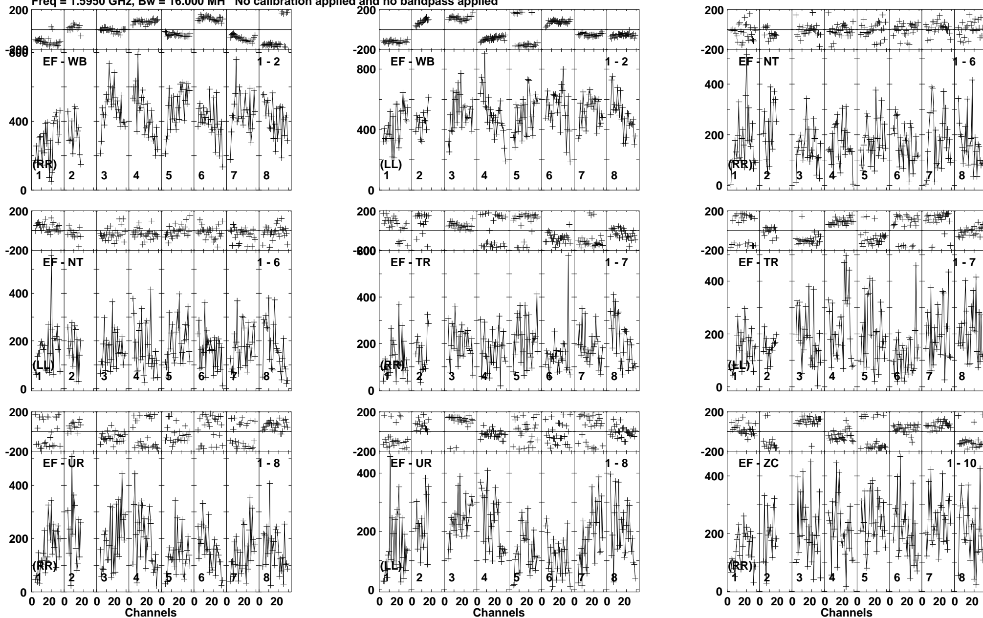
Lower frame: Micro Ampl Jy Top frame: Phas deg Vector averaged cross-power spectrum Baseline: EF (01) - WB (02) Timerange: 00/03:12:35 to 00/03:15:29
