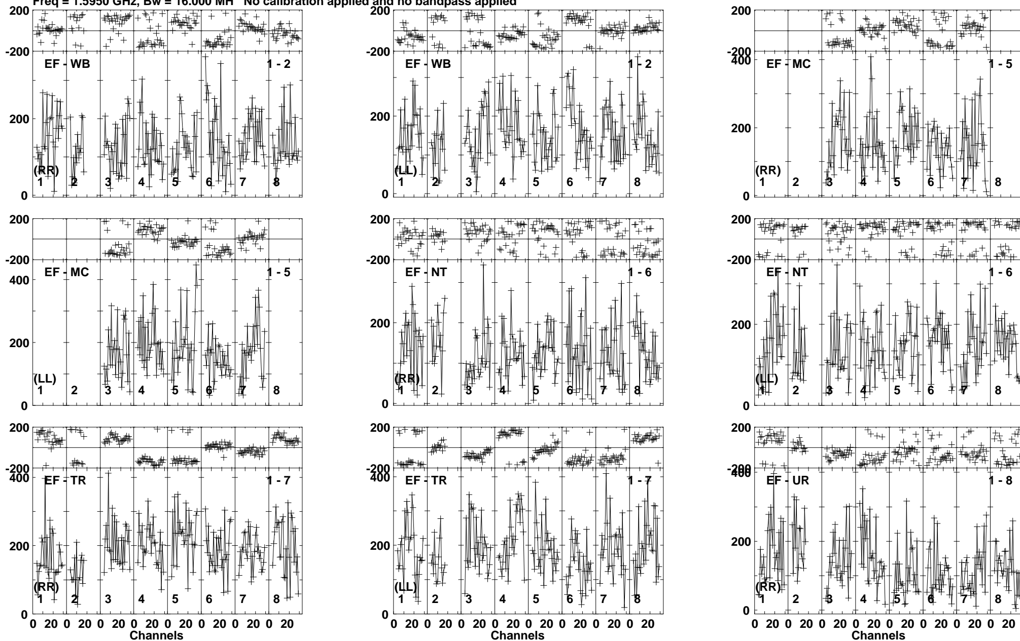
Lower frame: Micro Ampl Jy Top frame: Phas deg Vector averaged cross-power spectrum Baseline: EF (01) - WB (02) Timerange: 00/06:11:35 to 00/06:15:59
