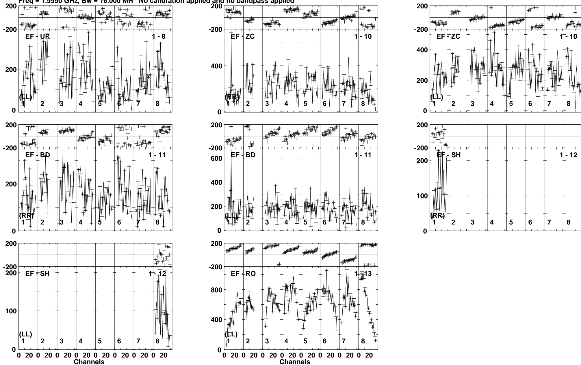
Lower frame: Micro Ampl Jy Top frame: Phas deg Vector averaged cross-power spectrum Baseline: EF (01) - UR (08) Timerange: 00/04:18:45 to 00/04:23:09
