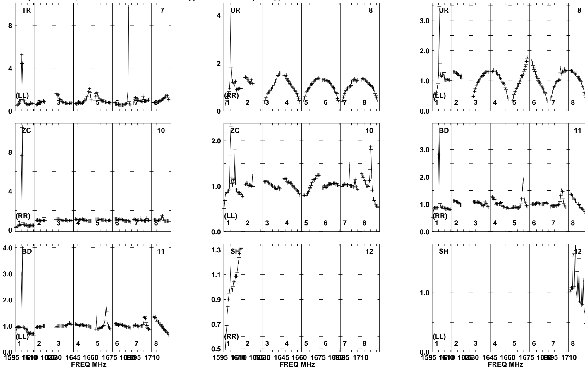
Lower frame: Real Jy Total-power spectrum Antenna: TR (07) Timerange: 00/04:52:35 to 00/04:56:59
