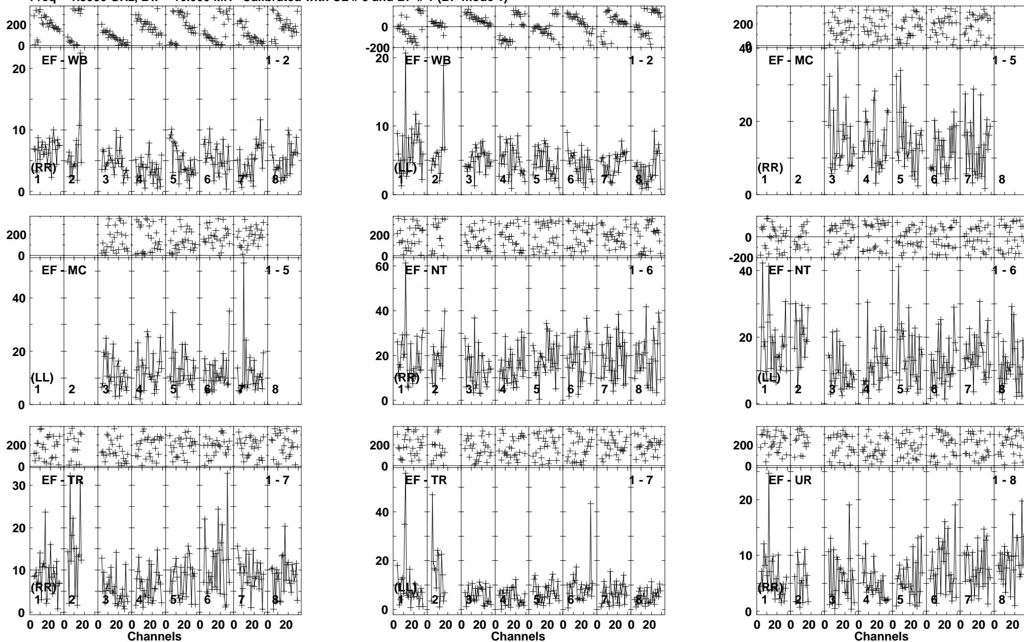
Lower frame: Milli Ampl Jy Top frame: Phas deg Vector averaged cross-power spectrum Baseline: EF (01) - WB (02) Timerange: 00/04:58:11 to 00/05:02:39
