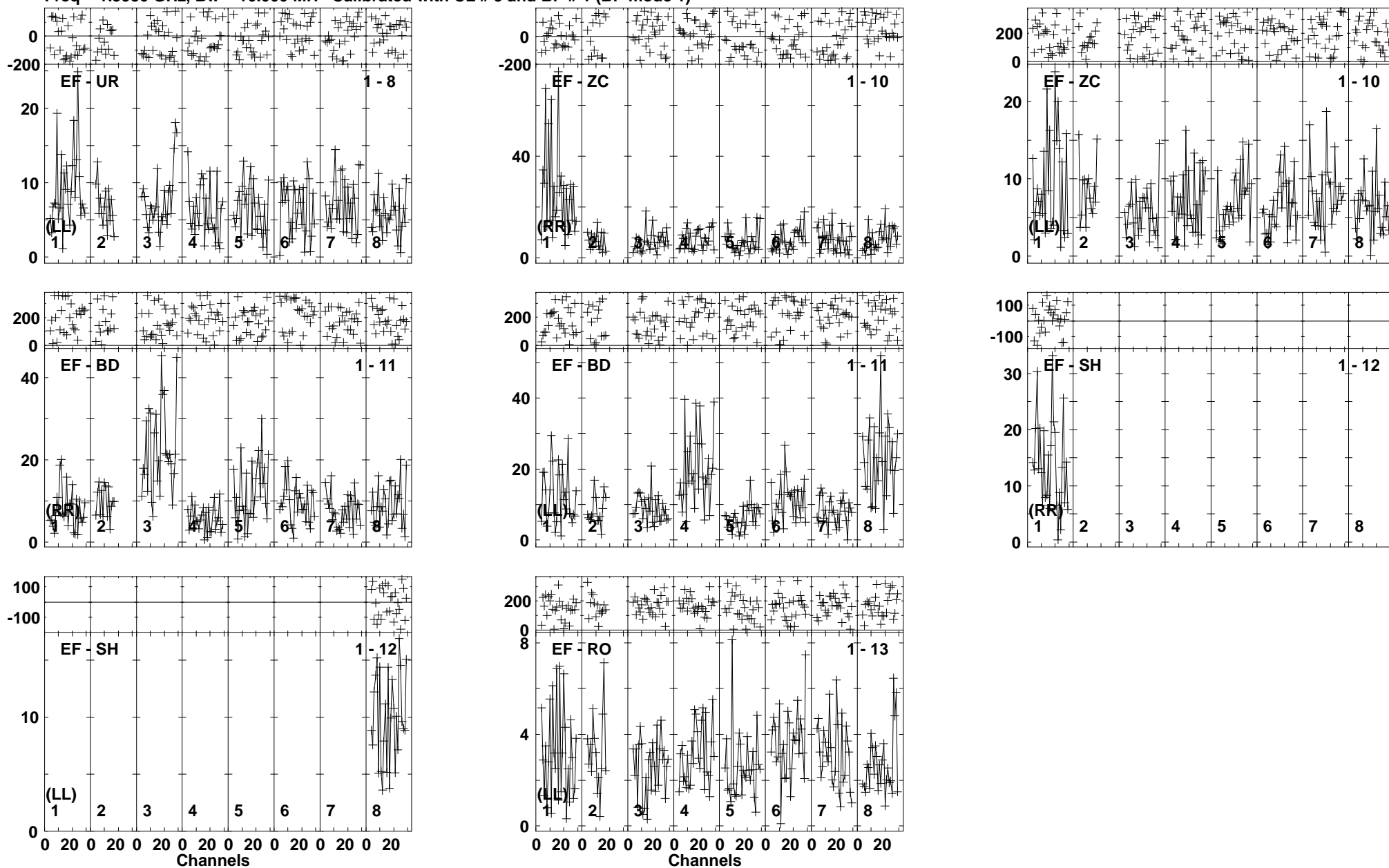
Lower frame: Milli Ampl Jy Top frame: Phas deg Vector averaged cross-power spectrum Baseline: EF (01) - UR (08) Timerange: 00/03:44:55 to 00/03:49:19
