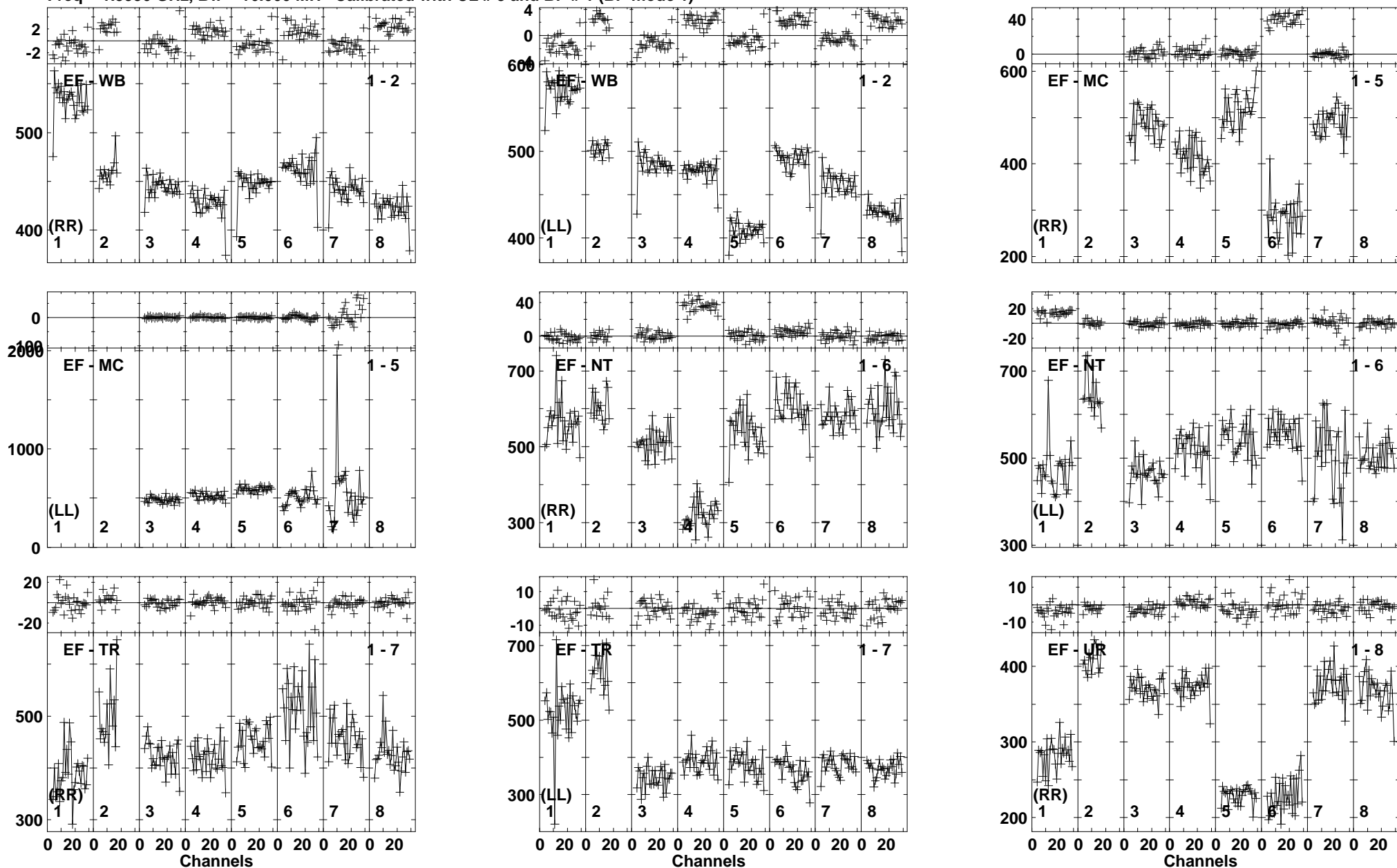
Lower frame: Milli Ampl Jy Top frame: Phas deg Vector averaged cross-power spectrum Baseline: EF (01) - WB (02) Timerange: 00/05:03:21 to 00/05:03:49
