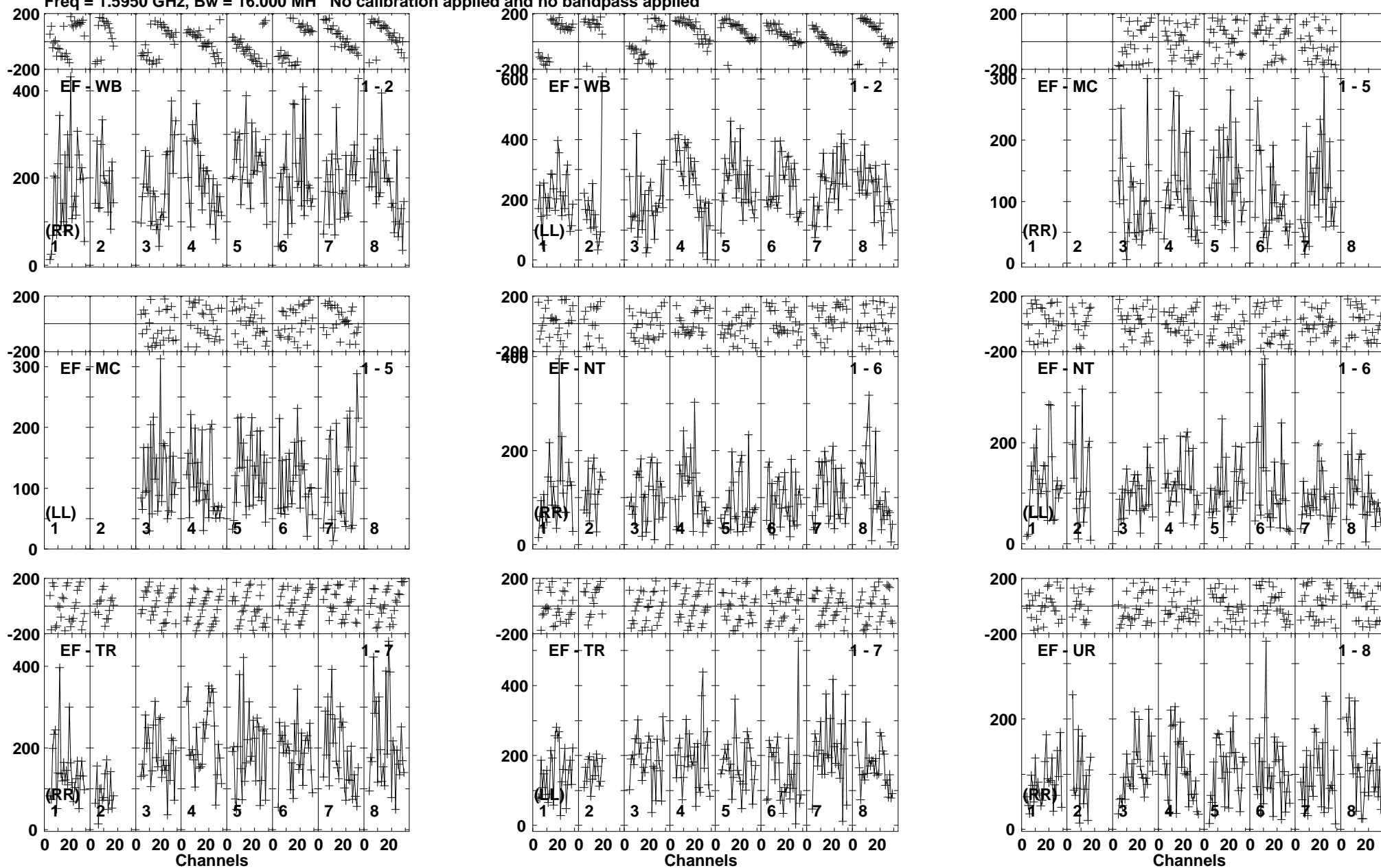
Lower frame: Micro Ampl Jy Top frame: Phas deg Vector averaged cross-power spectrum Baseline: EF (01) - WB (02) Timerange: 00/06:17:01 to 00/06:21:29
