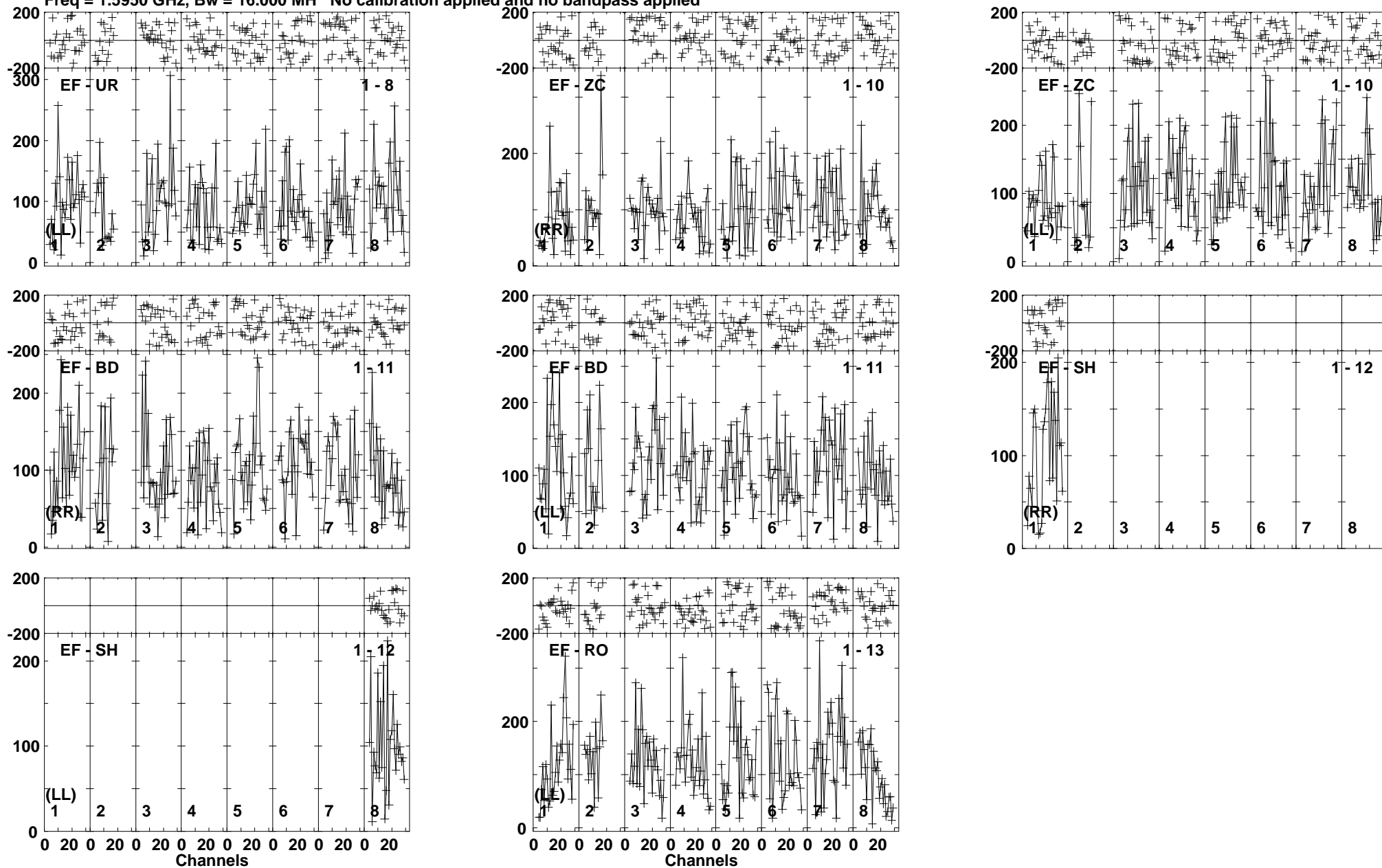
Lower frame: Micro Ampl Jy Top frame: Phas deg Vector average cross-power spectrum Baseline: EF (01) - UR (08) Timerange: 00/06:11:35 to 00/06:15:59
