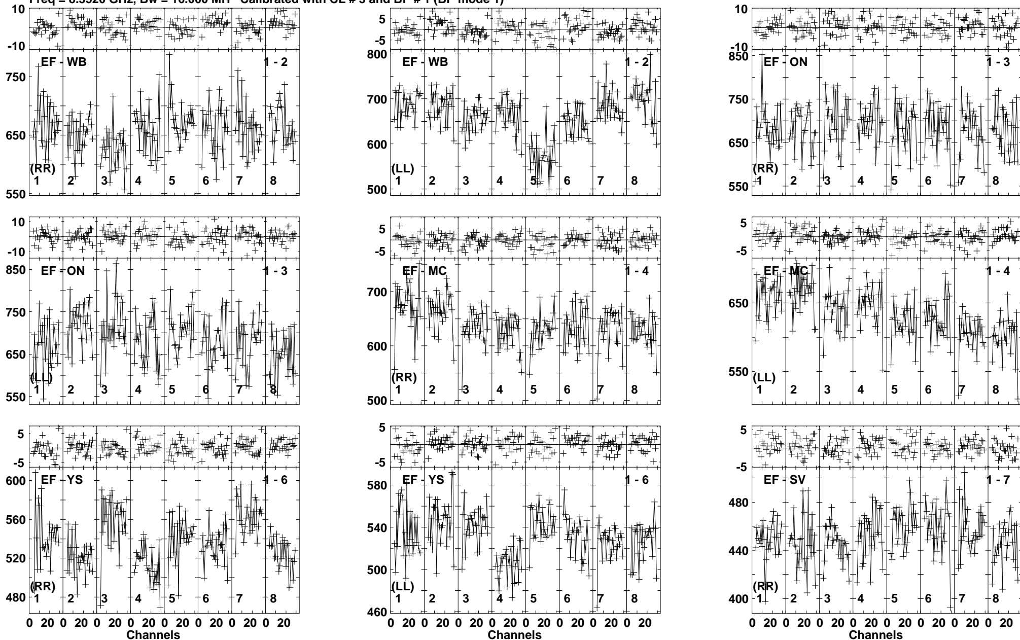
Lower frame: Milli Ampl Jy Top frame: Phas deg Vector averaged cross-power spectrum Baseline: EF (01) - WB (02) Timerange: 00/03:28:41 to 00/03:29:09
