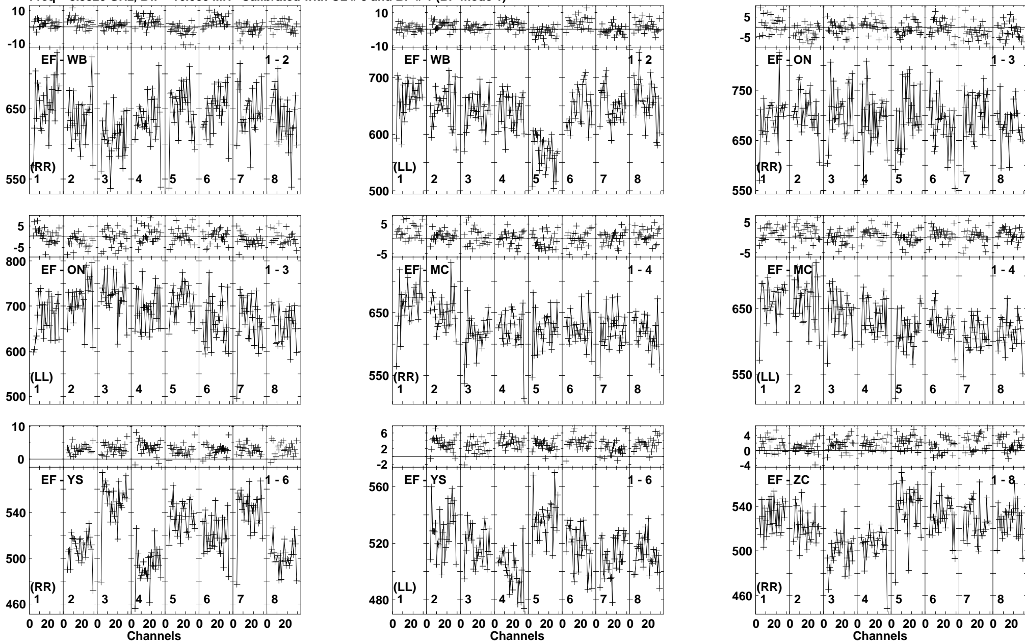
Lower frame: Milli Ampl Jy Top frame: Phas deg Vector averaged cross-power spectrum Baseline: EF (01) - WB (02) Timerange: 00/05:27:41 to 00/05:28:44
