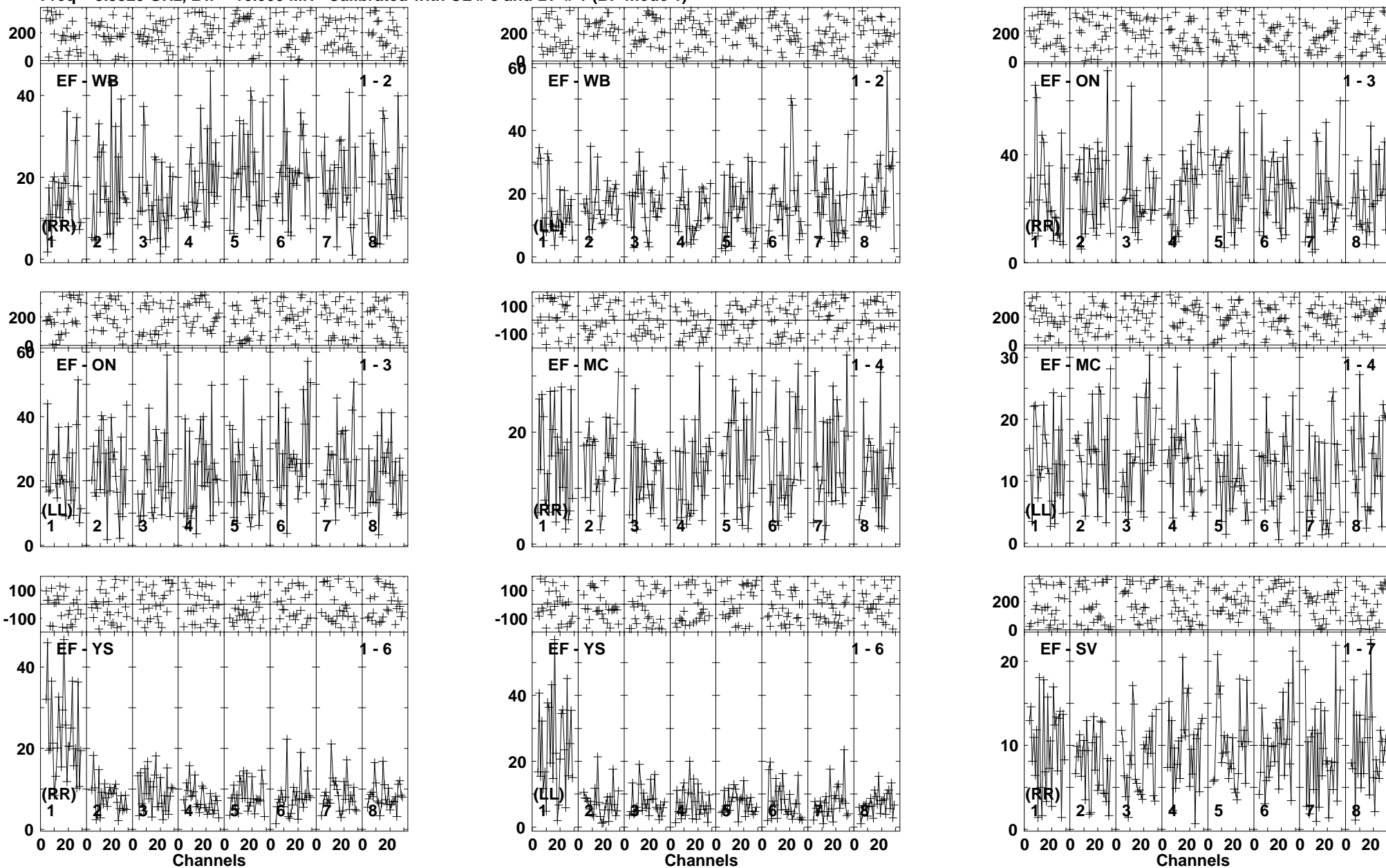
Lower frame: Milli Ampl Jy Top frame: Phas deg Vector averaged cross-power spectrum Baseline: EF (01) - WB (02) Timerange: 00/05:04:00 to 00/05:07:00
