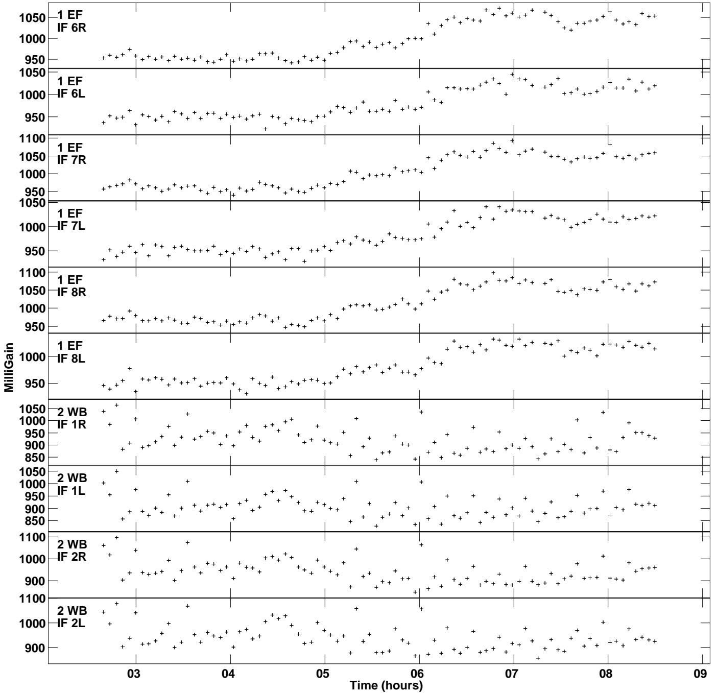
Plot file version 2 created 24-MAR-2014 13:35:00 Gain amp vs UTC time for J1128+5925.MULTI.1 SN 2 Rpol & Lpol IF 1 - 8
