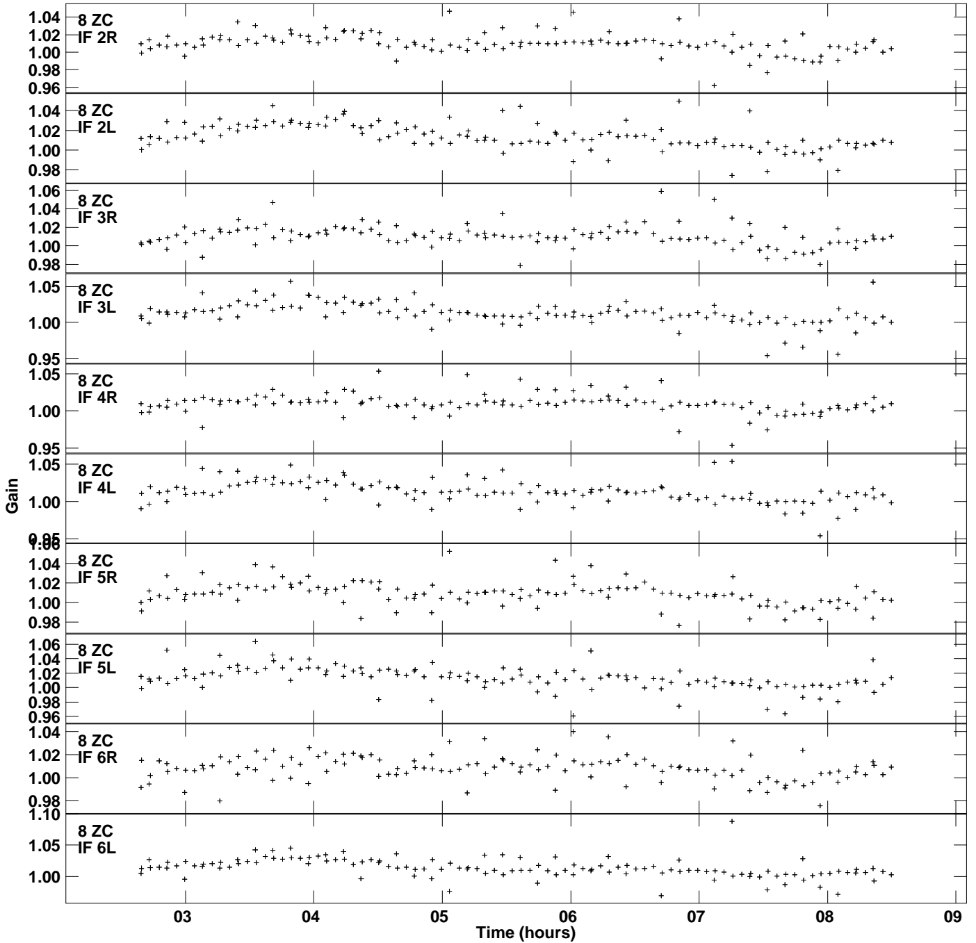
Plot file version 10 created 24-MAR-2014 13:35:17 Gain amp vs UTC time for J1128+5925.MULTI.1 SN 4 Rpol & Lpol IF 1 - 8
