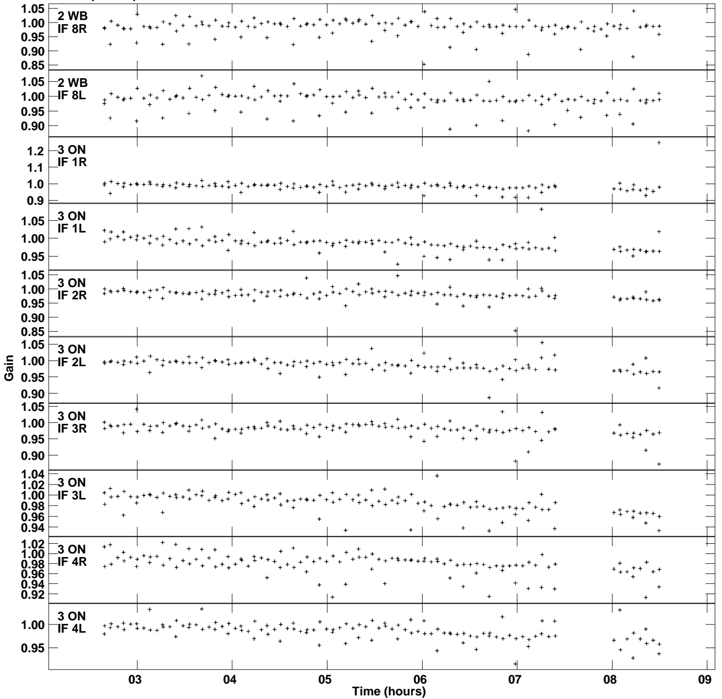
Plot file version 4 created 24-MAR-2014 13:35:17 Gain amp vs UTC time for J1128+5925.MULTI.1 SN 4 Rpol & Lpol IF 1 - 8
