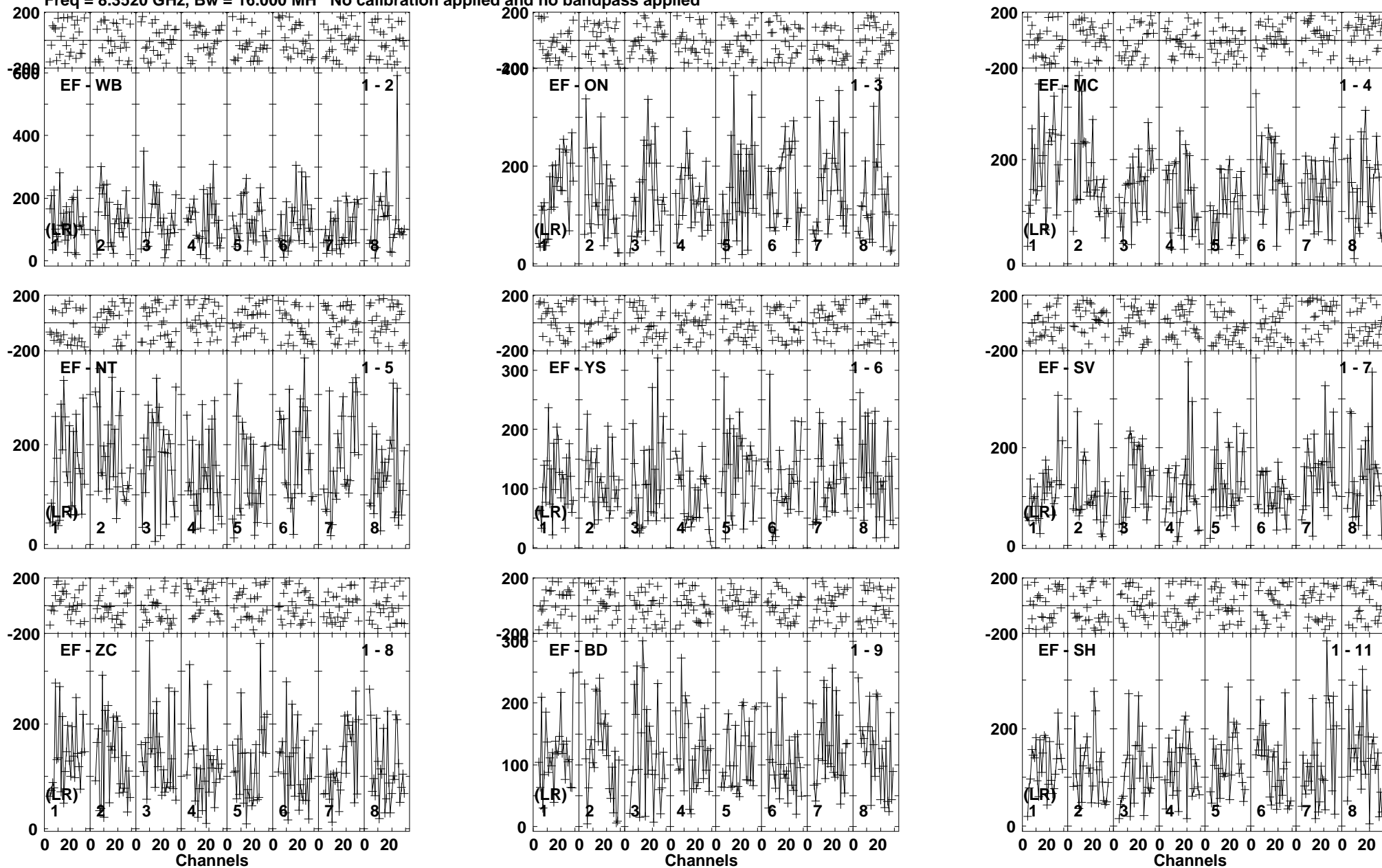
Lower frame: Micro Ampl Jy Top frame: Phas deg Vector averaged cross-power spectrum Baseline: EF (01) - WB (02) Timerange: 00/05:00:00 to 00/05:02:54
