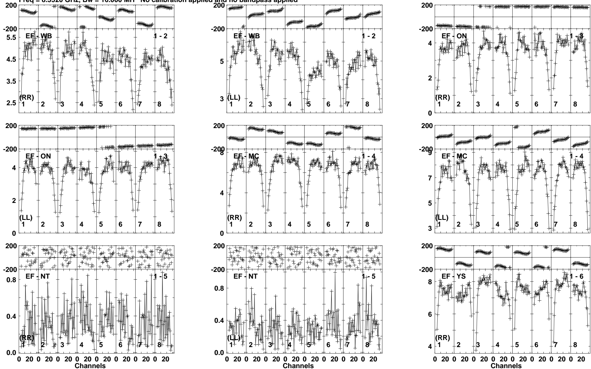
Lower frame: Milli Ampl Jy Top frame: Phas deg Vector averaged cross-power spectrum Baseline: EF (01) - WB (02) Timerange: 00/06:58:28 to 00/06:59:29
