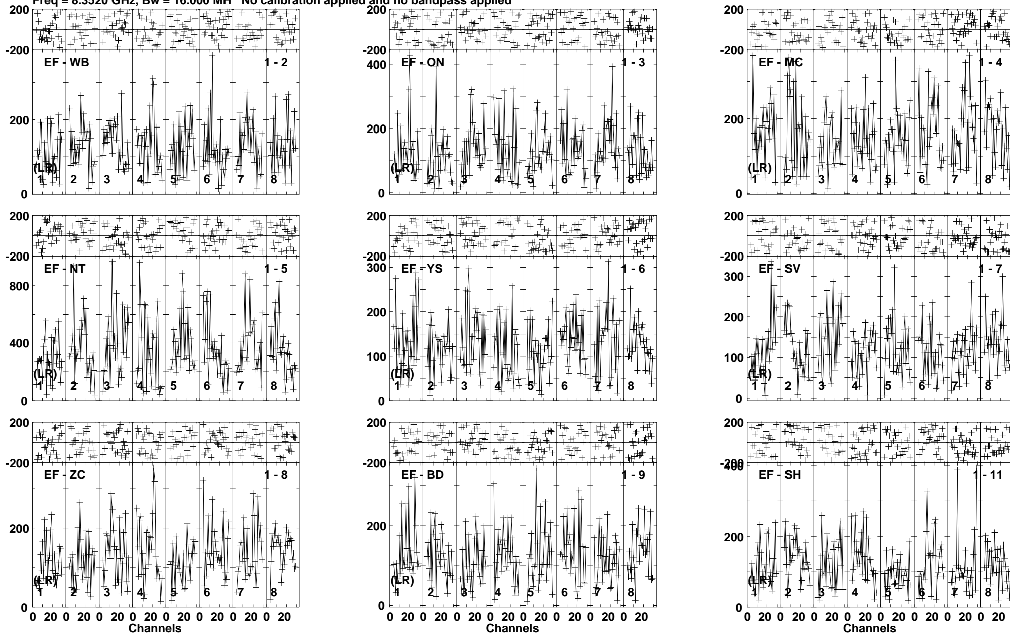
Lower frame: Micro Ampl Jy Top frame: Phas deg Vector averaged cross-power spectrum Baseline: EF (01) - WB (02) Timerange: 00/02:39:43 to 00/02:42:40
