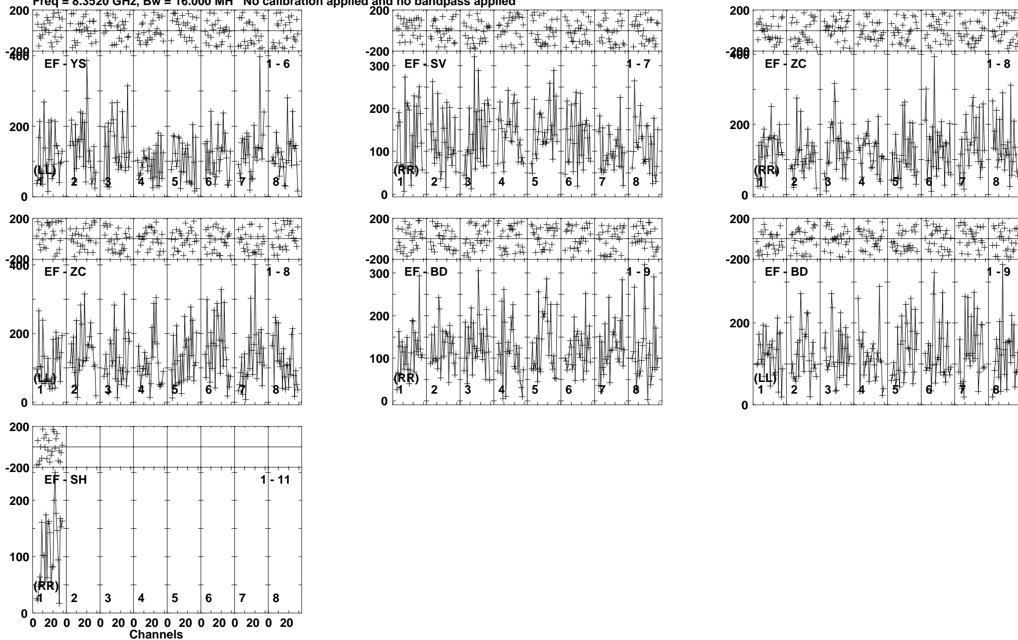
Lower frame: Micro Ampl Jy Top frame: Phas deg Vector averaged cross-power spectrum Baseline: EF (01) - YS (06) Timerange: 00/03:25:01 to 00/03:27:59
