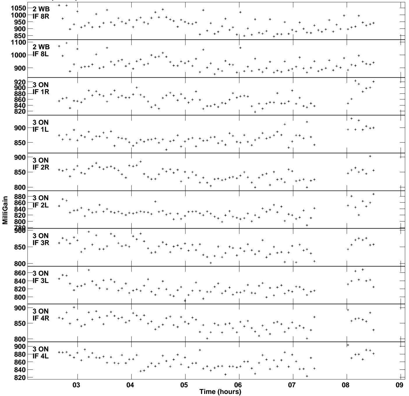
Plot file version 4 created 24-MAR-2014 14:20:49 Gain amp vs UTC time for J1128+5925.MULTI.1 SN 2 Rpol & Lpol IF 1 - 8
