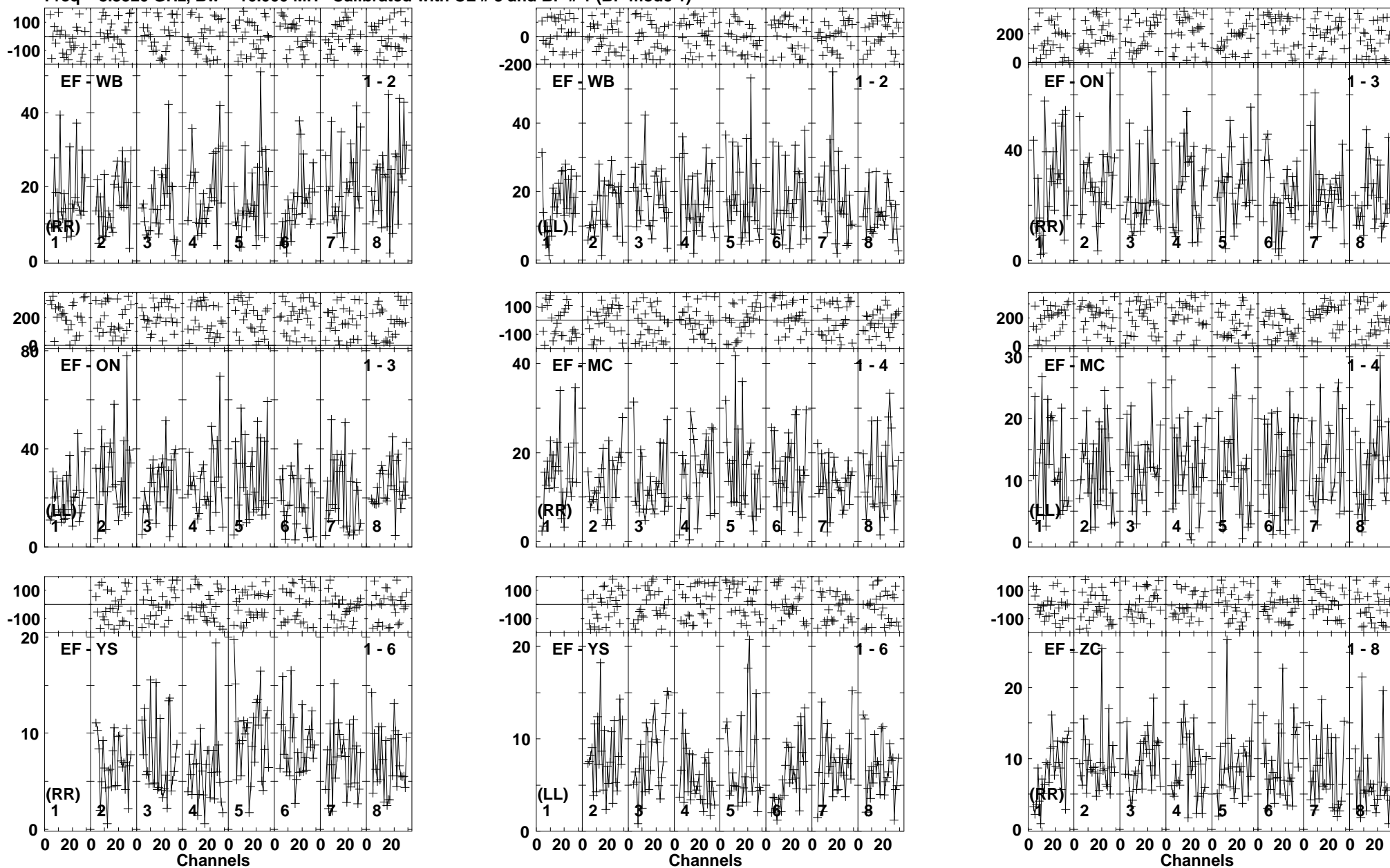
Lower frame: Milli Ampl Jy Top frame: Phas deg Vector averaged cross-power spectrum Baseline: EF (01) - WB (02) Timerange: 00/05:16:30 to 00/05:19:24
