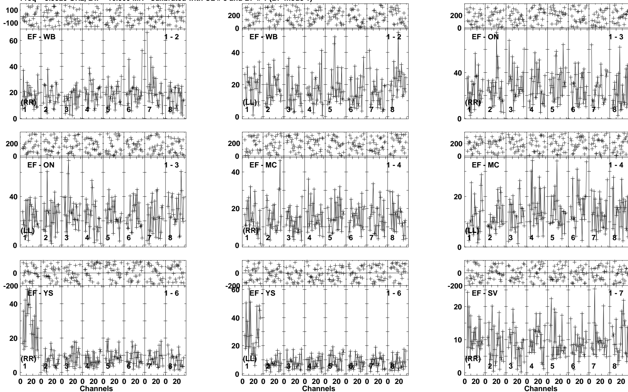
Lower frame: Milli Ampl Jy Top frame: Phas deg Vector averaged cross-power spectrum Baseline: EF (01) - WB (02) Timerange: 00/03:16:46 to 00/03:19:44
