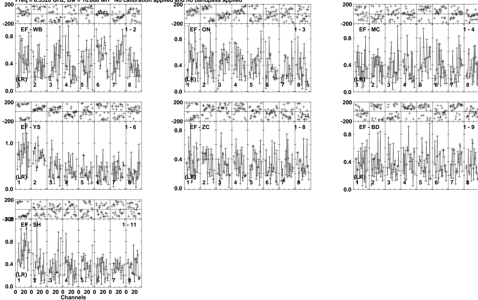
Lower frame: Milli Ampl Jy Top frame: Phas deg Vector averaged cross-power spectrum Baseline: EF (01) - WB (02) Timerange: 00/05:15:55 to 00/05:16:24
