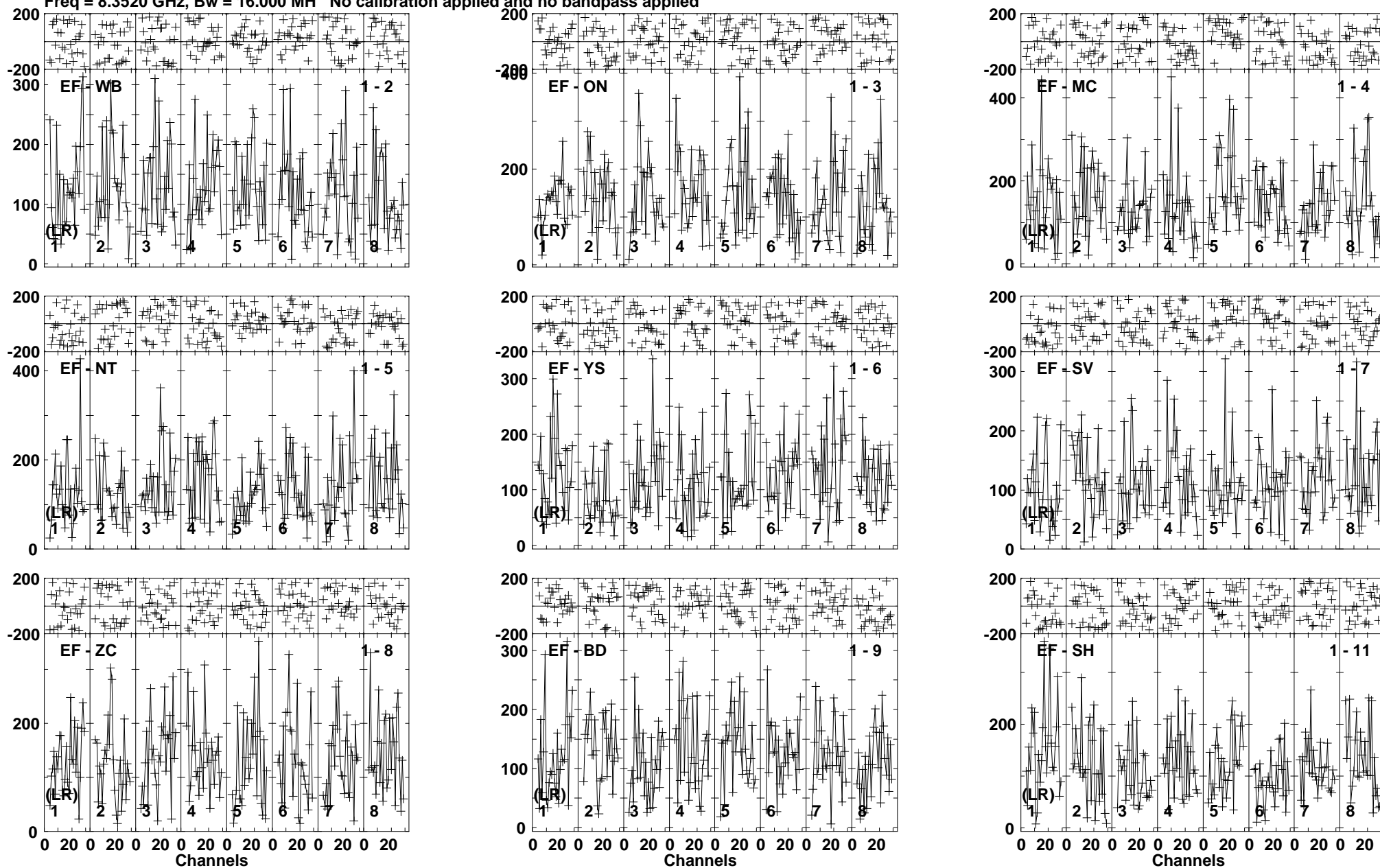
Lower frame: Micro Ampl Jy Top frame: Phas deg Vector averaged cross-power spectrum Baseline: EF (01) - WB (02) Timerange: 00/03:12:45 to 00/03:15:39
