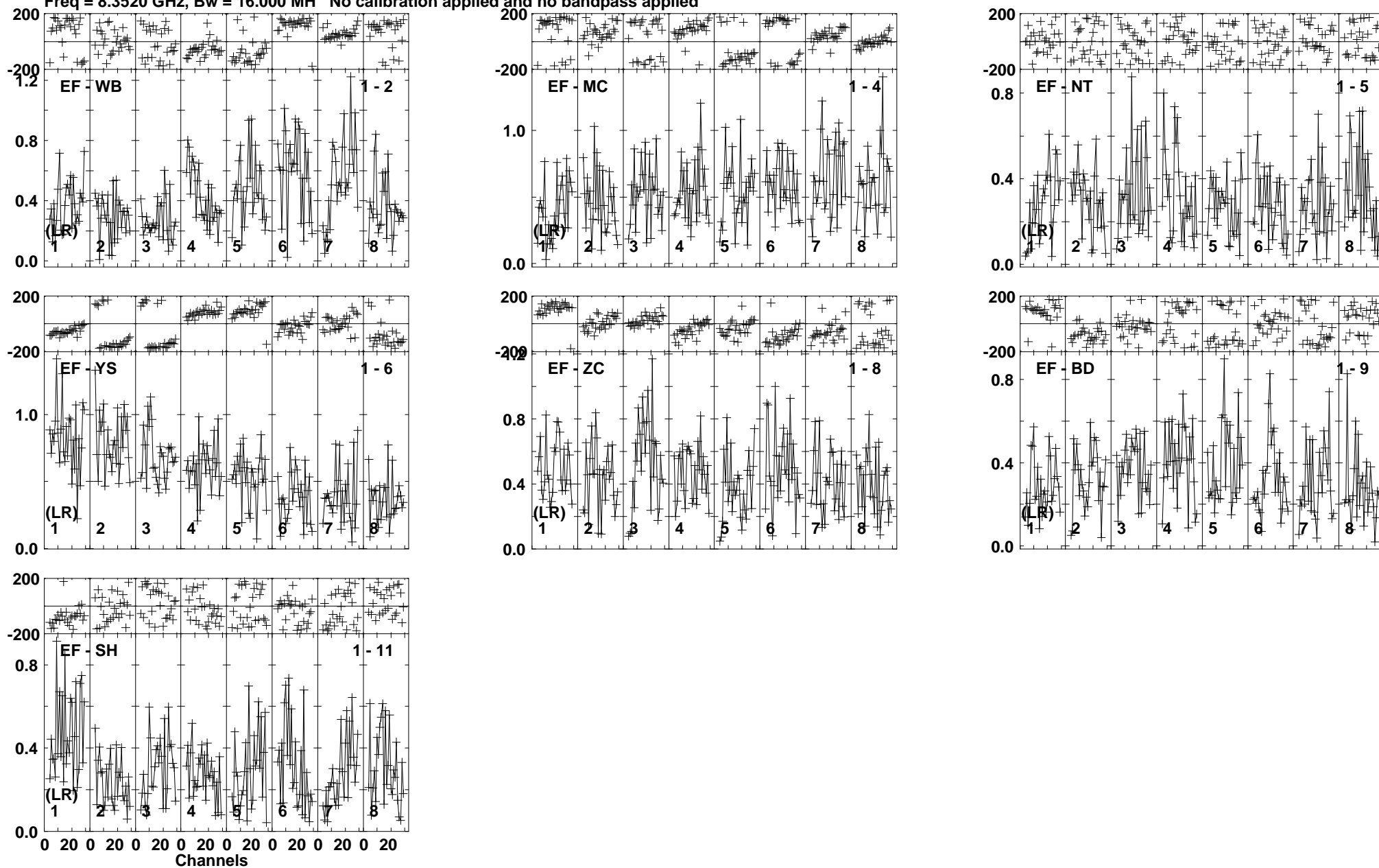
Lower frame: Milli Ampl Jy Top frame: Phas deg Vector averaged cross-power spectrum Baseline: EF (01) - WB (02) Timerange: 00/07:47:59 to 00/07:49:00
