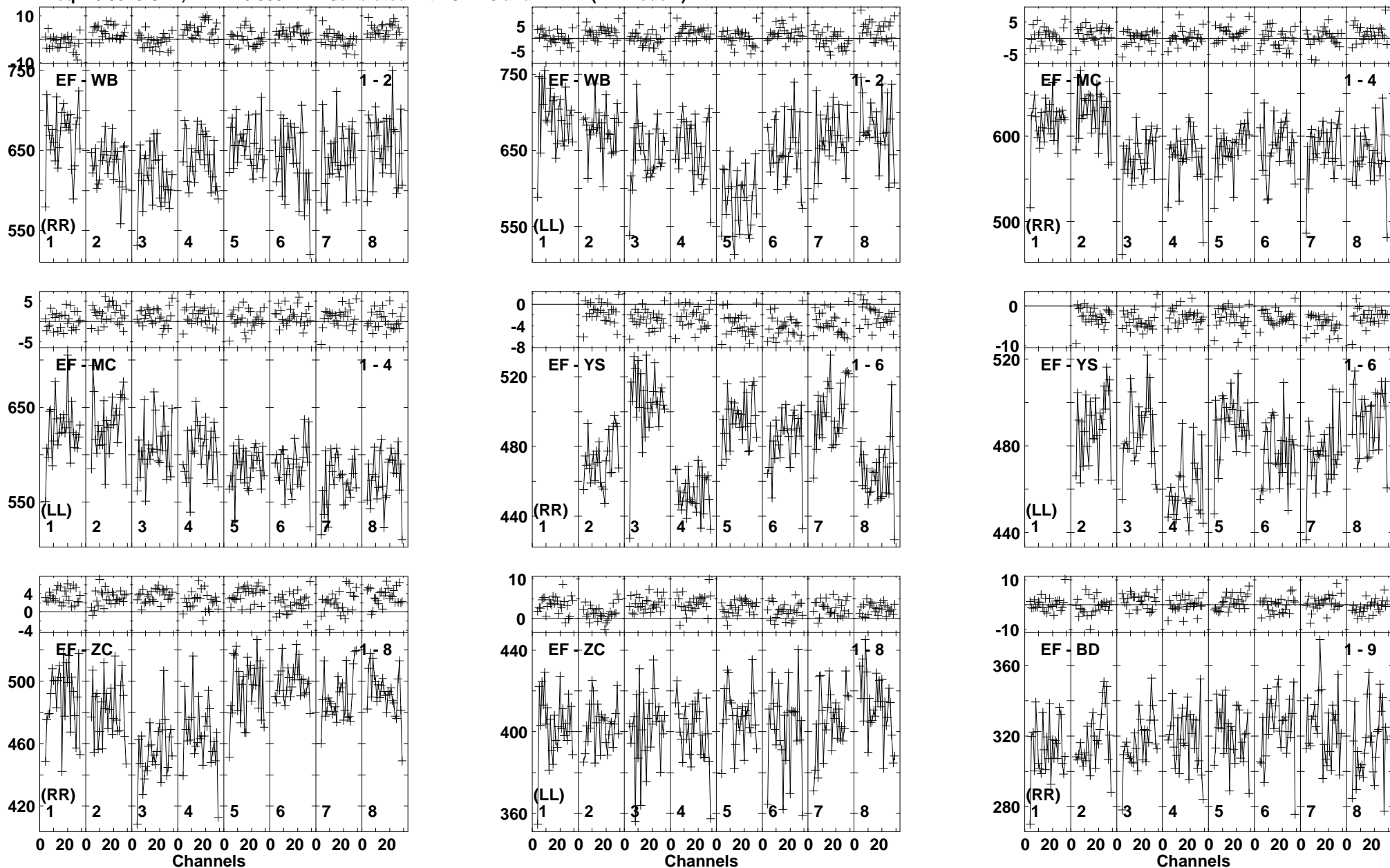
Lower frame: Milli Ampl Jy Top frame: Phas deg Vector averaged cross-power spectrum Baseline: EF (01) - WB (02) Timerange: 00/07:31:29 to 00/07:32:29
