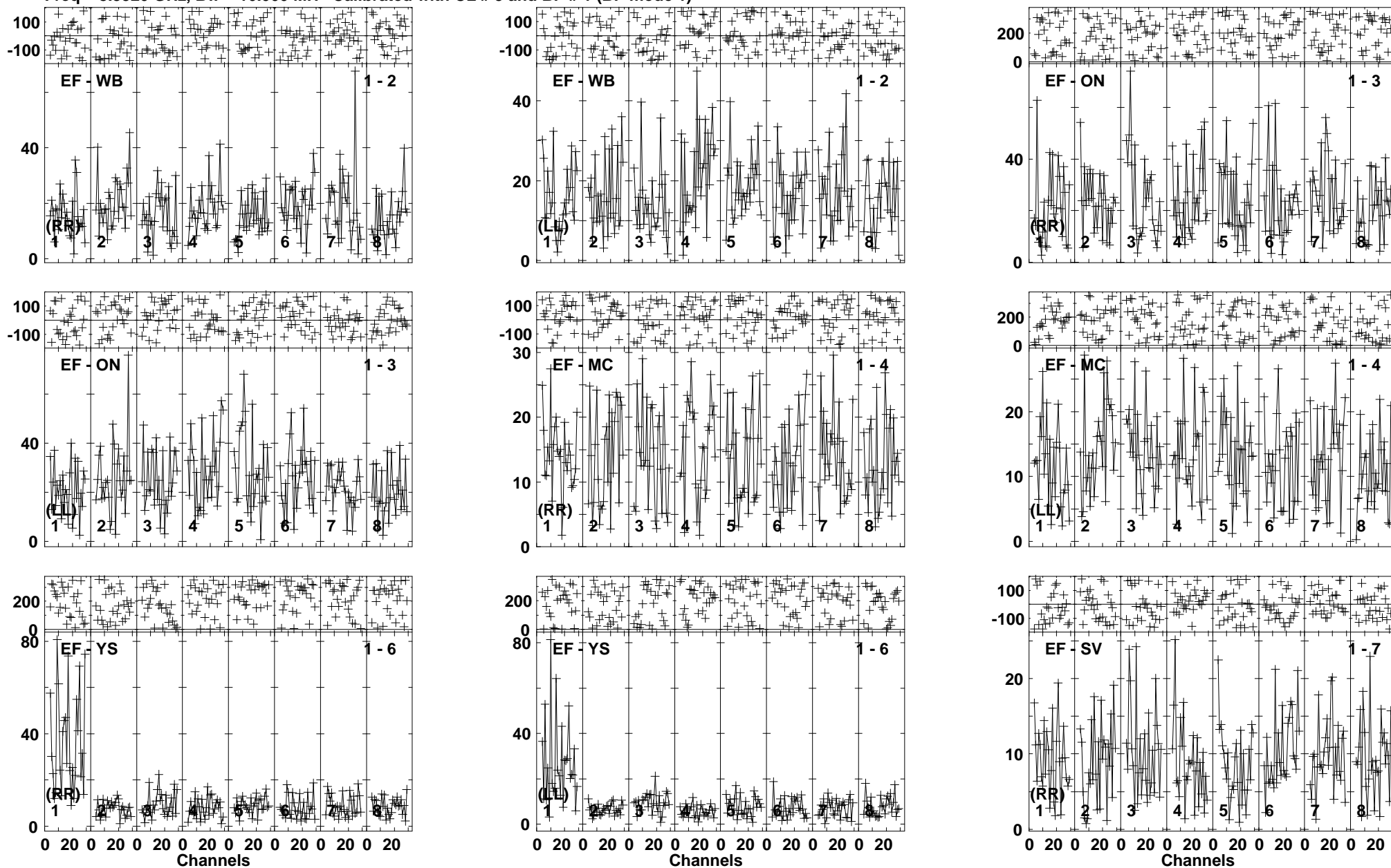
Lower frame: Milli Ampl Jy Top frame: Phas deg Vector averaged cross-power spectrum Baseline: EF (01) - WB (02) Timerange: 00/04:47:30 to 00/04:50:30
