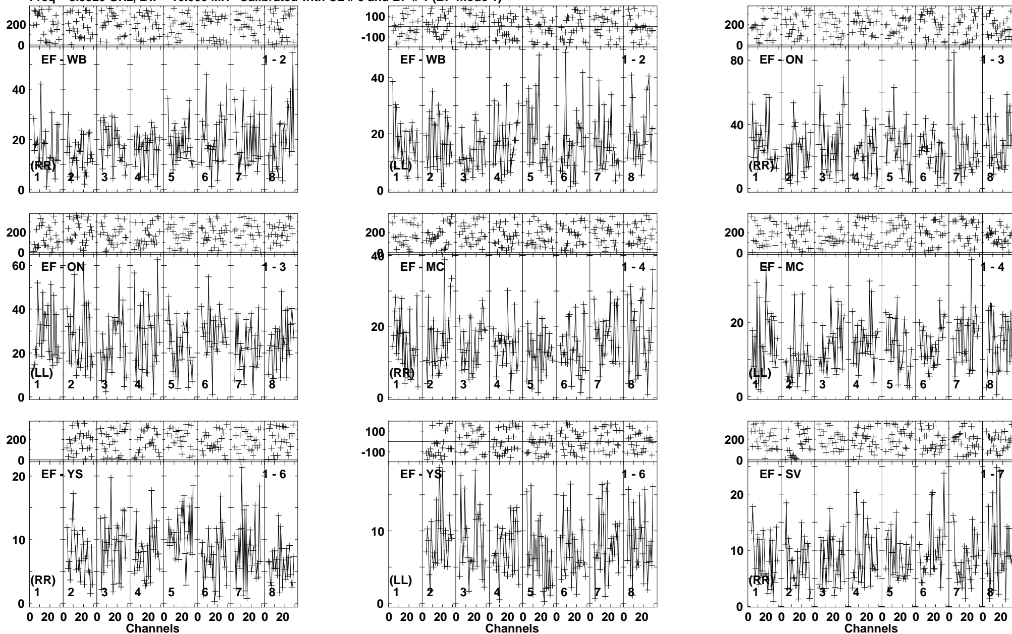
Lower frame: Milli Ampl Jy Top frame: Phas deg Vector averaged cross-power spectrum Baseline: EF (01) - WB (02) Timerange: 00/02:56:15 to 00/02:59:09
