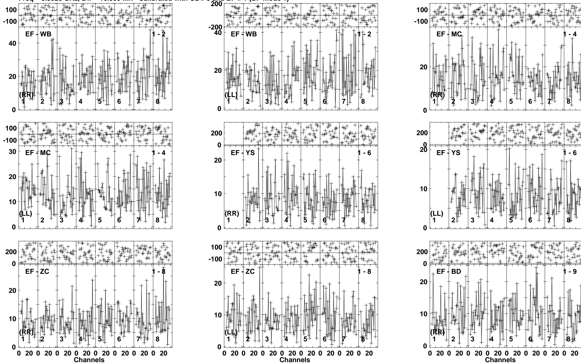
Lower frame: Milli Ampl Jy Top frame: Phas deg Vector averaged cross-power spectrum Baseline: EF (01) - WB (02) Timerange: 00/07:28:29 to 00/07:31:25
