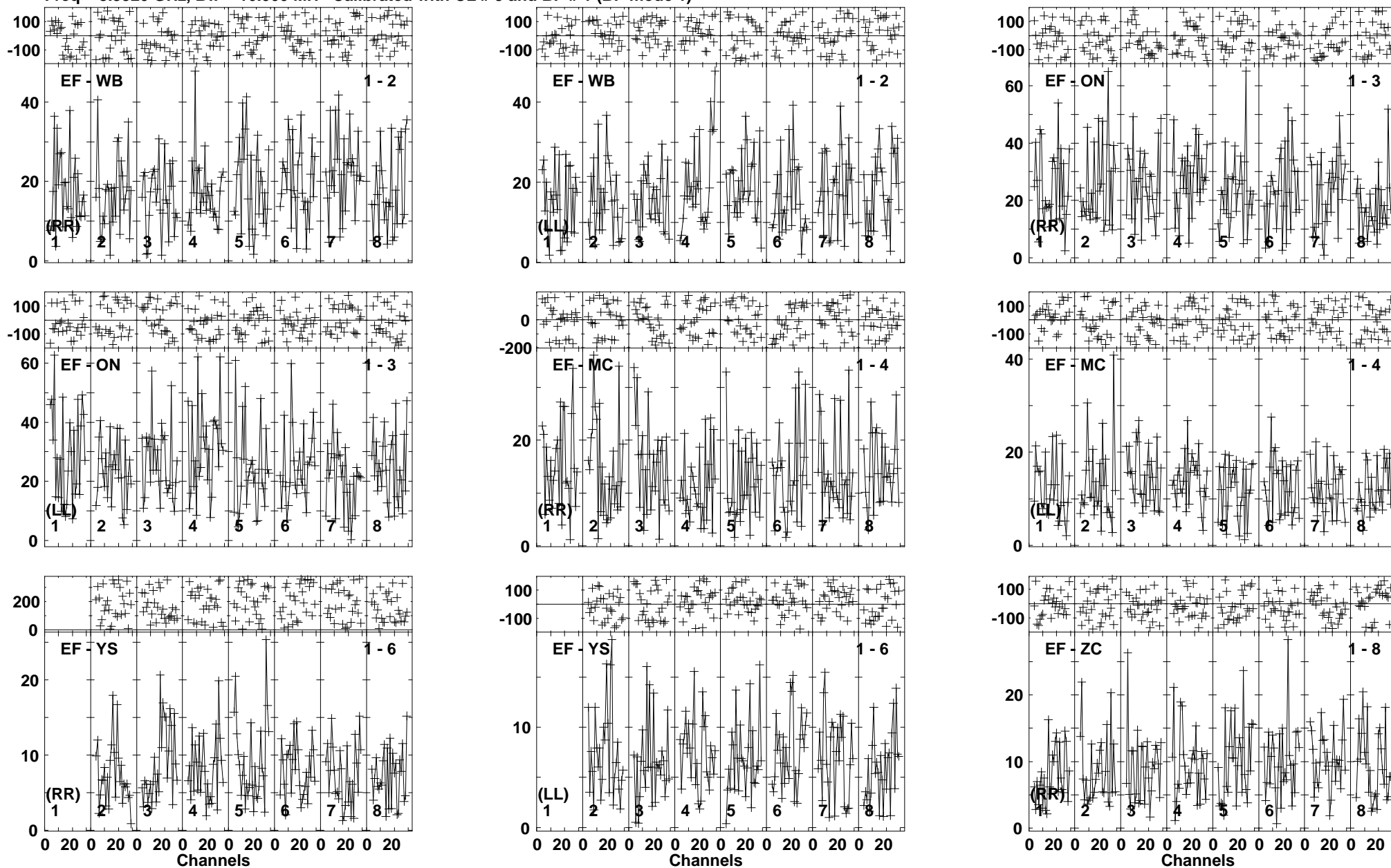
Lower frame: Milli Ampl Jy Top frame: Phas deg Vector averaged cross-power spectrum Baseline: EF (01) - WB (02) Timerange: 00/06:55:29 to 00/06:58:25
