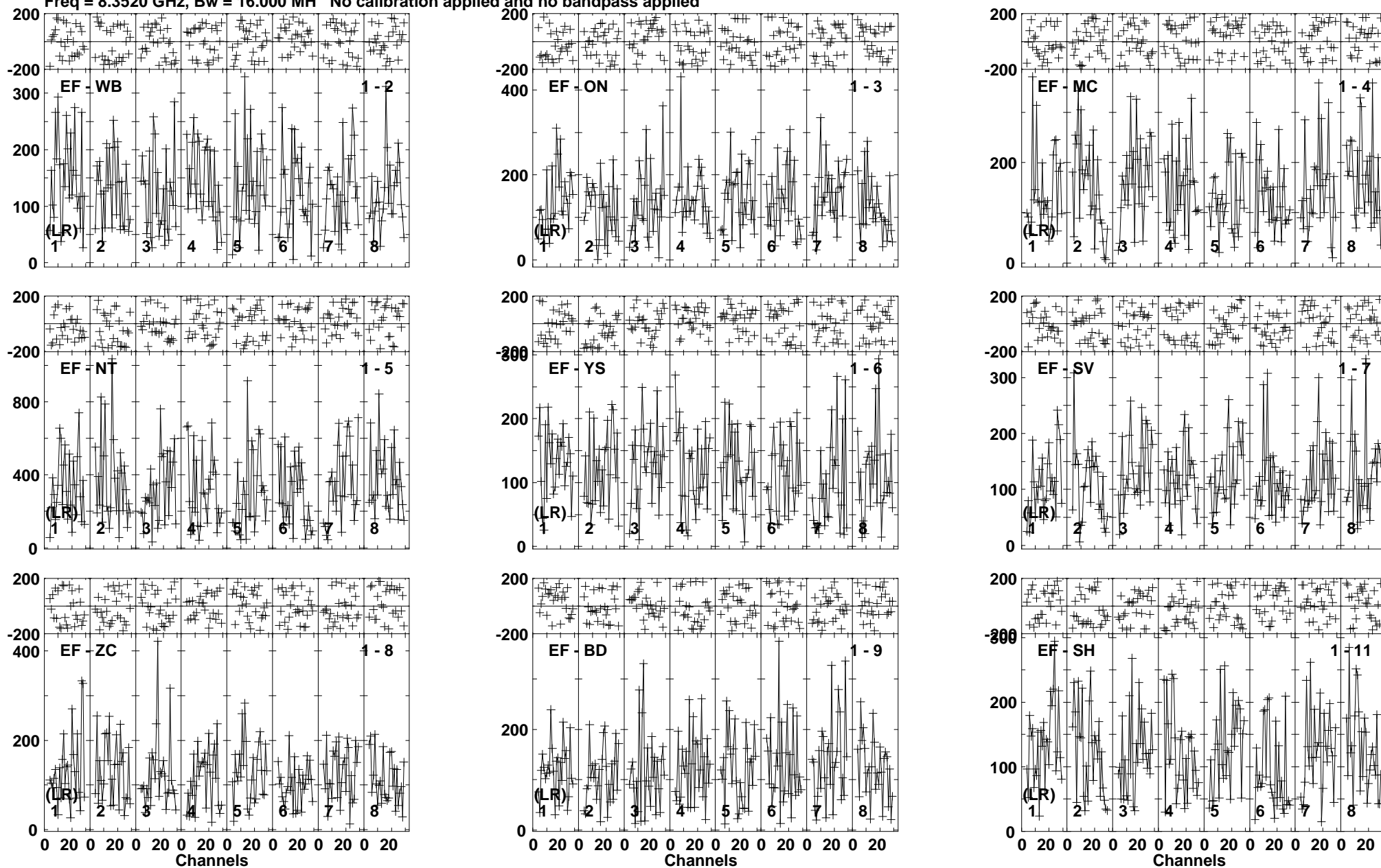
Lower frame: Micro Ampl Jy Top frame: Phas deg Vector averaged cross-power spectrum Baseline: EF (01) - WB (02) Timerange: 00/03:00:15 to 00/03:03:15
