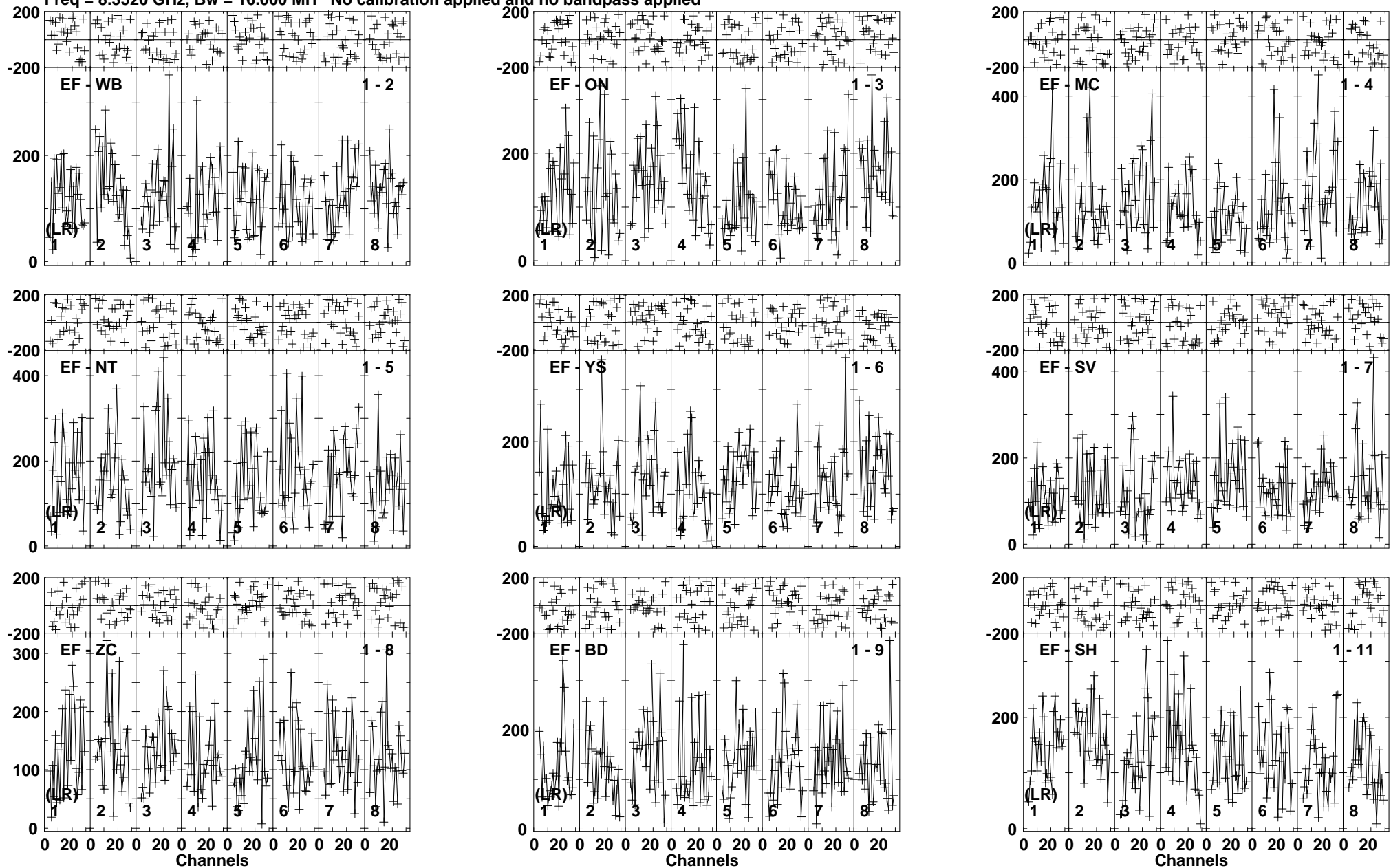
Lower frame: Micro Ampl Jy Top frame: Phas deg Vector averaged cross-power spectrum Baseline: EF (01) - WB (02) Timerange: 00/04:43:29 to 00/04:46:25
