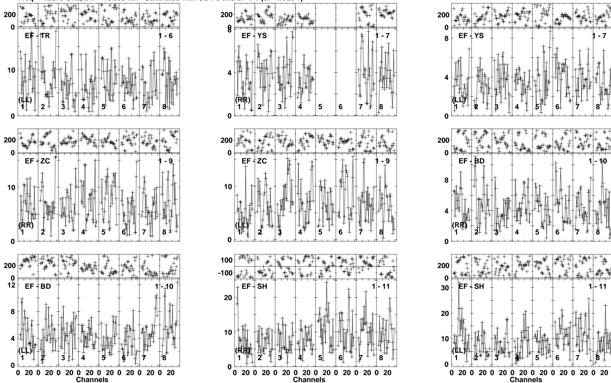
Lower frame: Milli Ampl Jy Top frame: Phas deg Vector averaged cross-power spectrum Baseline: EF (01) - TR (06) Timerange: 00/17:21:21 to 00/17:25:19
