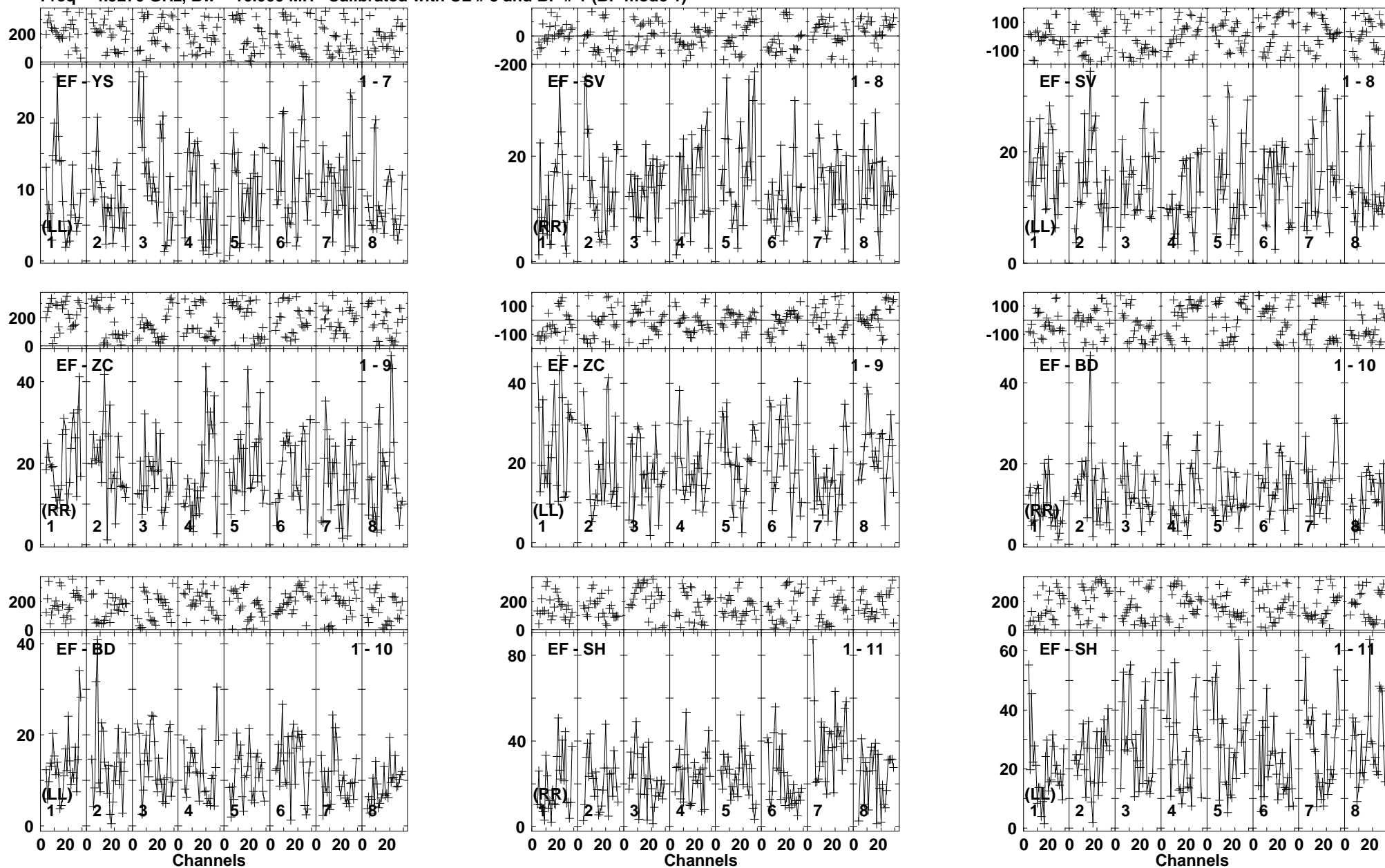
Lower frame: Milli Ampl Jy Top frame: Phas deg Vector averaged cross-power spectrum Baseline: EF (01) - YS (07) Timerange: 00:12:43:35 to 00:12:47:19
