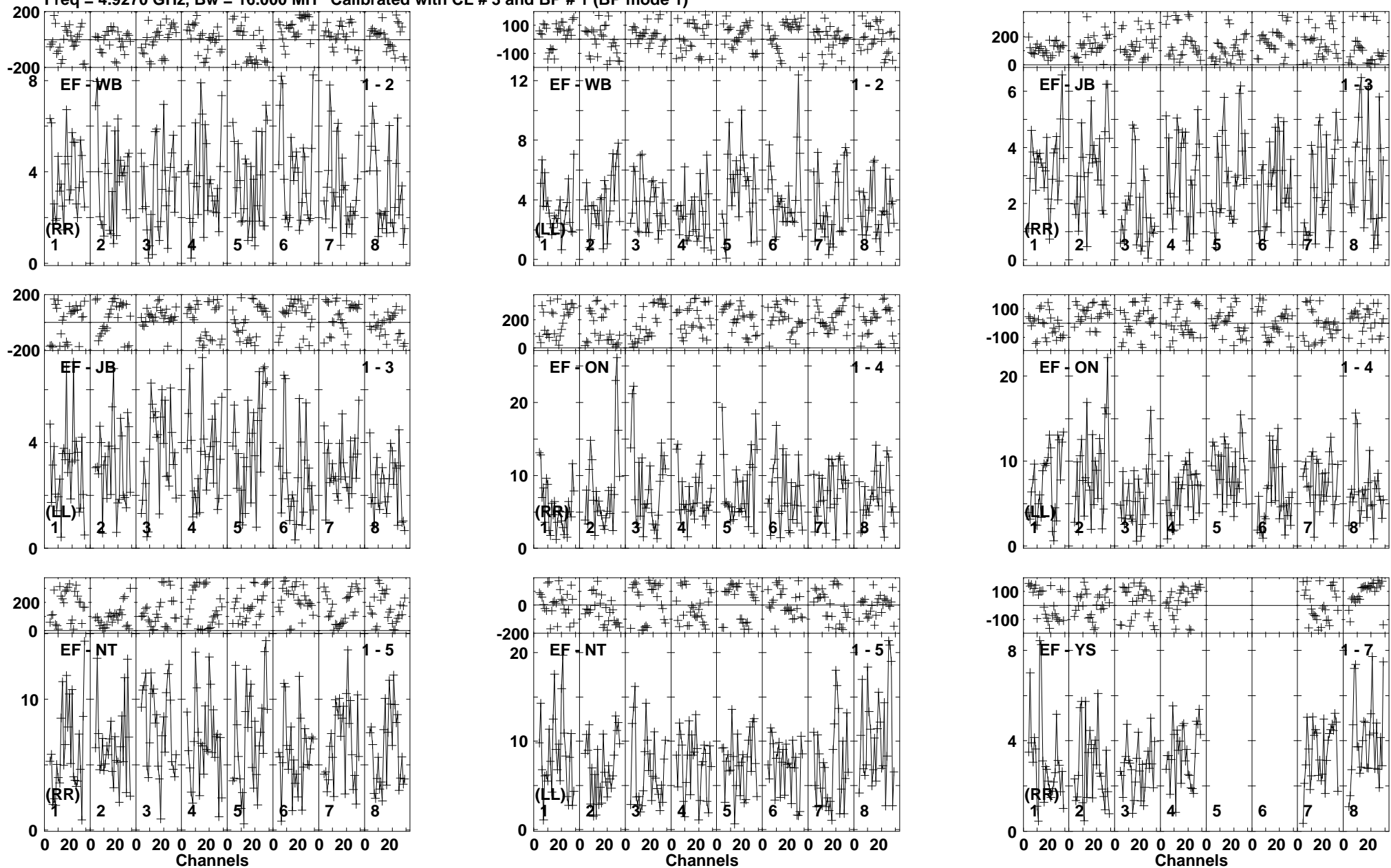
Lower frame: Milli Ampl Jy Top frame: Phas deg Vector averaged cross-power spectrum Baseline: EF (01) - WB (02) Timerange: 00/13:13:45 to 00/13:17:39
