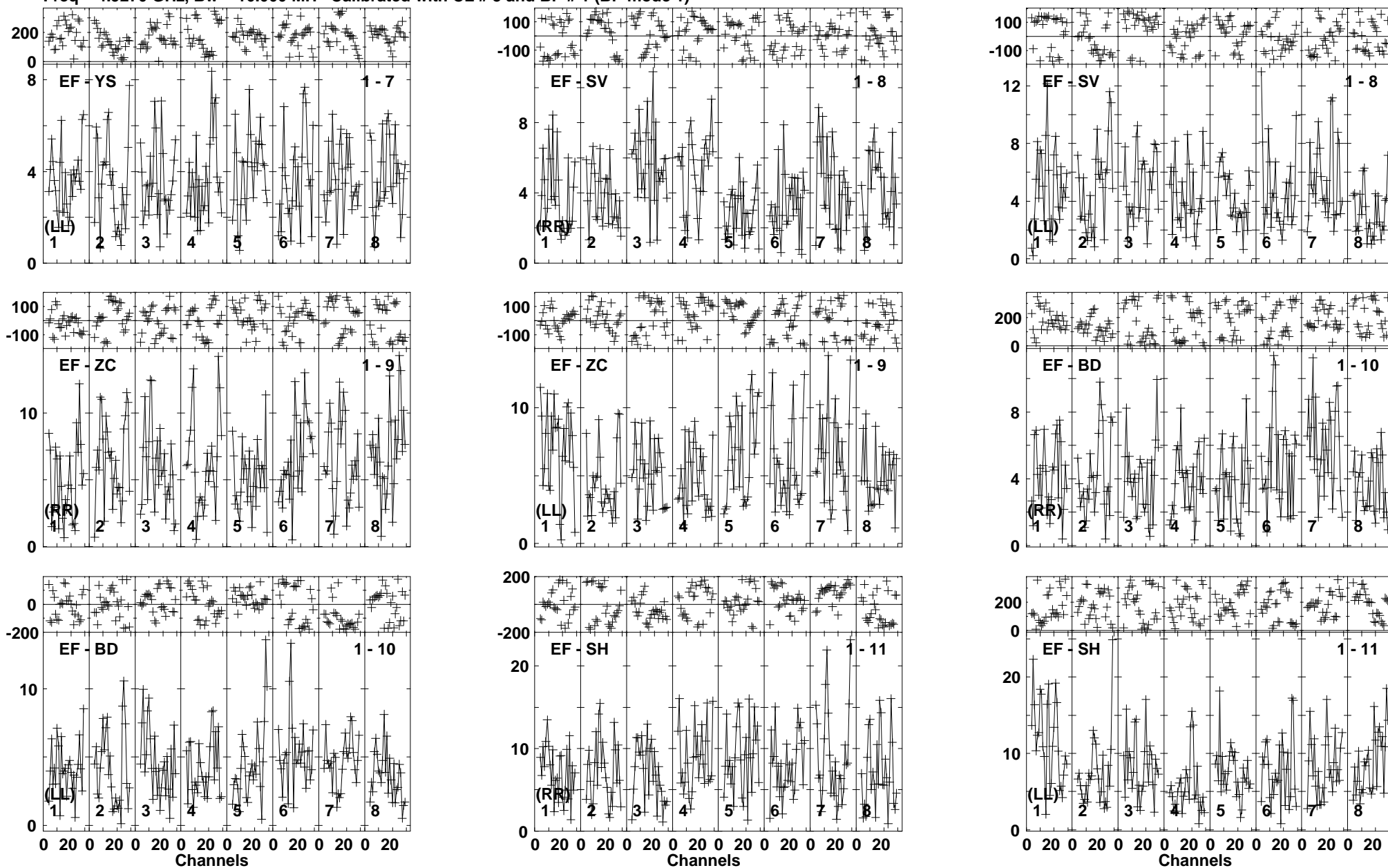
Lower frame: Milli Ampl Jy Top frame: Phas deg Vector averaged cross-power spectrum Baseline: EF (01) - YS (07) Timerange: 00/14:14:25 to 00/14:18:19
