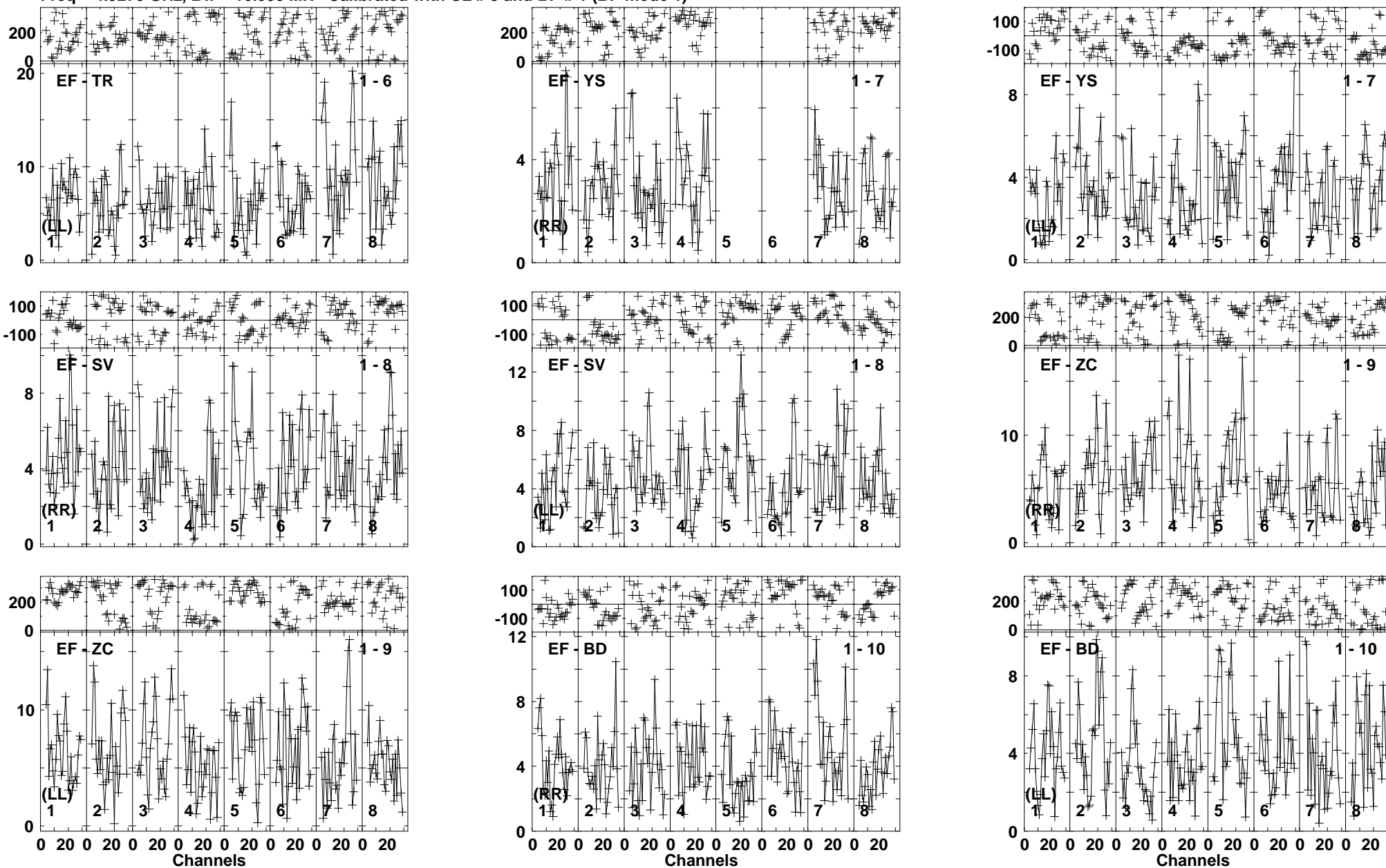
Lower frame: Milli Ampl Jy Top frame: Phas deg Vector averaged cross-power spectrum Baseline: EF (01) - TR (06) Timerange: 00/18:06:55 to 00/18:10:49
