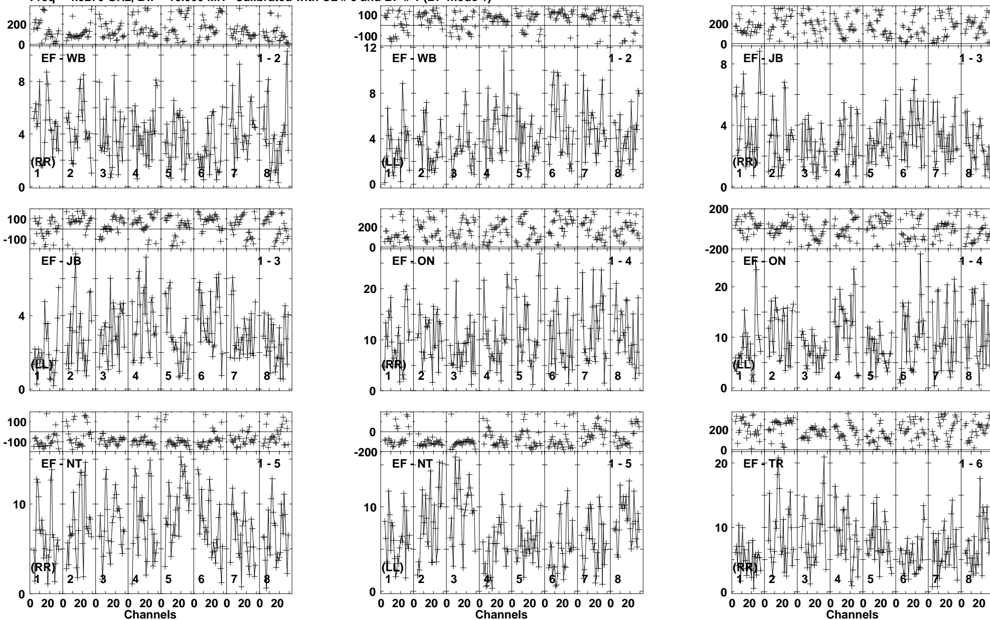
Lower frame: Milli Ampl Jy Top frame: Phas deg Vector averaged cross-power spectrum Baseline: EF (01) - WB (02) Timerange: 00/16:25:55 to 00/16:29:49
