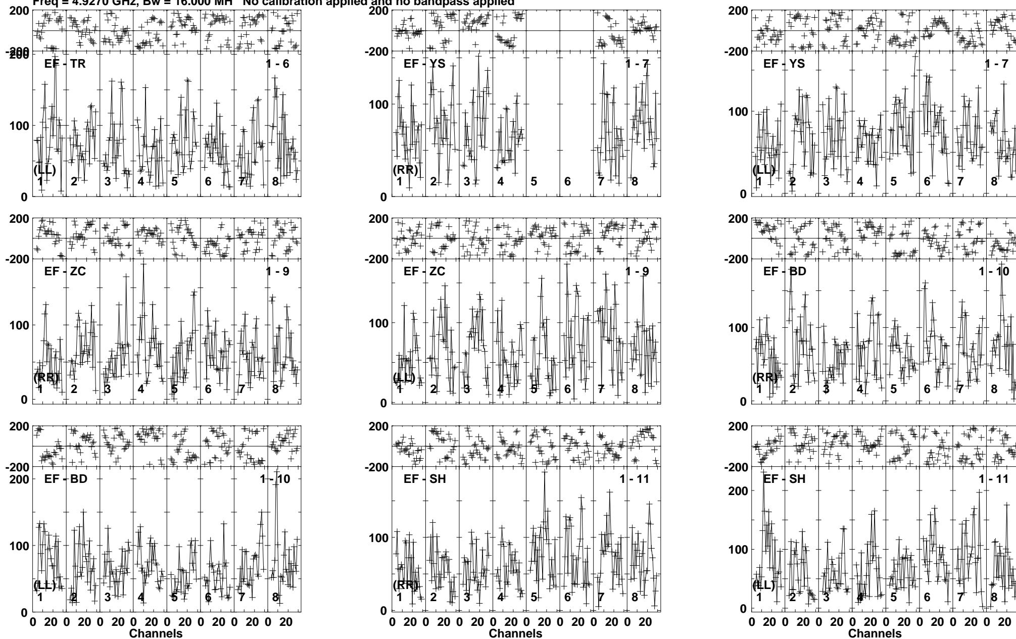
Lower frame: Micro Ampl Jy Top frame: Phas deg Vector averaged cross-power spectrum Baseline: EF (01) - TR (06) Timerange: 00/17:21:21 to 00/17:25:19
