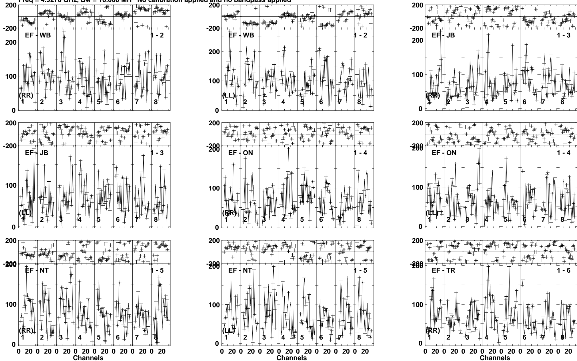
Lower frame: Micro Ampl Jy Top frame: Phas deg Vector averaged cross-power spectrum Baseline: EF (01) - WB (02) Timerange: 00/18:01:51 to 00/18:05:49
