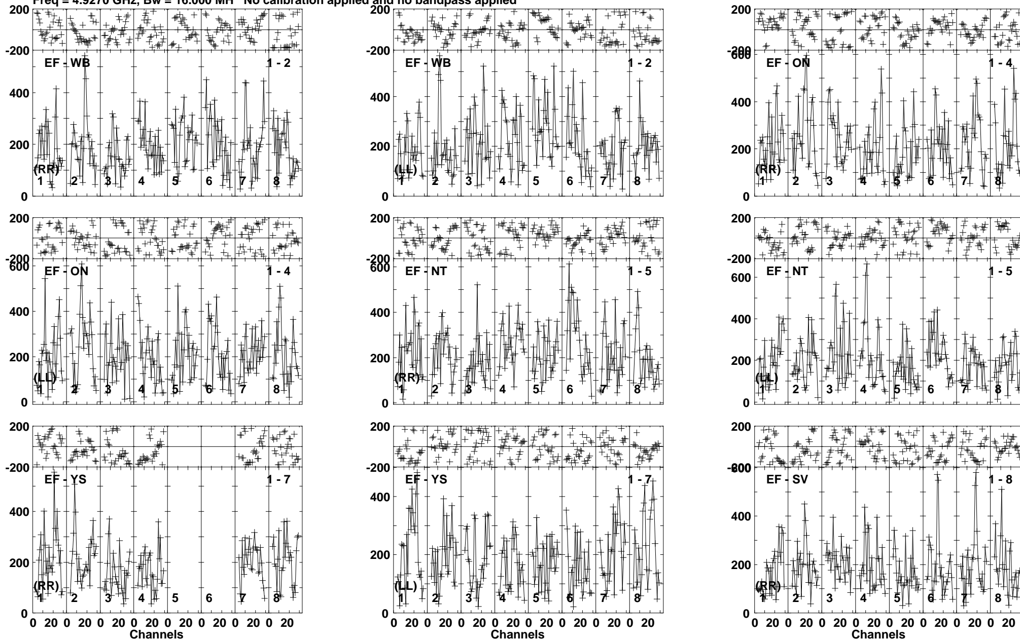
Lower frame: Micro Ampl Jy Top frame: Phas deg Vector averaged cross-power spectrum Baseline: EF (01) - WB (02) Timerange: 00/18:11:33 to 00/18:11:59
