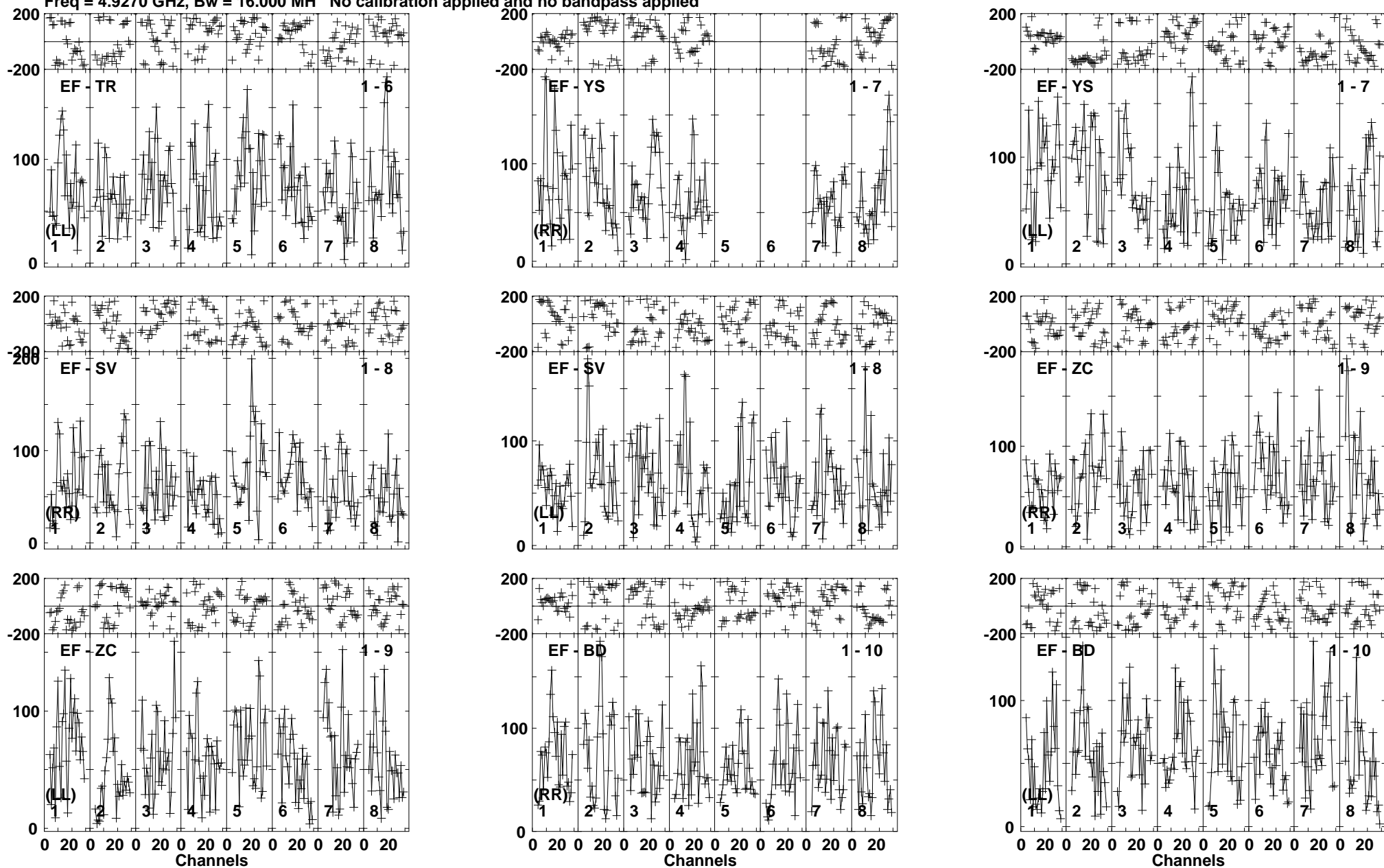
Lower frame: Micro Ampl Jy Top frame: Phas deg Vector averaged cross-power spectrum Baseline: EF (01) - TR (06) Timerange: 00/14:54:55 to 00/14:58:49
