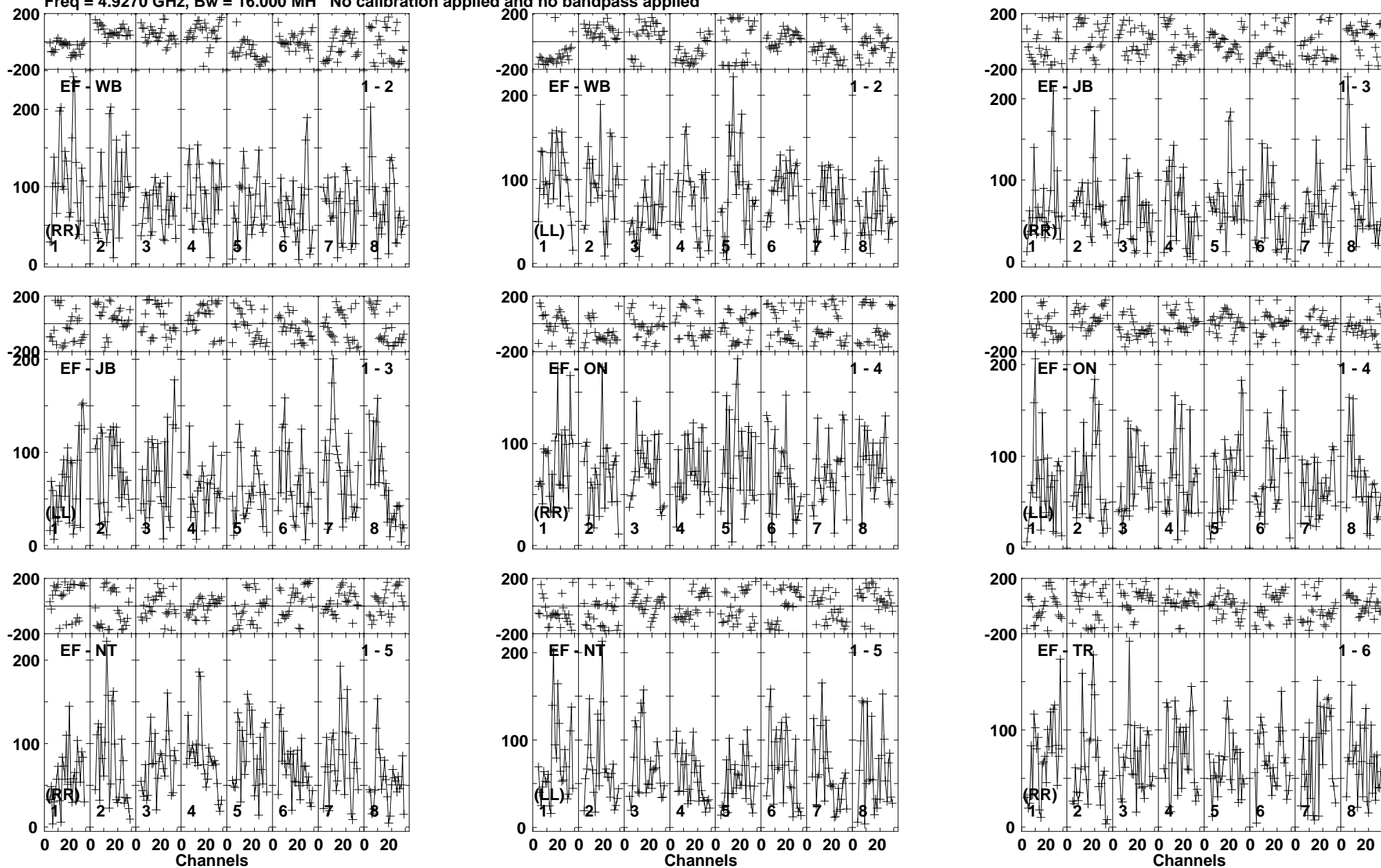
Lower frame: Micro Ampl Jy Top frame: Phas deg Vector averaged cross-power spectrum Baseline: EF (01) - WB (02) Timerange: 00/15:40:21 to 00/15:44:19
