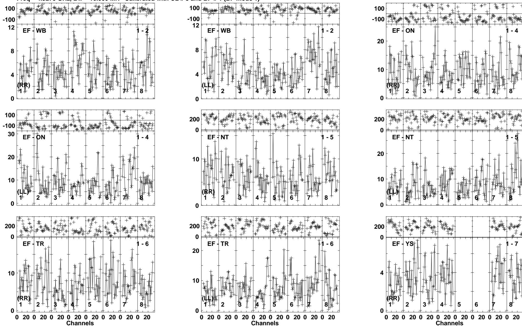
Lower frame: Milli Ampl Jy Top frame: Phas deg Vector averaged cross-power spectrum Baseline: EF (01) - WB (02) Timerange: 00/12:53:35 to 00/12:57:29
