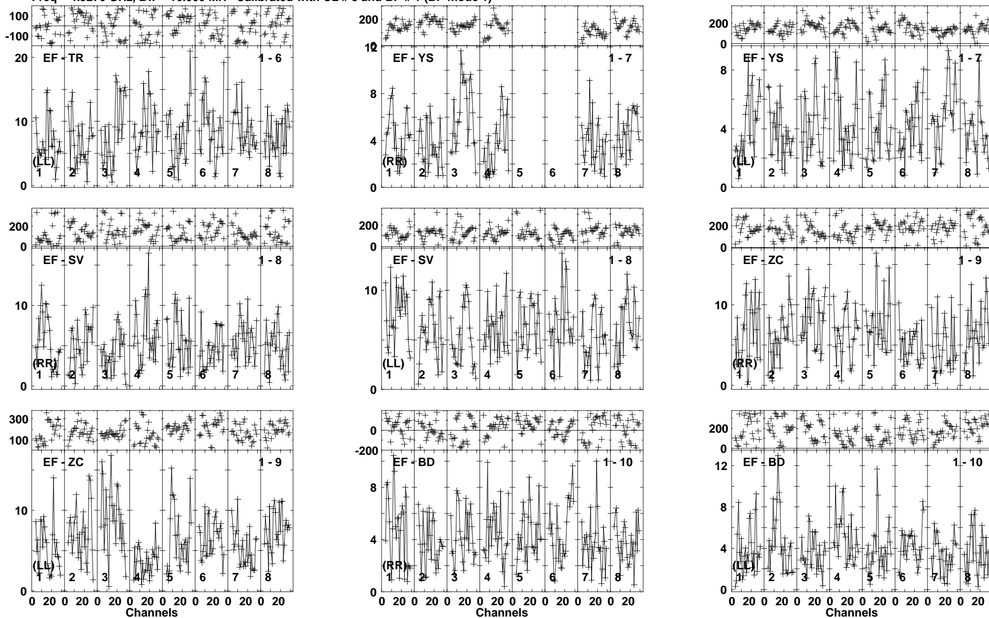
Lower frame: Milli Ampl Jy Top frame: Phas deg Vector averaged cross-power spectrum Baseline: EF (01) - TR (06) Timerange: 00/17:46:45 to 00/17:50:39
