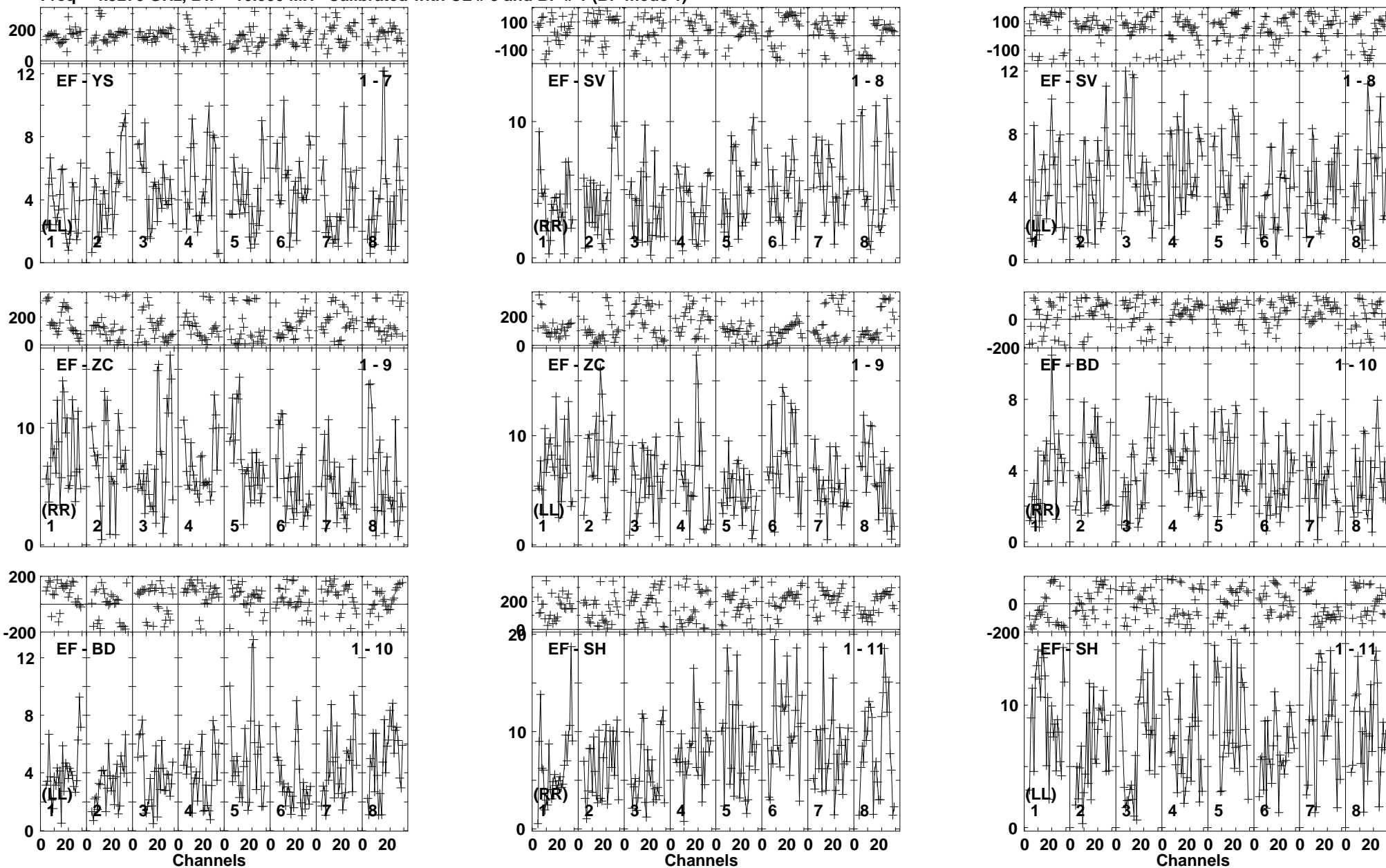
Lower frame: Milli Ampl Jy Top frame: Phas deg Vector averaged cross-power spectrum Baseline: EF (01) - YS (07) Timerange: 00/13:13:45 to 00/13:17:39
