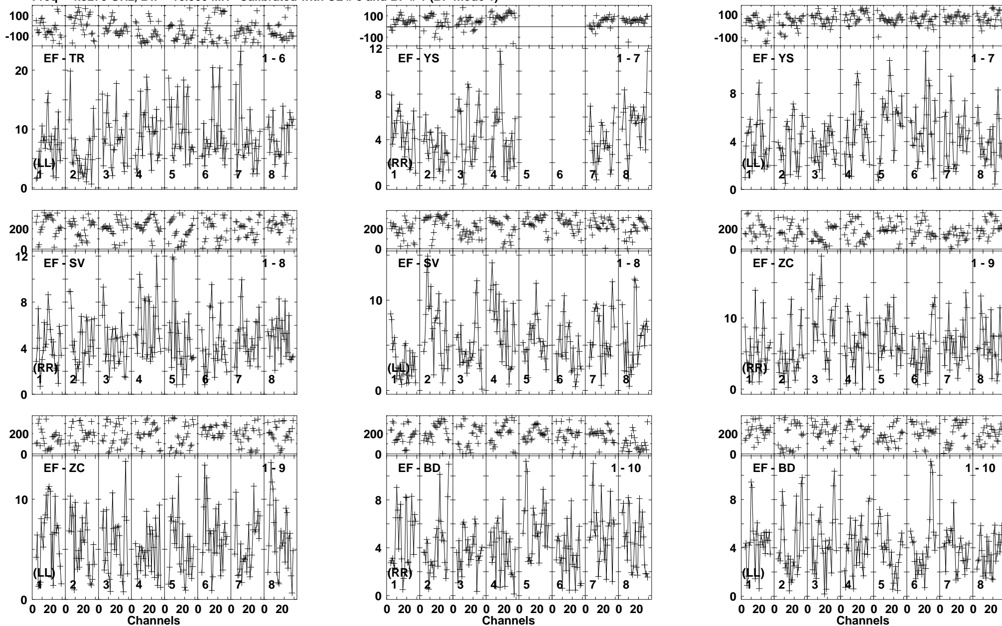
Lower frame: Milli Ampl Jy Top frame: Phas deg Vector averaged cross-power spectrum Baseline: EF (01) - TR (06) Timerange: 00/13:39:01 to 00/13:42:59
