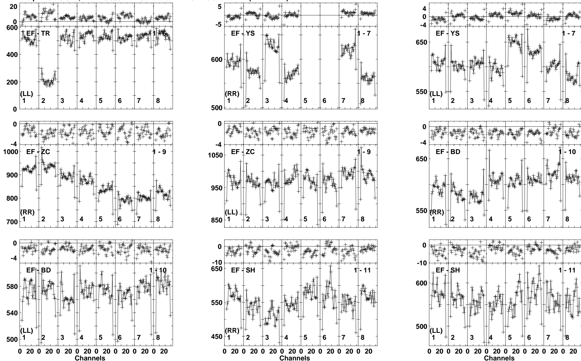
Lower frame: Milli Ampl Jy Top frame: Phas deg Vector averaged cross-power spectrum Baseline: EF (01) - TR (06) Timerange: 00/17:26:01 to 00/17:26:29
