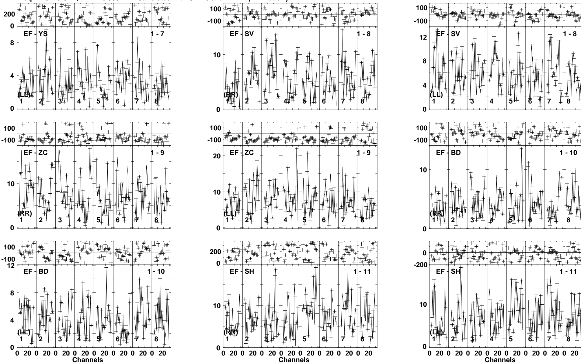
Lower frame: Milli Ampl Jy Top frame: Phas deg Vector averaged cross-power spectrum Baseline: EF (01) - YS (07) Timerange: 00/12:48:25 to 00/12:52:19
