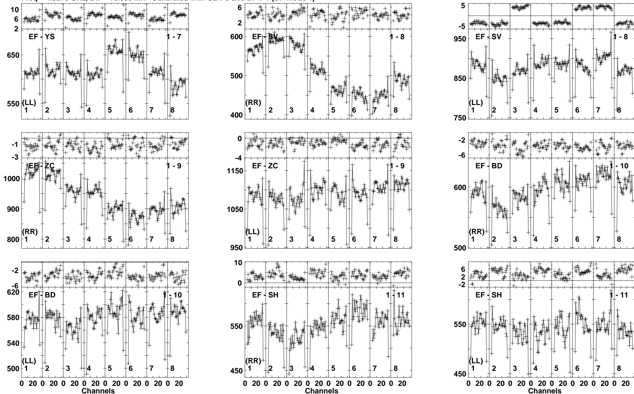
Lower frame: Milli Ampl Jy Top frame: Phas deg Vector averaged cross-power spectrum Baseline: EF (01) - YS (07) Timerange: 00/13:17:45 to 00/13:18:39
