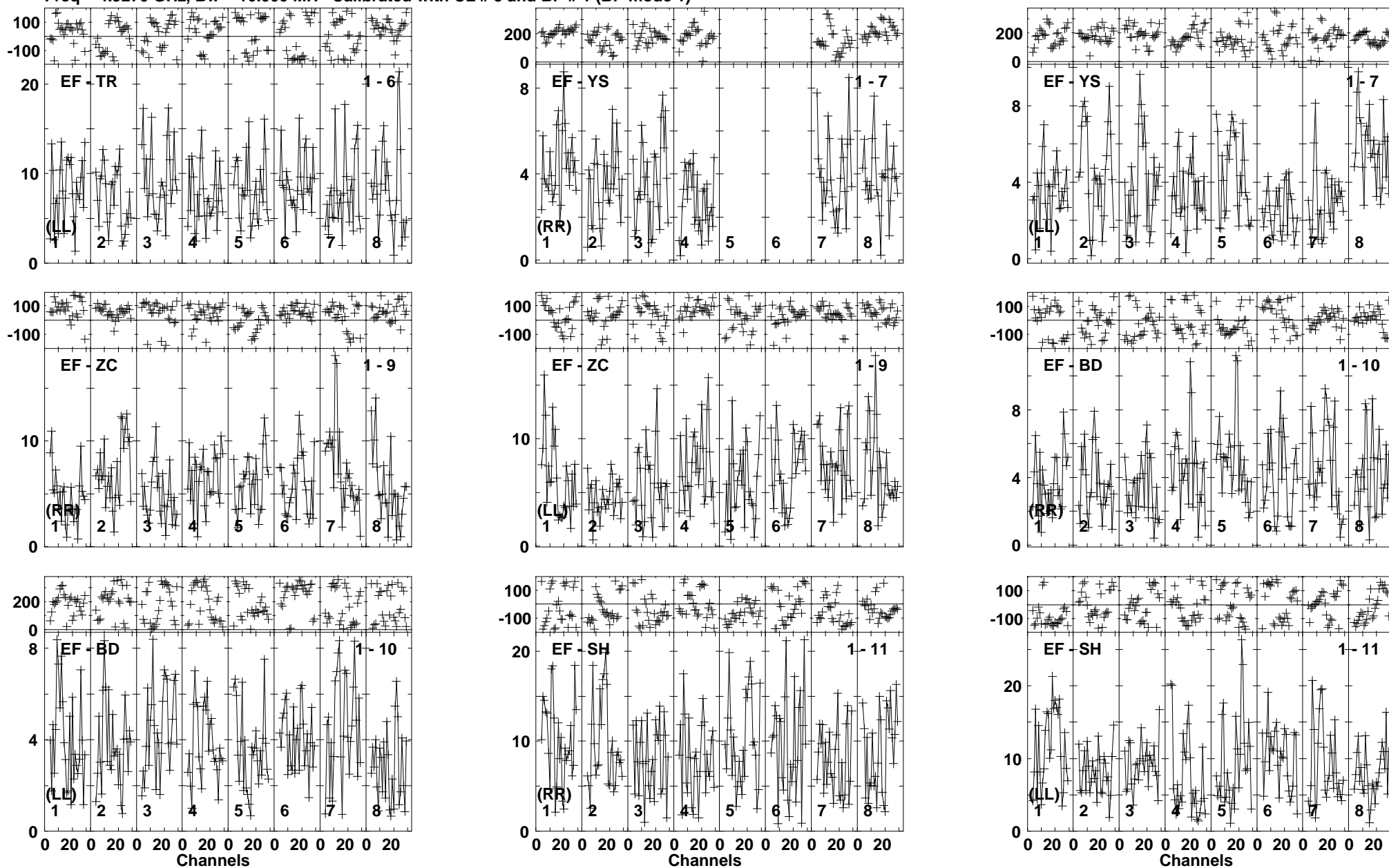
Lower frame: Milli Ampl Jy Top frame: Phas deg Vector averaged cross-power spectrum Baseline: EF (01) - TR (06) Timerange: 00/17:26:35 to 00/17:30:29
