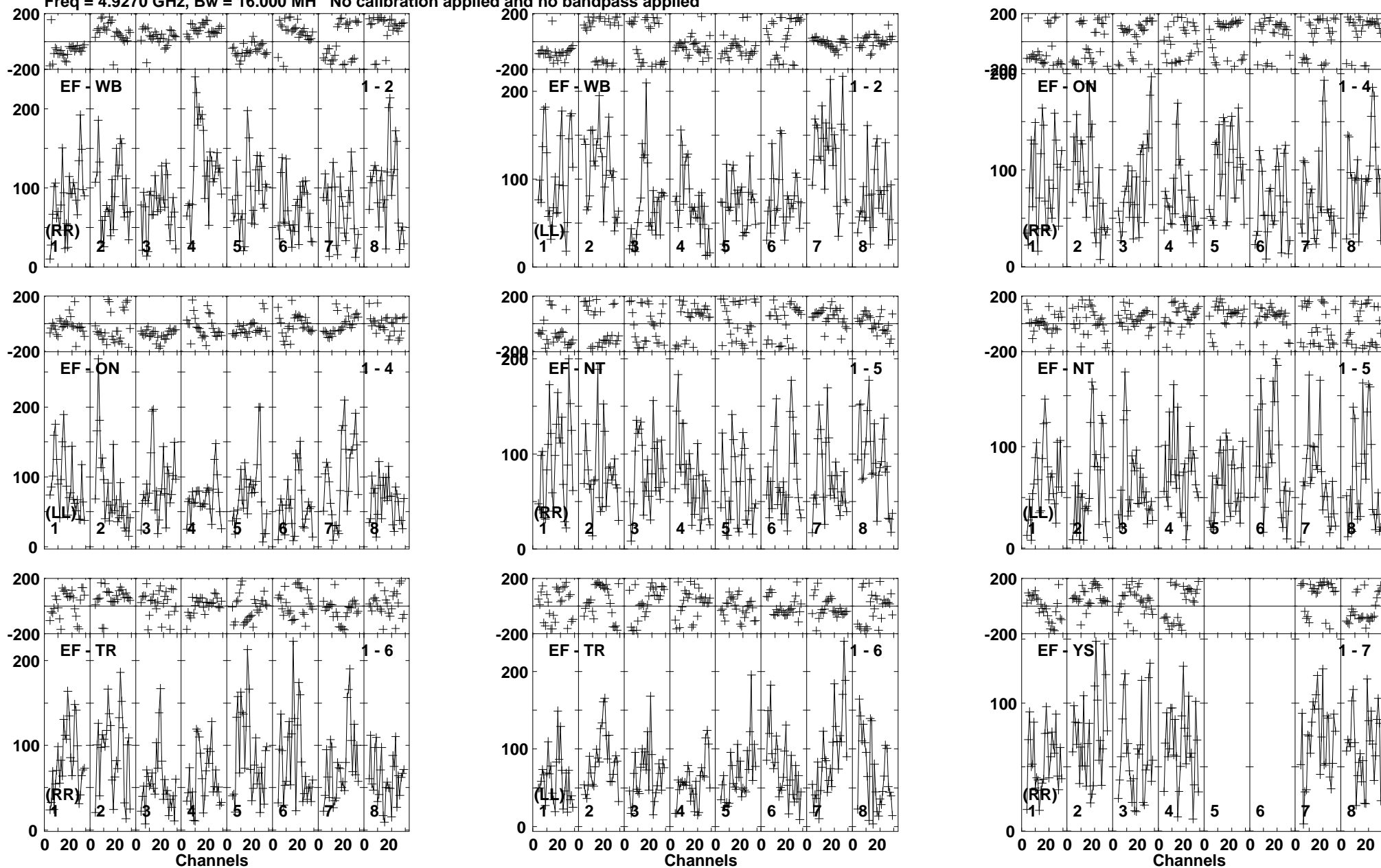
Lower frame: Micro Ampl Jy Top frame: Phas deg Vector averaged cross-power spectrum Baseline: EF (01) - WB (02) Timerange: 00:12:53:35 to 00:12:57:29
