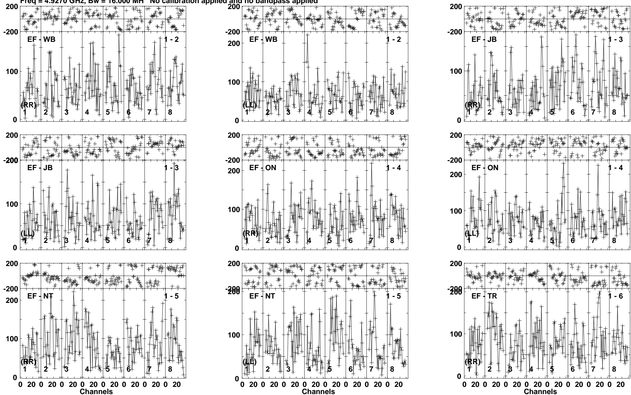
Lower frame: Micro Ampl Jy Top frame: Phas deg Vector averaged cross-power spectrum Baseline: EF (01) - WB (02) Timerange: 00/13:28:51 to 00/13:32:49
