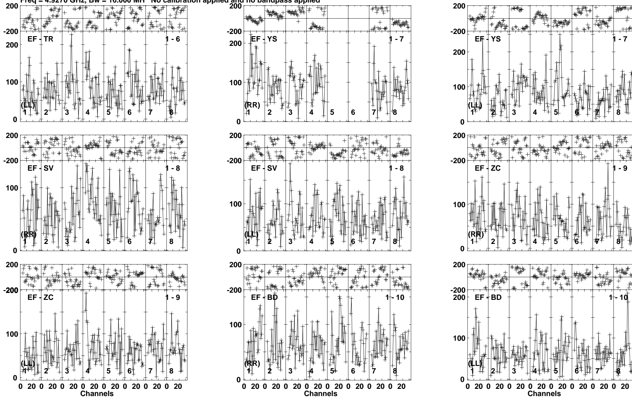
Lower frame: Micro Ampl Jy Top frame: Phas deg Vector averaged cross-power spectrum Baseline: EF (01) - TR (06) Timerange: 00/14:24:35 to 00/14:28:29
