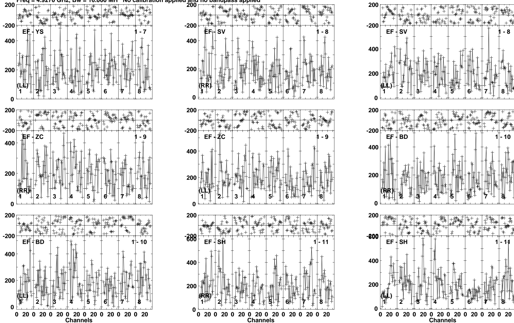
Lower frame: Micro Ampl Jy Top frame: Phas deg Vector averaged cross-power spectrum Baseline: EF (01) - YS (07) Timerange: 00/12:43:35 to 00/12:47:19
