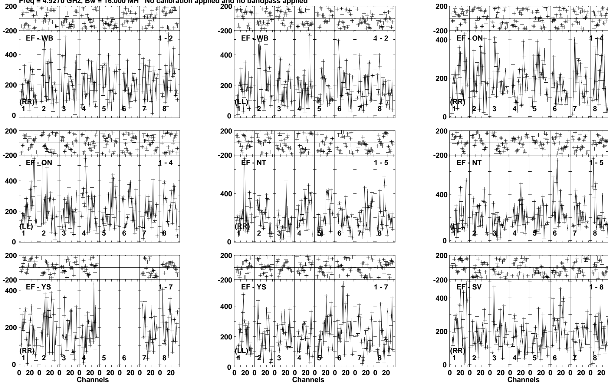
Lower frame: Micro Ampl Jy Top frame: Phas deg Vector averaged cross-power spectrum Baseline: EF (01) - WB (02) Timerange: 00/18:21:43 to 00/18:22:09
