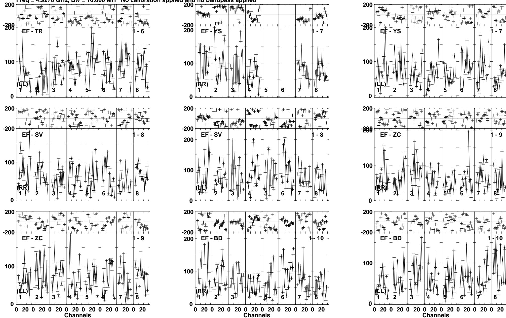
Lower frame: Micro Ampl Jy Top frame: Phas deg Vector averaged cross-power spectrum Baseline: EF (01) - TR (06) Timerange: 00/13:28:51 to 00/13:32:49
