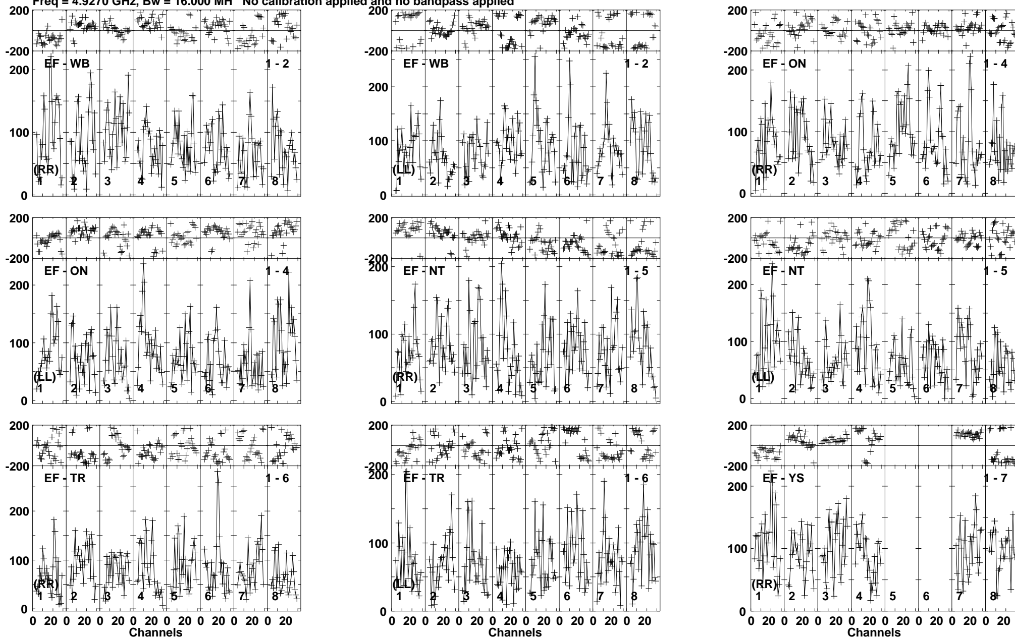
Lower frame: Micro Ampl Jy Top frame: Phas deg Vector averaged cross-power spectrum Baseline: EF (01) - WB (02) Timerange: 00/16:56:15 to 00/17:00:09
