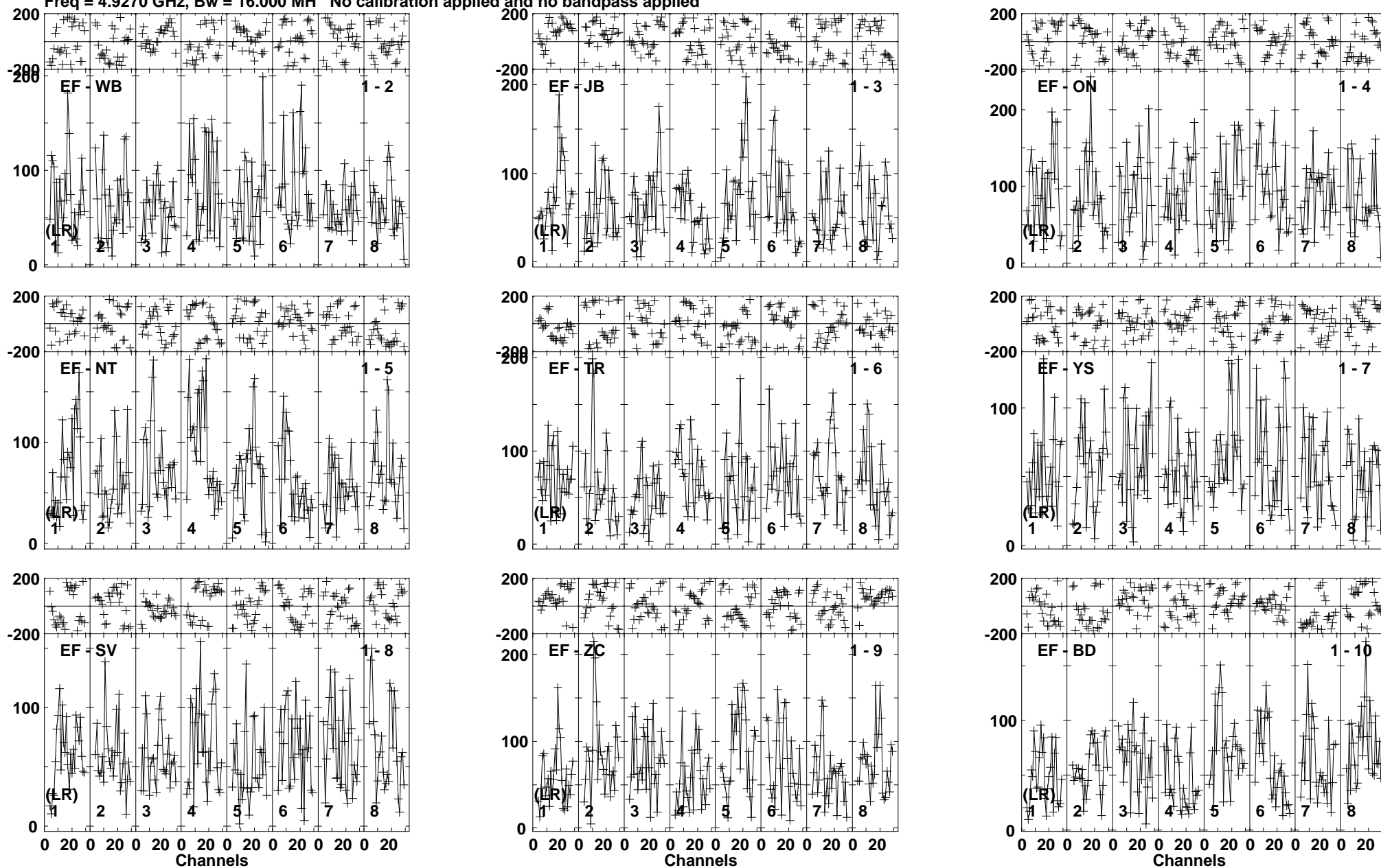
Lower frame: Micro Ampl Jy Top frame: Phas deg Vector averaged cross-power spectrum Baseline: EF (01) - WB (02) Timerange: 00/14:29:31 to 00/14:33:29
