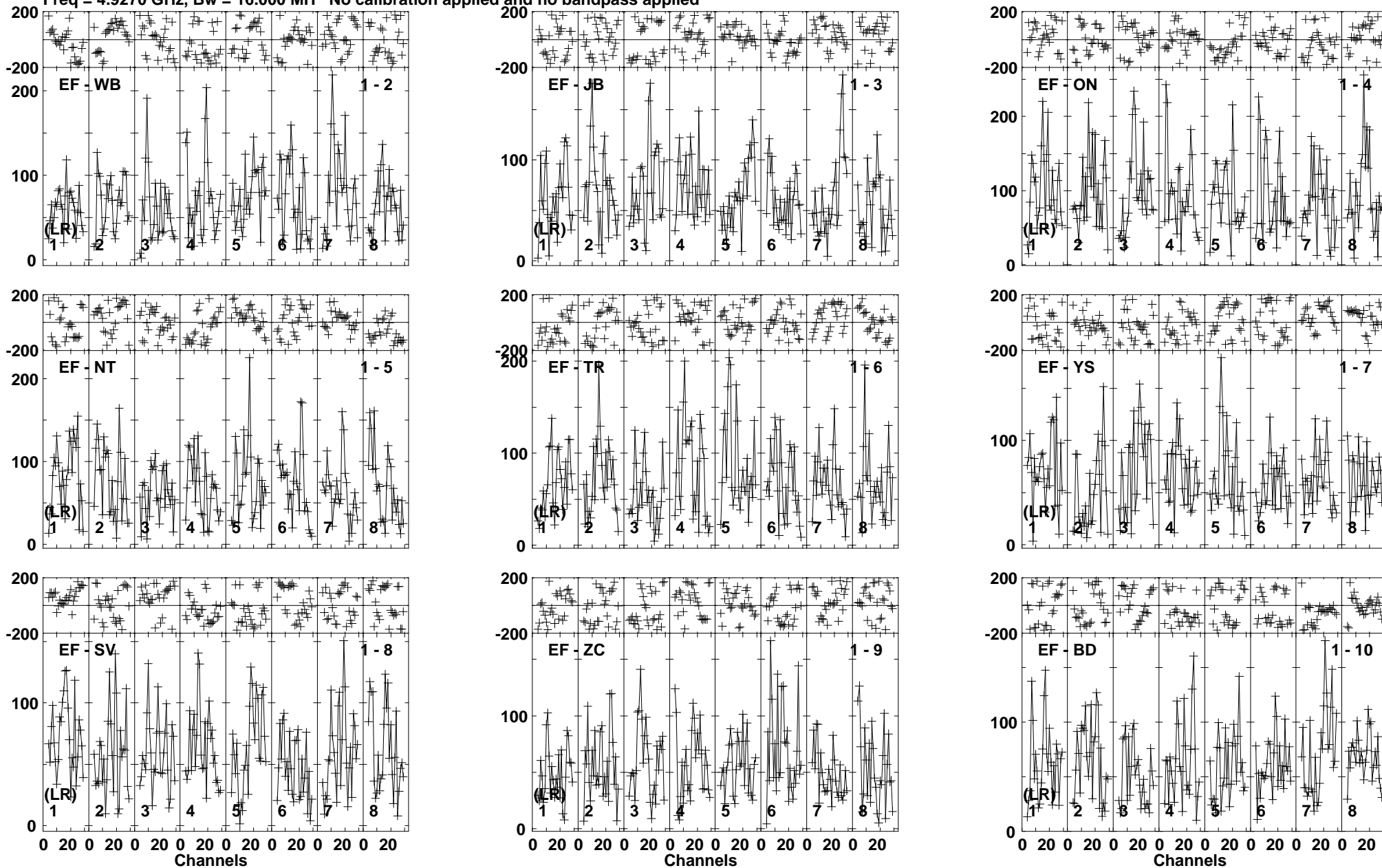
Lower frame: Micro Ampl Jy Top frame: Phas deg Vector averaged cross-power spectrum Baseline: EF (01) - WB (02) Timerange: 00/14:39:41 to 00/14:43:39
