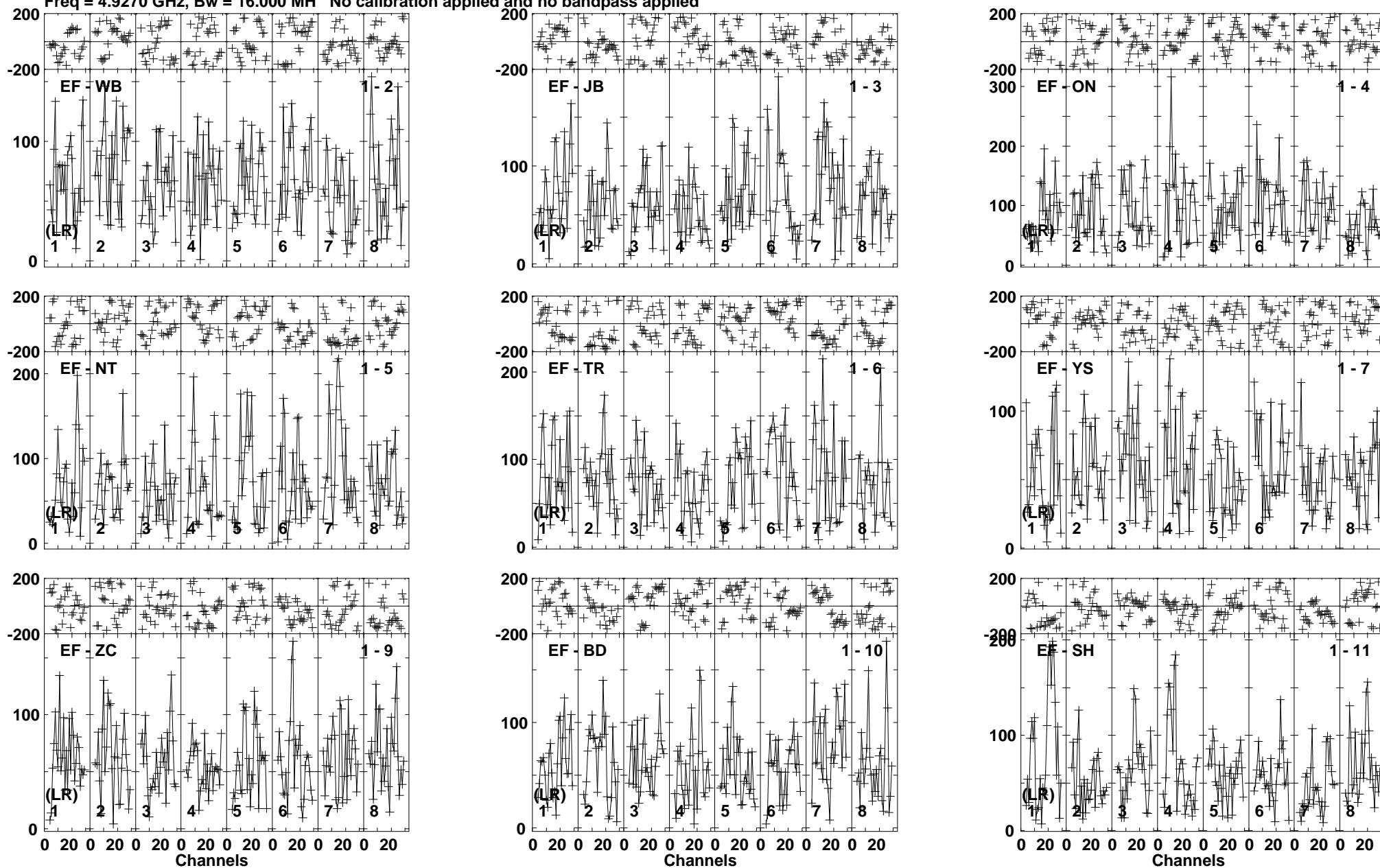
Lower frame: Micro Ampl Jy Top frame: Phas deg Vector averaged cross-power spectrum Baseline: EF (01) - WB (02) Timerange: 00/16:25:55 to 00/16:29:49
