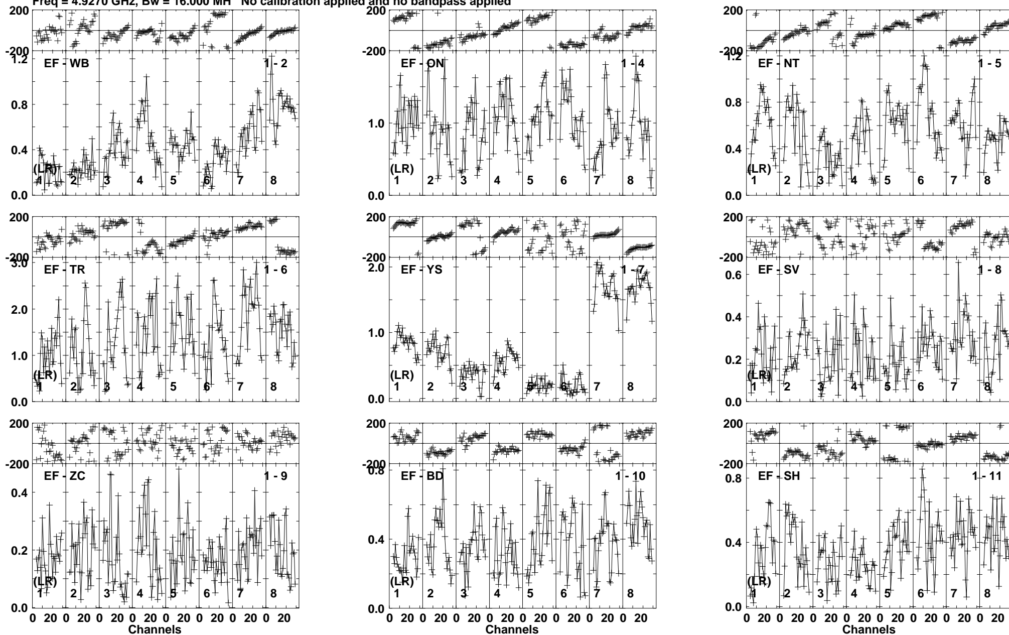
Lower frame: Milli Ampl Jy Top frame: Phas deg Vector averaged cross-power spectrum Baseline: EF (01) - WB (02) Timerange: 00/14:48:45 to 00/14:49:39
