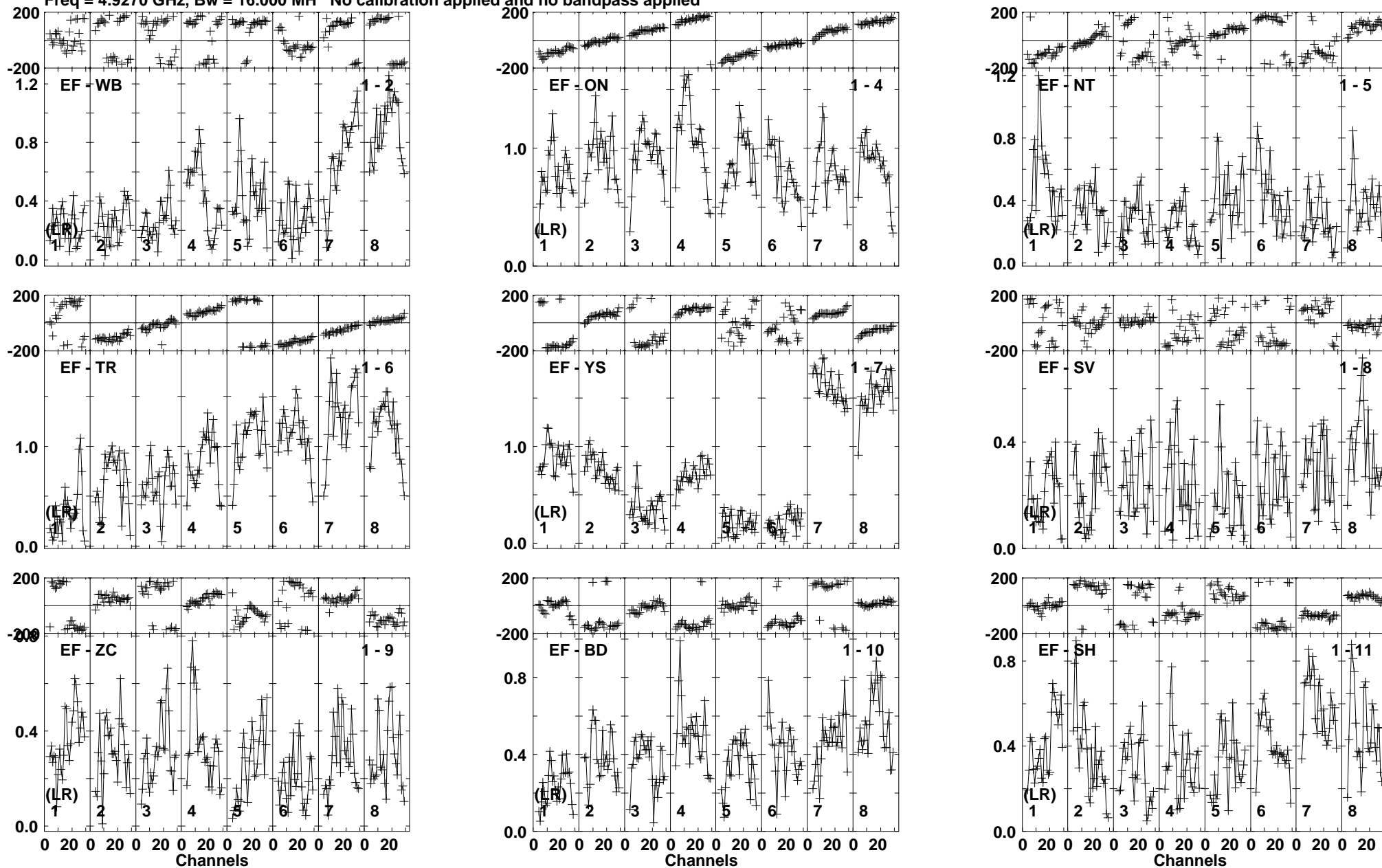
Lower frame: Milli Ampl Jy Top frame: Phas deg Vector averaged cross-power spectrum Baseline: EF (01) - WB (02) Timerange: 00/13:08:13 to 00/13:08:39
