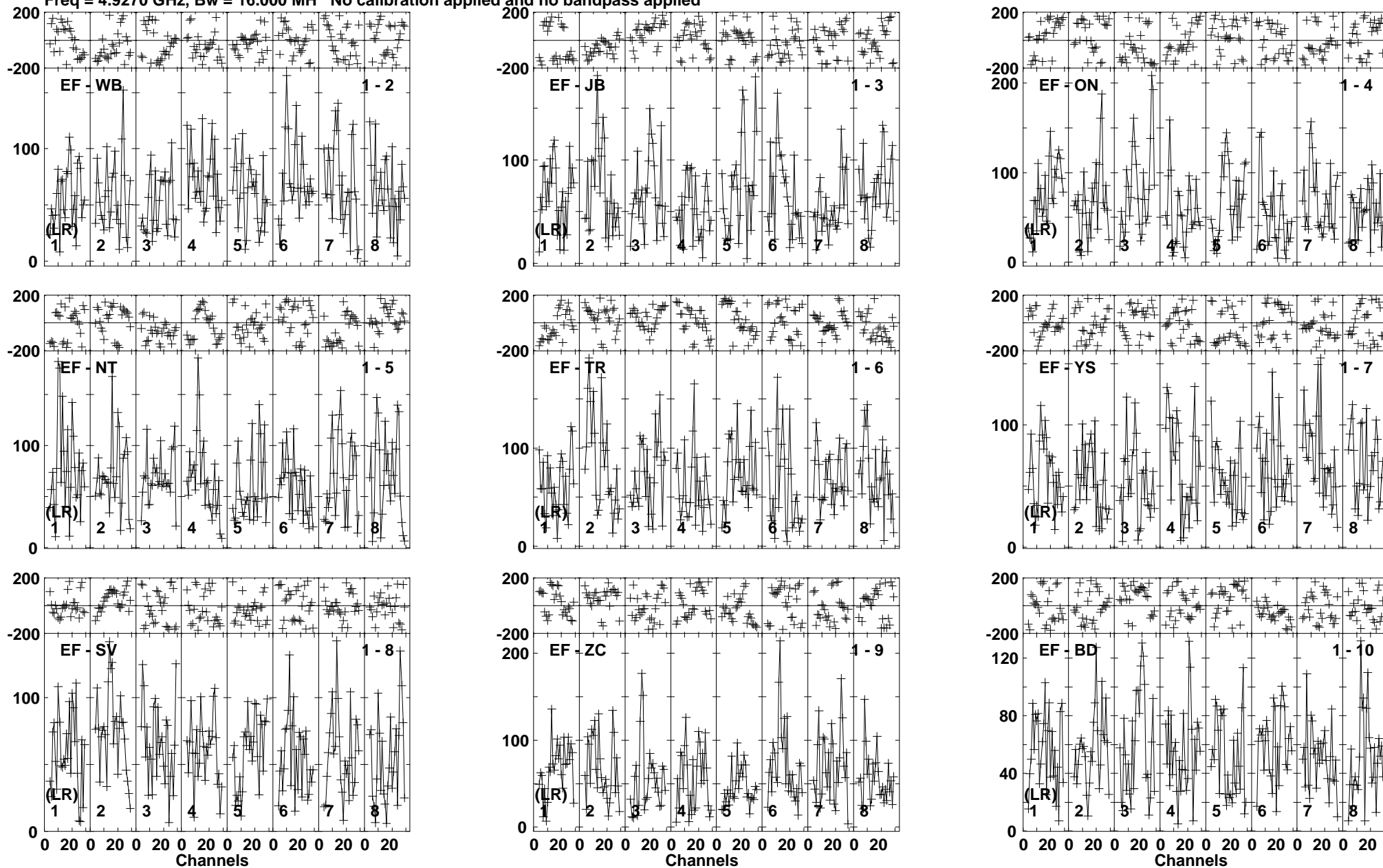
Lower frame: Micro Ampl Jy Top frame: Phas deg Vector averaged cross-power spectrum Baseline: EF (01) - WB (02) Timerange: 00/13:08:41 to 00/13:12:39
