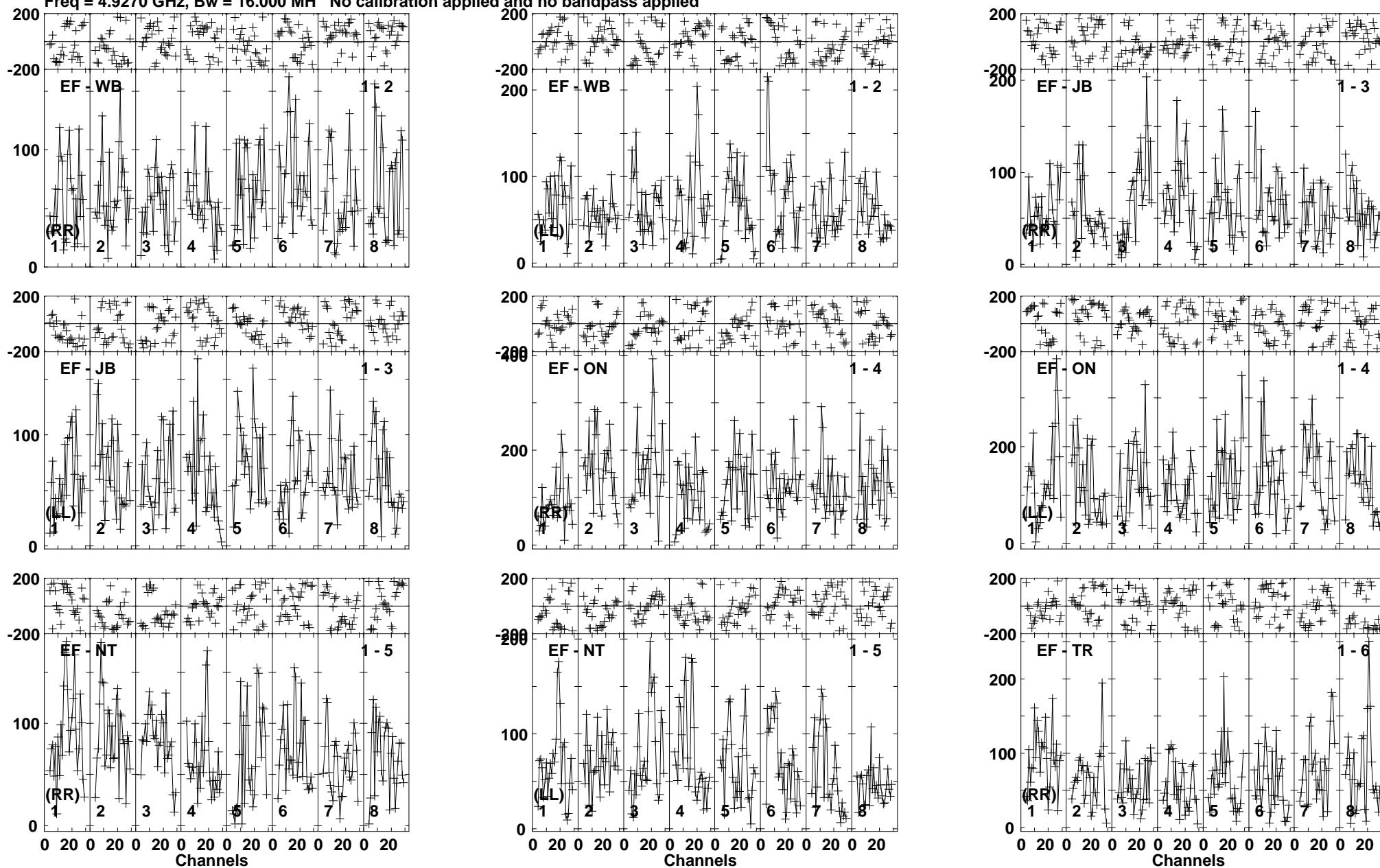
Lower frame: Micro Ampl Jy Top frame: Phas deg Vector averaged cross-power spectrum Baseline: EF (01) - WB (02) Timerange: 00/16:15:45 to 00/16:19:39
