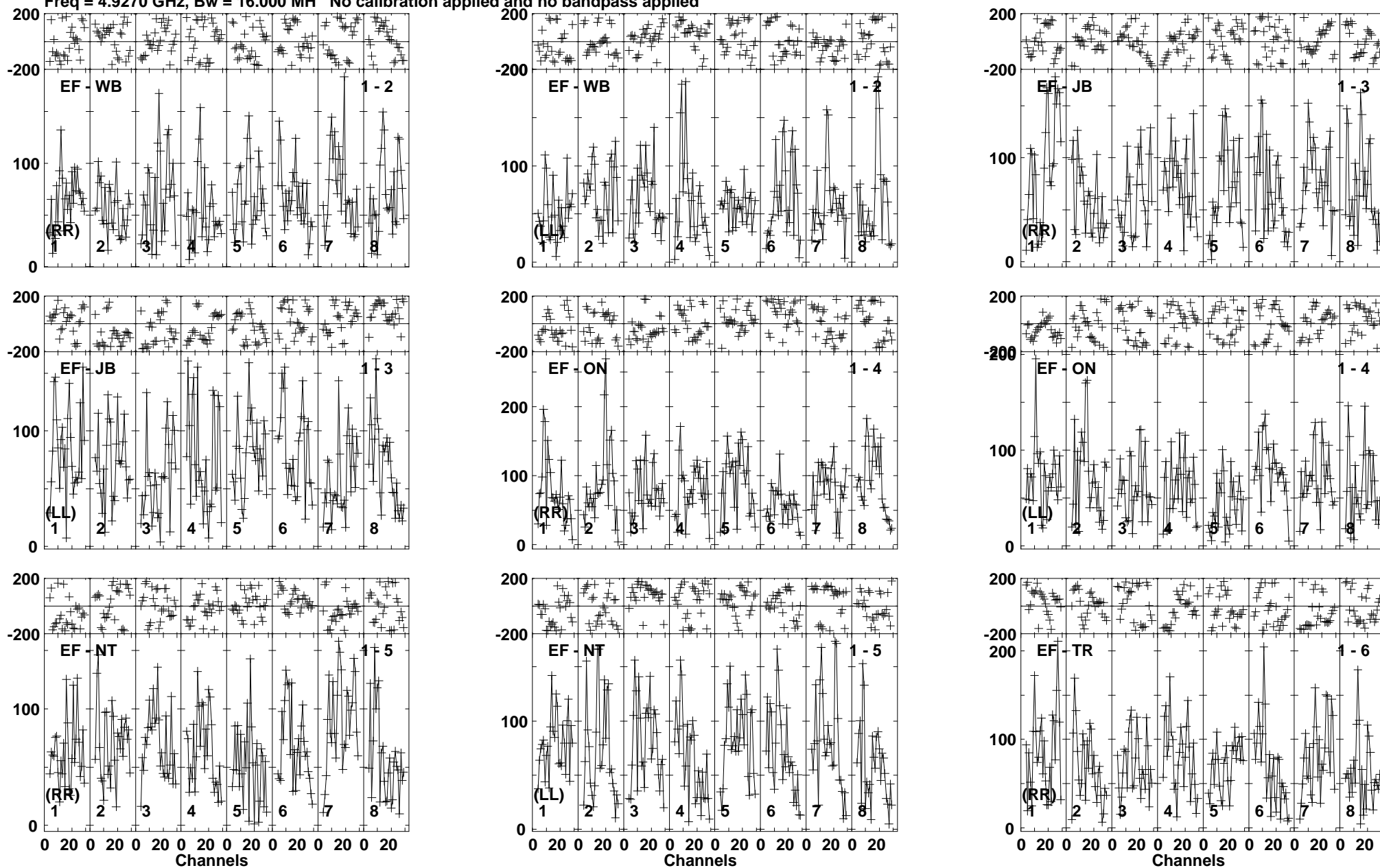
Lower frame: Micro Ampl Jy Top frame: Phas deg Vector averaged cross-power spectrum Baseline: EF (01) - WB (02) Timerange: 00/14:24:35 to 00/14:28:29
