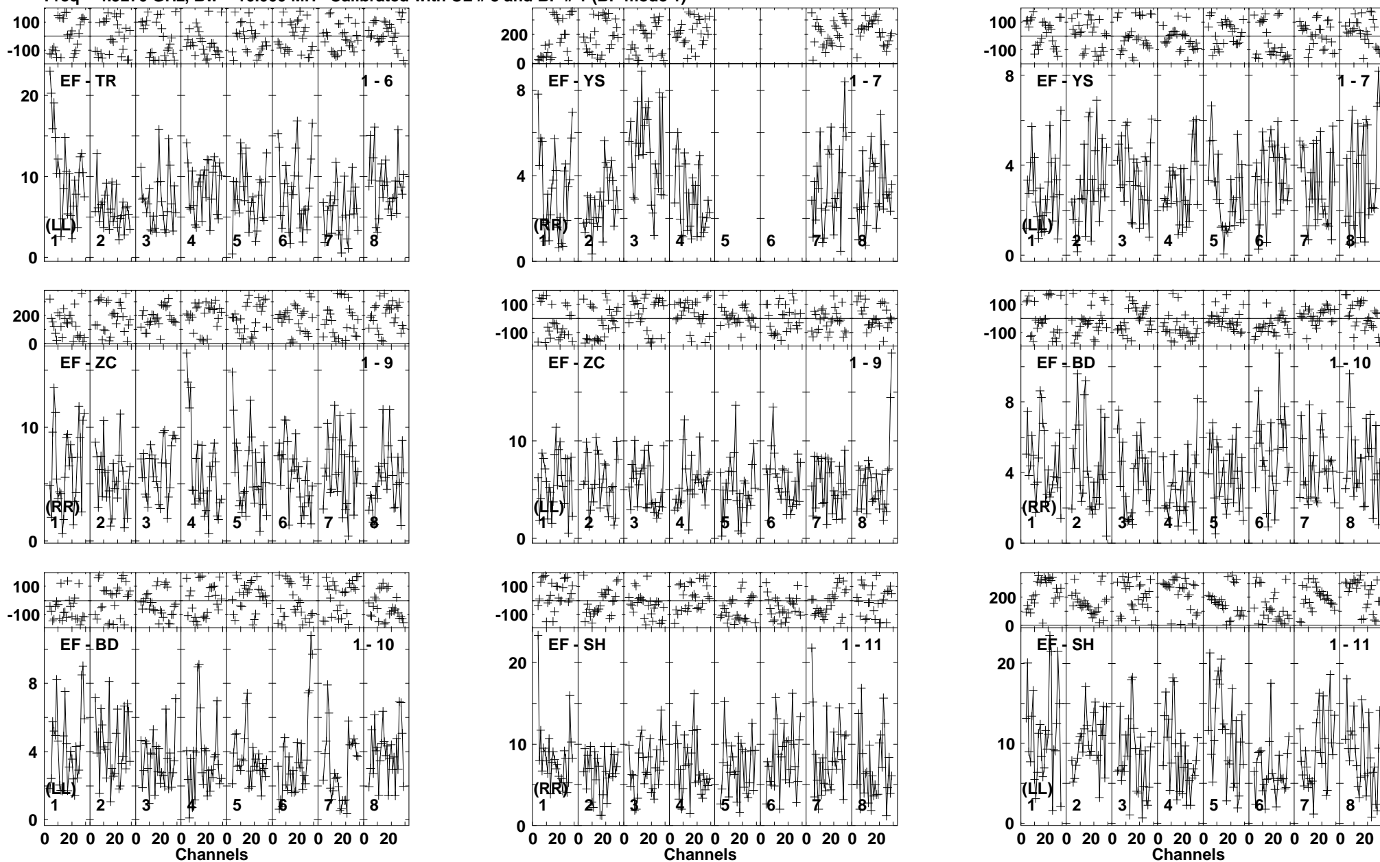
Lower frame: Milli Ampl Jy Top frame: Phas deg Vector averaged cross-power spectrum Baseline: EF (01) - TR (06) Timerange: 00/17:16:25 to 00/17:20:19
