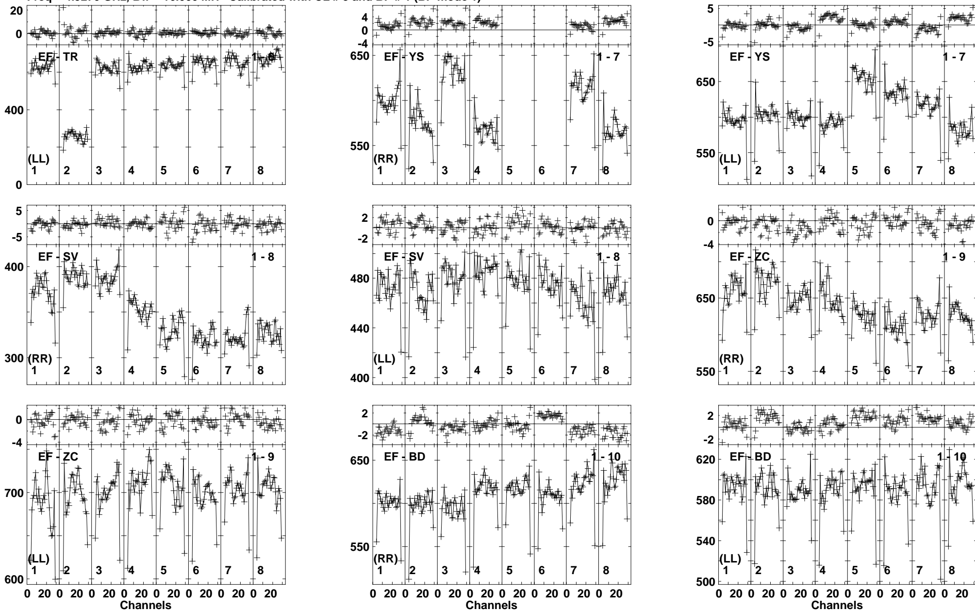
Lower frame: Milli Ampl Jy Top frame: Phas deg Vector averaged cross-power spectrum Baseline: EF (01) - TR (06) Timerange: 00/13:53:41 to 00/13:54:09
