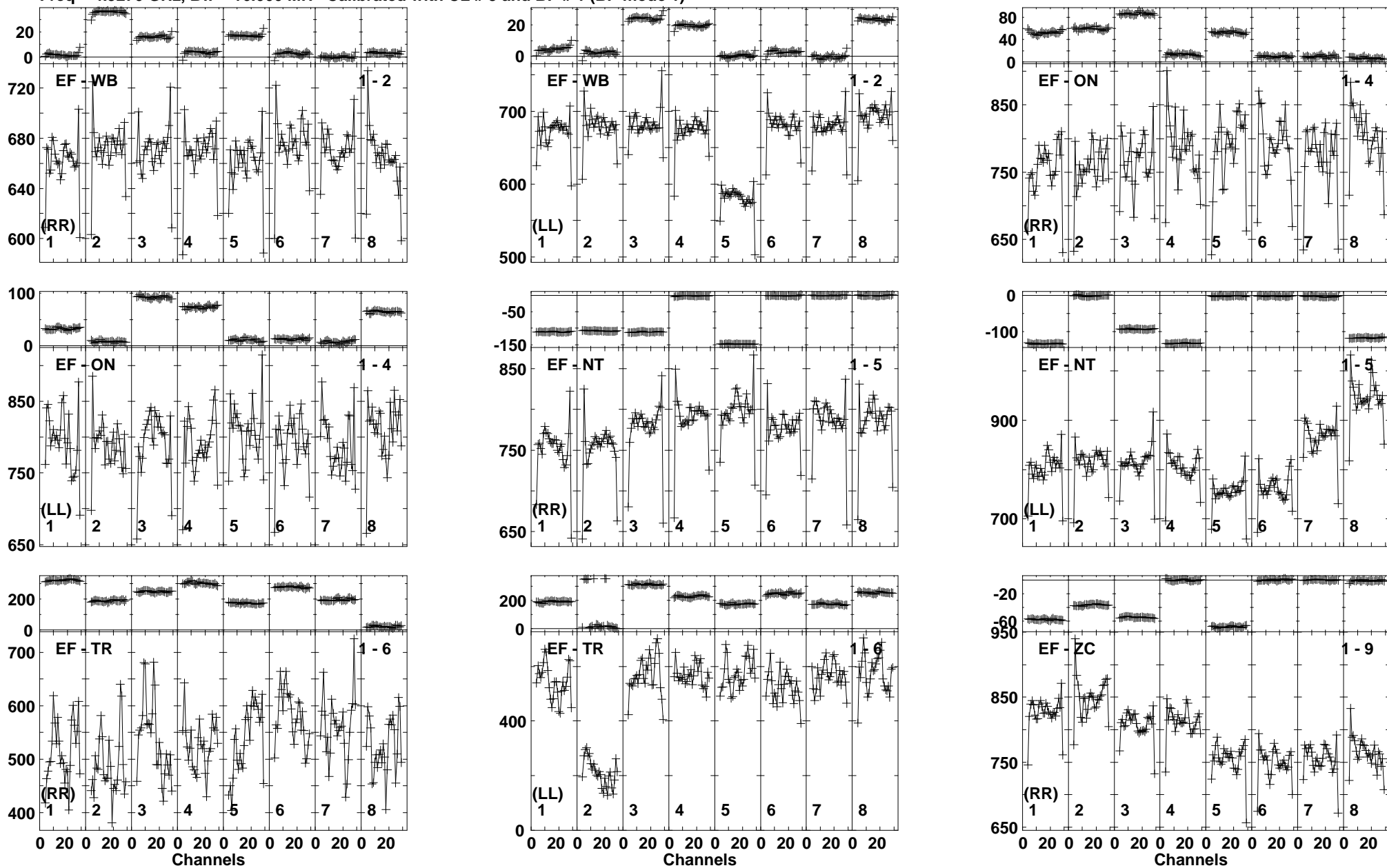
Lower frame: Milli Ampl Jy Top frame: Phas deg Vector averaged cross-power spectrum Baseline: EF (01) - WB (02) Timerange: 00/15:19:05 to 00/15:19:59
