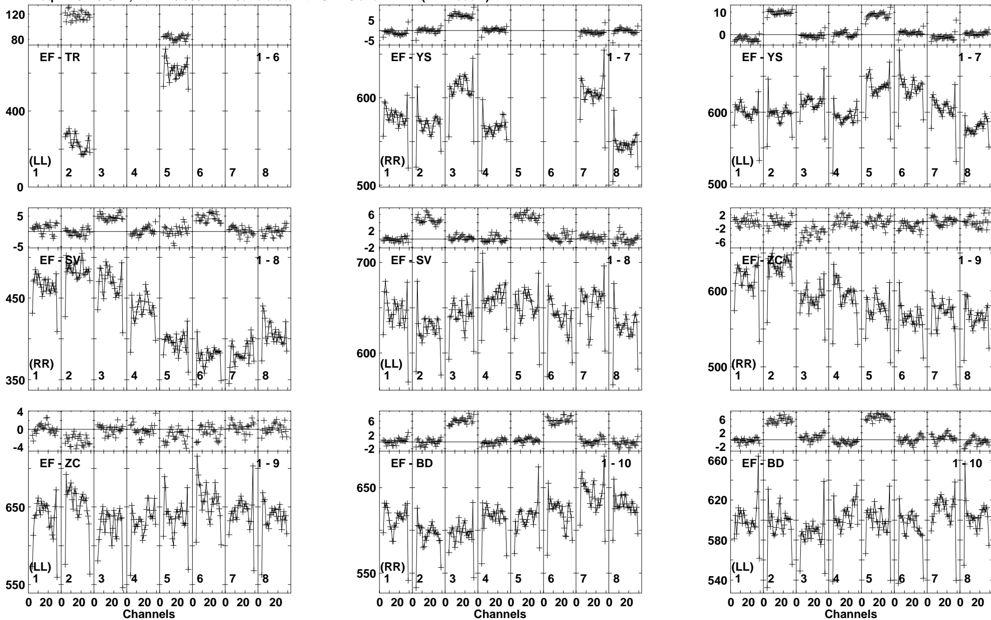
Lower frame: Milli Ampl Jy Top frame: Phas deg Vector averaged cross-power spectrum Baseline: EF (01) - TR (06) Timerange: 00/14:03:15 to 00/14:04:09
