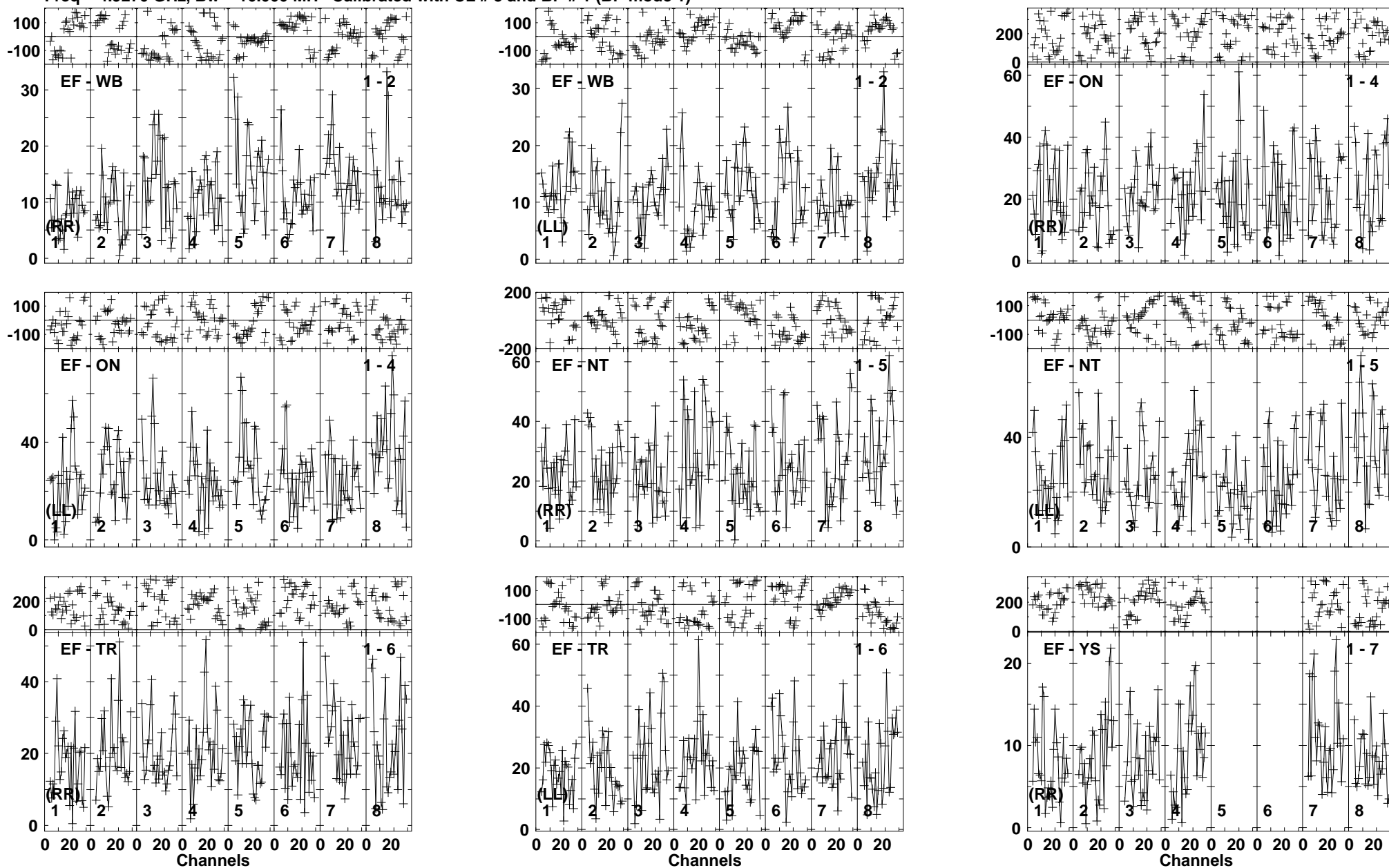
Lower frame: Milli Ampl Jy Top frame: Phas deg Vector averaged cross-power spectrum Baseline: EF (01) - WB (02) Timerange: 00:12:43:35 to 00:12:47:19
