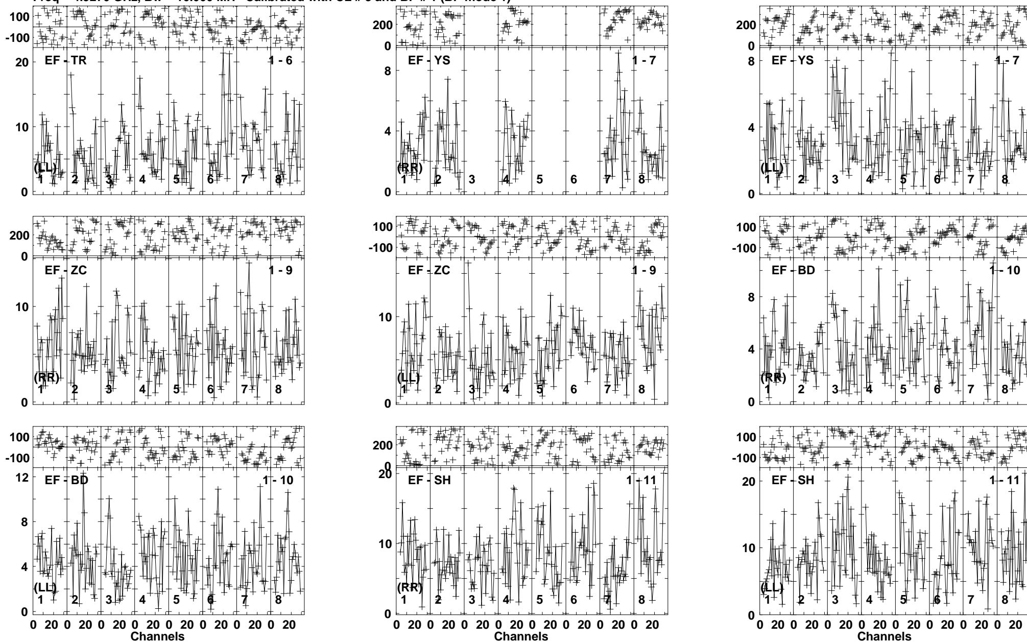
Lower frame: Milli Ampl Jy Top frame: Phas deg Vector averaged cross-power spectrum Baseline: EF (01) - TR (06) Timerange: 00/17:06:15 to 00/17:10:09
