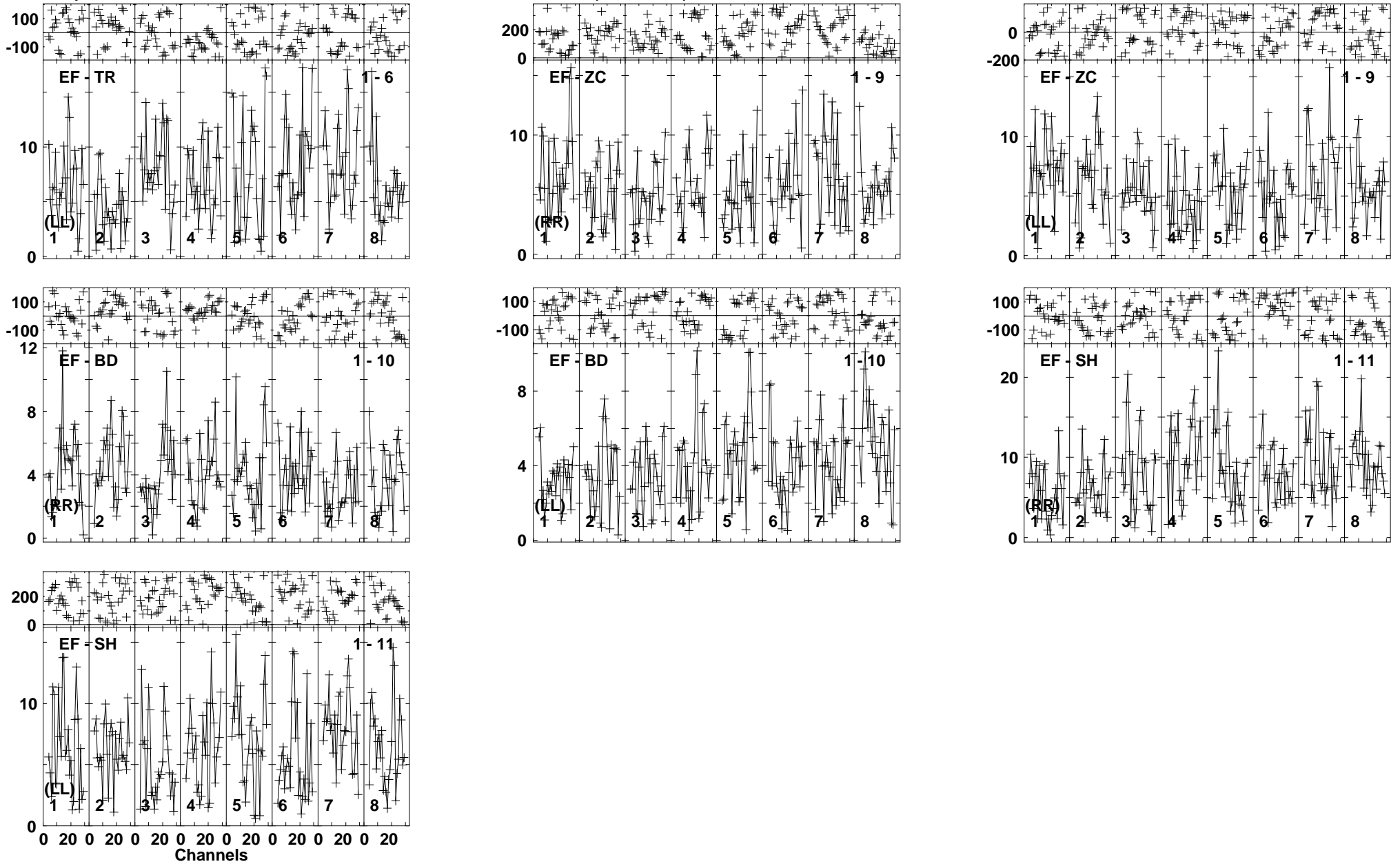
Lower frame: Milli Ampl Jy Top frame: Phas deg Vector averaged cross-power spectrum Baseline: EF (01) - TR (06) Timerange: 00/15:35:15 to 00/15:39:09
