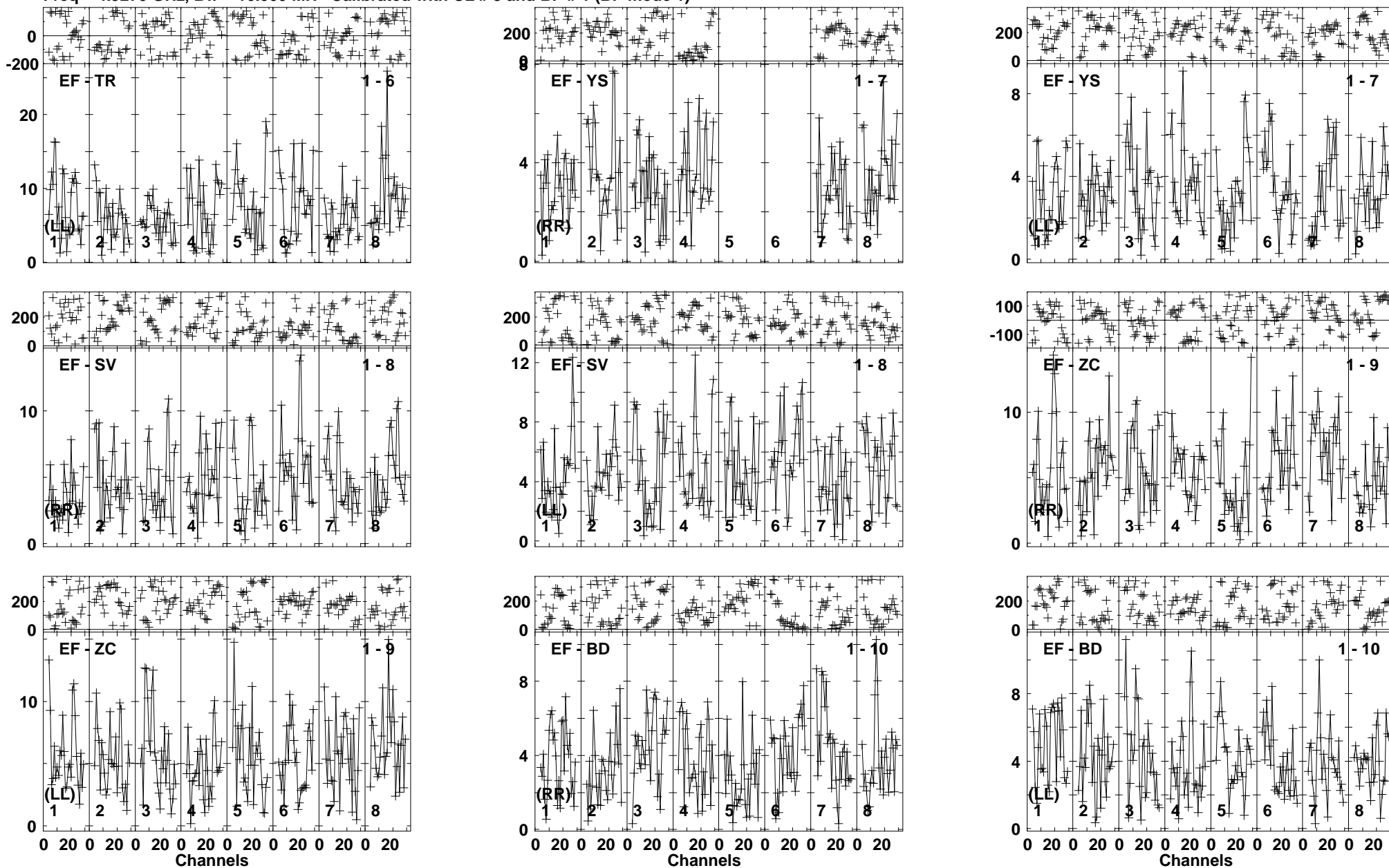
Lower frame: Milli Ampl Jy Top frame: Phas deg Vector averaged cross-power spectrum Baseline: EF (01) - TR (06) Timerange: 00/14:34:35 to 00/14:38:29
