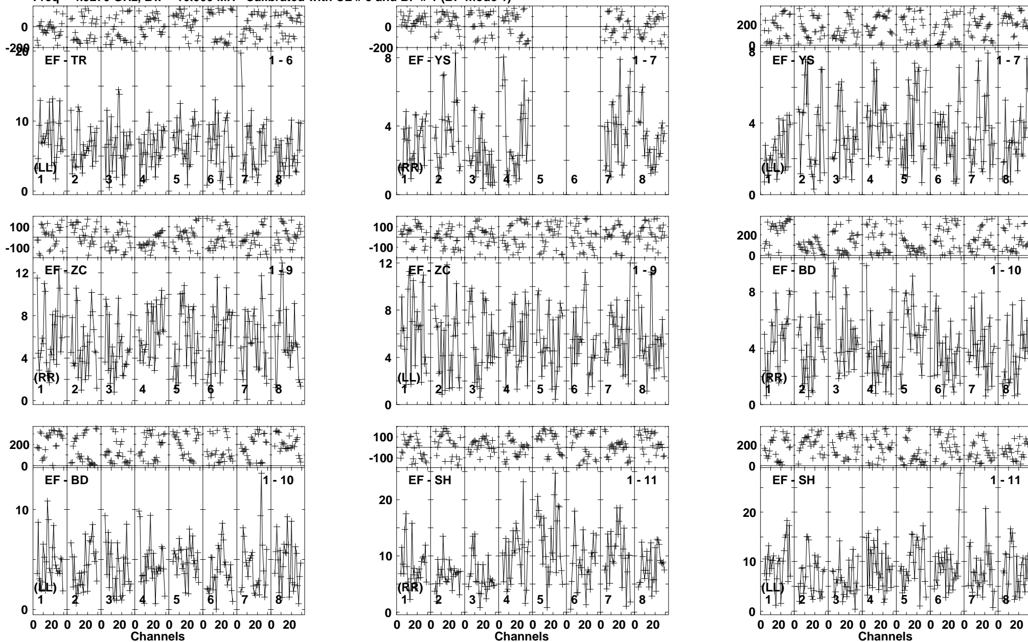
Lower frame: Milli Ampl Jy Top frame: Phas deg Vector averaged cross-power spectrum Baseline: EF (01) - TR (06) Timerange: 00/16:25:55 to 00/16:29:49
