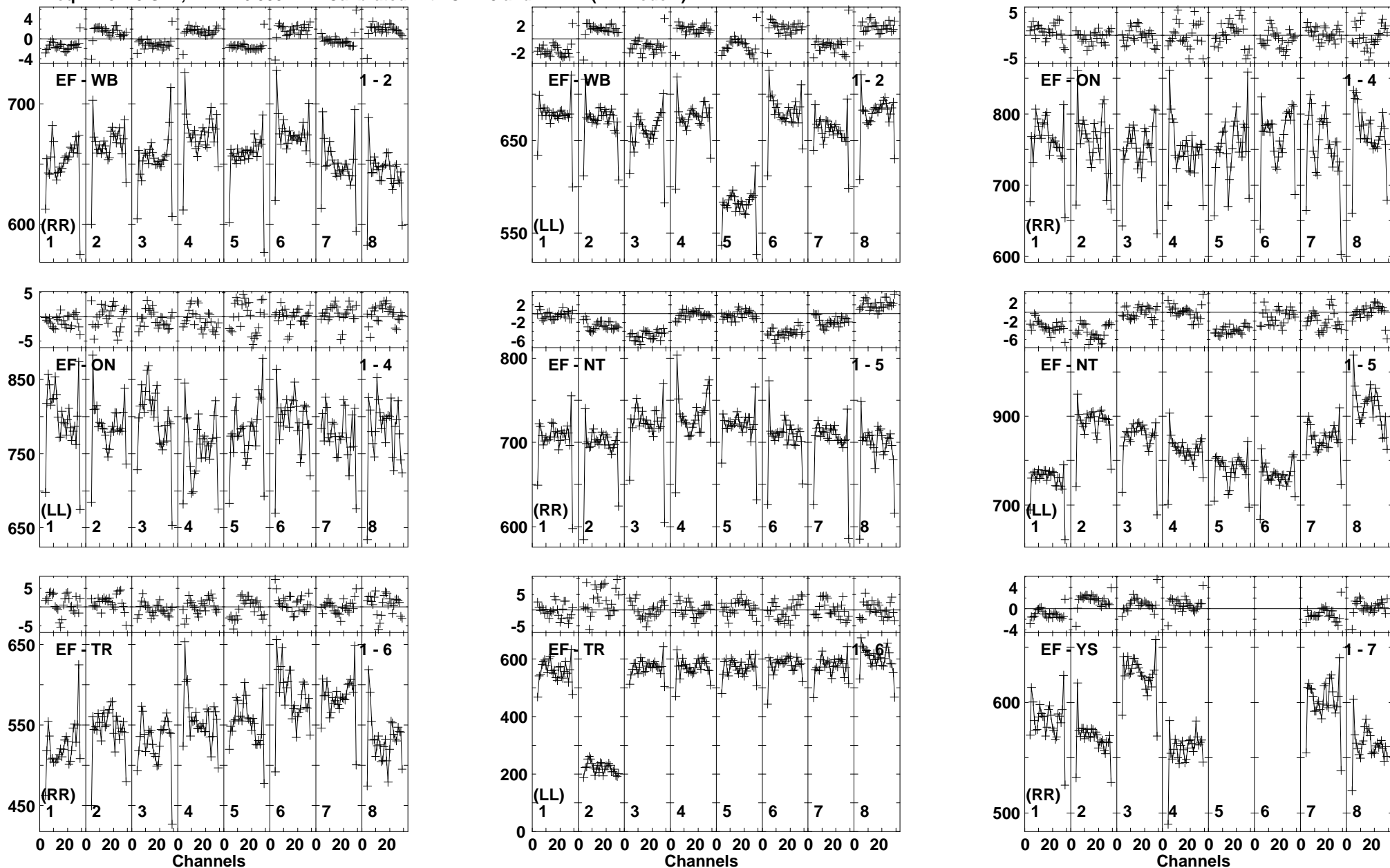
Lower frame: Milli Ampl Jy Top frame: Phas deg Vector averaged cross-power spectrum Baseline: EF (01) - WB (02) Timerange: 00/14:39:13 to 00/14:39:39
