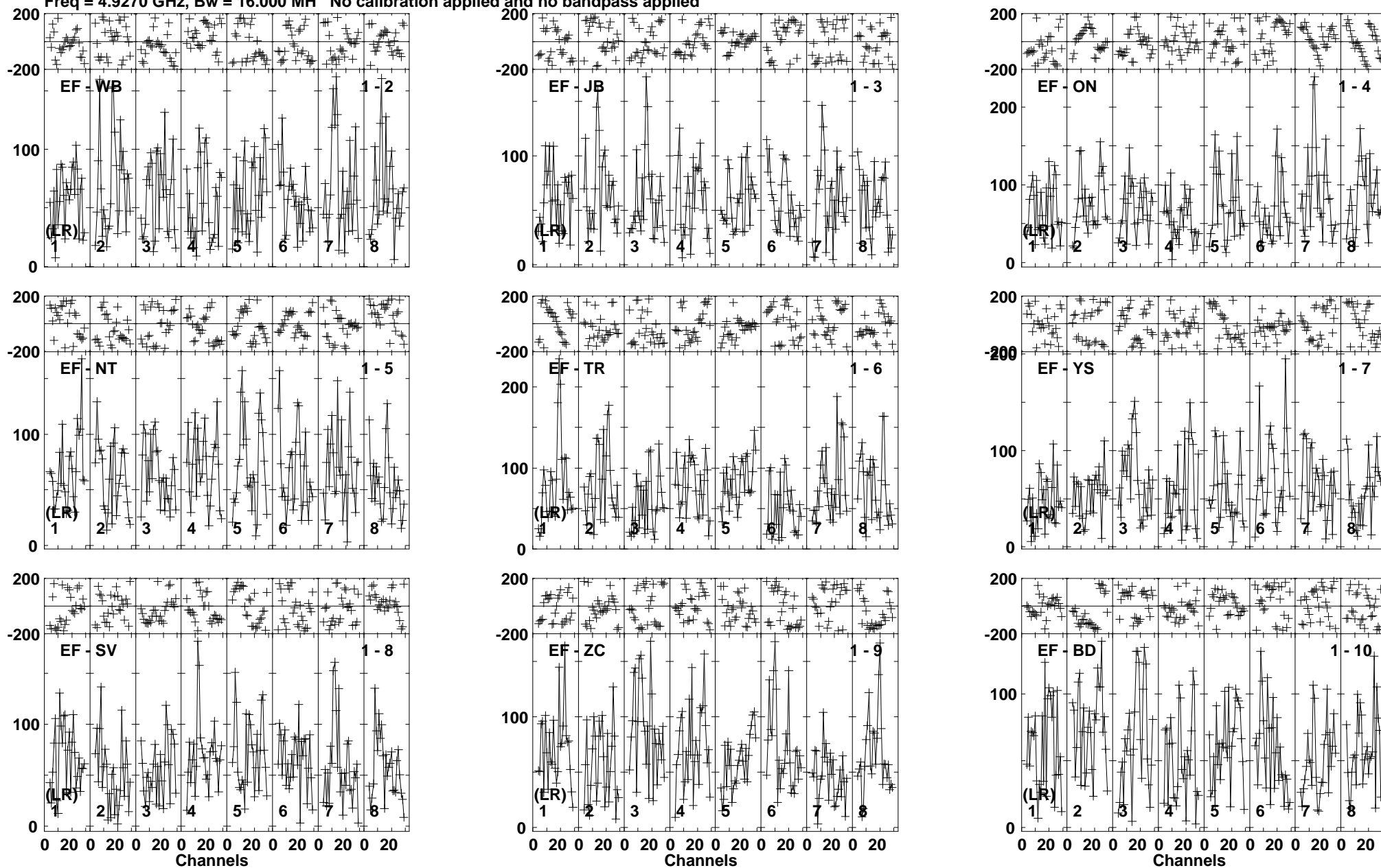
Lower frame: Micro Ampl Jy Top frame: Phas deg Vector averaged cross-power spectrum Baseline: EF (01) - WB (02) Timerange: 00/12:58:31 to 00/13:02:29
