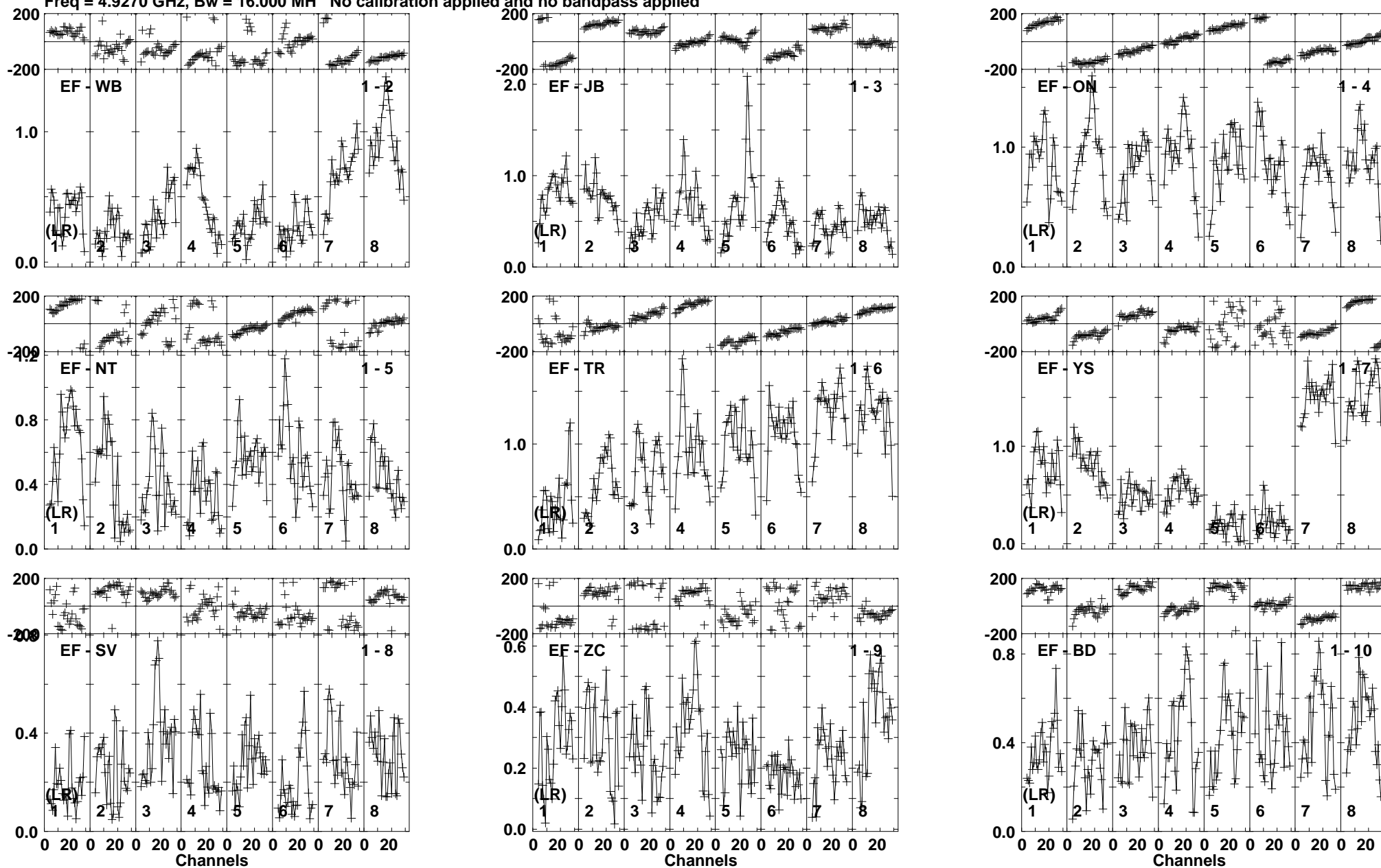
Lower frame: Milli Ampl Jy Top frame: Phas deg Vector averaged cross-power spectrum Baseline: EF (01) - WB (02) Timerange: 00/13:23:21 to 00/13:23:49
