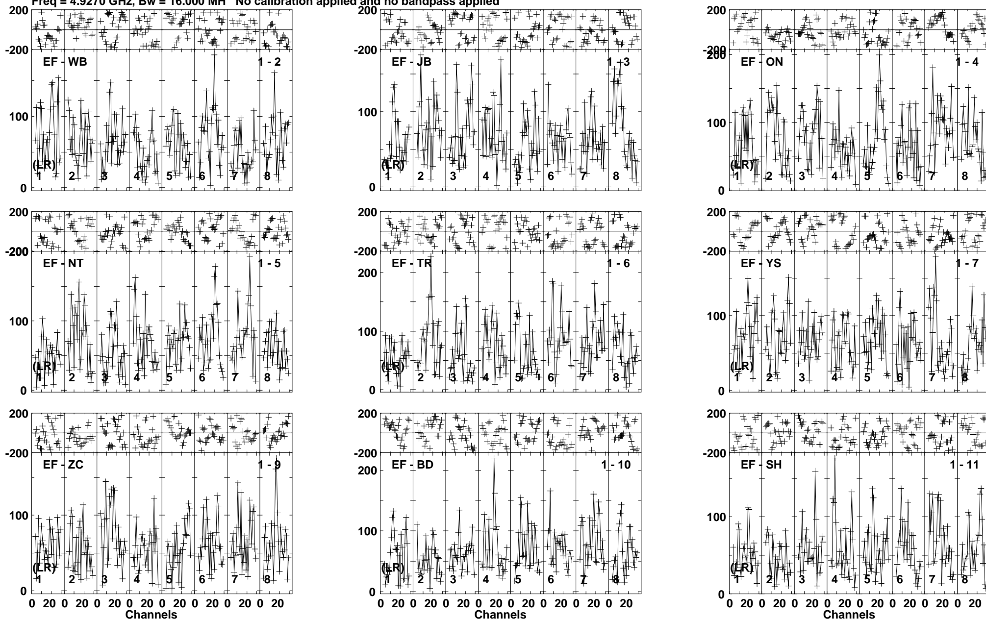
Lower frame: Micro Ampl Jy Top frame: Phas deg Vector averaged cross-power spectrum Baseline: EF (01) - WB (02) Timerange: 00/17:06:15 to 00/17:10:09
