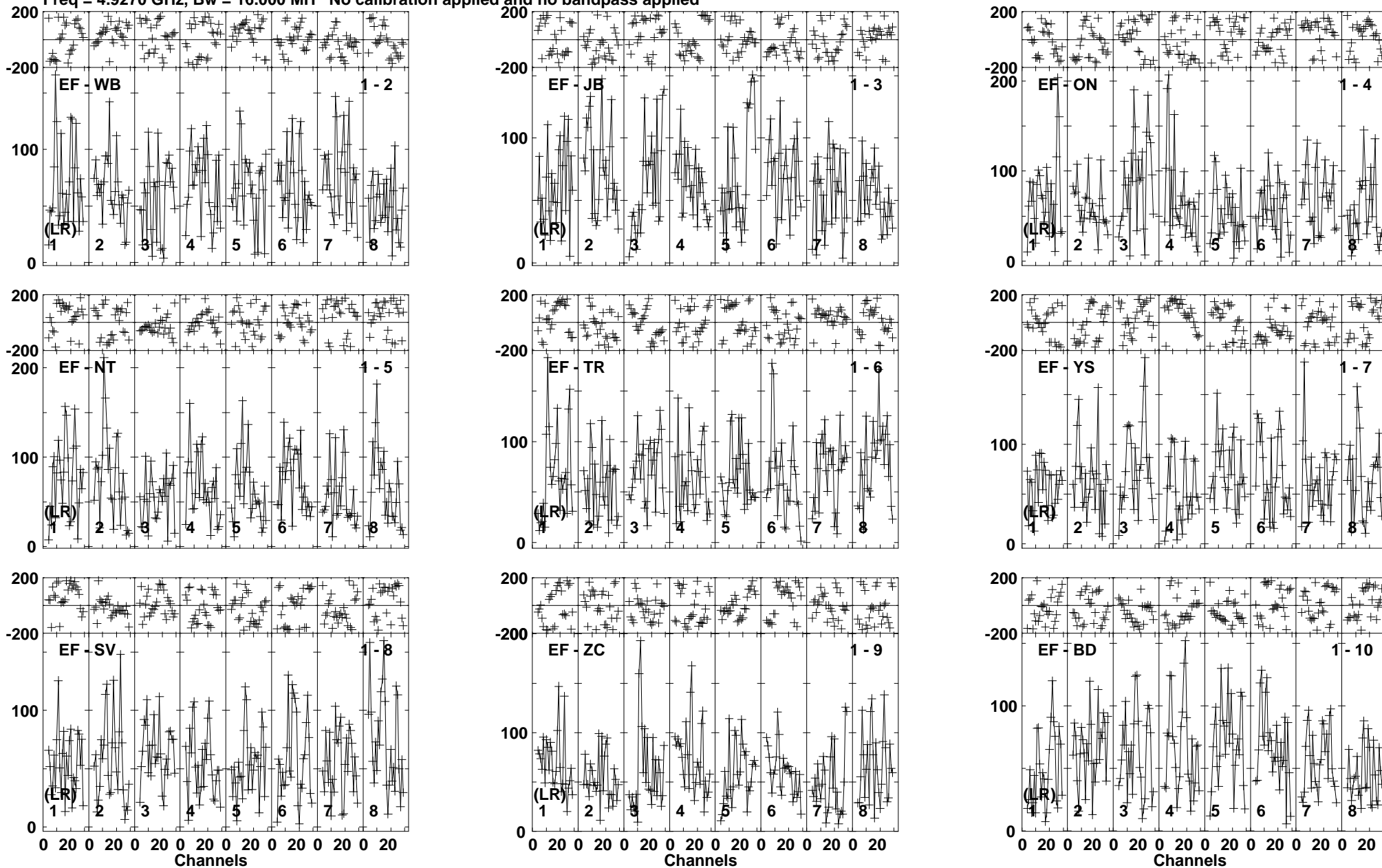
Lower frame: Micro Ampl Jy Top frame: Phas deg Vector averaged cross-power spectrum Baseline: EF (01) - WB (02) Timerange: 00/18:06:55 to 00/18:10:49
