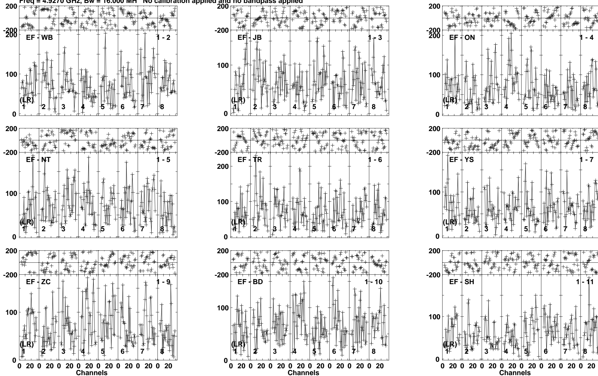
Lower frame: Micro Ampl Jy Top frame: Phas deg Vector averaged cross-power spectrum Baseline: EF (01) - WB (02) Timerange: 00/17:21:21 to 00/17:25:19
