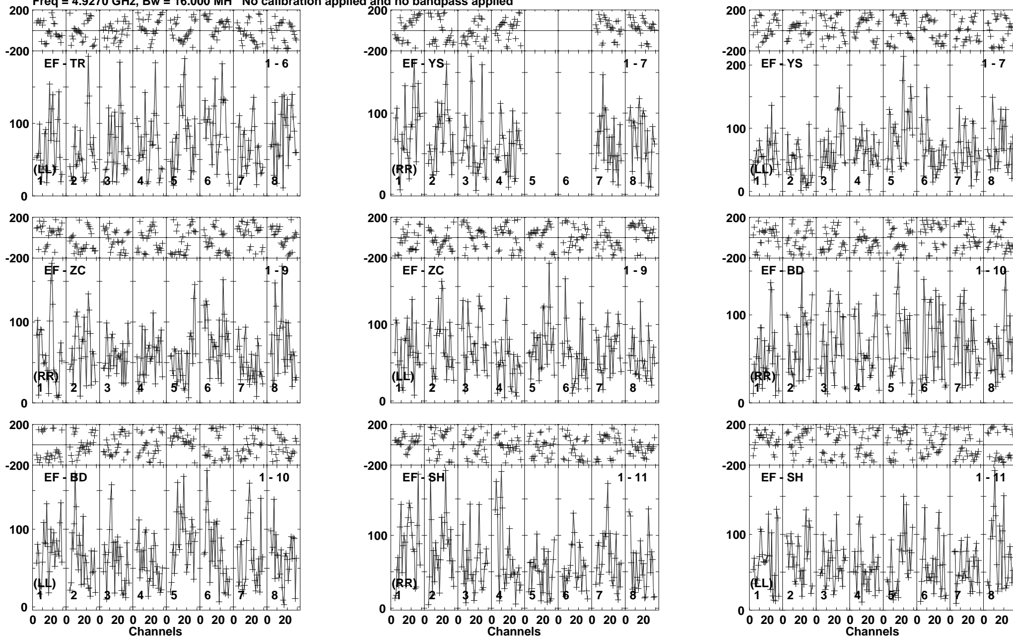
Lower frame: Micro Ampl Jy Top frame: Phas deg Vector averaged cross-power spectrum Baseline: EF (01) - TR (06) Timerange: 00/17:31:31 to 00/17:35:29
