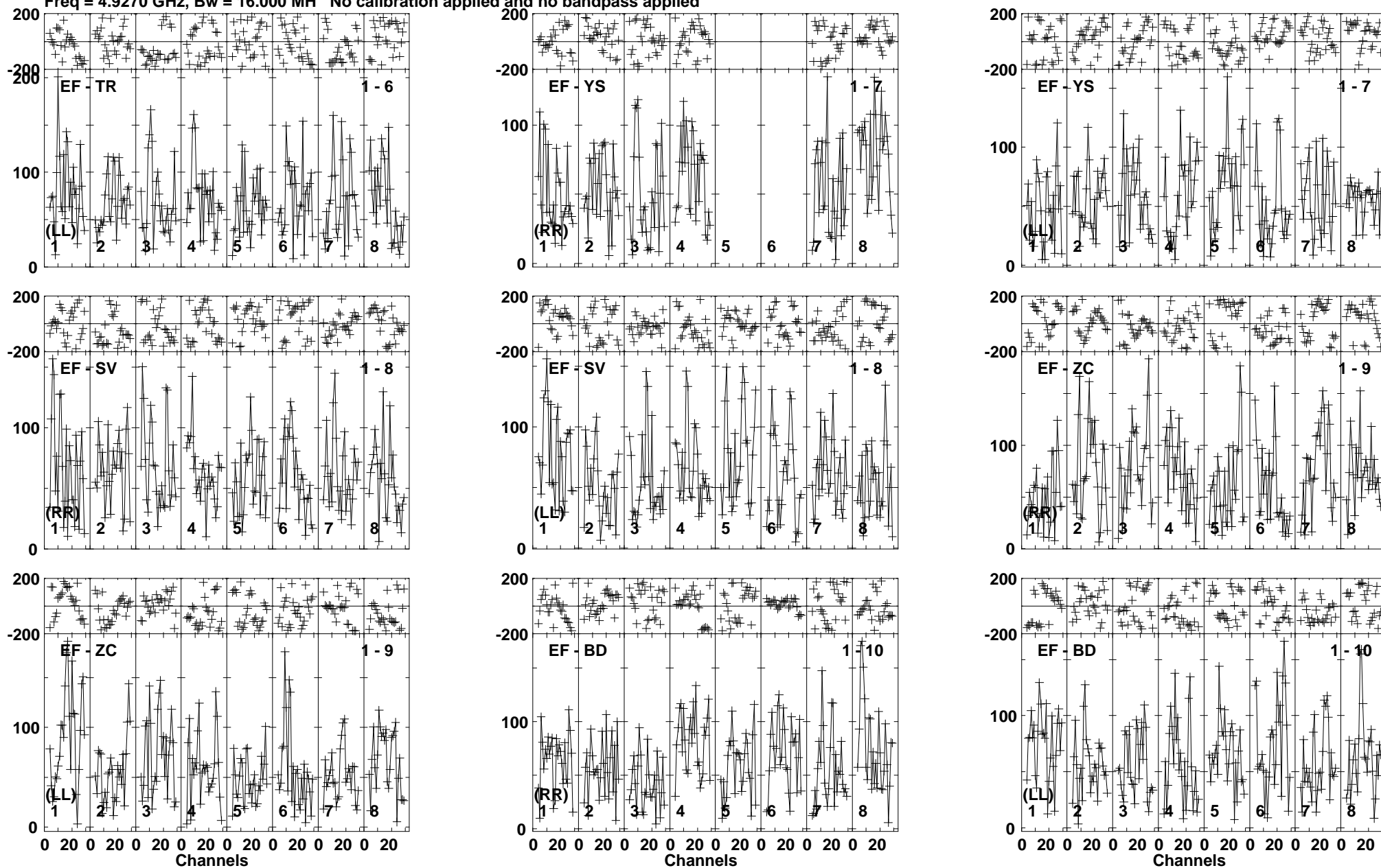
Lower frame: Micro Ampl Jy Top frame: Phas deg Vector averaged cross-power spectrum Baseline: EF (01) - TR (06) Timerange: 00/14:19:21 to 00/14:23:19
