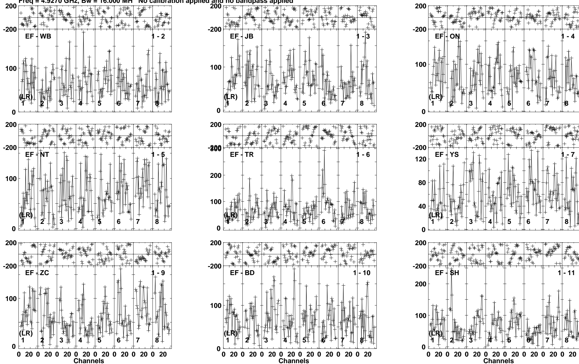
Lower frame: Micro Ampl Jy Top frame: Phas deg Vector averaged cross-power spectrum Baseline: EF (01) - WB (02) Timerange: 00/16:35:55 to 00/16:39:49
