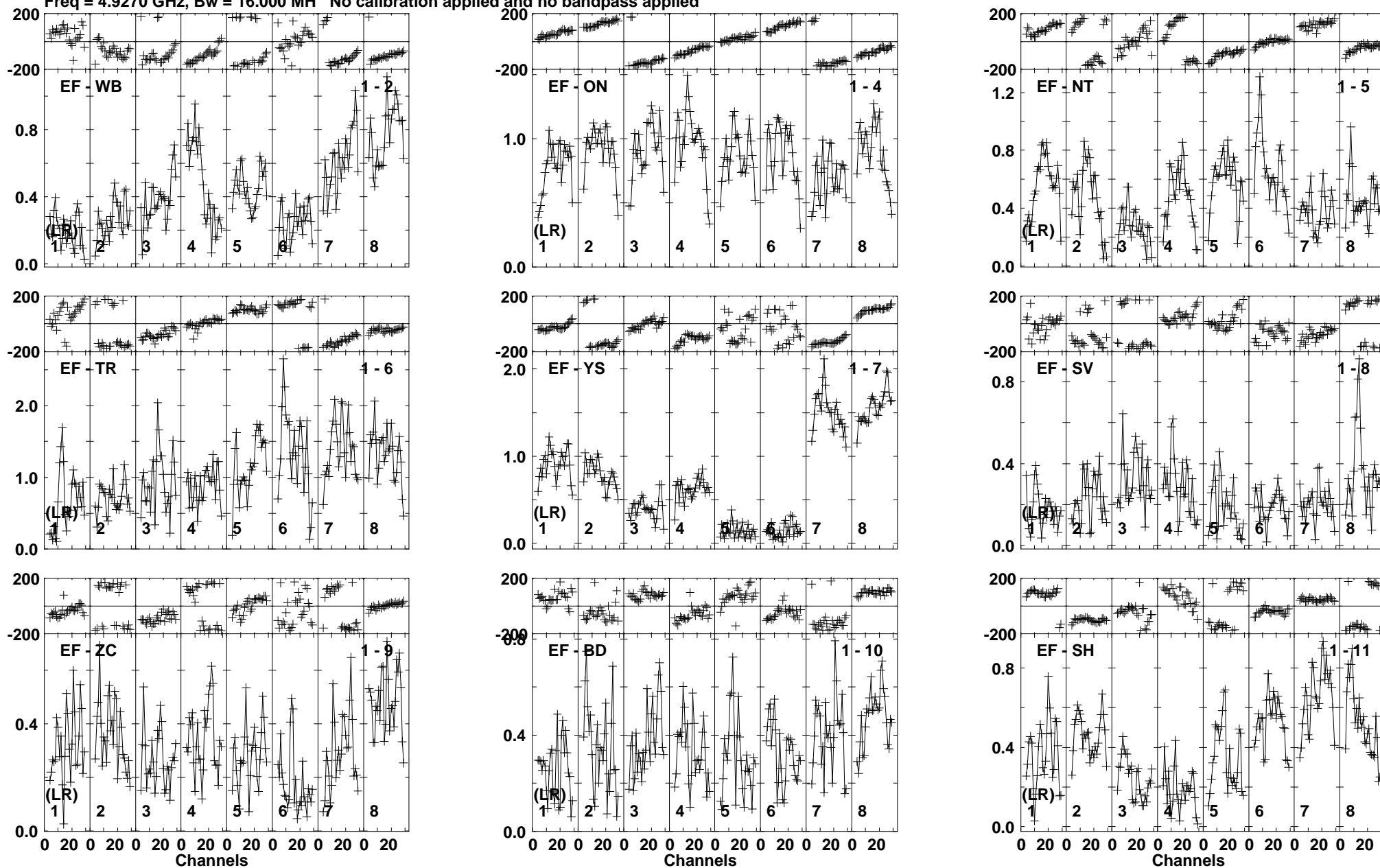
Lower frame: Milli Ampl Jy Top frame: Phas deg Vector averaged cross-power spectrum Baseline: EF (01) - WB (02) Timerange: 00/13:17:45 to 00/13:18:39
