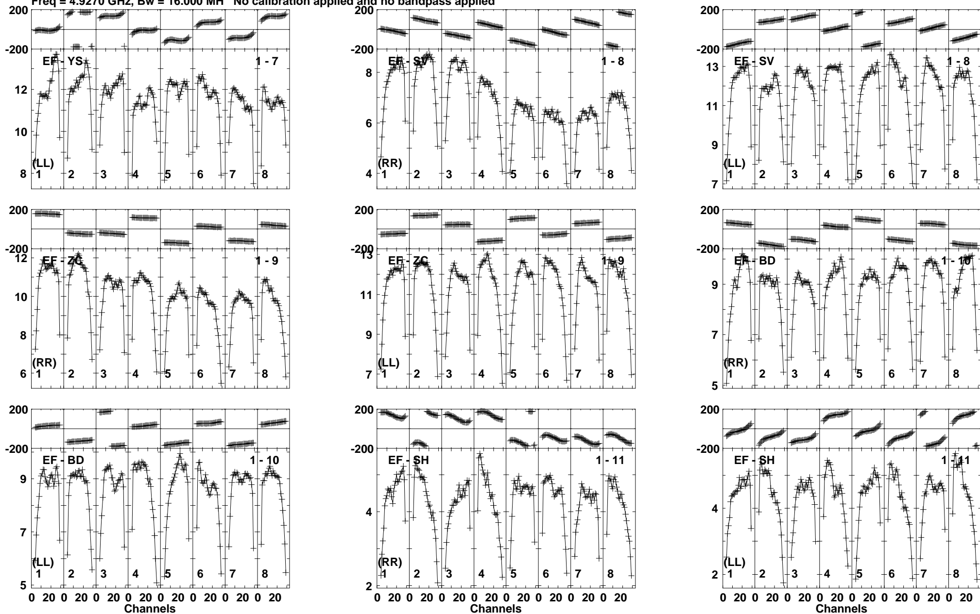
Lower frame: Milli Ampl Jy Top frame: Phas deg Vector averaged cross-power spectrum Baseline: EF (01) - YS (07) Timerange: 00/13:08:13 to 00/13:08:39
