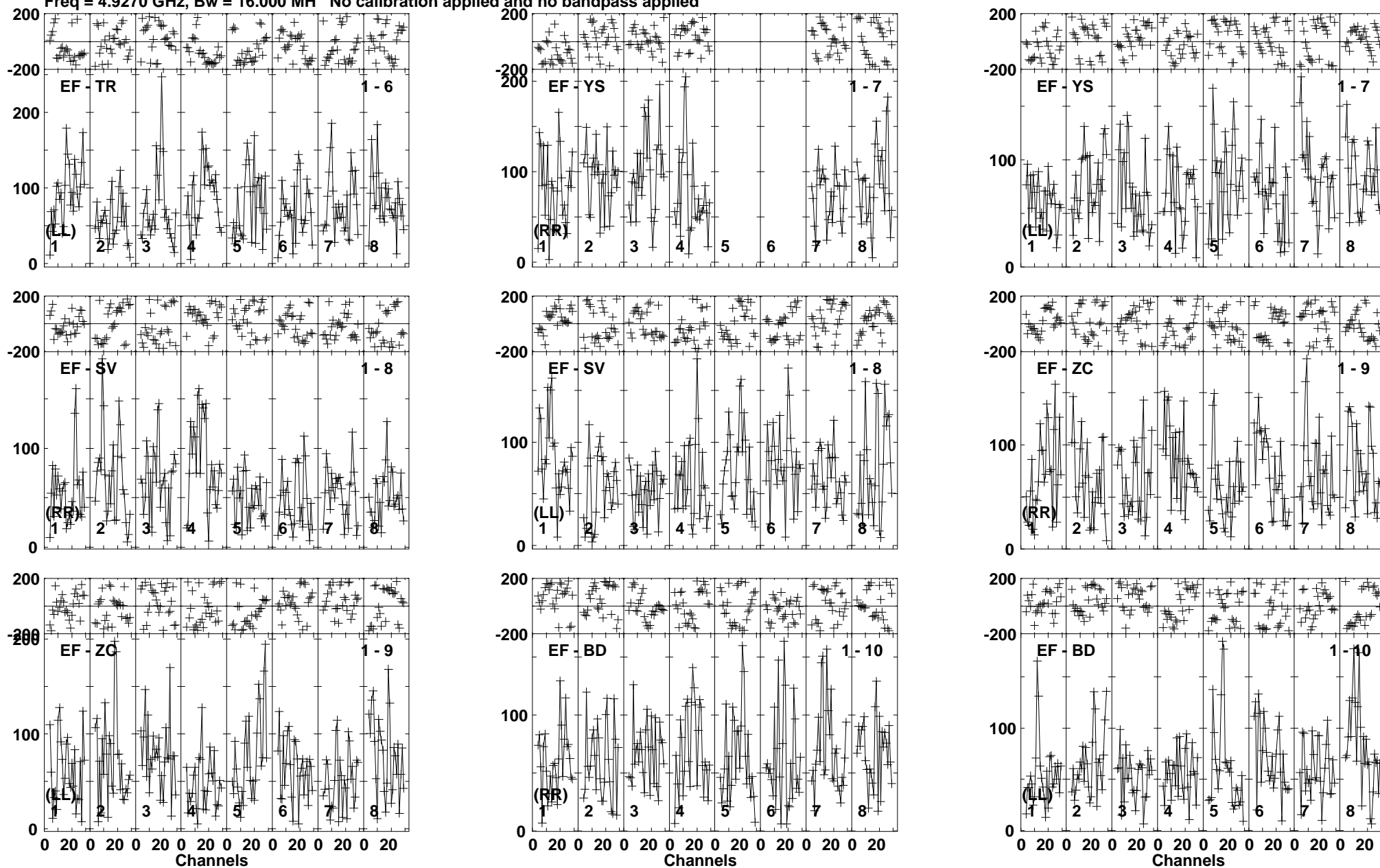
Lower frame: Micro Ampl Jy Top frame: Phas deg Vector averaged cross-power spectrum Baseline: EF (01) - TR (06) Timerange: 00/14:14:25 to 00/14:18:19
