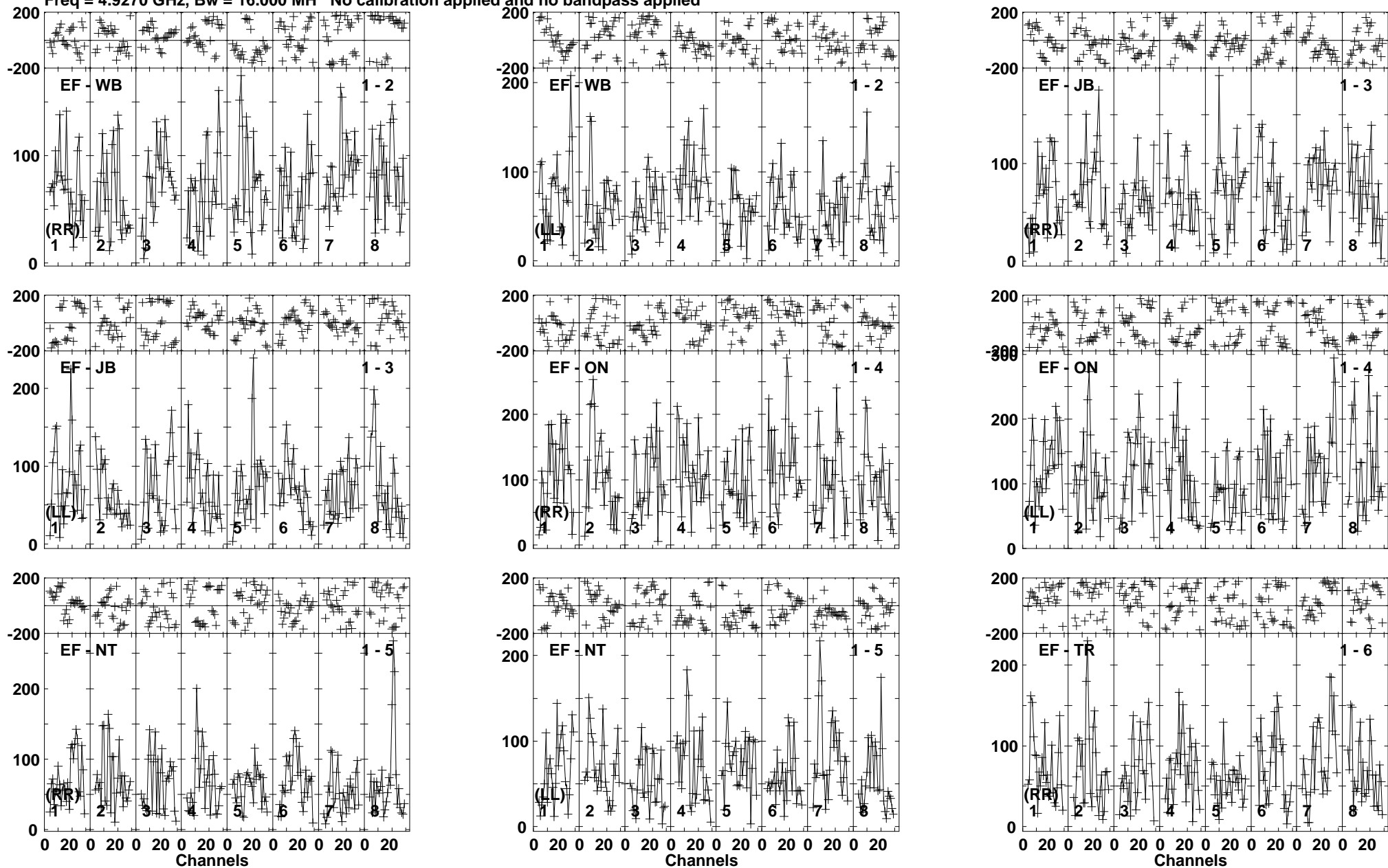
Lower frame: Micro Ampl Jy Top frame: Phas deg Vector averaged cross-power spectrum Baseline: EF (01) - WB (02) Timerange: 00/14:44:45 to 00/14:48:39
