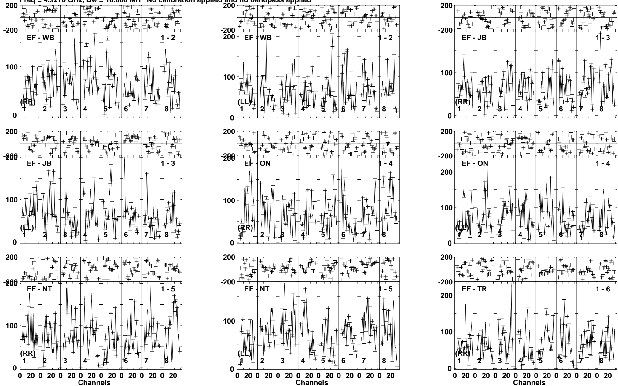
Lower frame: Micro Ampl Jy Top frame: Phas deg Vector averaged cross-power spectrum Baseline: EF (01) - WB (02) Timerange: 00/17:16:25 to 00/17:20:19
