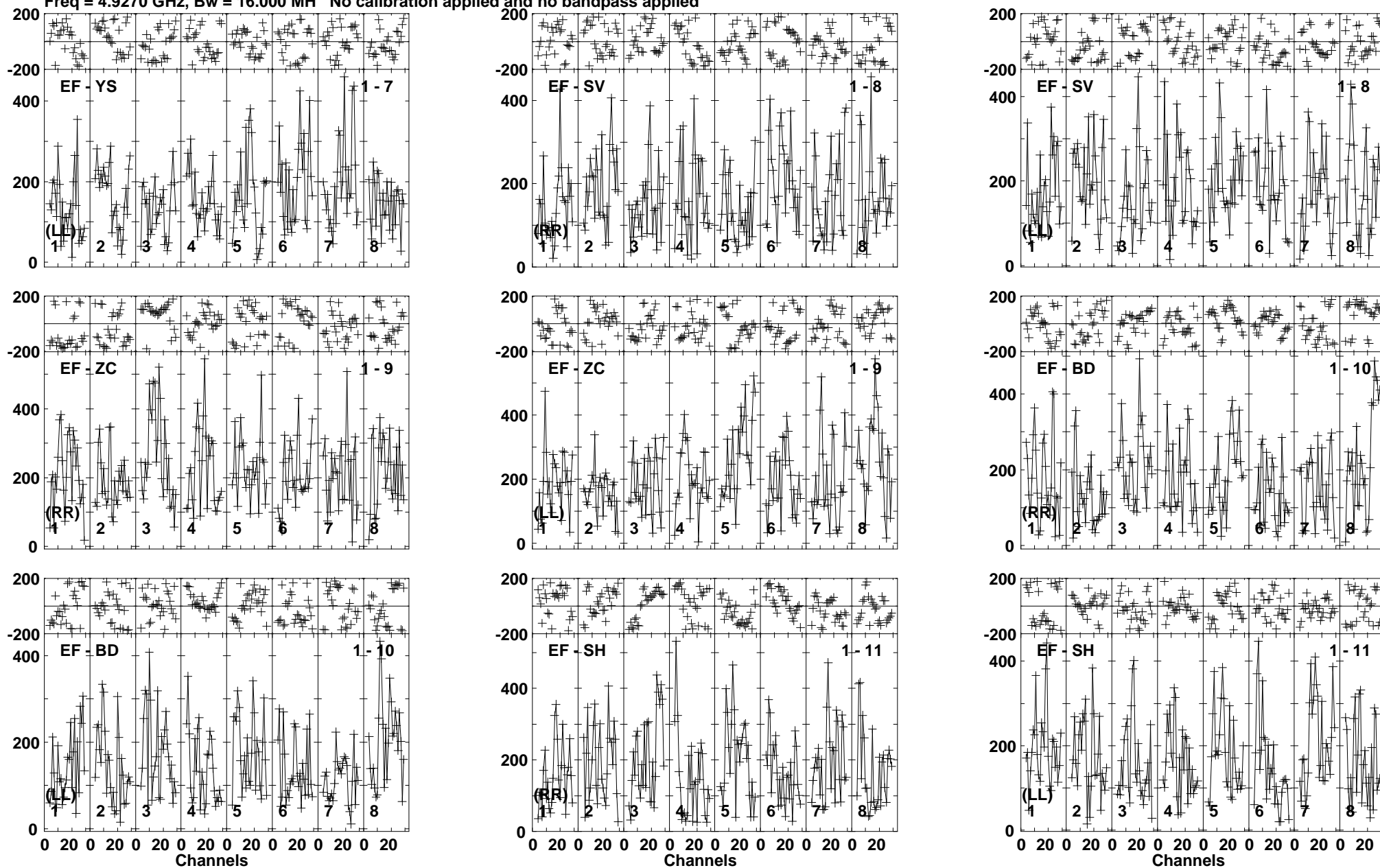
Lower frame: Micro Ampl Jy Top frame: Phas deg Vector averaged cross-power spectrum Baseline: EF (01) - YS (07) Timerange: 00/18:16:05 to 00/18:16:59
