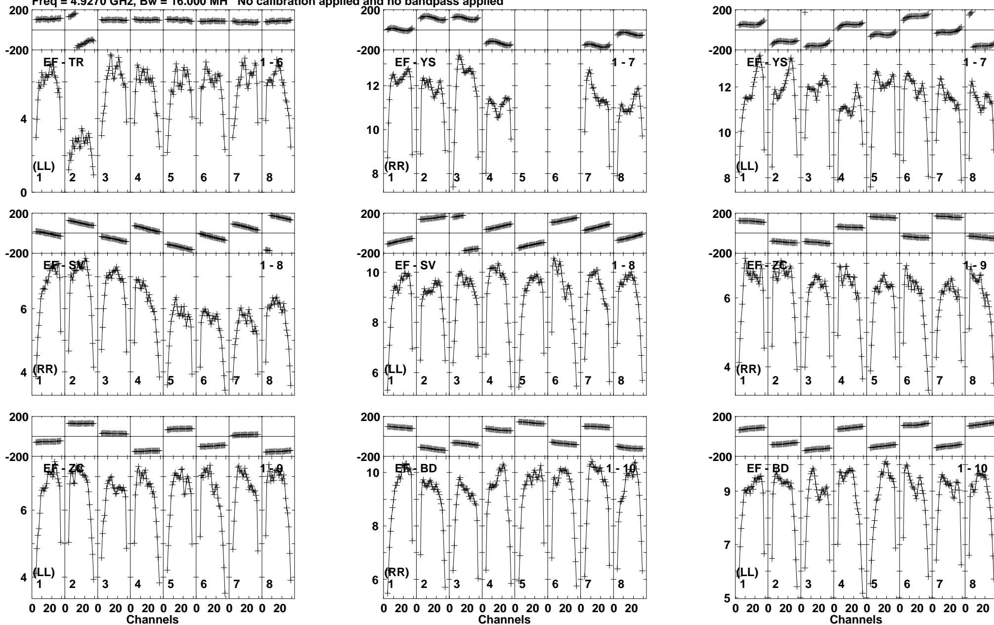
Lower frame: Milli Ampl Jy Top frame: Phas deg Vector averaged cross-power spectrum Baseline: EF (01) - TR (06) Timerange: 00/14:13:25 to 00/14:14:19
