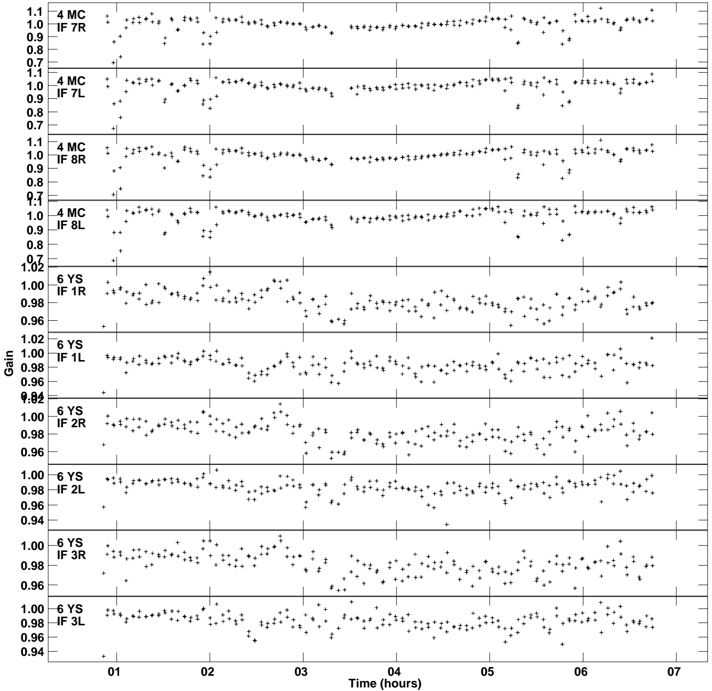
Plot file version 7 created 07-JUL-2016 18:21:18 Gain amp vs UTC time for J1128+5925.MULTI.1 SN 4 Rpol & Lpol IF 1 - 8
