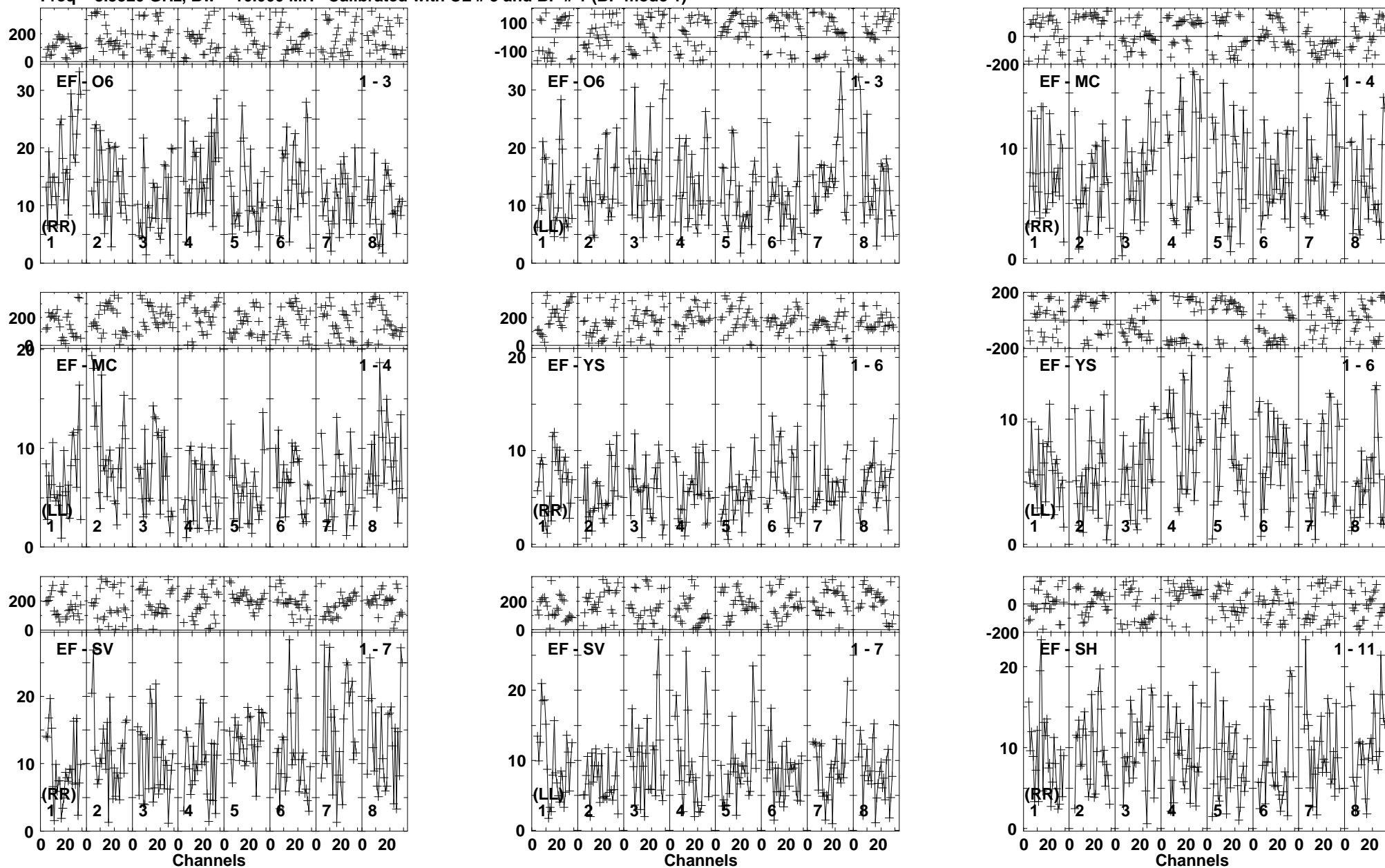
Lower frame: Milli Ampl Jy Top frame: Phas deg Vector averaged cross-power spectrum Baseline: EF (01) - O6 (03) Timerange: 00/01:27:35 to 00/01:30:30
