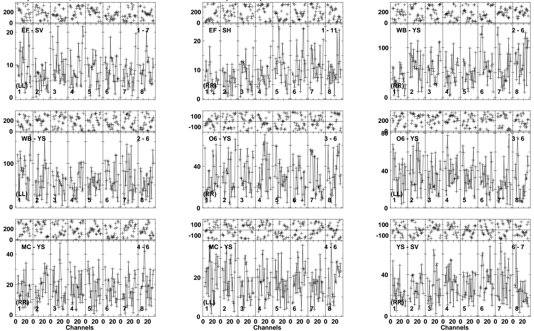
Lower frame: Milli Ampl Jy Top frame: Phas deg Vector averaged cross-power spectrum Baseline: EF (01) - SV (07) Timerange: 00/02:45:49 to 00/02:48:44
