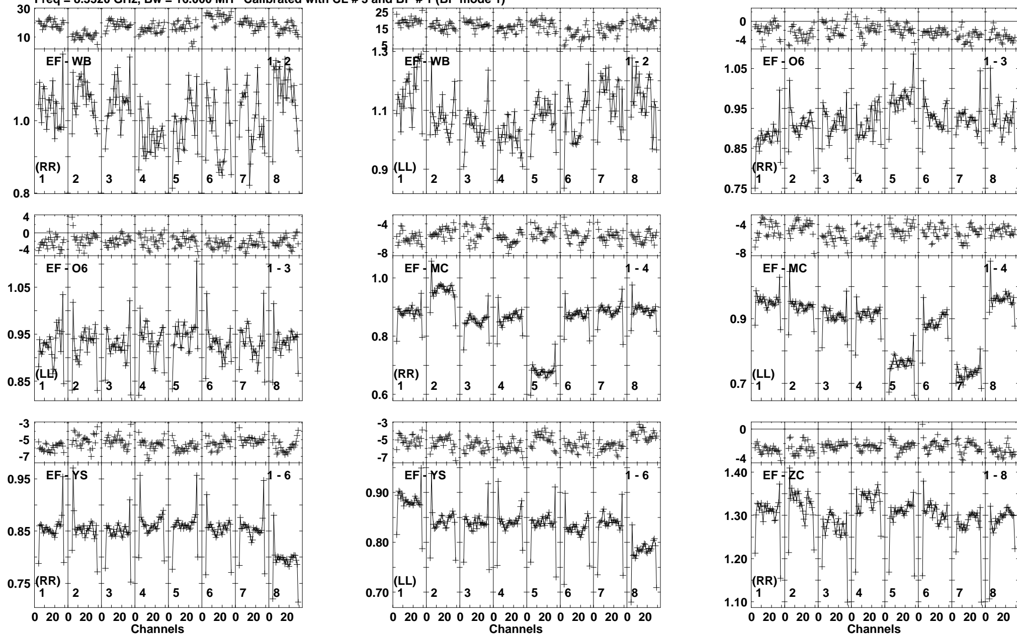
Lower frame: Ampl Jy Top frame: Phas deg Vector averaged cross-power spectrum Baseline: EF (01) - WB (02) Timerange: 00/06:27:35 to 00/06:28:30
