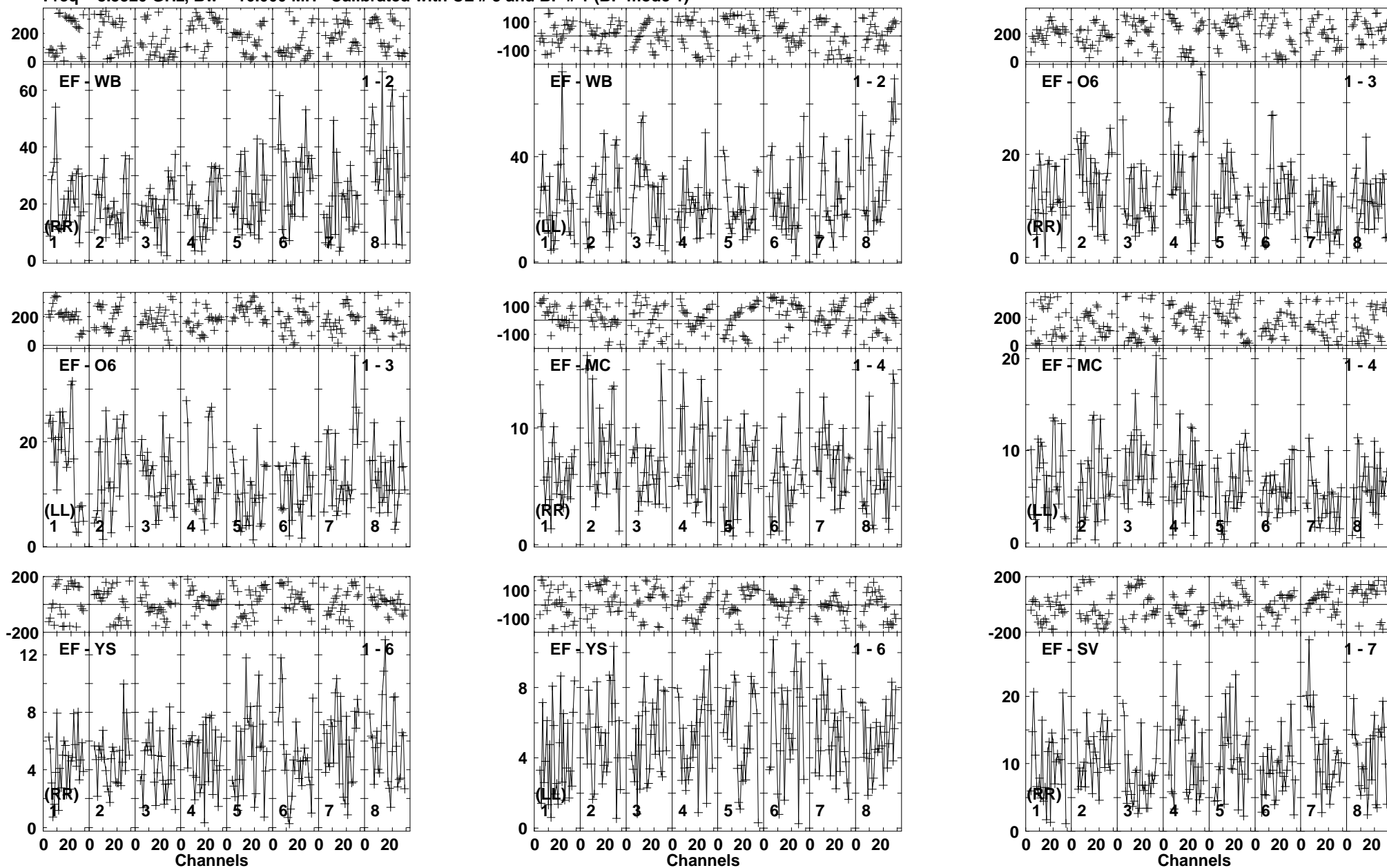
Lower frame: Milli Ampl Jy Top frame: Phas deg Vector averaged cross-power spectrum Baseline: EF (01) - WB (02) Timerange: 00/04:16:35 to 00/04:19:29
