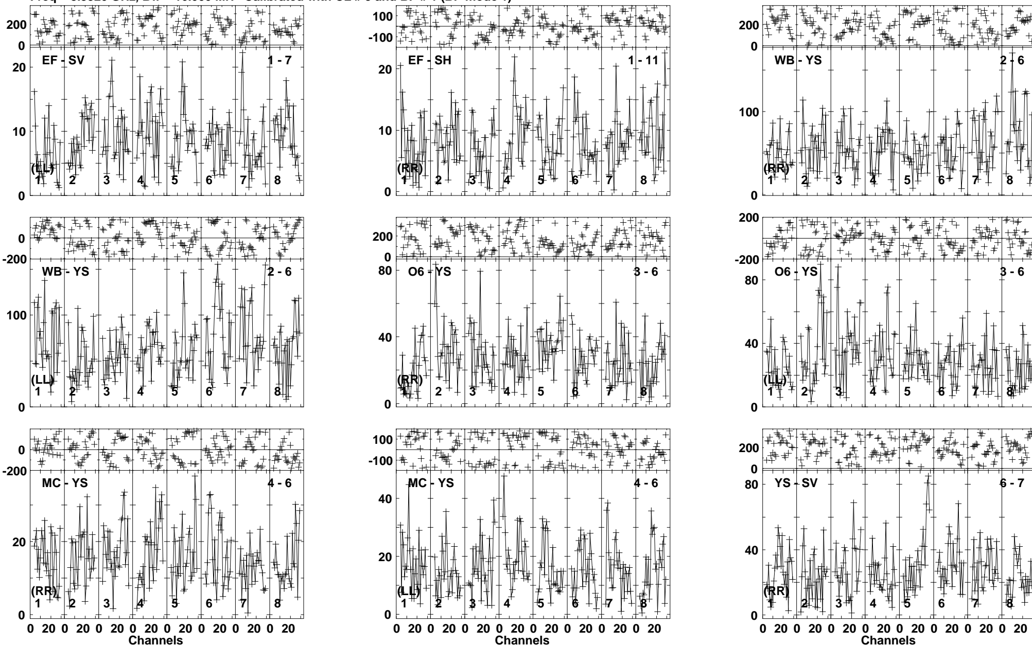
Lower frame: Milli Ampl Jy Top frame: Phas deg Vector averaged cross-power spectrum Baseline: EF (01) - SV (07) Timerange: 00/04:20:50 to 00/04:23:45
