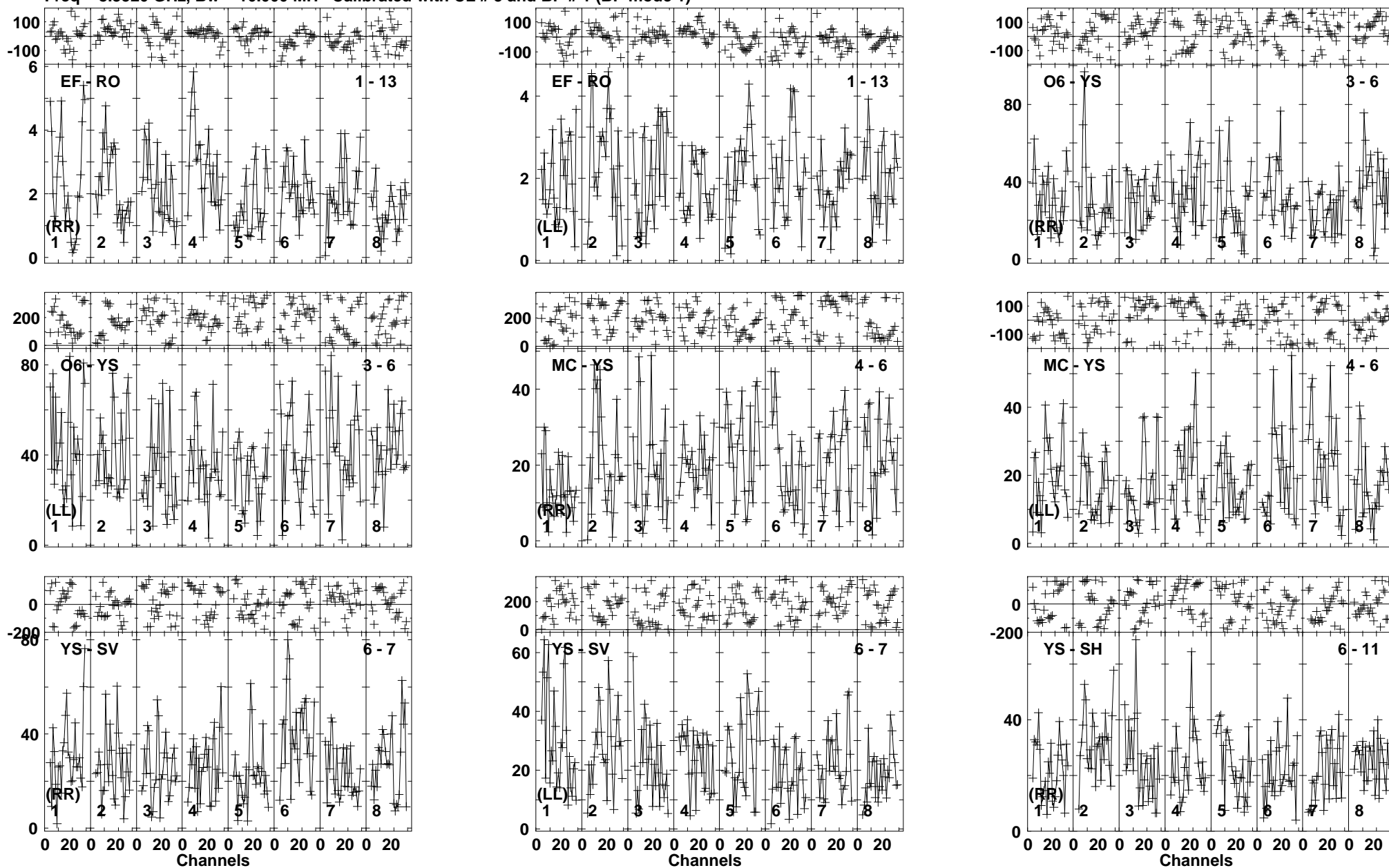
Lower frame: Milli Ampl Jy Top frame: Phas deg Vector averaged cross-power spectrum Baseline: EF (01) - RO (13) Timerange: 00/02:08:51 to 00/02:11:45
