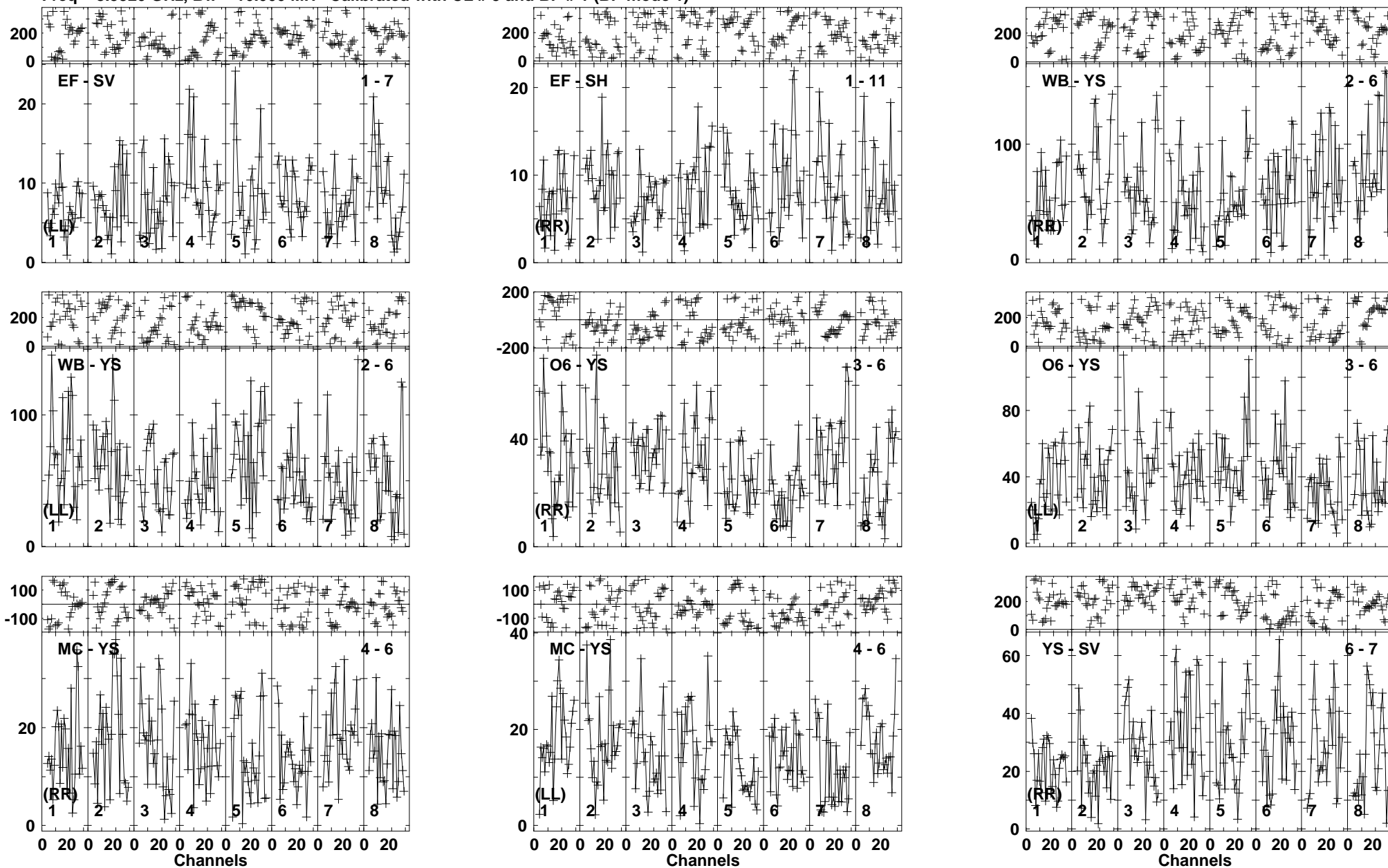
Lower frame: Milli Ampl Jy Top frame: Phas deg Vector averaged cross-power spectrum Baseline: EF (01) - SV (07) Timerange: 00/04:57:51 to 00/05:00:45
