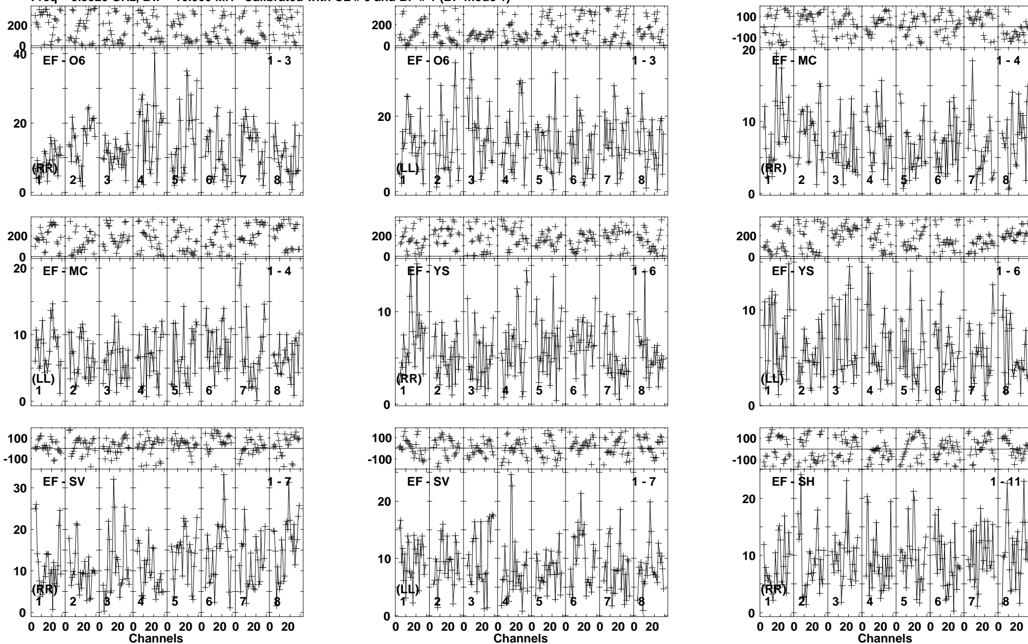
Lower frame: Milli Ampl Jy Top frame: Phas deg Vector averaged cross-power spectrum Baseline: EF (01) - O6 (03) Timerange: 00/01:44:05 to 00/01:46:59
