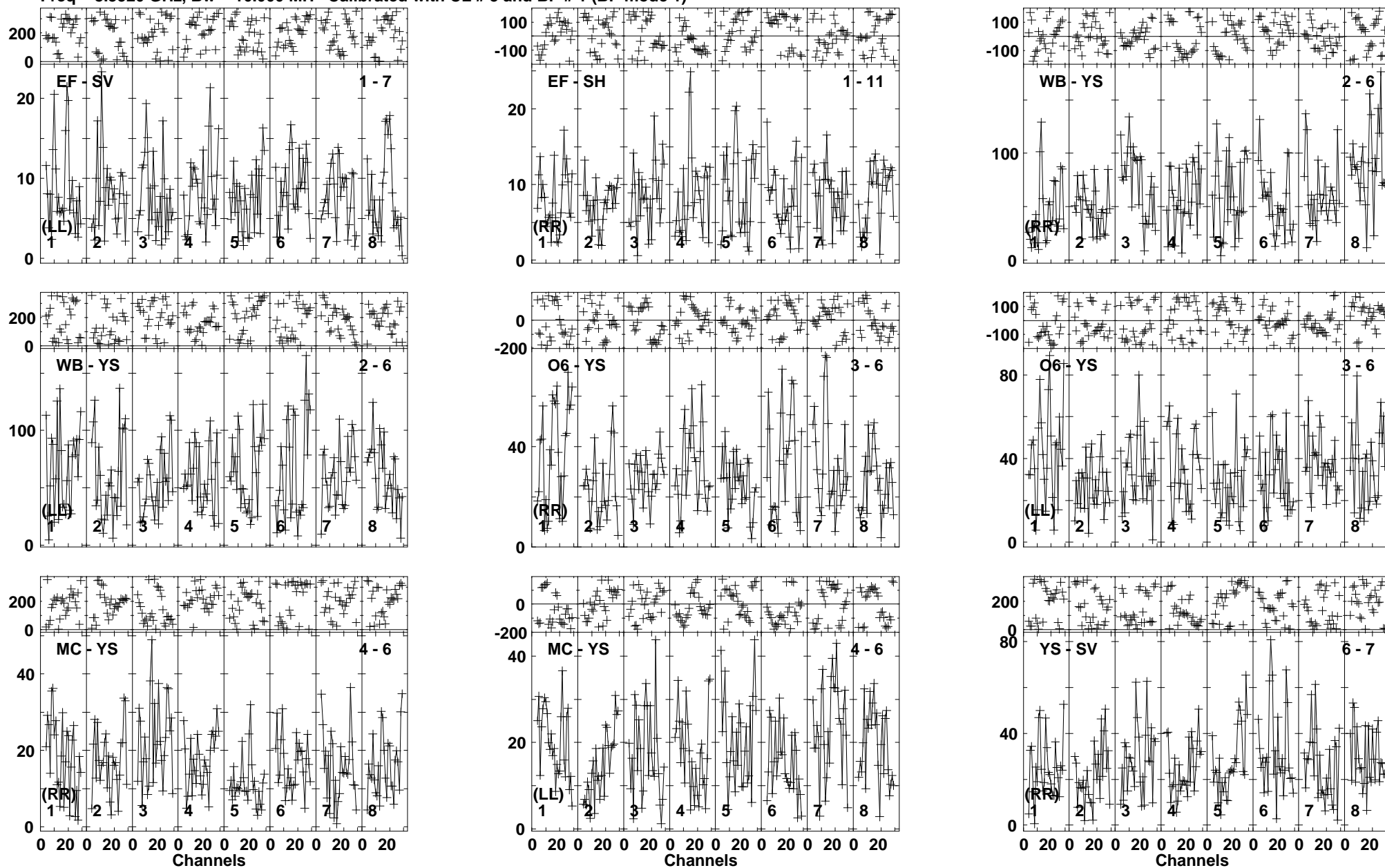
Lower frame: Milli Ampl Jy Top frame: Phas deg Vector averaged cross-power spectrum Baseline: EF (01) - SV (07) Timerange: 00/03:51:49 to 00/03:54:45
