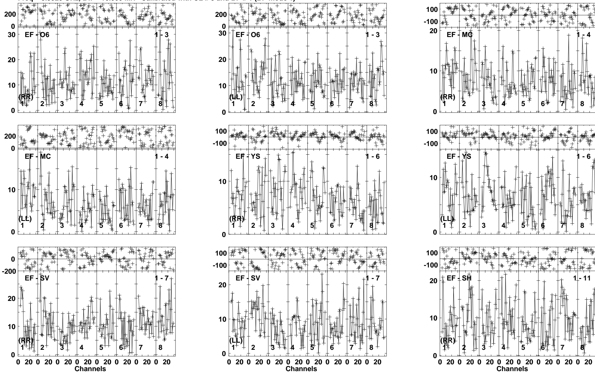
Lower frame: Milli Ampl Jy Top frame: Phas deg Vector averaged cross-power spectrum Baseline: EF (01) - O6 (03) Timerange: 00/02:12:50 to 00/02:15:44
