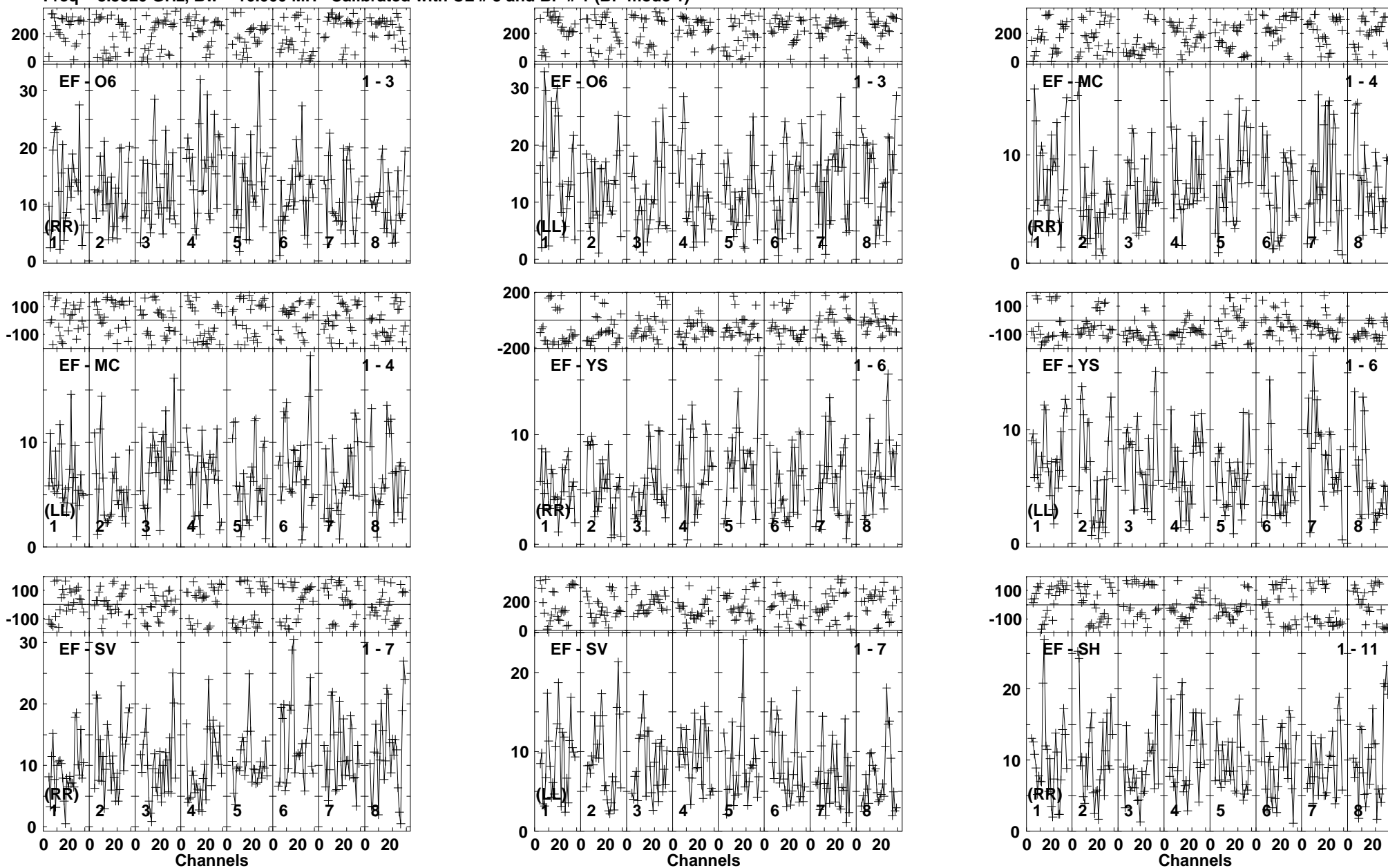
Lower frame: Milli Ampl Jy Top frame: Phas deg Vector averaged cross-power spectrum Baseline: EF (01) - O6 (03) Timerange: 00/02:04:36 to 00/02:07:30
