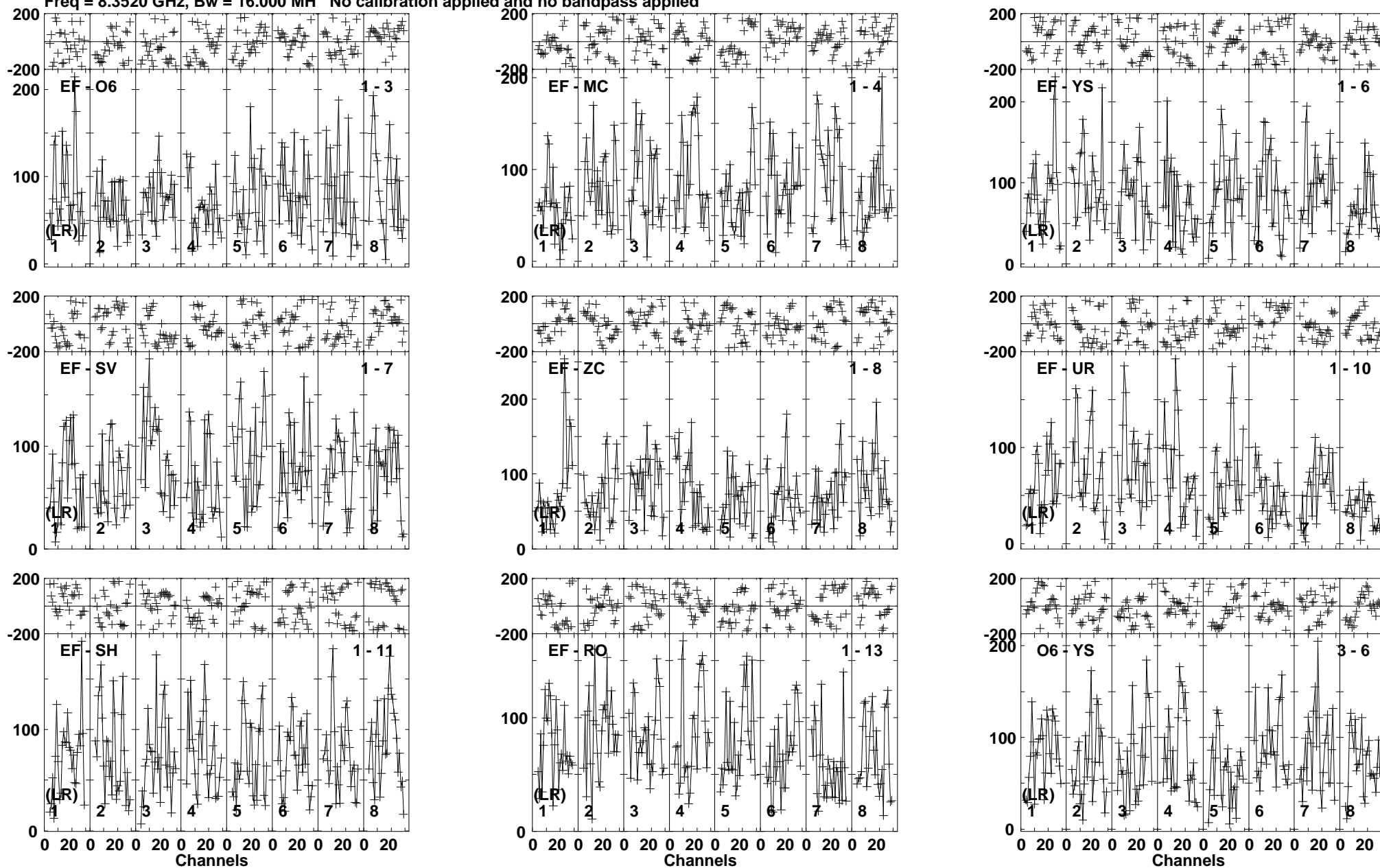
Lower frame: Micro Ampl Jy Top frame: Phas deg Vector averaged cross-power spectrum Baseline: EF (01) - O6 (03) Timerange: 00/01:56:21 to 00/01:59:15
