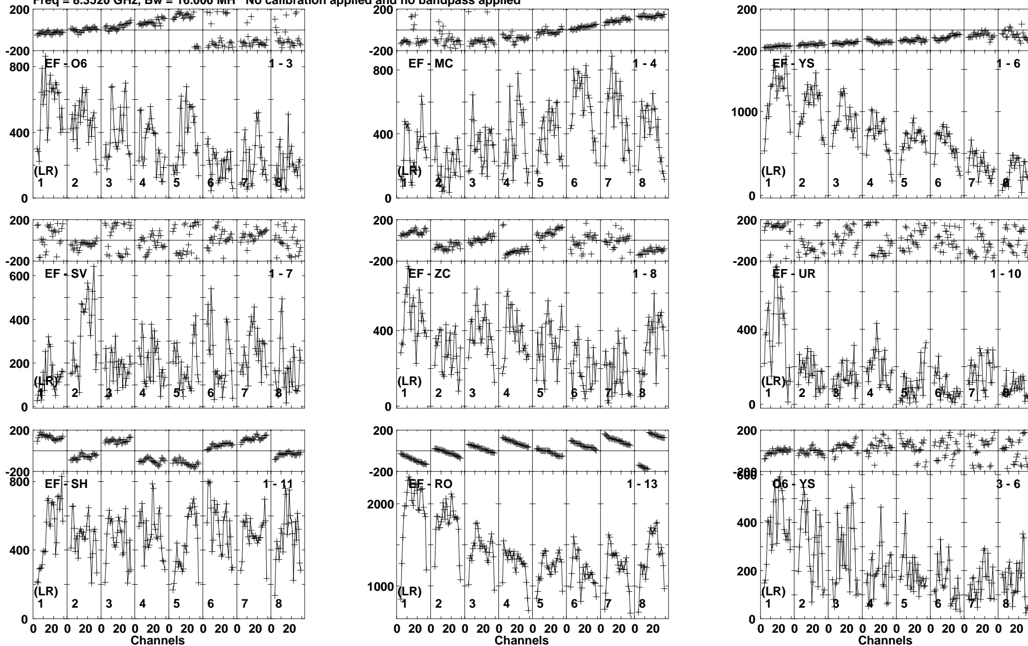
Lower frame: Micro Ampl Jy Top frame: Phas deg Vector averaged cross-power spectrum Baseline: EF (01) - O6 (03) Timerange: 00/02:20:04 to 00/02:21:00
