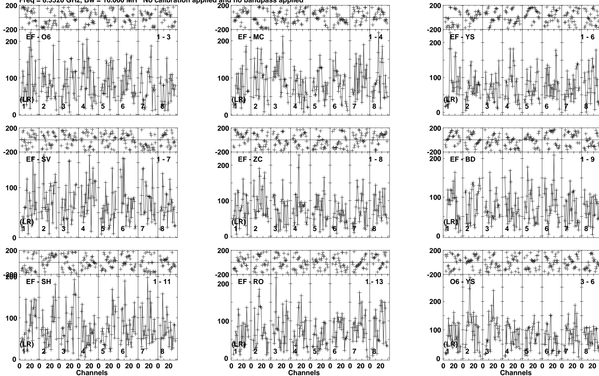
Lower frame: Micro Ampl Jy Top frame: Phas deg Vector averaged cross-power spectrum Baseline: EF (01) - O6 (03) Timerange: 00/00:58:35 to 00/01:01:29
