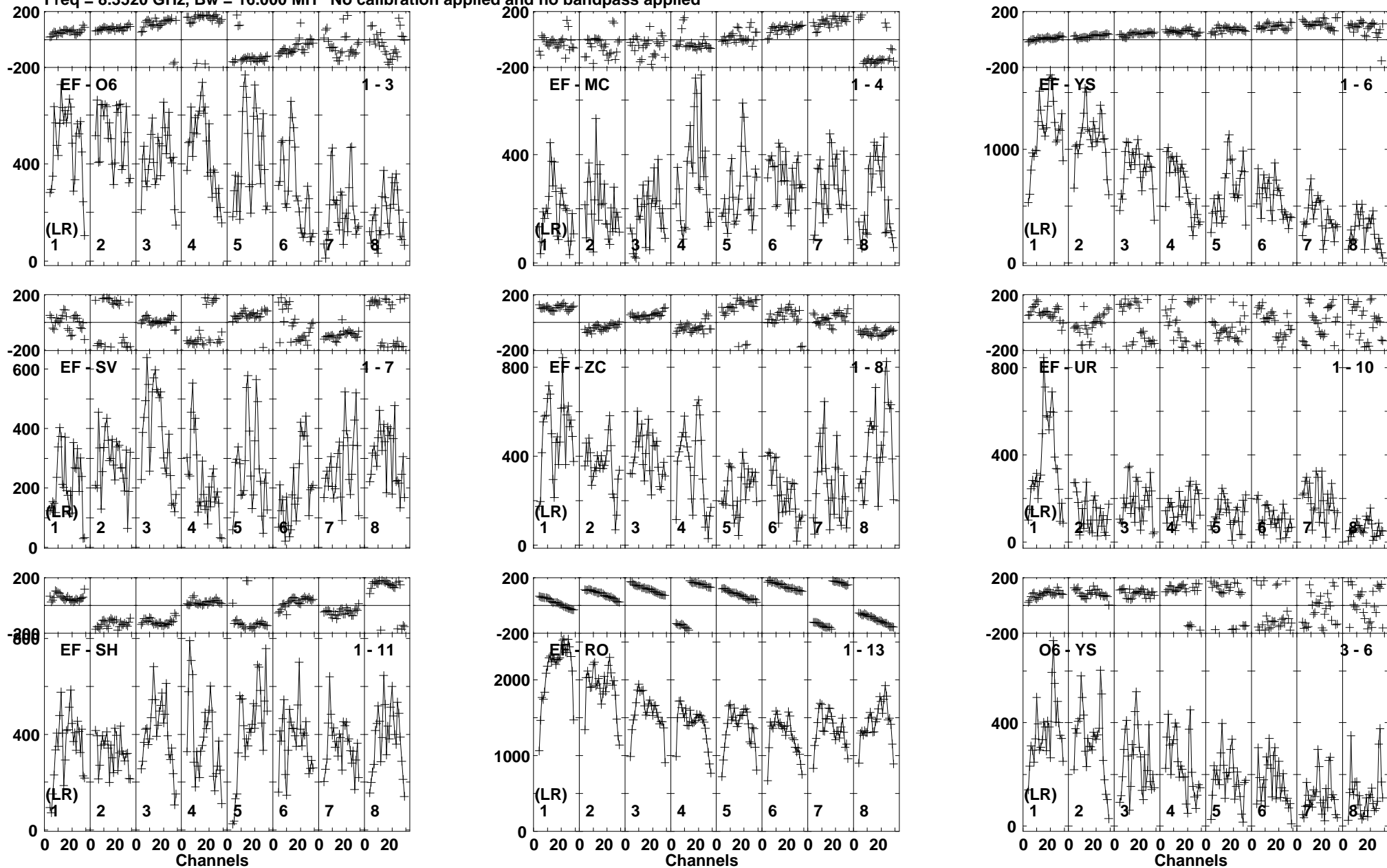
Lower frame: Micro Ampl Jy Top frame: Phas deg Vector averaged cross-power spectrum Baseline: EF (01) - O6 (03) Timerange: 00/01:38:50 to 00/01:39:45
