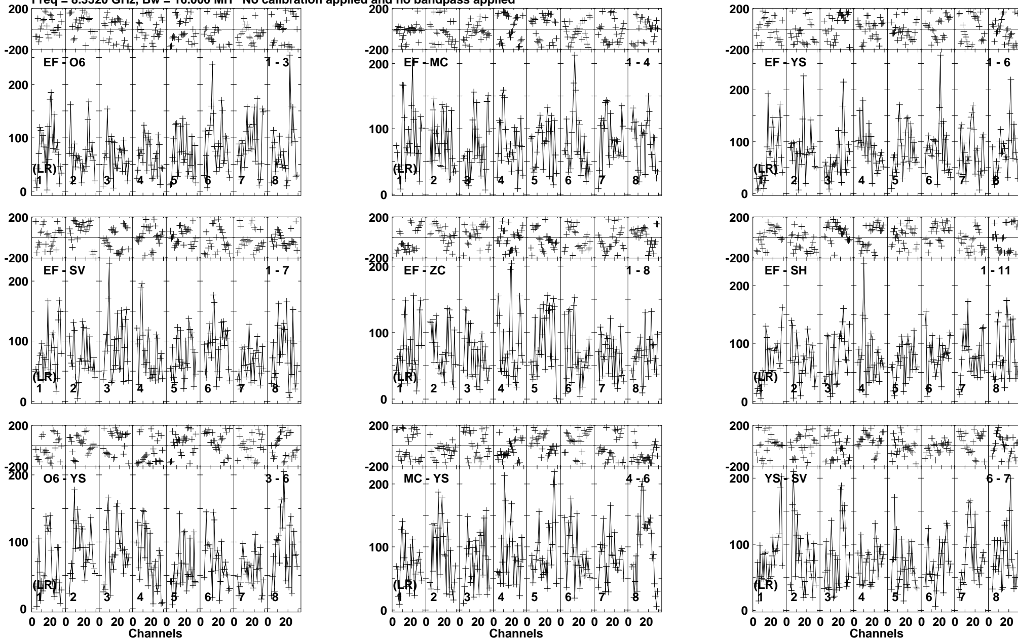
Lower frame: Micro Ampl Jy Top frame: Phas deg Vector averaged cross-power spectrum Baseline: EF (01) - O6 (03) Timerange: 00/02:25:21 to 00/02:28:15
