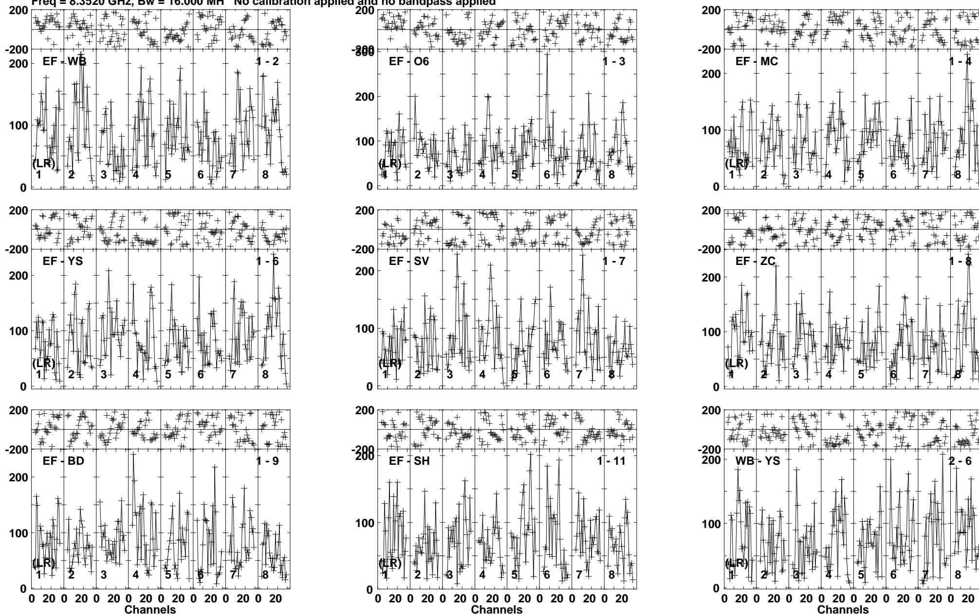
Lower frame: Micro Ampl Jy Top frame: Phas deg Vector averaged cross-power spectrum Baseline: EF (01) - WB (02) Timerange: 00/05:55:32 to 00/05:58:30
