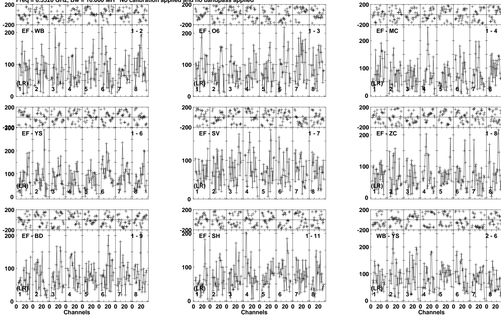
Lower frame: Micro Ampl Jy Top frame: Phas deg Vector averaged cross-power spectrum Baseline: EF (01) - WB (02) Timerange: 00/03:47:50 to 00/03:50:45
