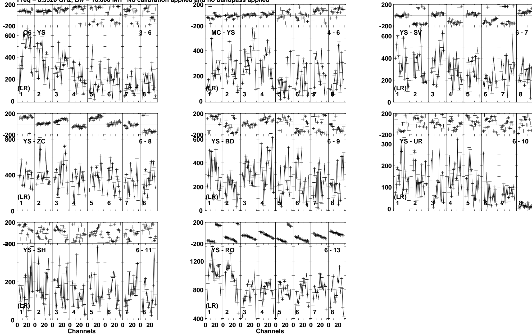
Lower frame: Micro Ampl Jy Top frame: Phas deg Vector averaged cross-power spectrum Baseline: O6 (03) - YS (06) Timerange: 00/01:22:20 to 00/01:23:14
