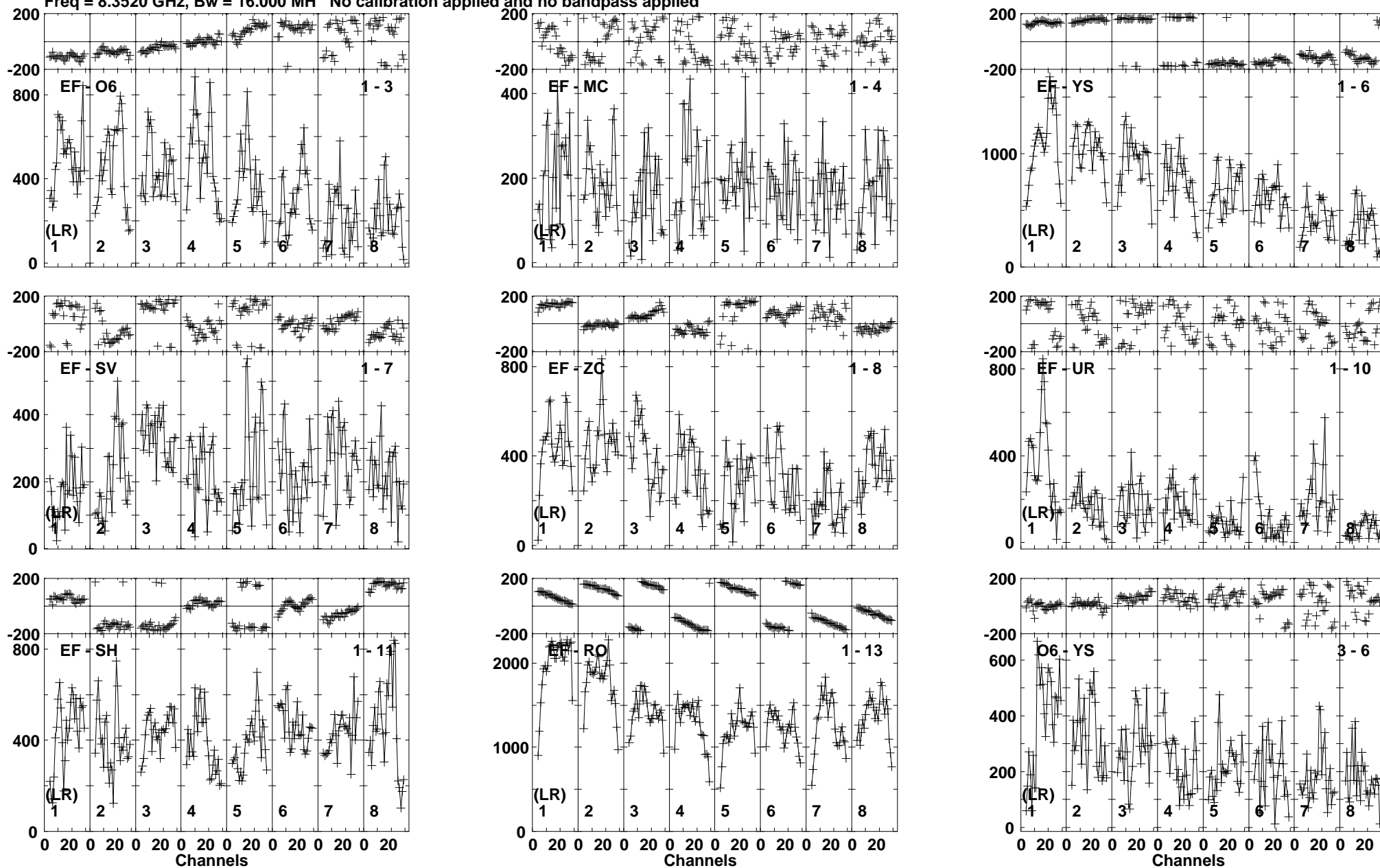
Lower frame: Micro Ampl Jy Top frame: Phas deg Vector averaged cross-power spectrum Baseline: EF (01) - O6 (03) Timerange: 00/01:59:55 to 00/02:00:29
