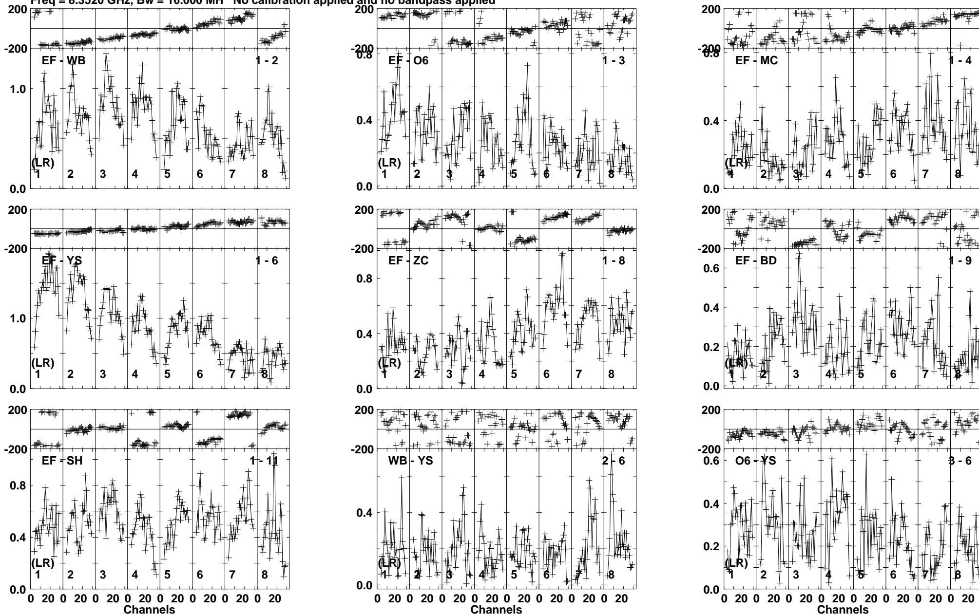
Lower frame: Milli Ampl Jy Top frame: Phas deg Vector averaged cross-power spectrum Baseline: EF (01) - WB (02) Timerange: 00/06:23:57 to 00/06:24:30
