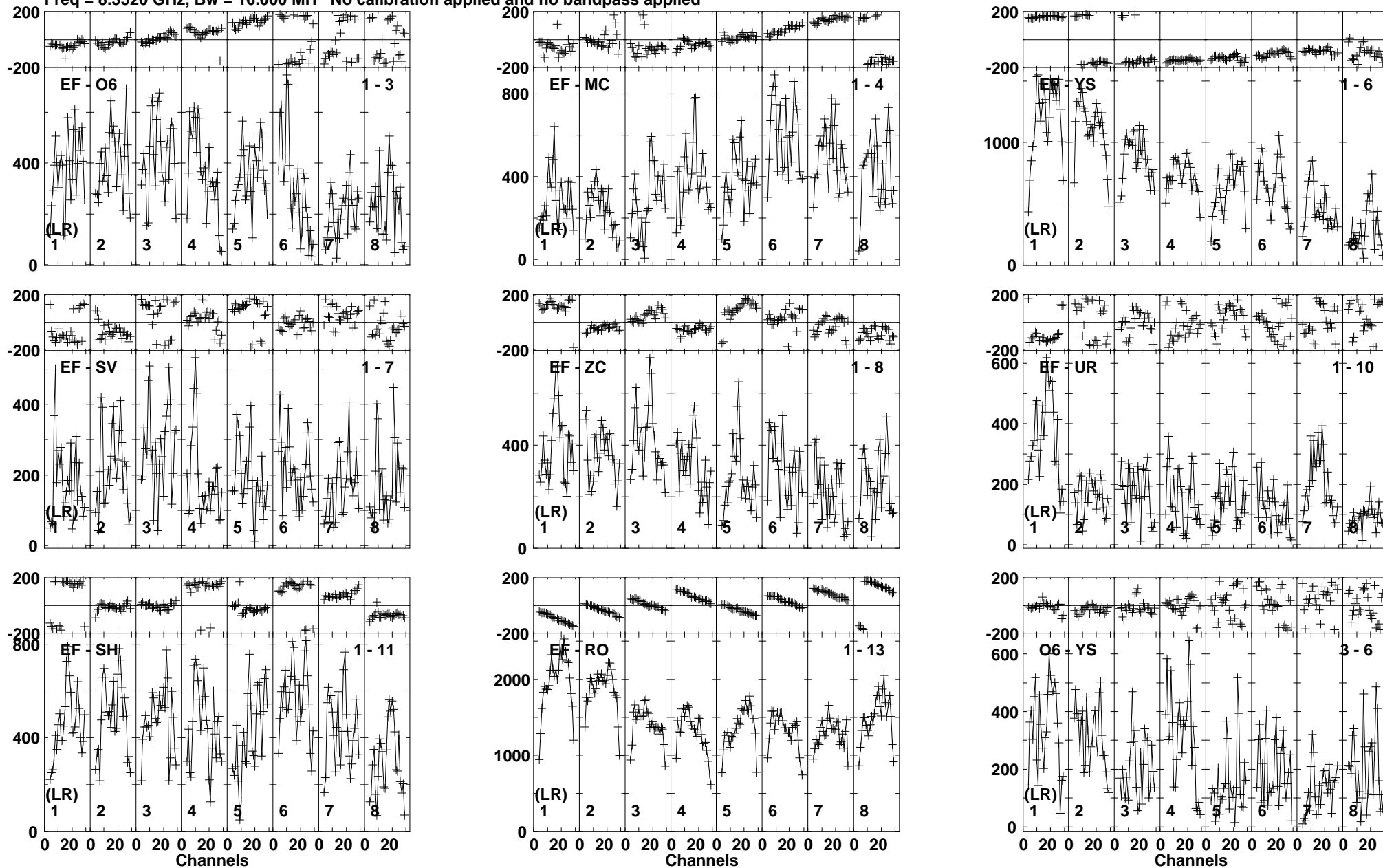
Lower frame: Micro Ampl Jy Top frame: Phas deg Vector averaged cross-power spectrum Baseline: EF (01) - O6 (03) Timerange: 00/02:08:11 to 00/02:08:44
