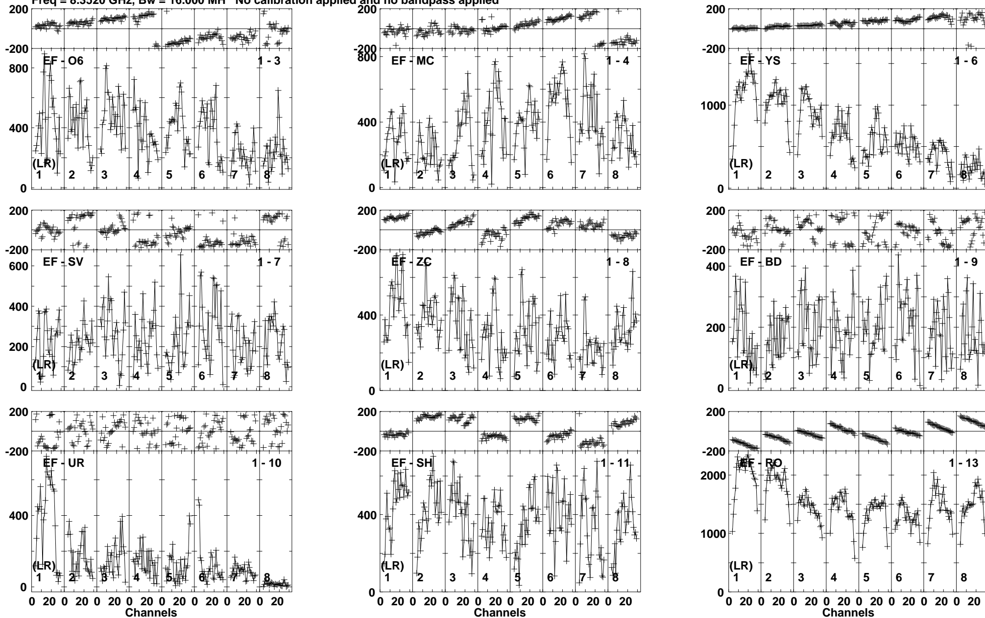
Lower frame: Micro Ampl Jy Top frame: Phas deg Vector averaged cross-power spectrum Baseline: EF (01) - O6 (03) Timerange: 00/01:35:11 to 00/01:35:44
