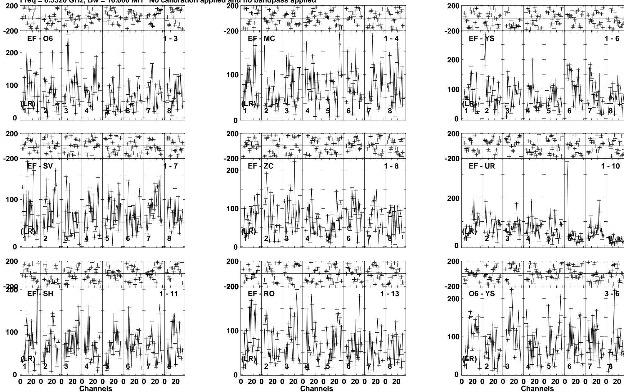
Lower frame: Micro Ampl Jy Top frame: Phas deg Vector averaged cross-power spectrum Baseline: EF (01) - O6 (03) Timerange: 00/01:35:50 to 00/01:38:44
