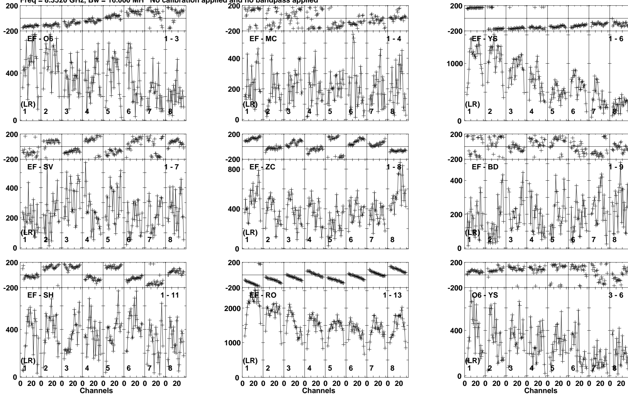
Lower frame: Micro Ampl Jy Top frame: Phas deg Vector averaged cross-power spectrum Baseline: EF (01) - O6 (03) Timerange: 00/01:10:26 to 00/01:10:59
