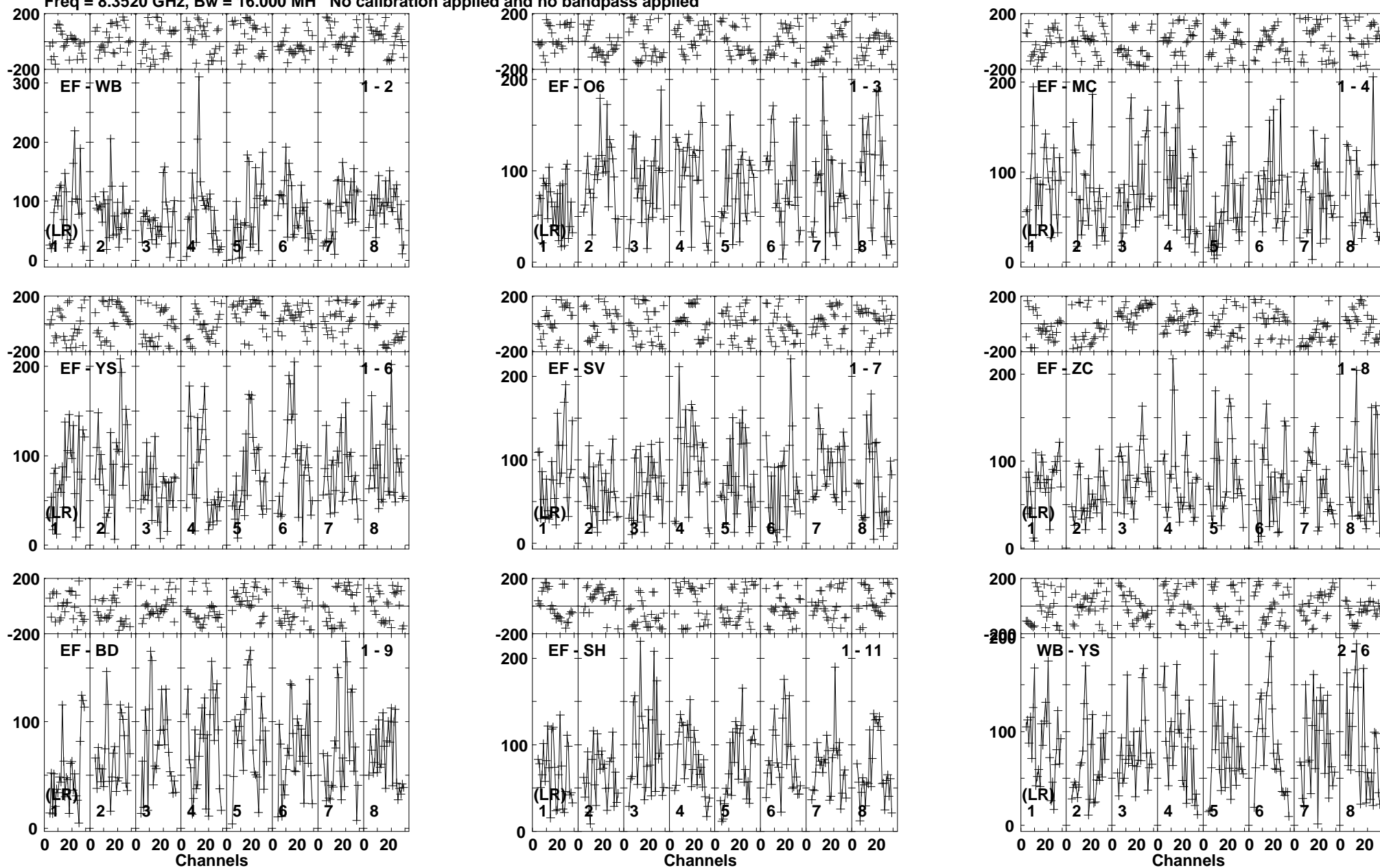
Lower frame: Micro Ampl Jy Top frame: Phas deg Vector averaged cross-power spectrum Baseline: EF (01) - WB (02) Timerange: 00/04:24:50 to 00/04:27:45
