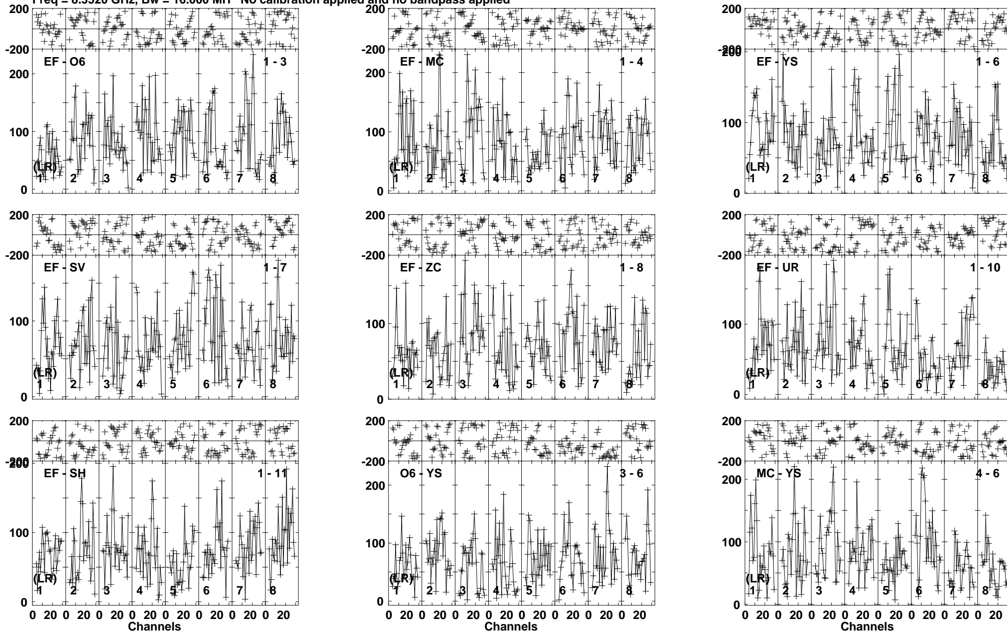
Lower frame: Micro Ampl Jy Top frame: Phas deg Vector averaged cross-power spectrum Baseline: EF (01) - O6 (03) Timerange: 00/02:21:05 to 00/02:23:59
