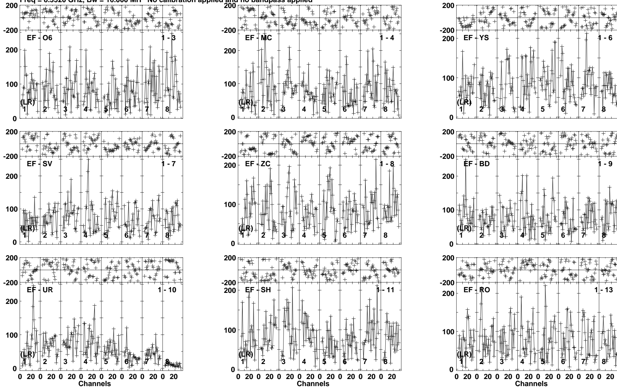
Lower frame: Micro Ampl Jy Top frame: Phas deg Vector averaged cross-power spectrum Baseline: EF (01) - O6 (03) Timerange: 00/01:15:05 to 00/01:17:59
