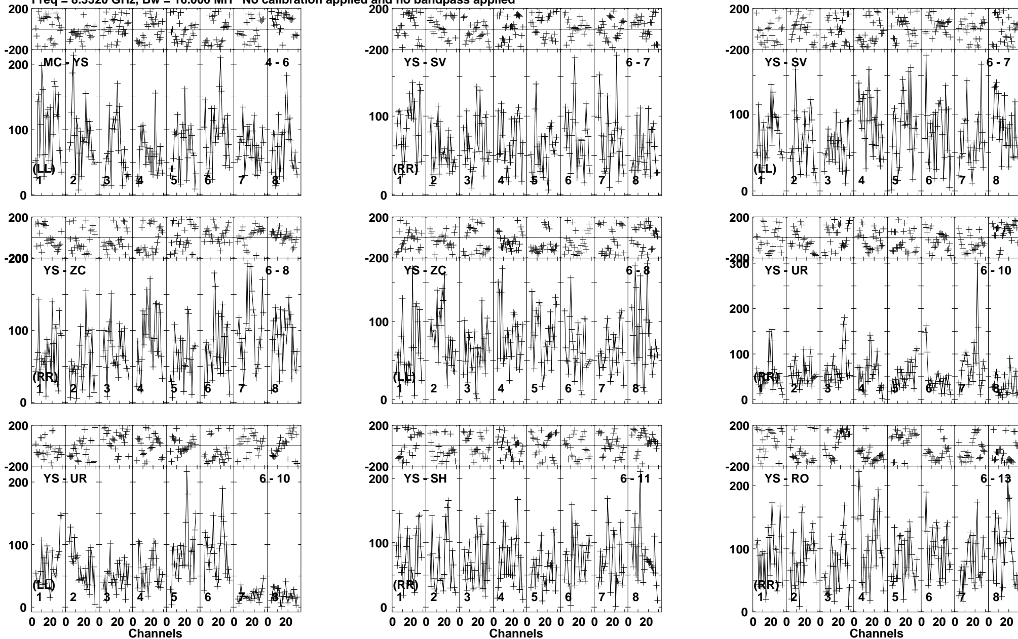
Lower frame: Micro Ampl Jy Top frame: Phas deg Vector averaged cross-power spectrum Baseline: MC (04) - YS (06) Timerange: 00/02:04:36 to 00/02:07:30
