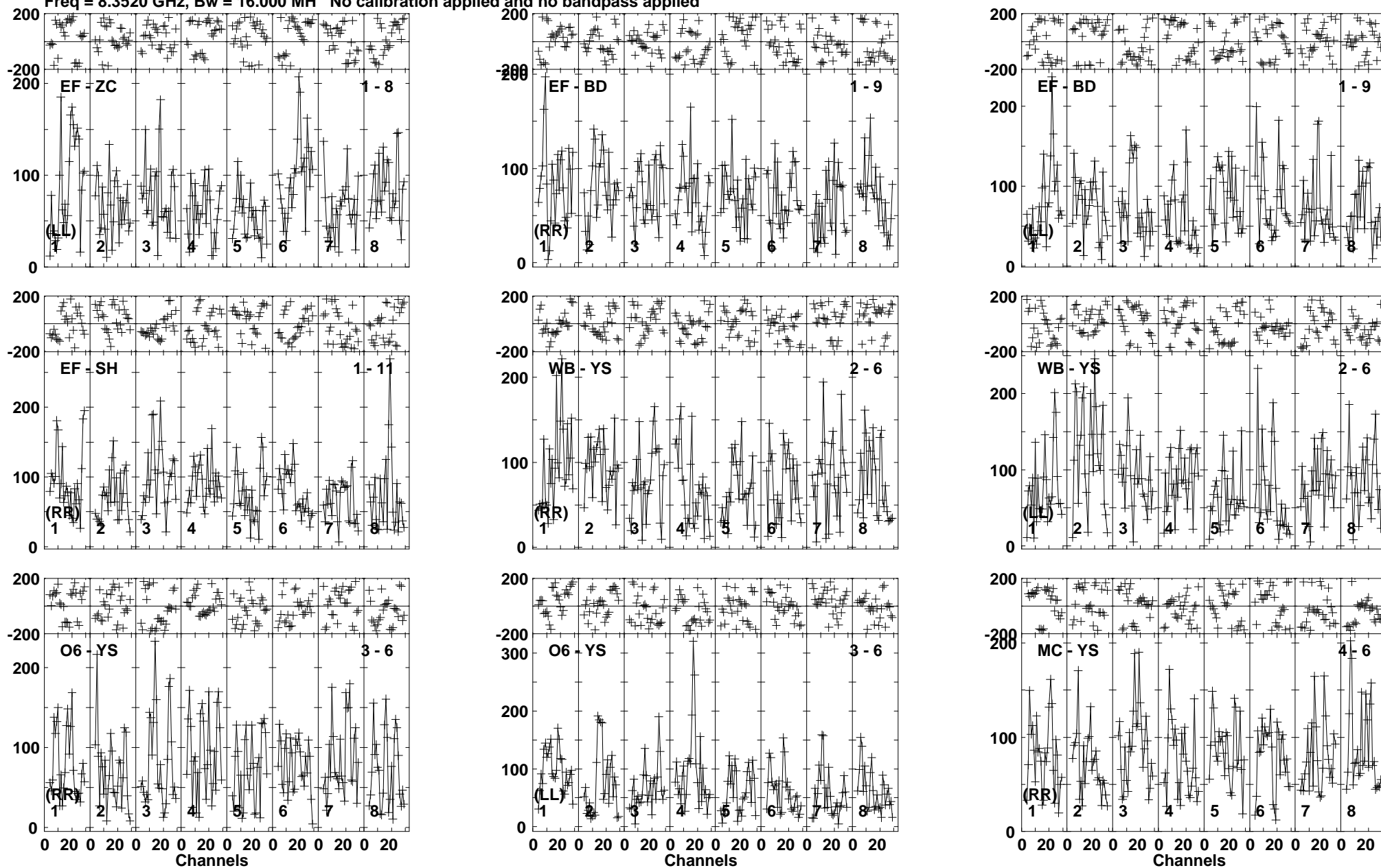
Lower frame: Micro Ampl Jy Top frame: Phas deg Vector averaged cross-power spectrum Baseline: EF (01) - ZC (08) Timerange: 00/06:32:50 to 00/06:35:45
