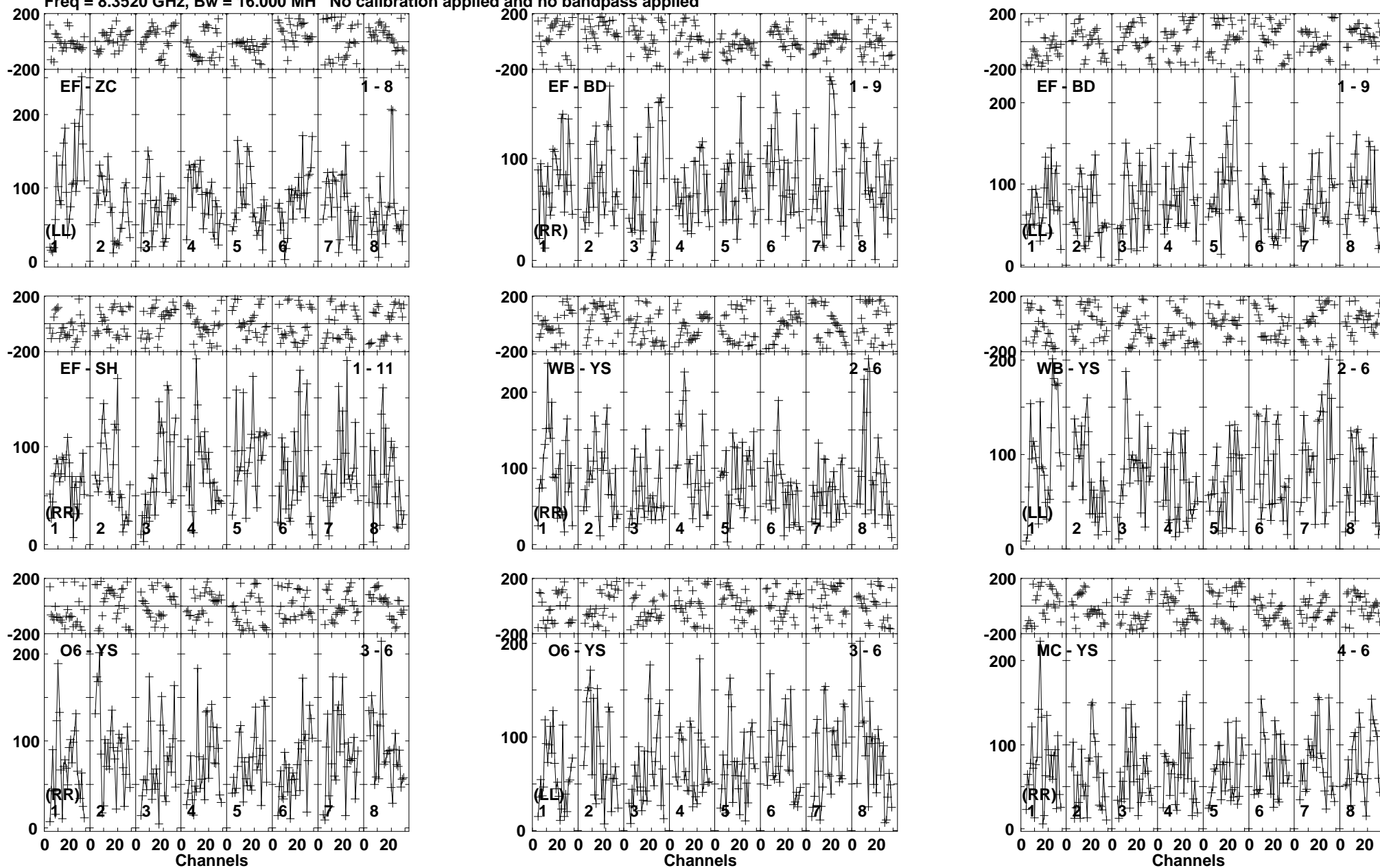
Lower frame: Micro Ampl Jy Top frame: Phas deg Vector averaged cross-power spectrum Baseline: EF (01) - ZC (08) Timerange: 00/06:20:20 to 00/06:23:14
