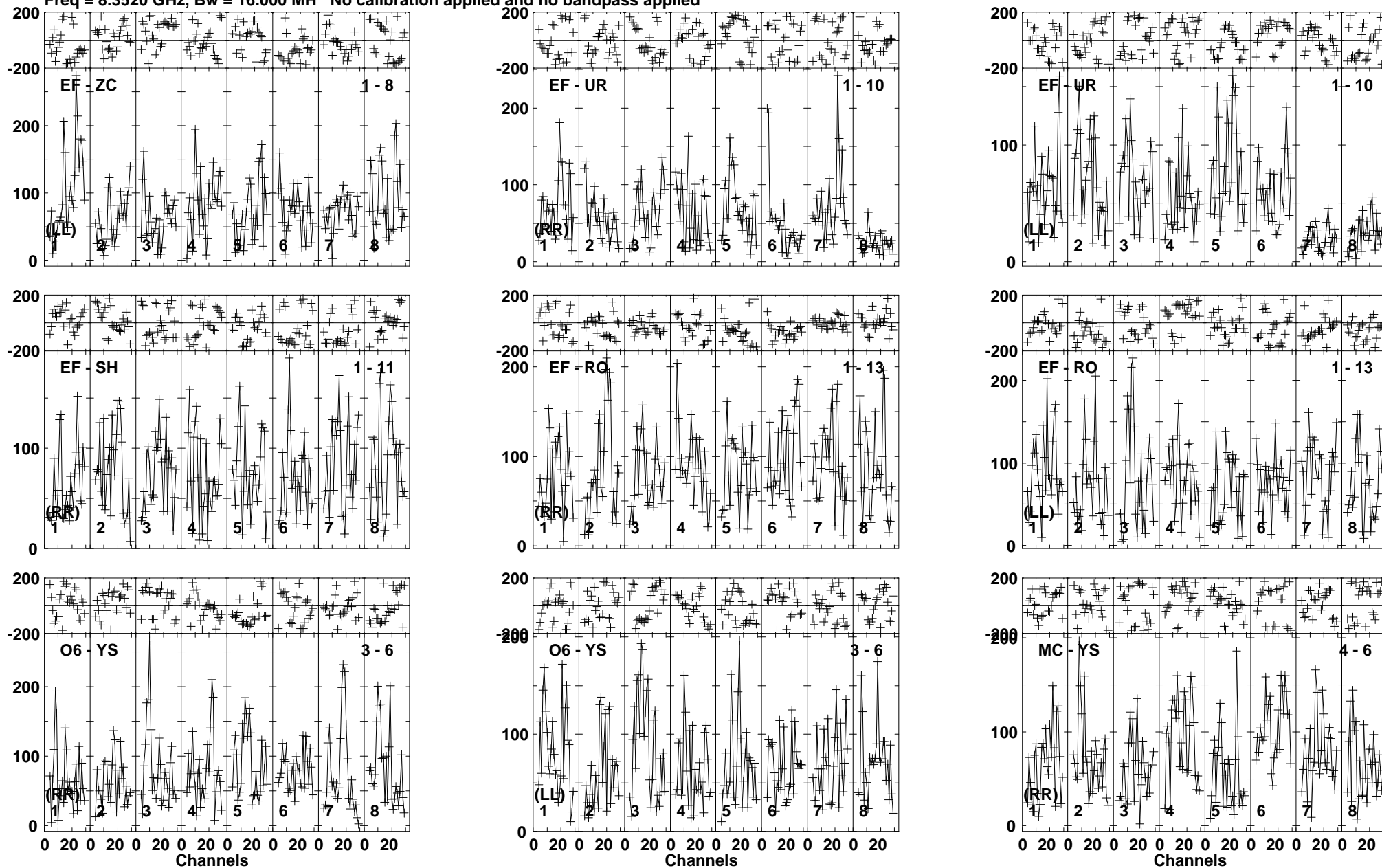
Lower frame: Micro Ampl Jy Top frame: Phas deg Vector averaged cross-power spectrum Baseline: EF (01) - ZC (08) Timerange: 00/02:00:35 to 00/02:03:30
