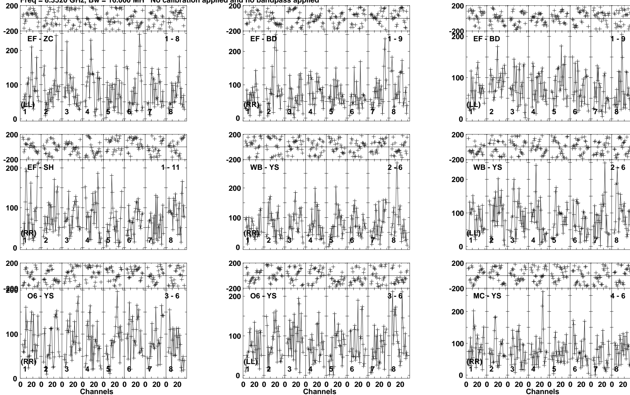
Lower frame: Micro Ampl Jy Top frame: Phas deg Vector averaged cross-power spectrum Baseline: EF (01) - ZC (08) Timerange: 00/06:16:20 to 00/06:19:15
