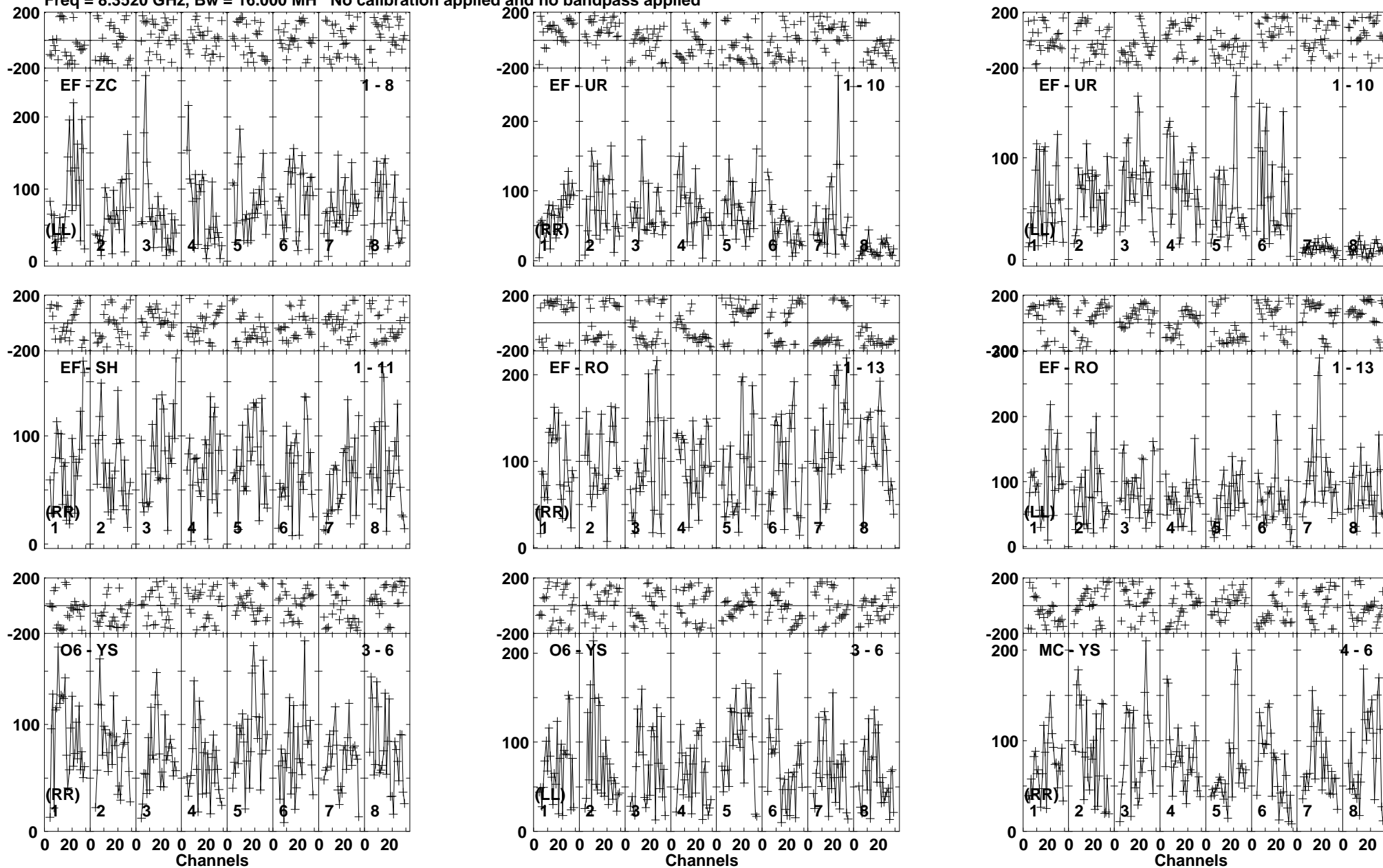
Lower frame: Micro Ampl Jy Top frame: Phas deg Vector averaged cross-power spectrum Baseline: EF (01) - ZC (08) Timerange: 00/01:35:50 to 00/01:38:44
