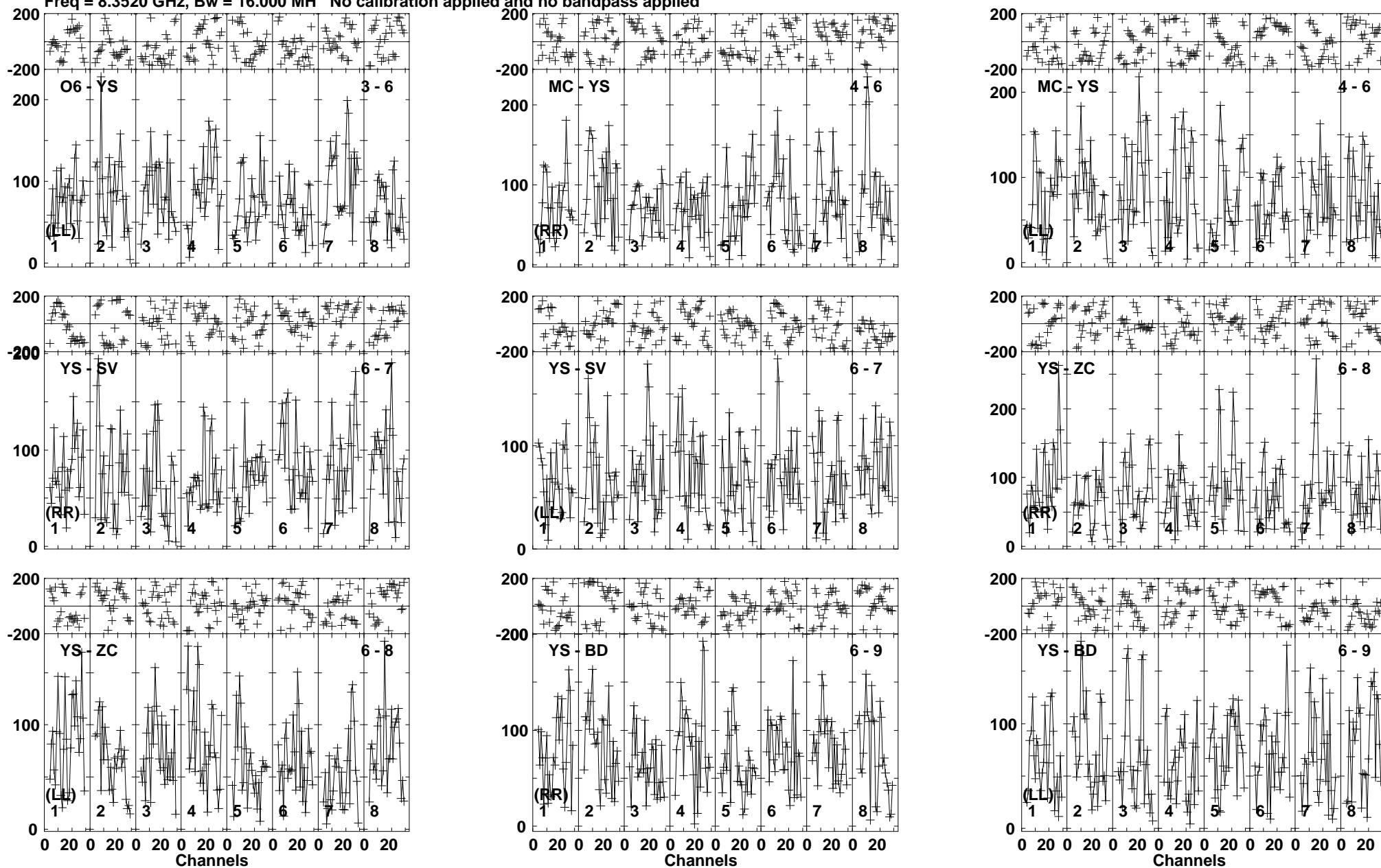
Lower frame: Micro Ampl Jy Top frame: Phas deg Vector averaged cross-power spectrum Baseline: O6 (03) - YS (06) Timerange: 00/05:51:35 to 00/05:54:30
