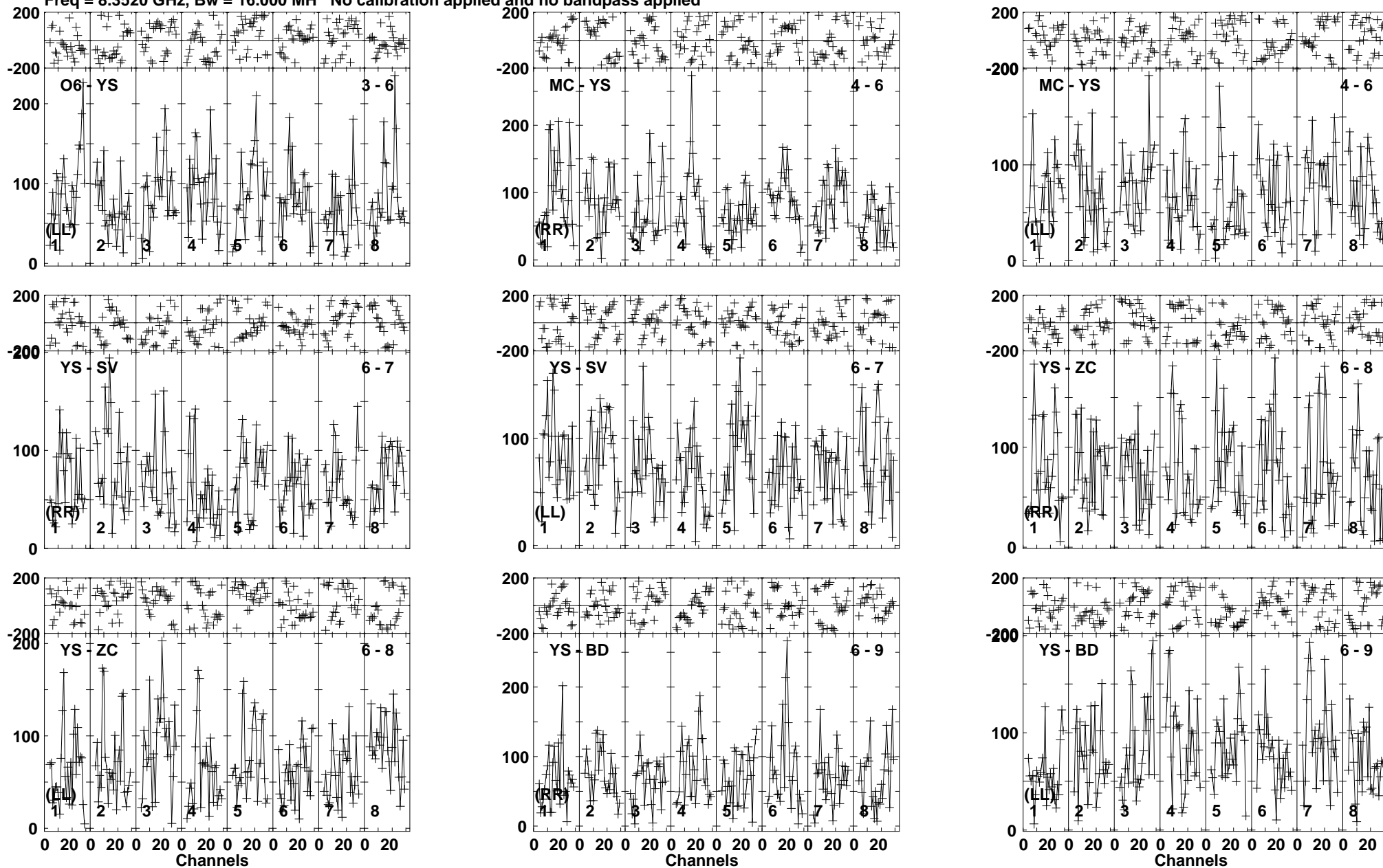
Lower frame: Micro Ampl Jy Top frame: Phas deg Vector averaged cross-power spectrum Baseline: O6 (03) - YS (06) Timerange: 00/05:35:06 to 00/05:37:59
