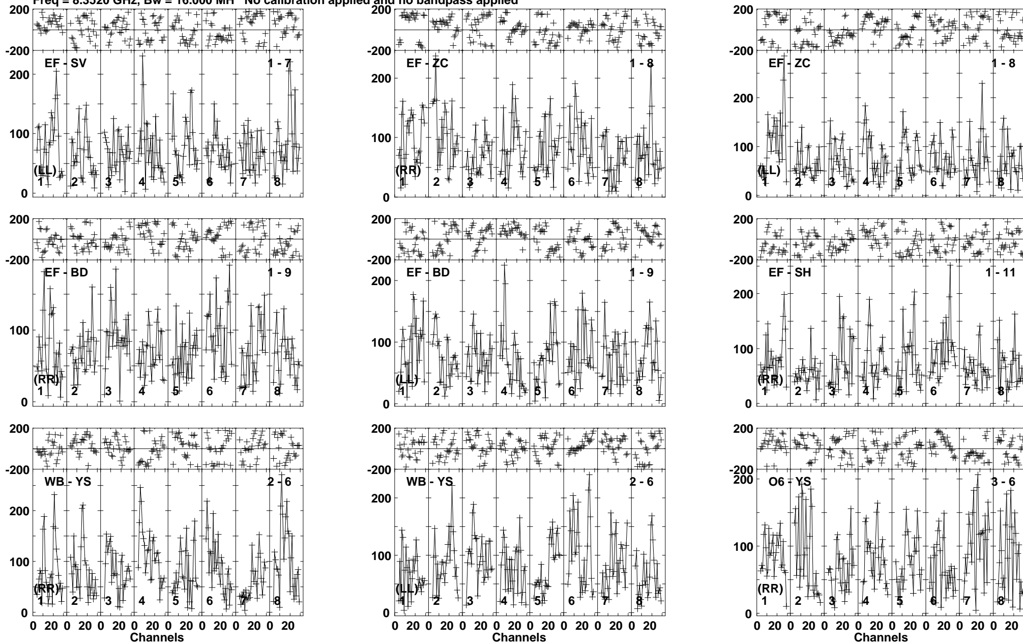
Lower frame: Micro Ampl Jy Top frame: Phas deg Vector averaged cross-power spectrum Baseline: EF (01) - SV (07) Timerange: 00/04:00:06 to 00/04:02:59
