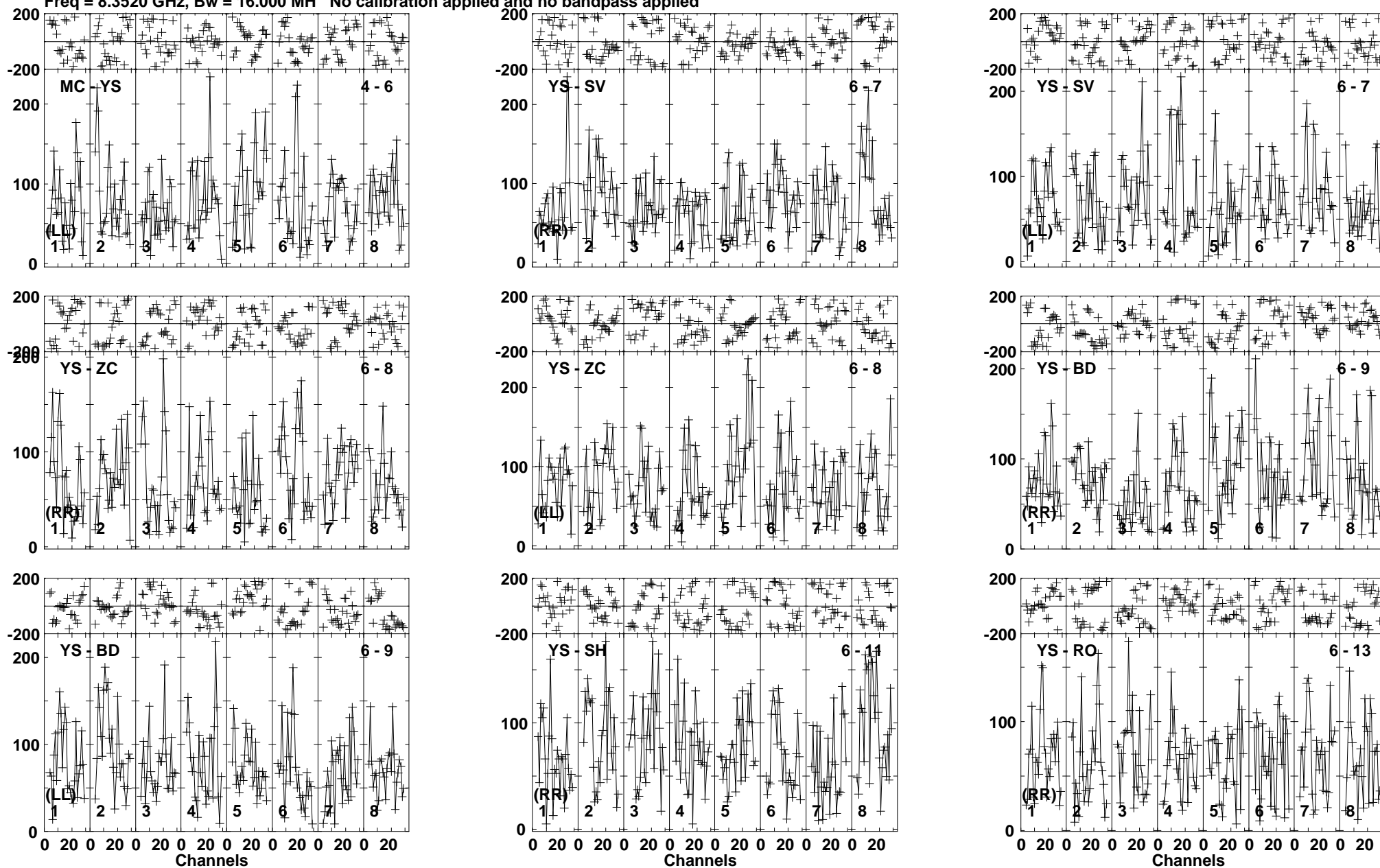
Lower frame: Micro Ampl Jy Top frame: Phas deg Vector averaged cross-power spectrum Baseline: MC (04) - YS (06) Timerange: 00/01:02:51 to 00/01:05:45
