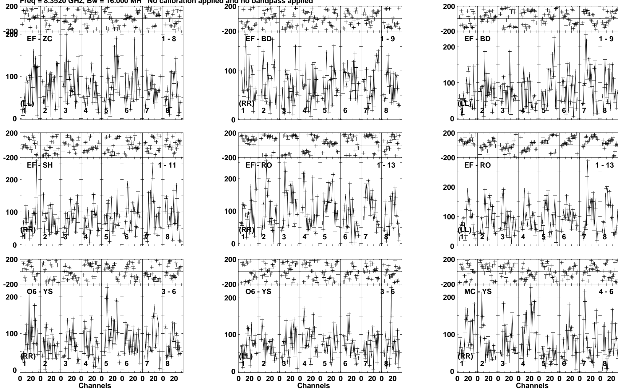
Lower frame: Micro Ampl Jy Top frame: Phas deg Vector averaged cross-power spectrum Baseline: EF (01) - ZC (08) Timerange: 00/00:58:35 to 00/01:01:29
