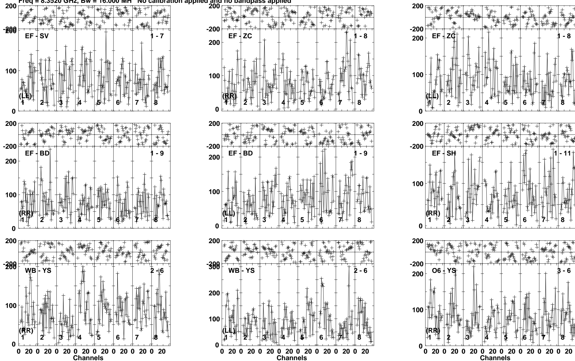
Lower frame: Micro Ampl Jy Top frame: Phas deg Vector averaged cross-power spectrum Baseline: EF (01) - SV (07) Timerange: 00/03:39:35 to 00/03:42:29
