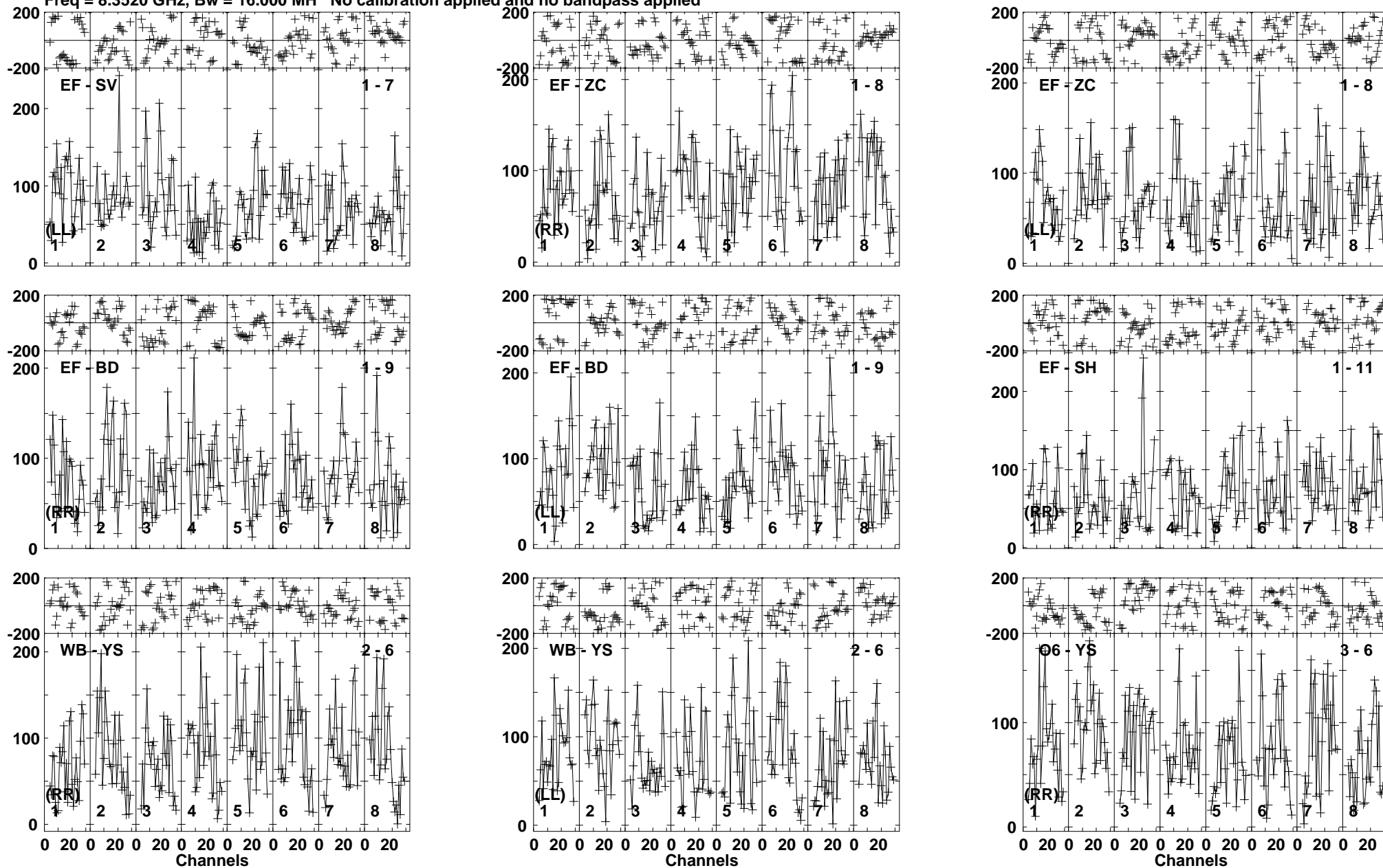
Lower frame: Micro Ampl Jy Top frame: Phas deg Vector averaged cross-power spectrum Baseline: EF (01) - SV (07) Timerange: 00/03:56:06 to 00/03:58:59
