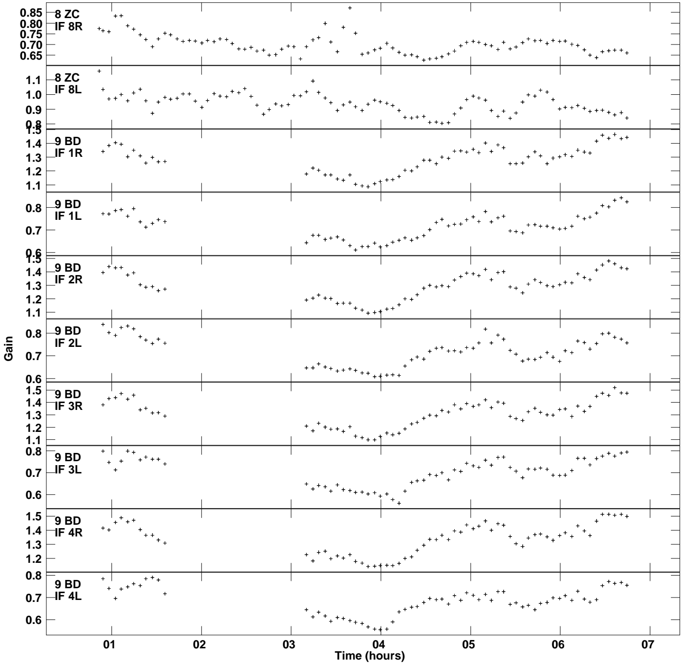
Plot file version 12 created 06-JUL-2016 18:19:28 Gain amp vs UTC time for J1128+5925.MULTI.1 SN 2 Rpol & Lpol IF 1 - 8
