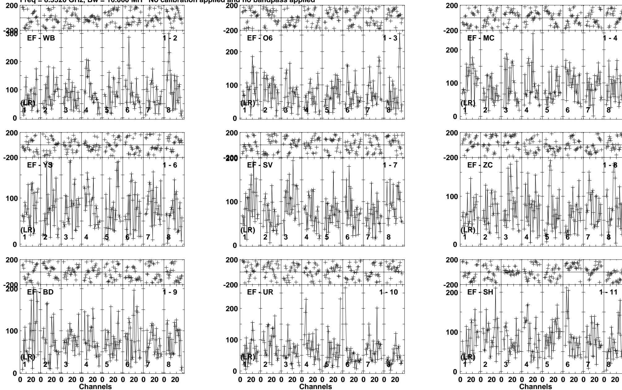
Lower frame: Micro Ampl Jy Top frame: Phas deg Vector averaged cross-power spectrum Baseline: EF (01) - WB (02) Timerange: 00/03:43:34 to 00/03:46:30
