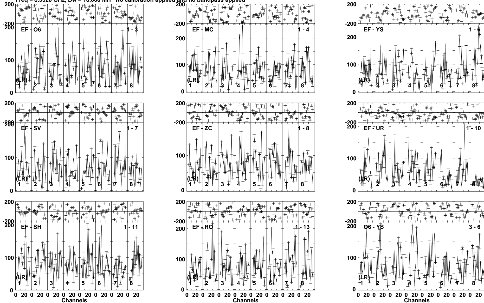
Lower frame: Micro Ampl Jy Top frame: Phas deg Vector averaged cross-power spectrum Baseline: EF (01) - O6 (03) Timerange: 00/02:00:35 to 00/02:03:30
