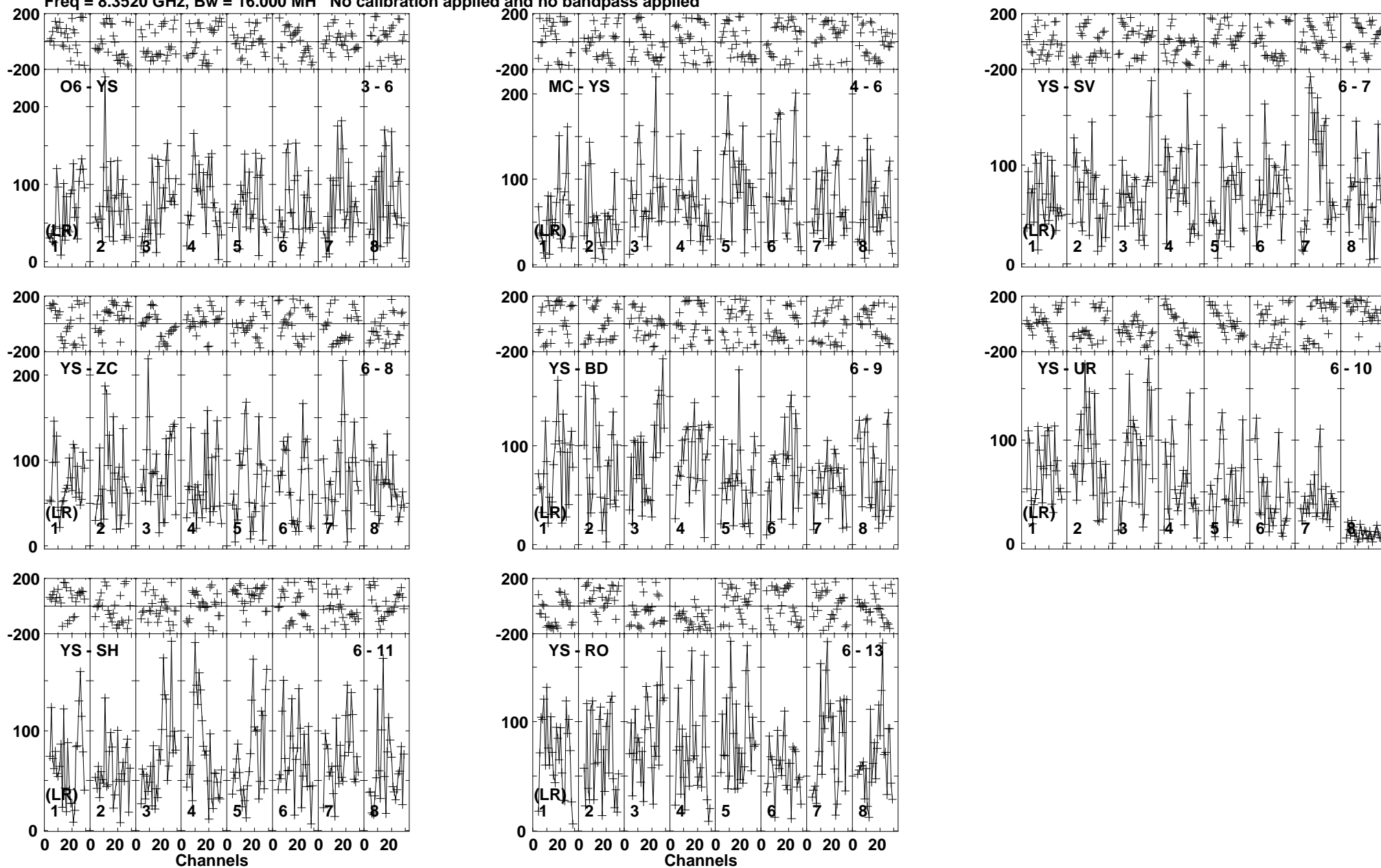
Lower frame: Micro Ampl Jy Top frame: Phas deg Vector averaged cross-power spectrum Baseline: O6 (03) - YS (06) Timerange: 00/01:19:20 to 00/01:22:14
