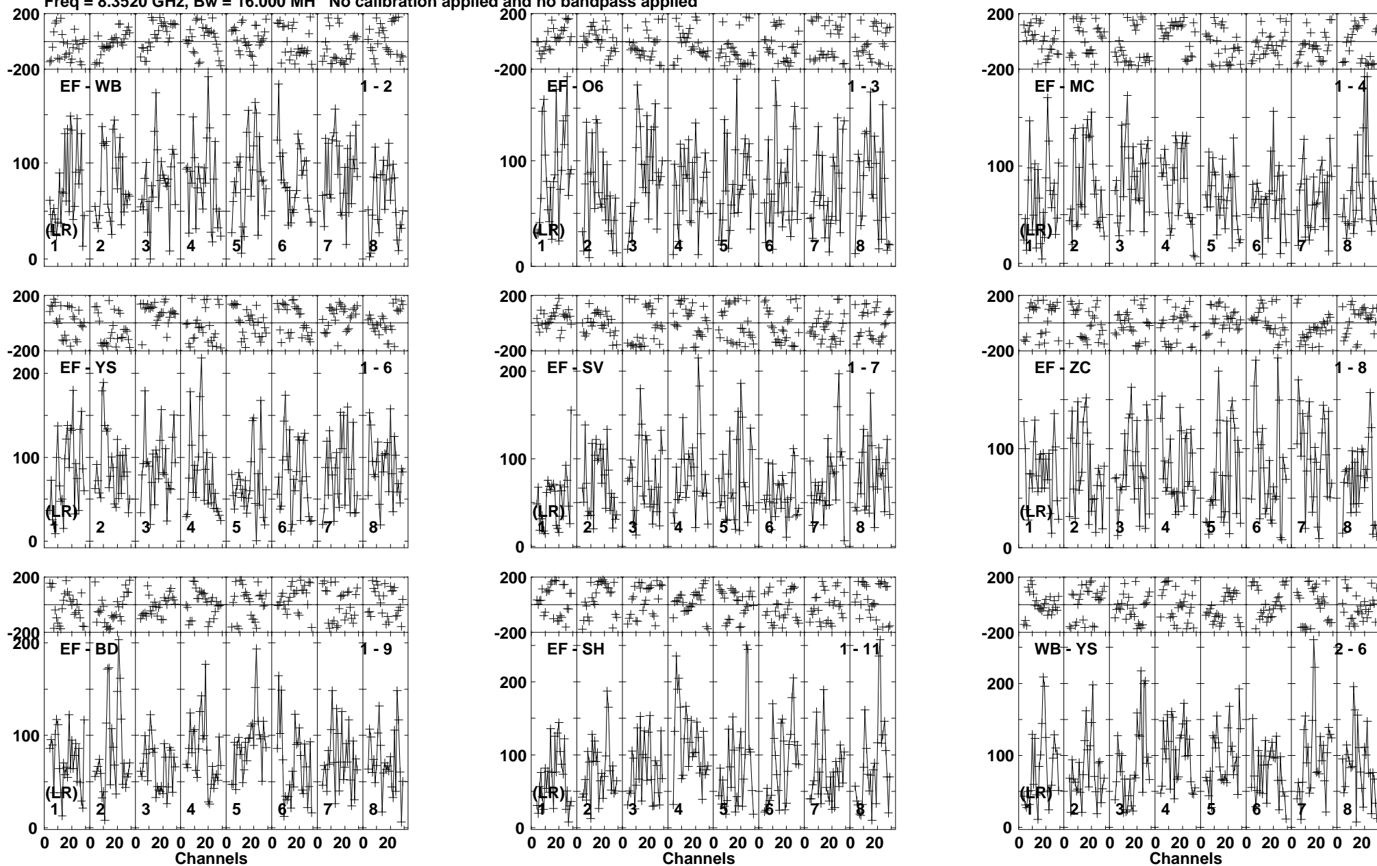
Lower frame: Micro Ampl Jy Top frame: Phas deg Vector averaged cross-power spectrum Baseline: EF (01) - WB (02) Timerange: 00/05:39:06 to 00/05:41:59
