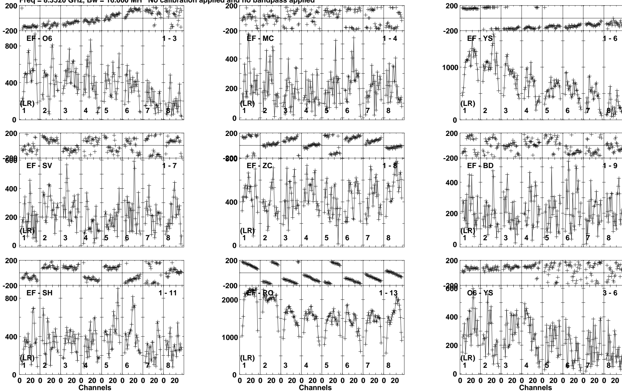
Lower frame: Micro Ampl Jy Top frame: Phas deg Vector averaged cross-power spectrum Baseline: EF (01) - O6 (03) Timerange: 00/01:05:50 to 00/01:06:44
