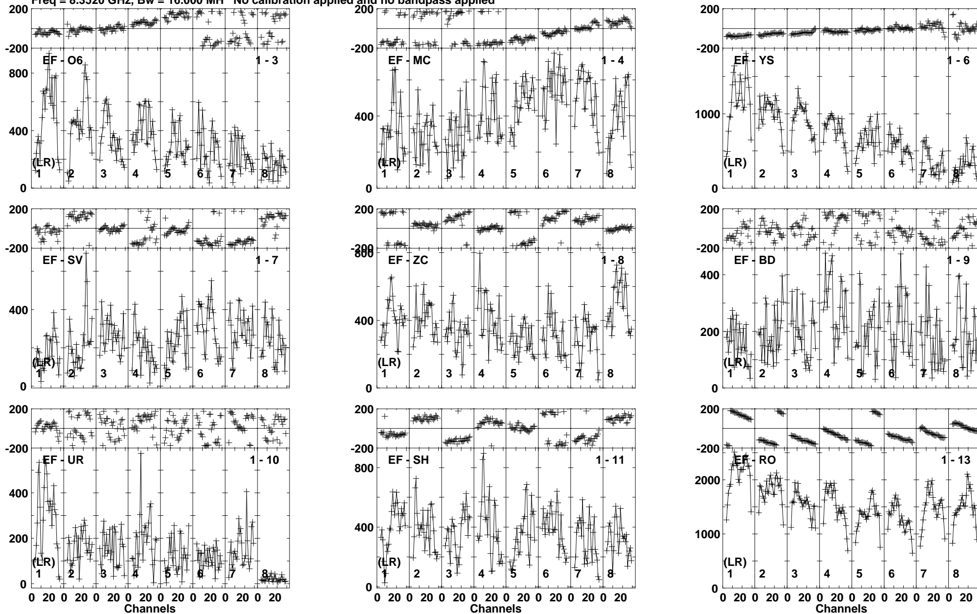
Lower frame: Micro Ampl Jy Top frame: Phas deg Vector averaged cross-power spectrum Baseline: EF (01) - O6 (03) Timerange: 00/01:18:40 to 00/01:19:15
