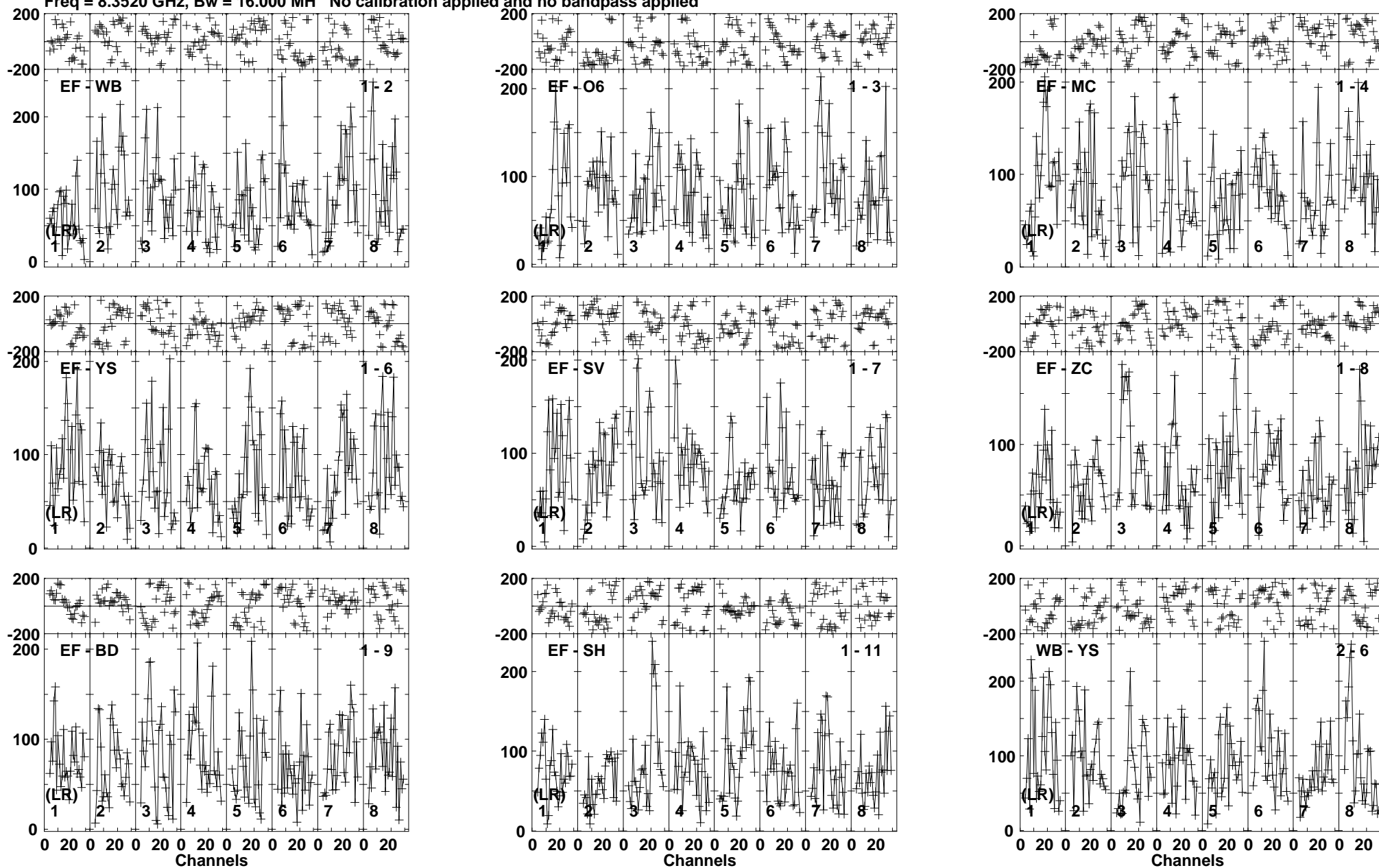
Lower frame: Micro Ampl Jy Top frame: Phas deg Vector averaged cross-power spectrum Baseline: EF (01) - WB (02) Timerange: 00/03:56:06 to 00/03:58:59
