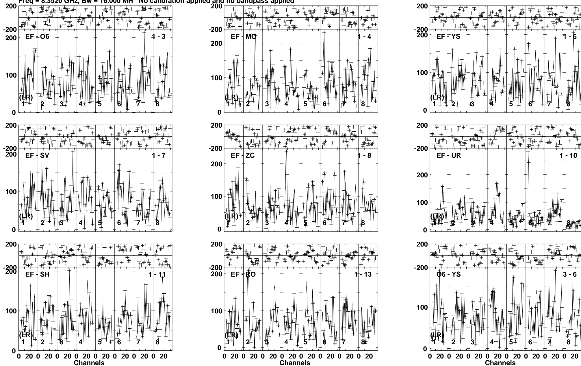
Lower frame: Micro Ampl Jy Top frame: Phas deg Vector averaged cross-power spectrum Baseline: EF (01) - O6 (03) Timerange: 00/01:39:51 to 00/01:42:45
