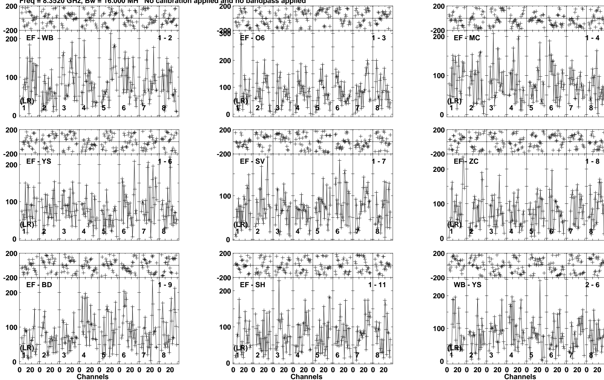
Lower frame: Micro Ampl Jy Top frame: Phas deg Vector averaged cross-power spectrum Baseline: EF (01) - WB (02) Timerange: 00/04:12:36 to 00/04:15:30
