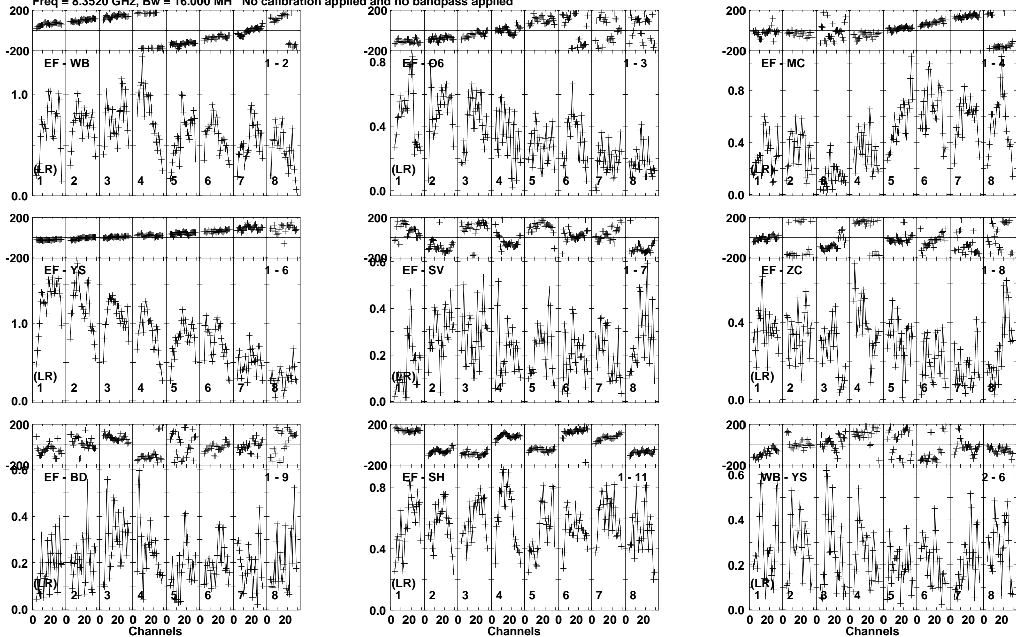
Lower frame: Milli Ampl Jy Top frame: Phas deg Vector averaged cross-power spectrum Baseline: EF (01) - WB (02) Timerange: 00/04:20:11 to 00/04:20:45
