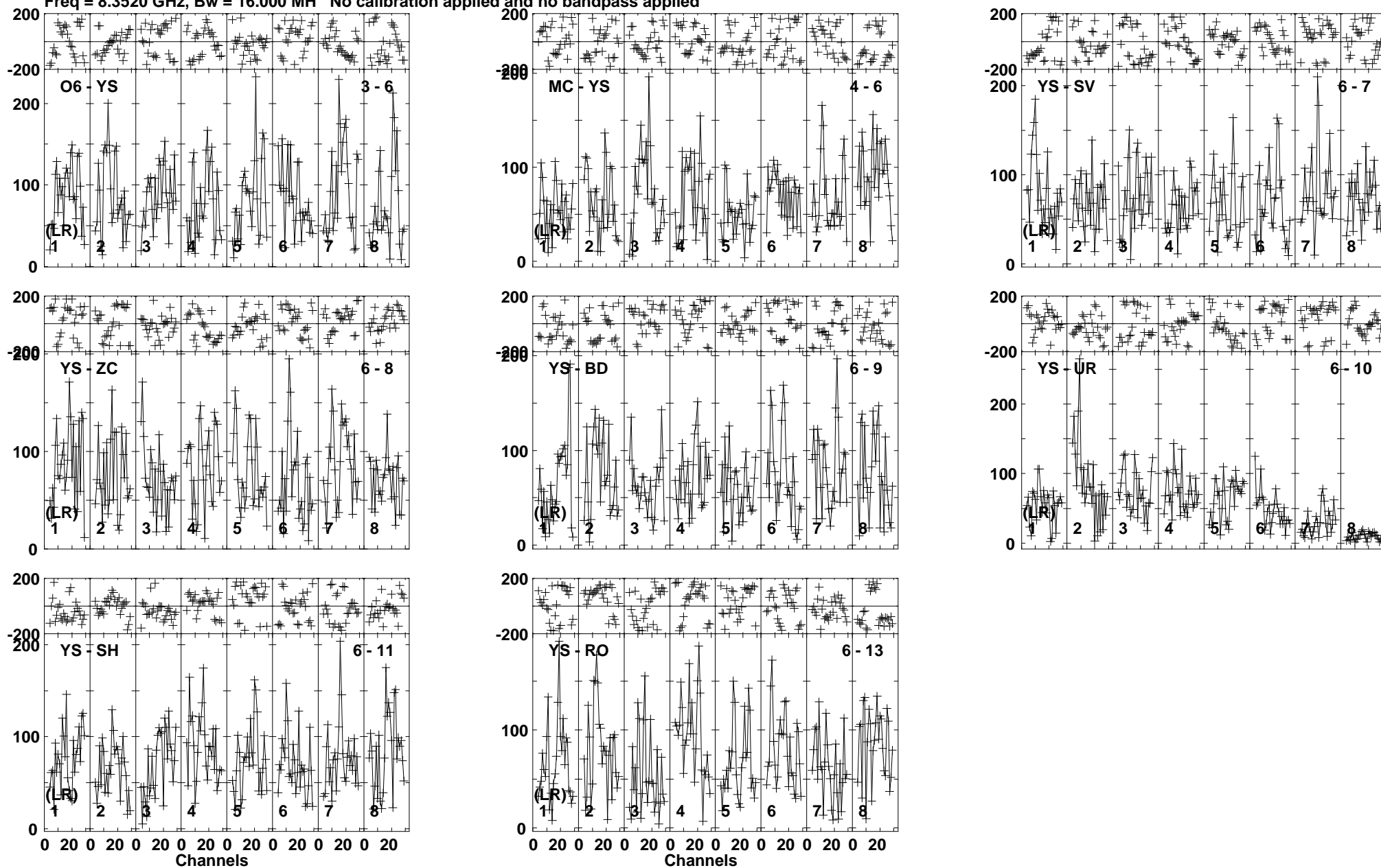
Lower frame: Micro Ampl Jy Top frame: Phas deg Vector averaged cross-power spectrum Baseline: O6 (03) - YS (06) Timerange: 00/01:15:05 to 00/01:17:59
