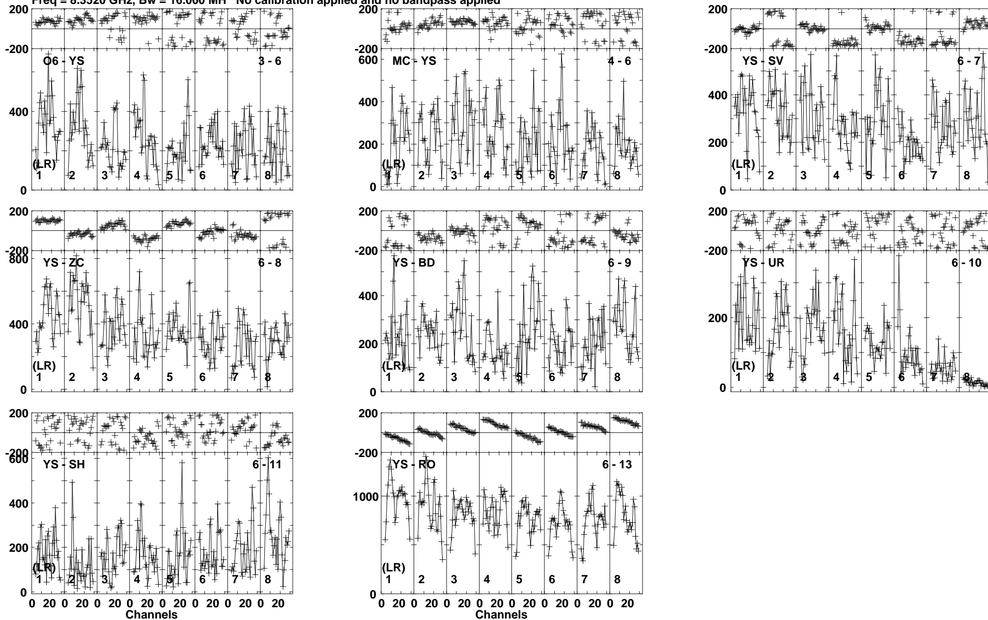
Lower frame: Micro Ampl Jy Top frame: Phas deg Vector averaged cross-power spectrum Baseline: O6 (03) - YS (06) Timerange: 00/01:26:56 to 00/01:27:30
