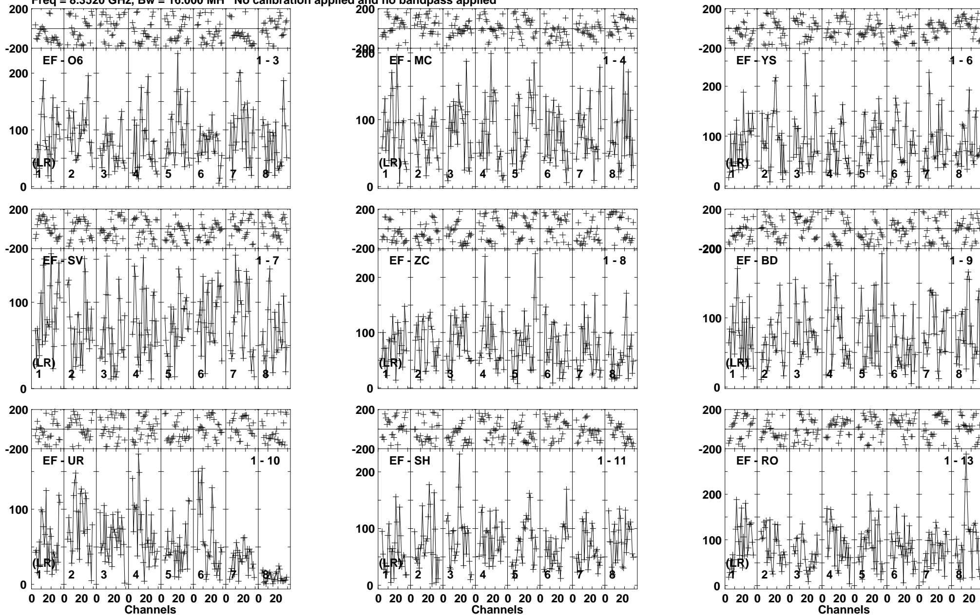
Lower frame: Micro Ampl Jy Top frame: Phas deg Vector averaged cross-power spectrum Baseline: EF (01) - O6 (03) Timerange: 00/01:19:20 to 00/01:22:14
