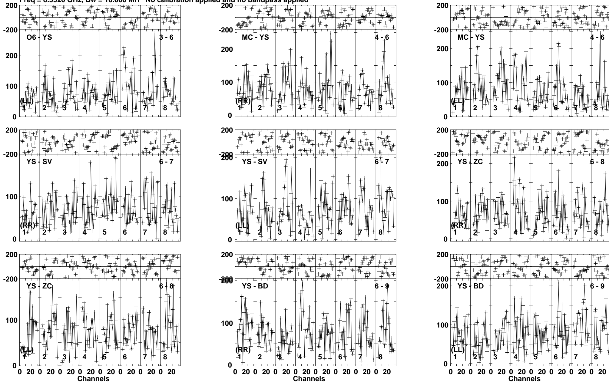
Lower frame: Micro Ampl Jy Top frame: Phas deg Vector average cross-power spectrum Baseline: O6 (03) - YS (06) Timerange: 00/05:55:32 to 00/05:58:30
