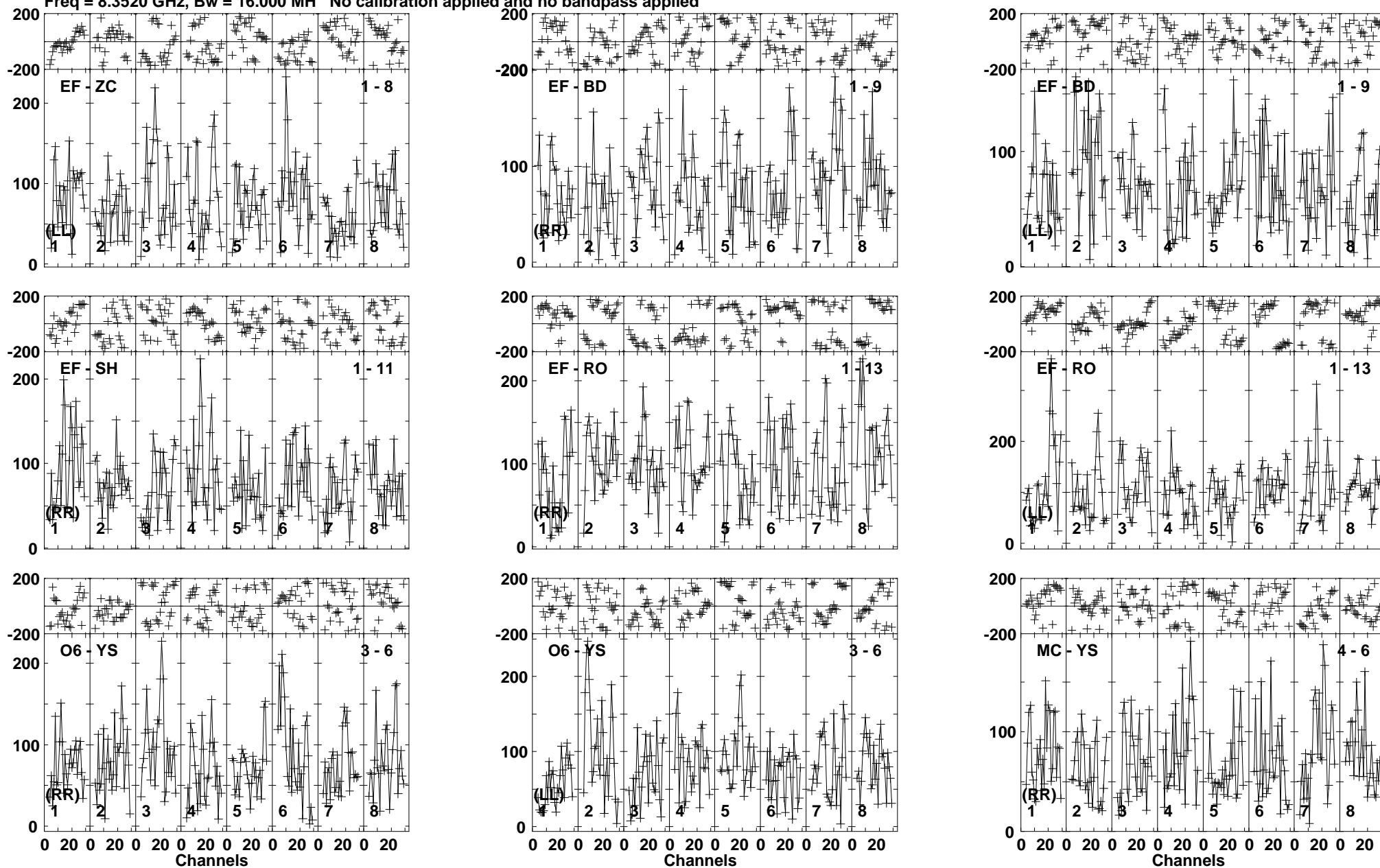
Lower frame: Micro Ampl Jy Top frame: Phas deg Vector averaged cross-power spectrum Baseline: EF (01) - ZC (08) Timerange: 00/00:54:36 to 00/00:57:30
