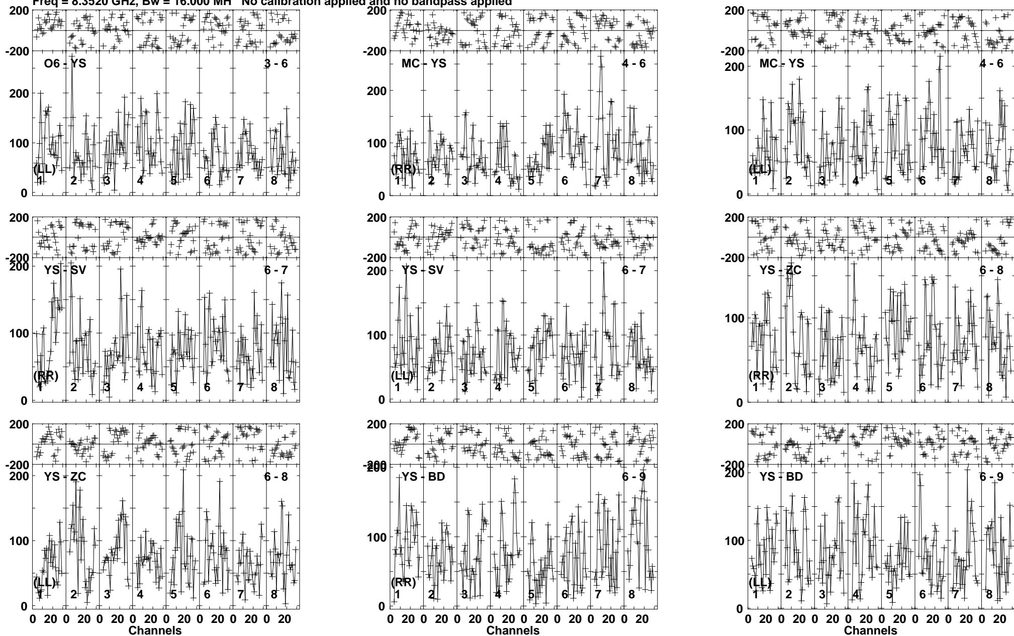
Lower frame: Micro Ampl Jy Top frame: Phas deg Vector averaged cross-power spectrum Baseline: O6 (03) - YS (06) Timerange: 00/04:16:35 to 00/04:19:29
