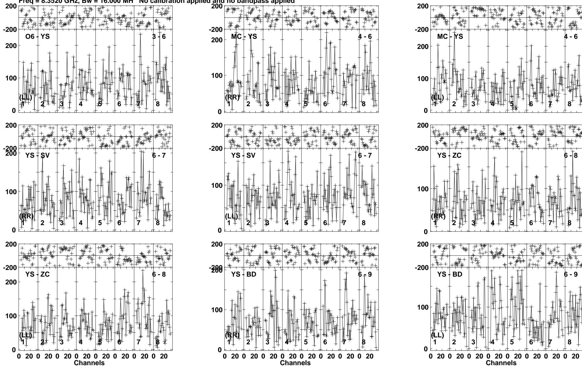
Lower frame: Micro Ampl Jy Top frame: Phas deg Vector averaged cross-power spectrum Baseline: O6 (03) - YS (06) Timerange: 00/04:45:35 to 00/04:48:29
