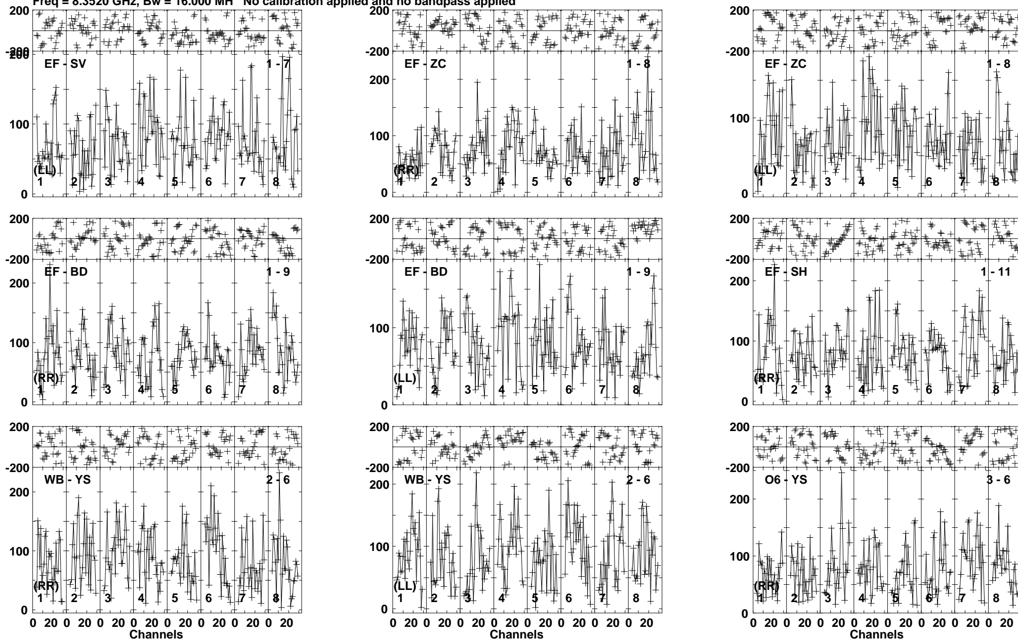
Lower frame: Micro Ampl Jy Top frame: Phas deg Vector averaged cross-power spectrum Baseline: EF (01) - SV (07) Timerange: 00/05:35:06 to 00/05:37:59
