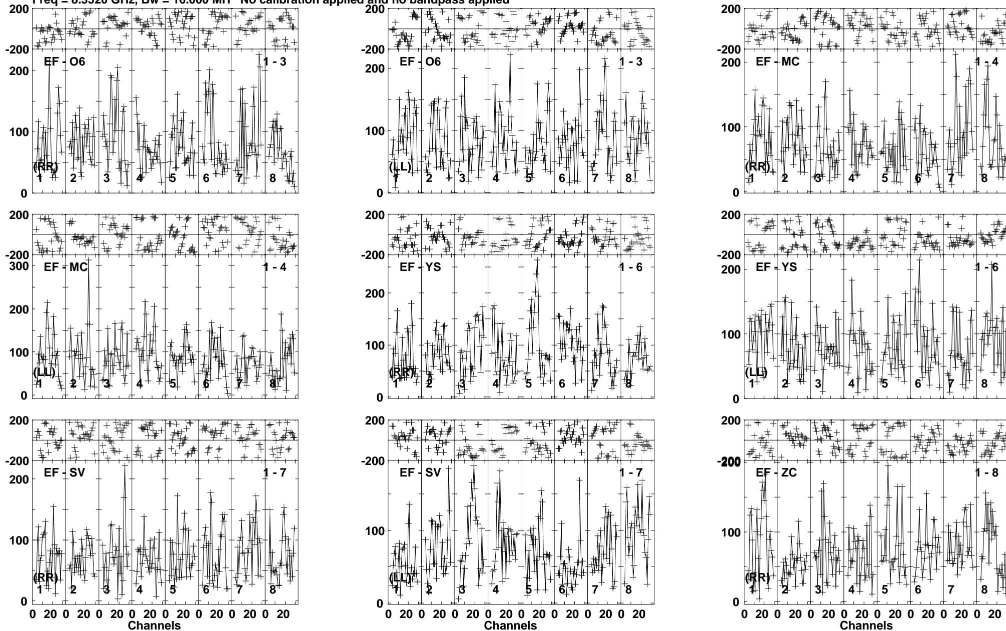
Lower frame: Micro Ampl Jy Top frame: Phas deg Vector averaged cross-power spectrum Baseline: EF (01) - O6 (03) Timerange: 00/02:12:50 to 00/02:15:44
