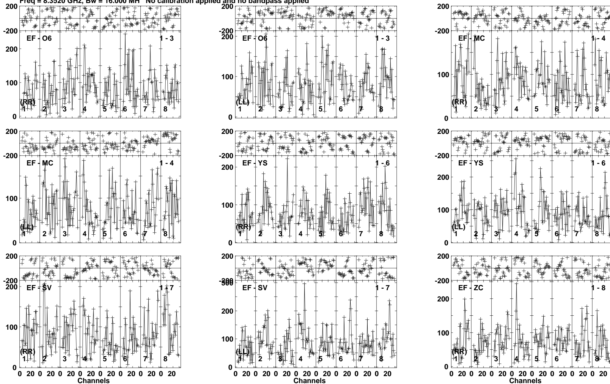
Lower frame: Micro Ampl Jy Top frame: Phas deg Vector averaged cross-power spectrum Baseline: EF (01) - O6 (03) Timerange: 00/01:27:35 to 00/01:30:30
