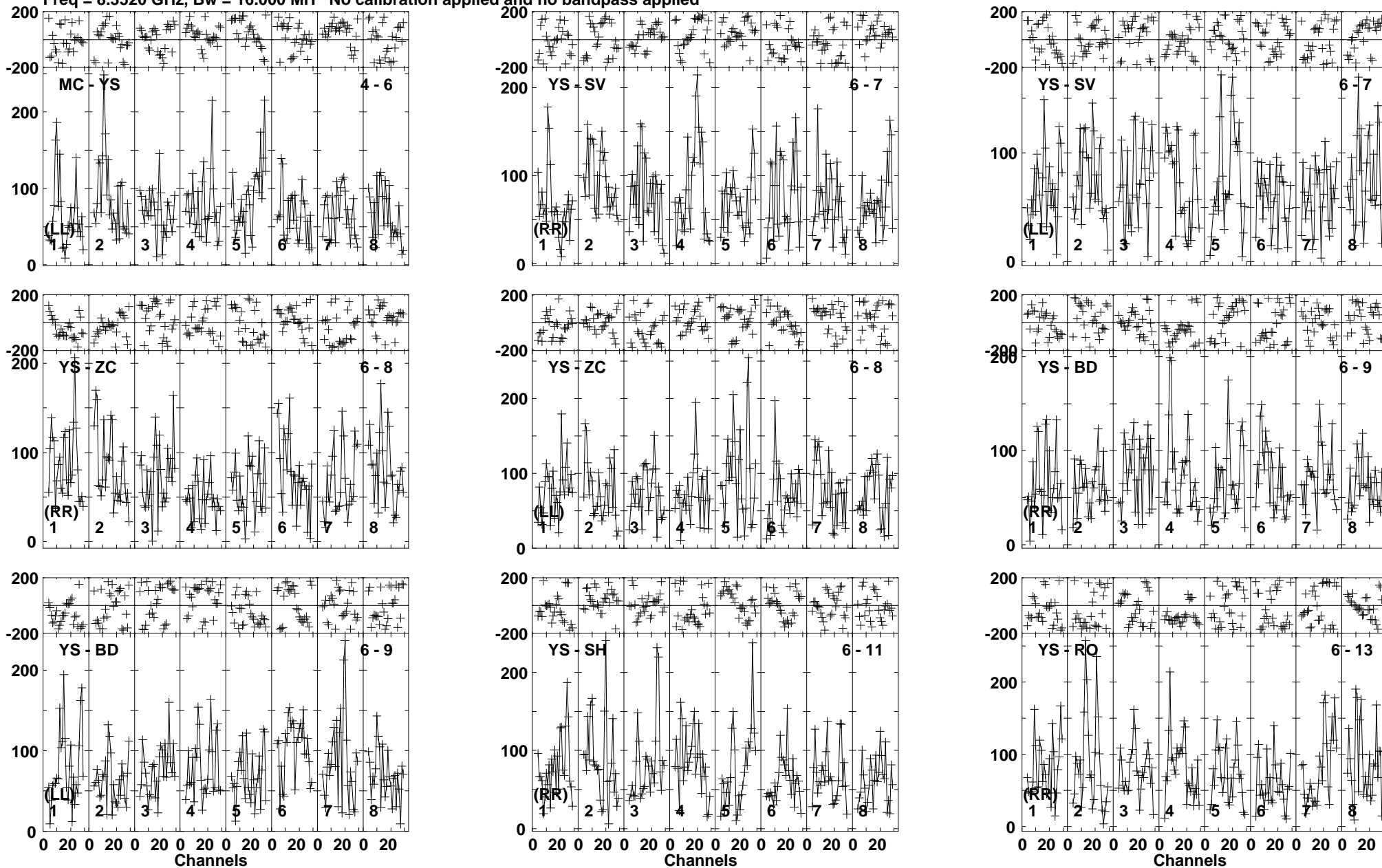
Lower frame: Micro Ampl Jy Top frame: Phas deg Vector averaged cross-power spectrum Baseline: MC (04) - YS (06) Timerange: 00/00:58:35 to 00/01:01:29
