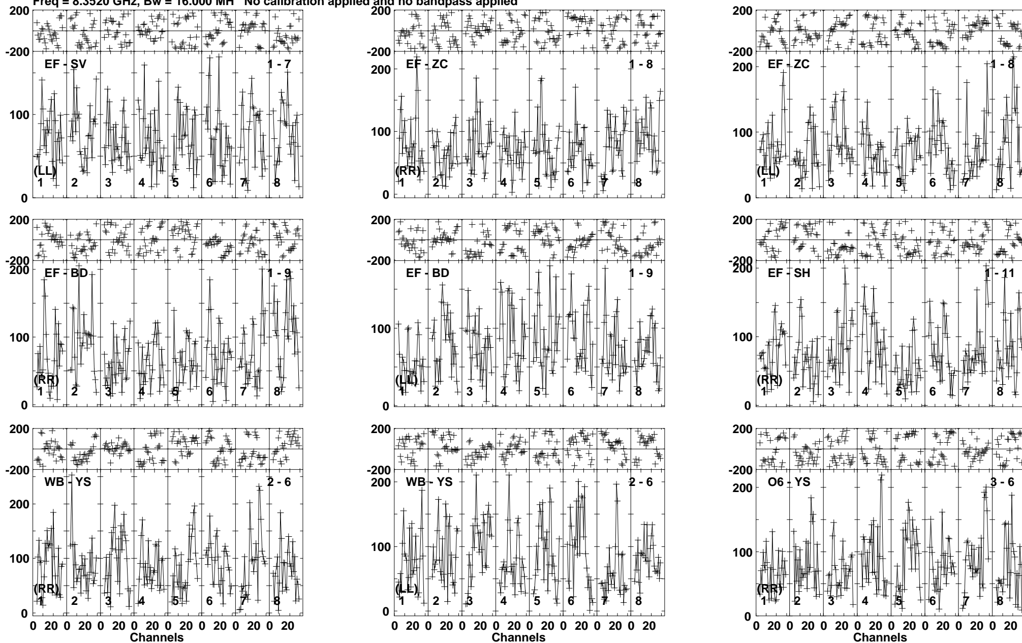
Lower frame: Micro Ampl Jy Top frame: Phas deg Vector averaged cross-power spectrum Baseline: EF (01) - SV (07) Timerange: 00/04:16:35 to 00/04:19:29
