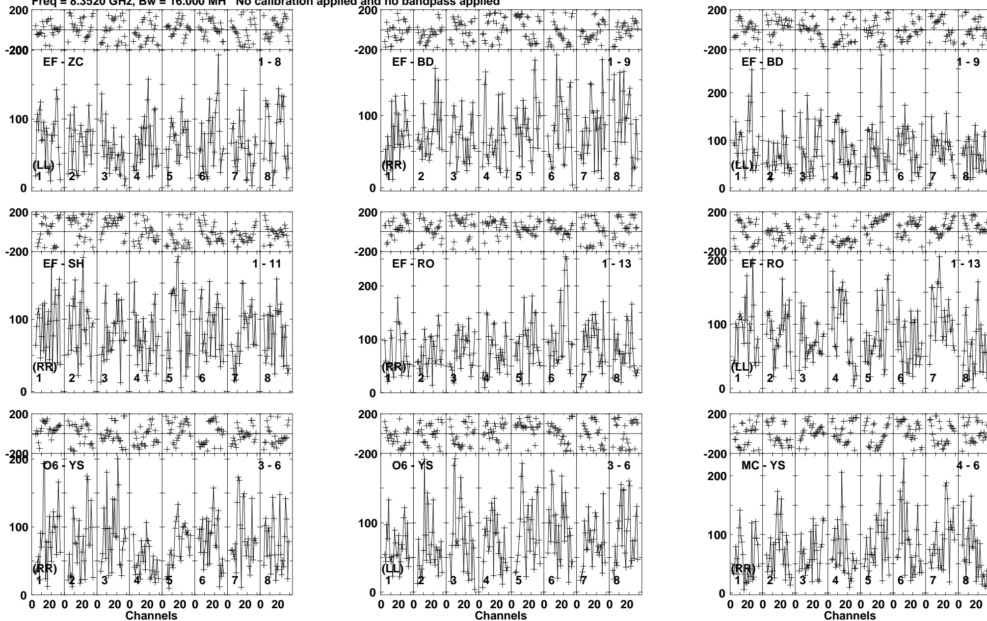
Lower frame: Micro Ampl Jy Top frame: Phas deg Vector averaged cross-power spectrum Baseline: EF (01) - ZC (08) Timerange: 00/01:06:50 to 00/01:09:45
