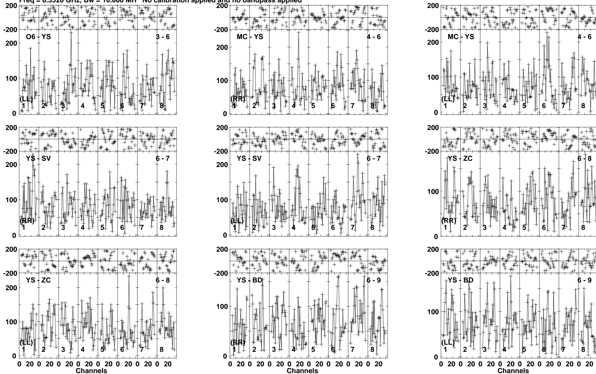
Lower frame: Micro Ampl Jy Top frame: Phas deg Vector averaged cross-power spectrum Baseline: O6 (03) - YS (06) Timerange: 00/04:33:06 to 00/04:36:00
