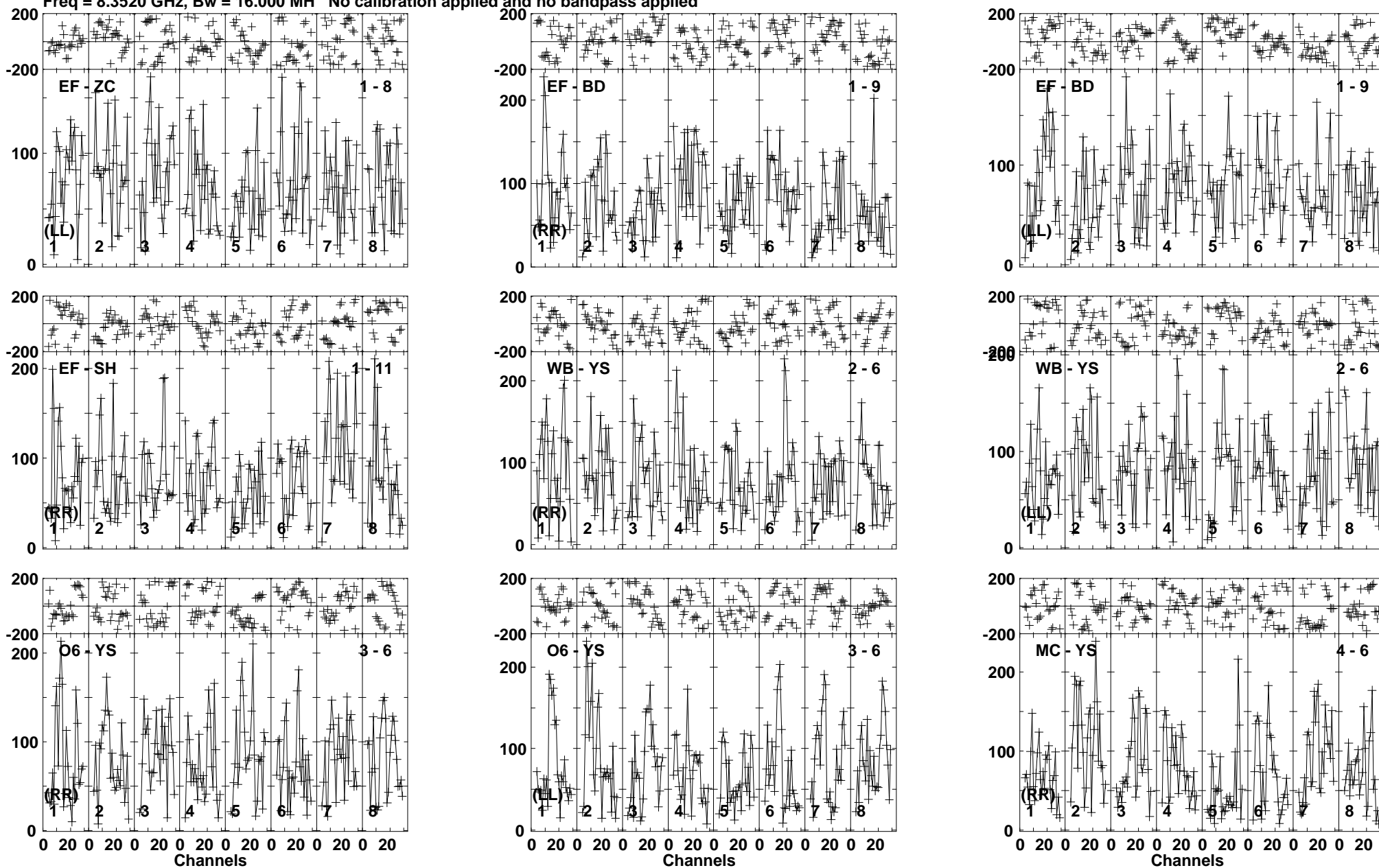
Lower frame: Micro Ampl Jy Top frame: Phas deg Vector averaged cross-power spectrum Baseline: EF (01) - ZC (08) Timerange: 00/06:12:05 to 00/06:15:00
