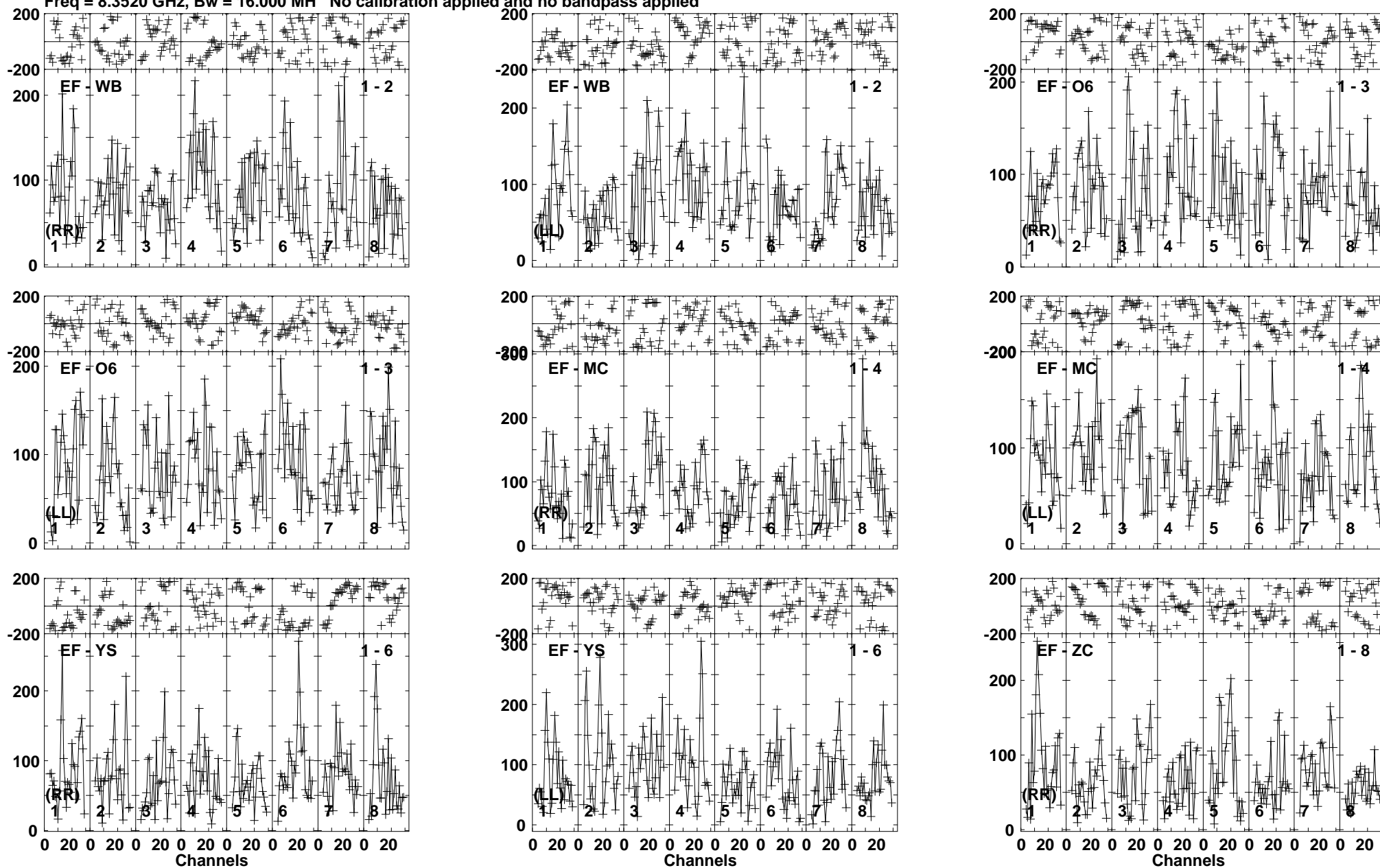
Lower frame: Micro Ampl Jy Top frame: Phas deg Vector averaged cross-power spectrum Baseline: EF (01) - WB (02) Timerange: 00/05:59:51 to 00/06:02:44
