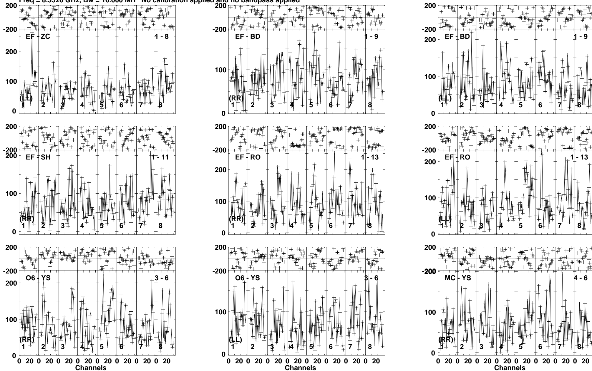
Lower frame: Micro Ampl Jy Top frame: Phas deg Vector averaged cross-power spectrum Baseline: EF (01) - ZC (08) Timerange: 00/01:11:05 to 00/01:13:59
