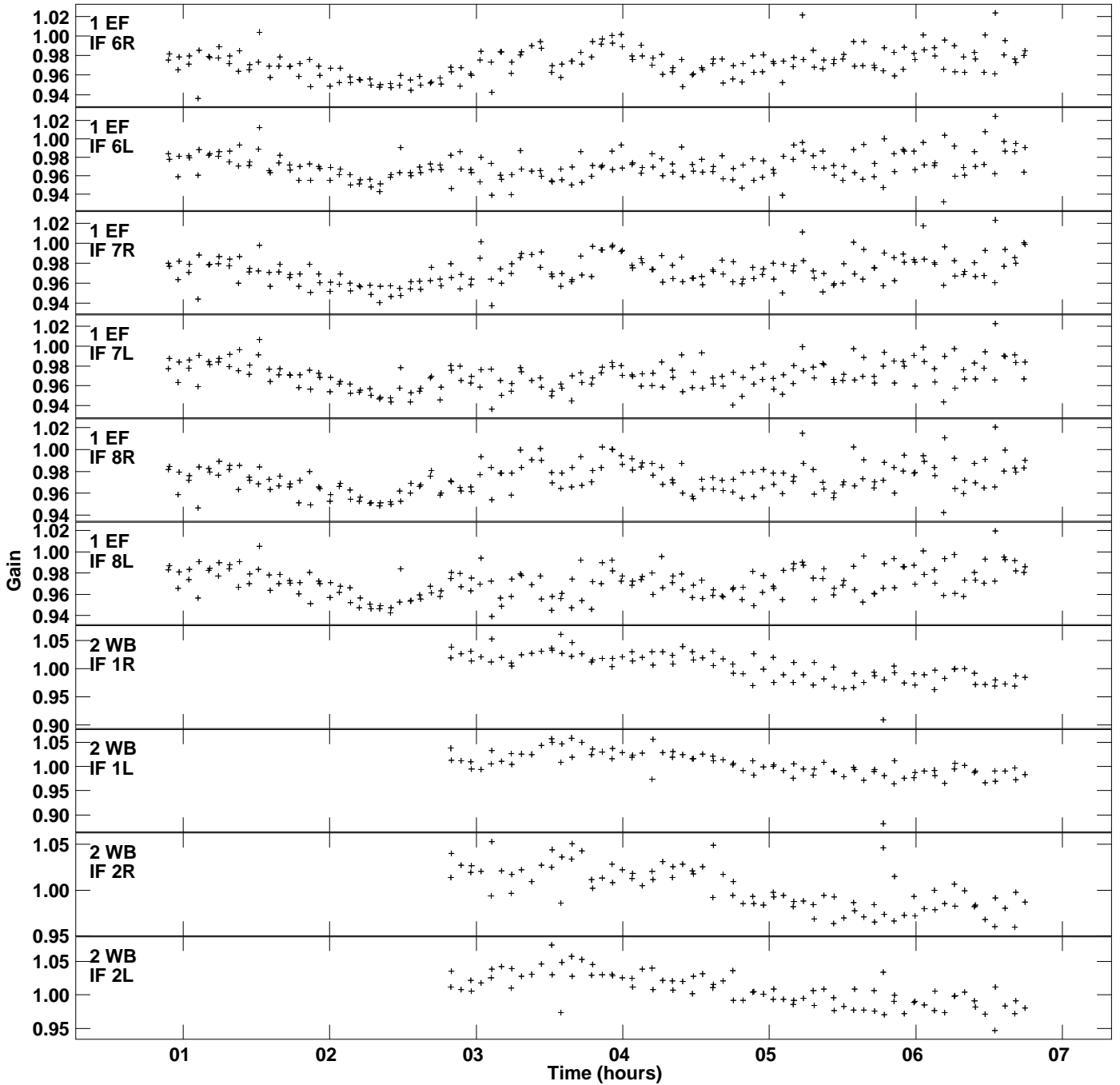
Plot file version 2 created 06-JUL-2016 18:51:17 Gain amp vs UTC time for J1128+5925.MULTI.1 SN 4 Rpol & Lpol IF 1 - 8
