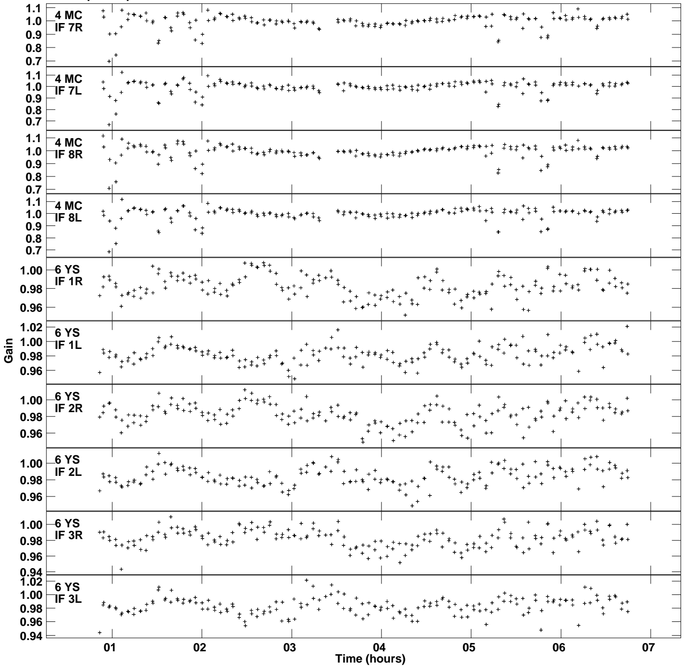
Plot file version 7 created 06-JUL-2016 18:51:17 Gain amp vs UTC time for J1128+5925.MULTI.1 SN 4 Rpol & Lpol IF 1 - 8
