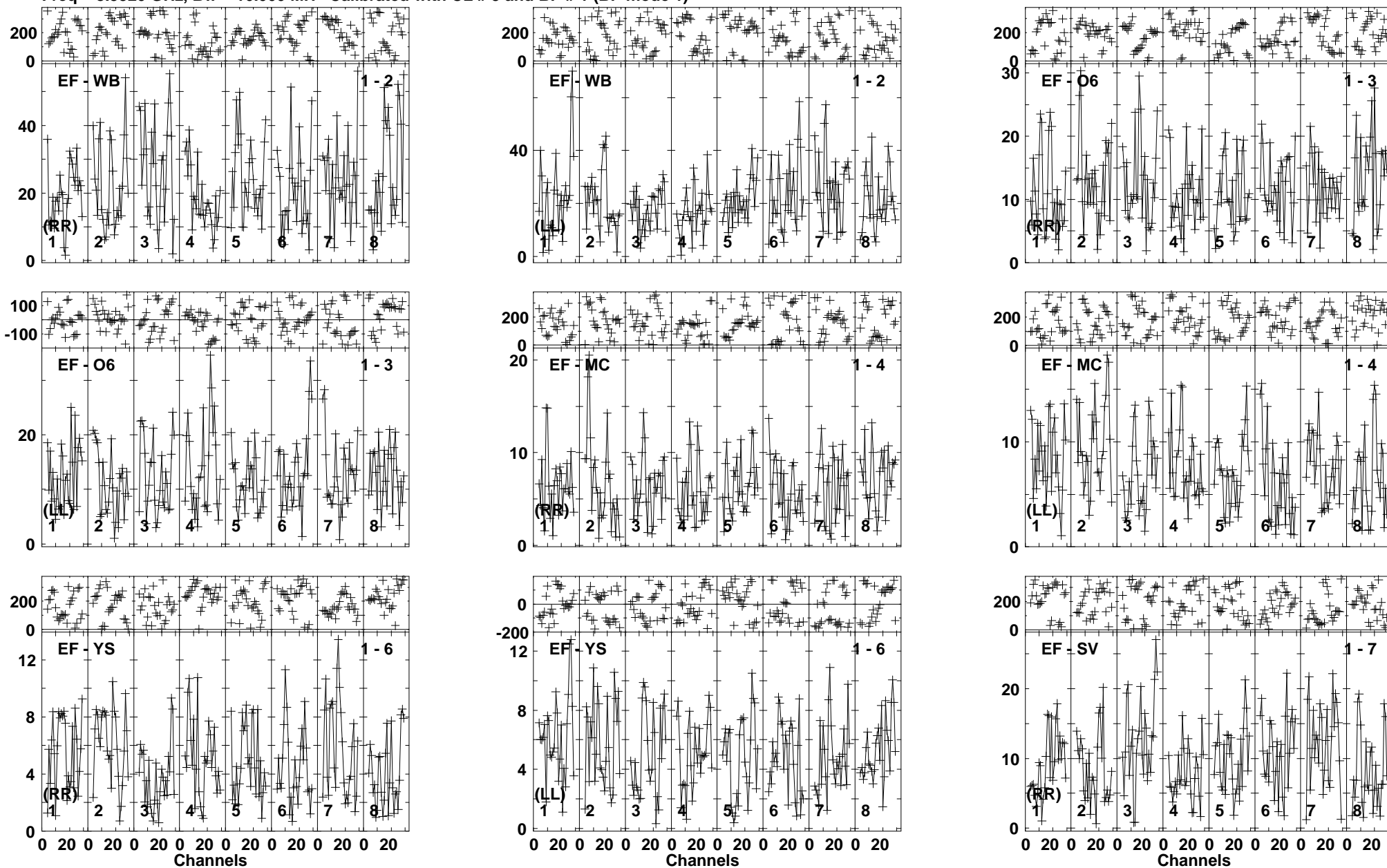
Lower frame: Milli Ampl Jy Top frame: Phas deg Vector averaged cross-power spectrum Baseline: EF (01) - WB (02) Timerange: 00/03:18:50 to 00/03:21:44
