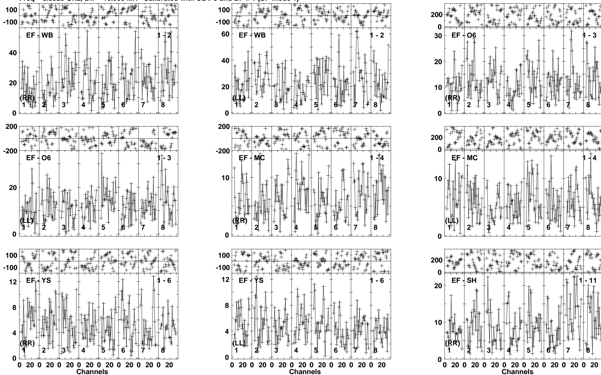
Lower frame: Milli Ampl Jy Top frame: Phas deg Vector averaged cross-power spectrum Baseline: EF (01) - WB (02) Timerange: 00/06:36:50 to 00/06:39:45
