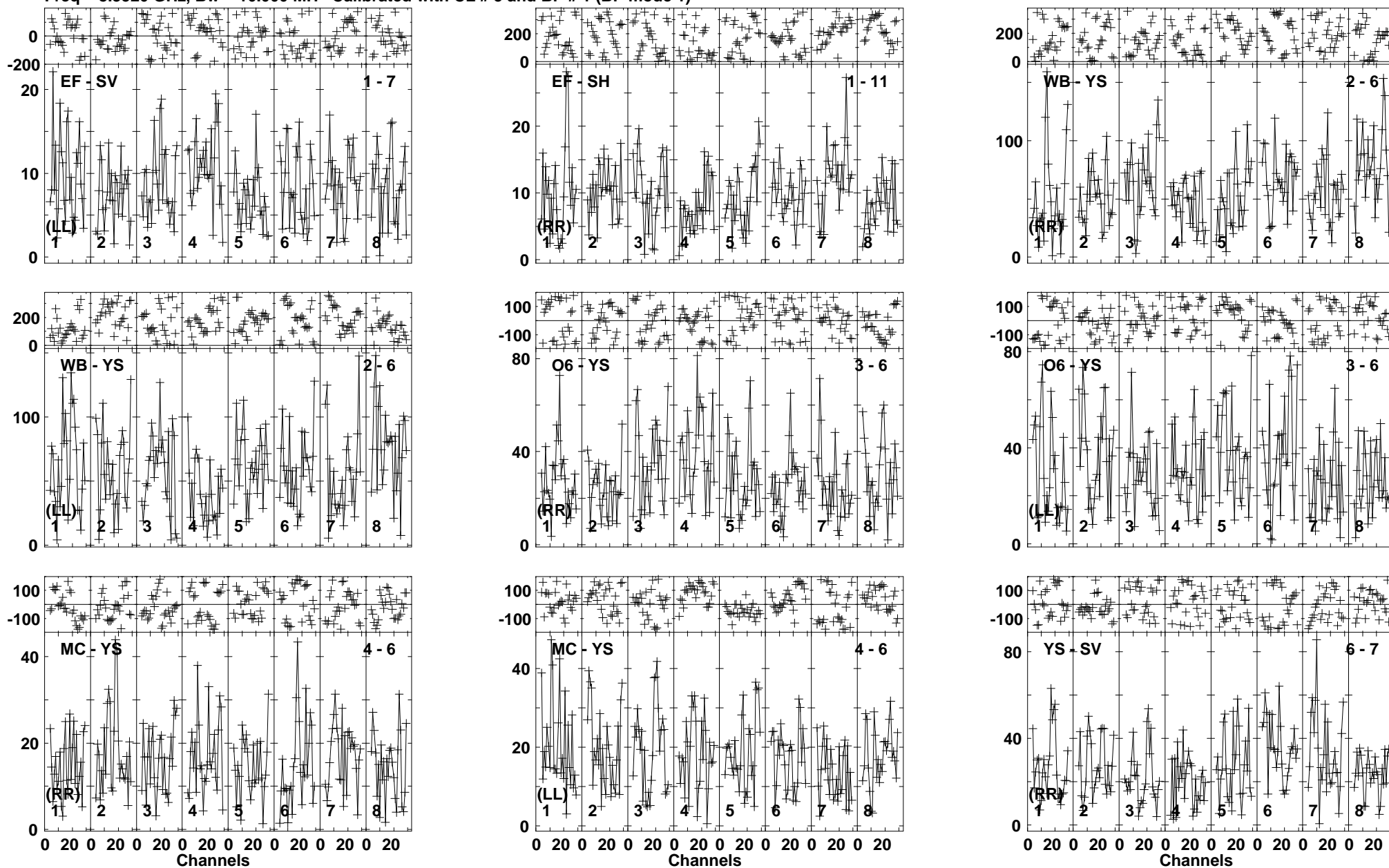
Lower frame: Milli Ampl Jy Top frame: Phas deg Vector averaged cross-power spectrum Baseline: EF (01) - SV (07) Timerange: 00/04:08:21 to 00/04:11:14
