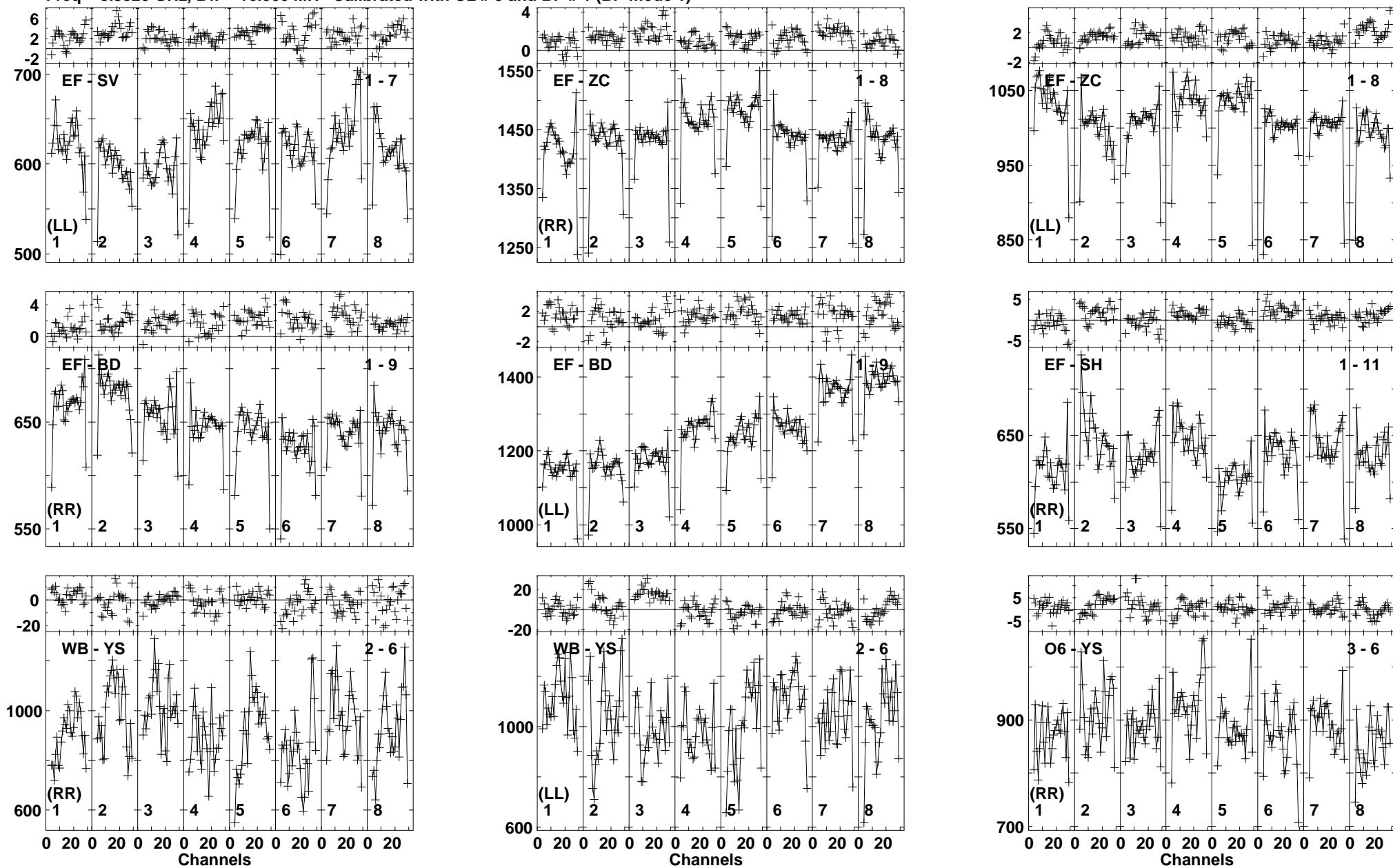
Lower frame: Milli Ampl Jy Top frame: Phas deg Vector averaged cross-power spectrum Baseline: EF (01) - SV (07) Timerange: 00/03:50:49 to 00/03:51:44
