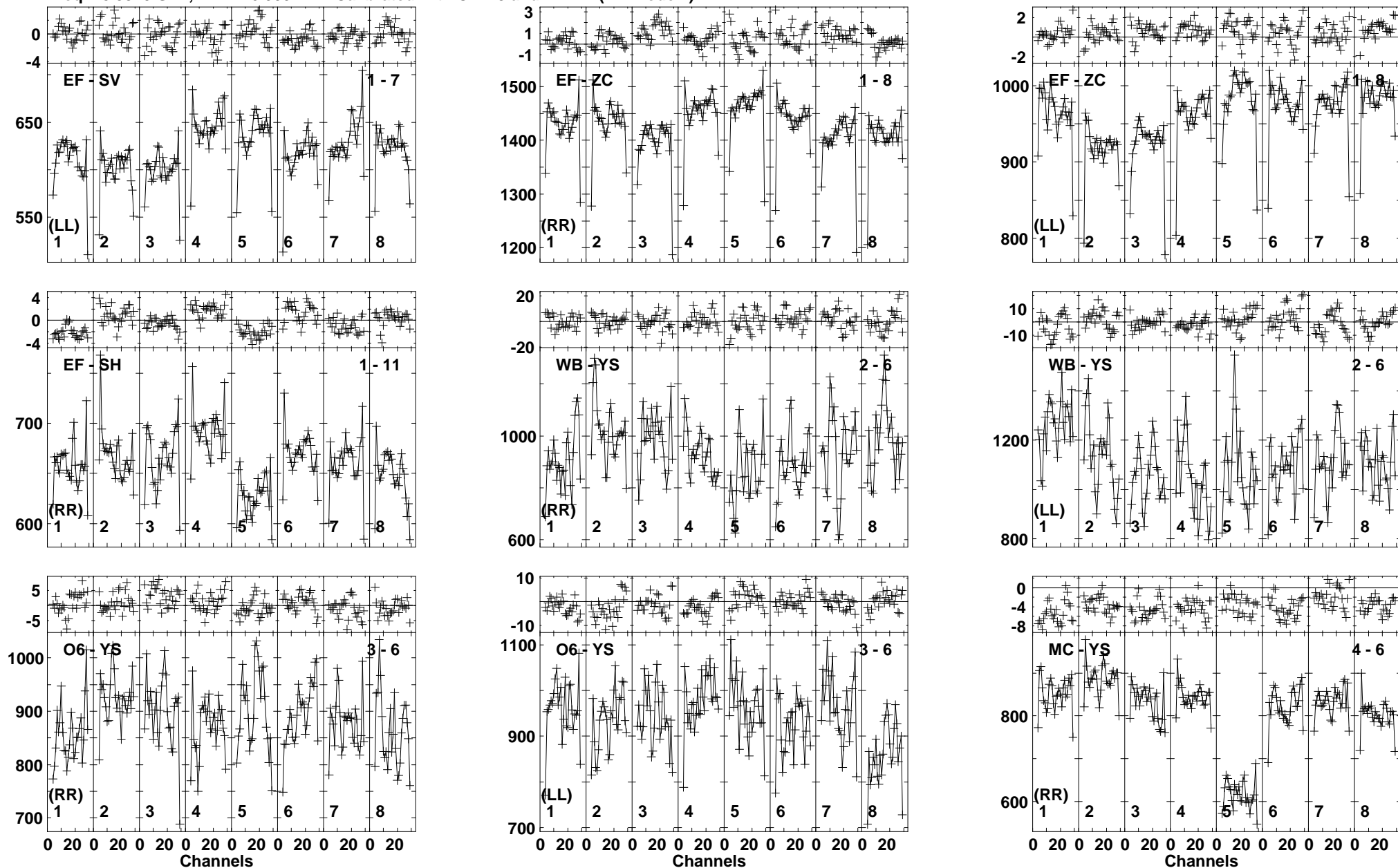
Lower frame: Milli Ampl Jy Top frame: Phas deg Vector averaged cross-power spectrum Baseline: EF (01) - SV (07) Timerange: 00/02:49:26 to 00/02:50:00
