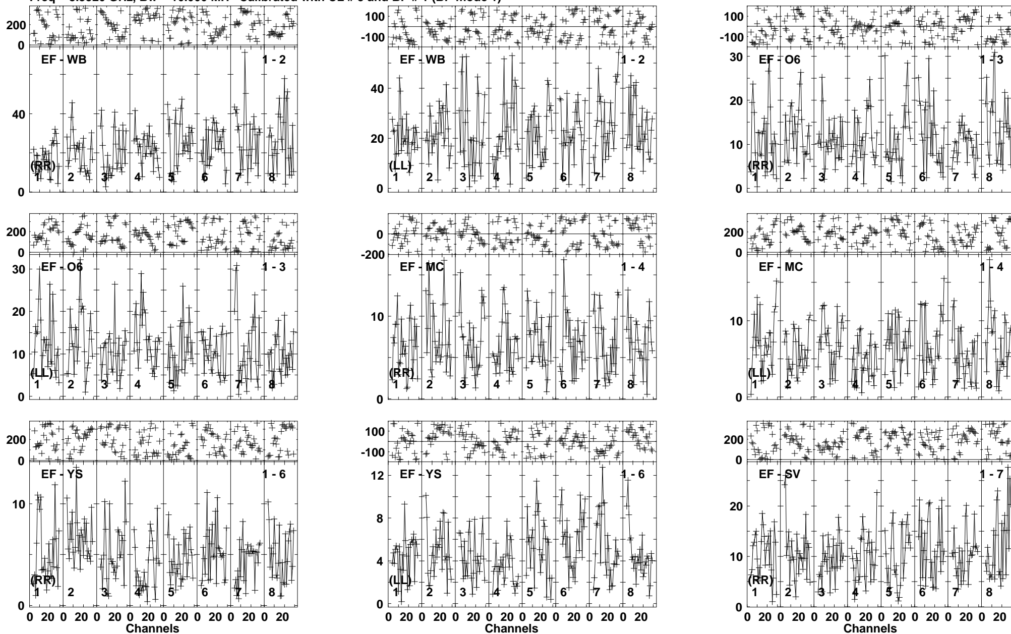
Lower frame: Milli Ampl Jy Top frame: Phas deg Vector averaged cross-power spectrum Baseline: EF (01) - WB (02) Timerange: 00/05:47:20 to 00/05:50:15
