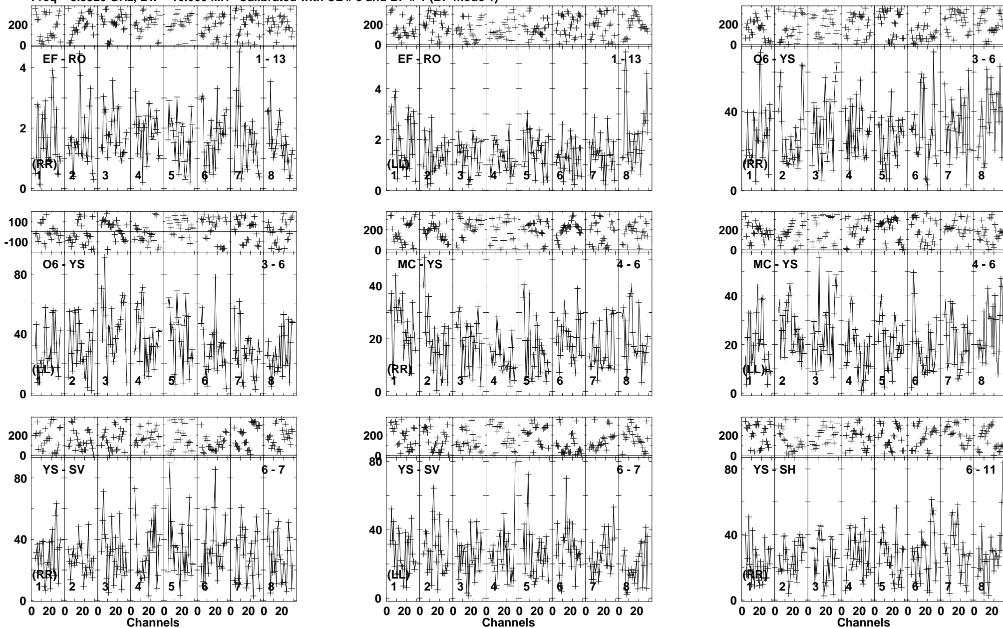
Lower frame: Milli Ampl Jy Top frame: Phas deg Vector averaged cross-power spectrum Baseline: EF (01) - RO (13) Timerange: 00/02:00:35 to 00/02:03:30
