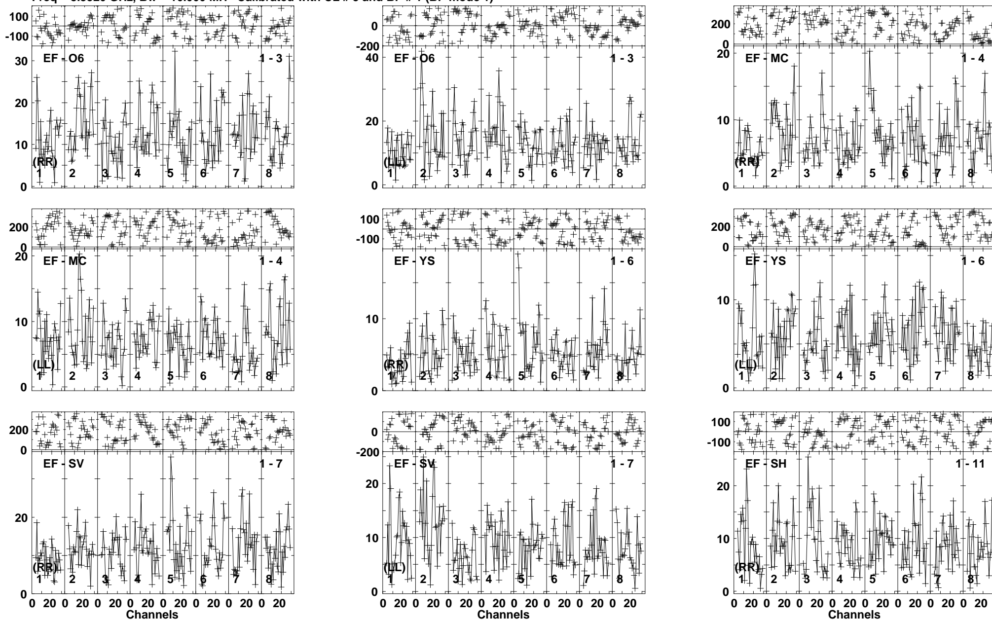
Lower frame: Milli Ampl Jy Top frame: Phas deg Vector averaged cross-power spectrum Baseline: EF (01) - O6 (03) Timerange: 00/01:56:21 to 00/01:59:15
