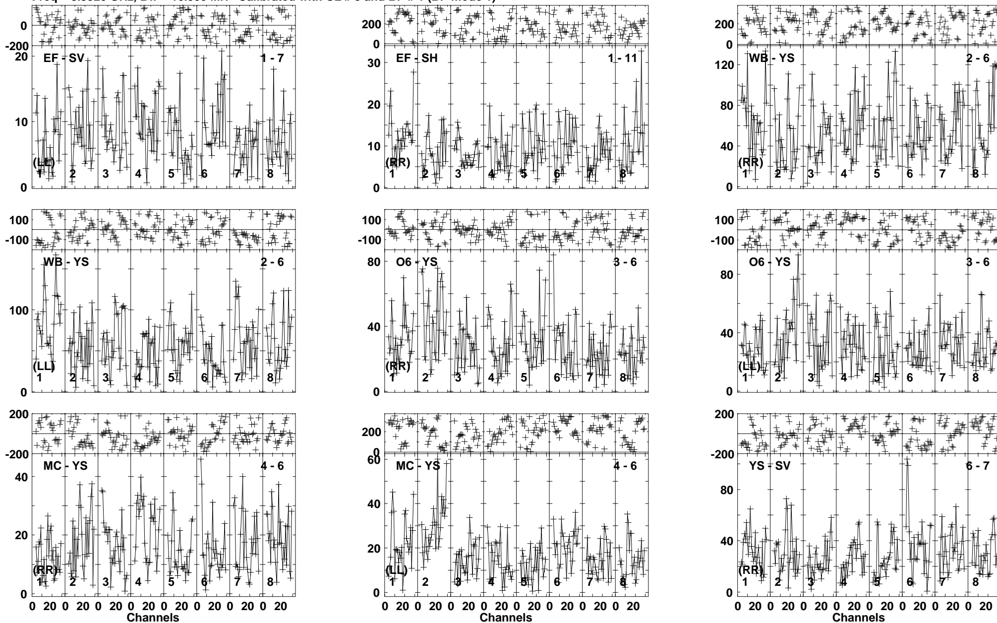
Lower frame: Milli Ampl Jy Top frame: Phas deg Vector averaged cross-power spectrum Baseline: EF (01) - SV (07) Timerange: 00/04:04:20 to 00/04:07:15
