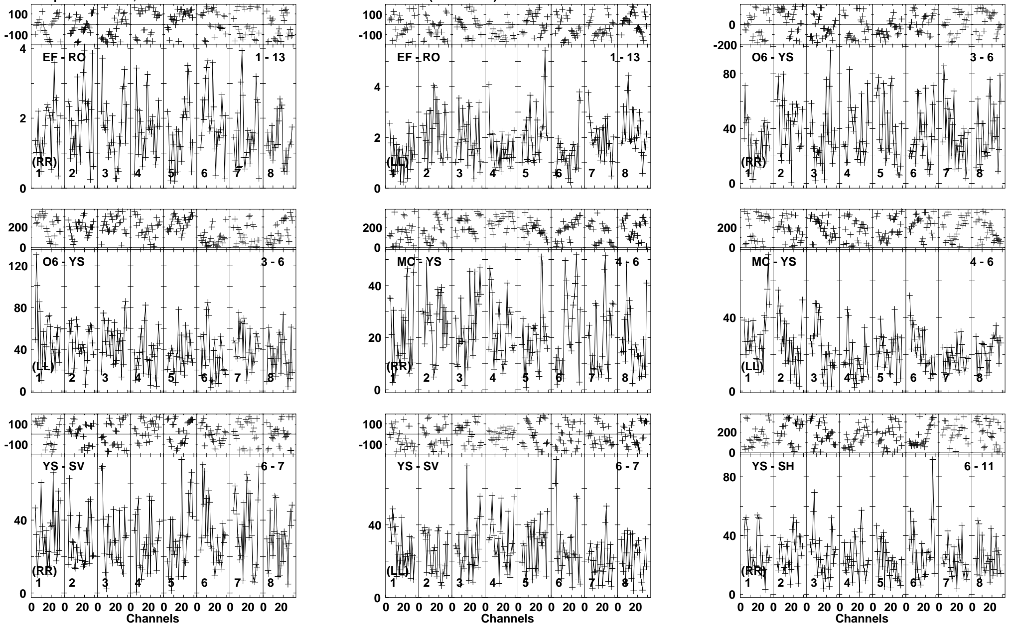
Lower frame: Milli Ampl Jy Top frame: Phas deg Vector averaged cross-power spectrum Baseline: EF (01) - RO (13) Timerange: 00/01:06:50 to 00/01:09:45
