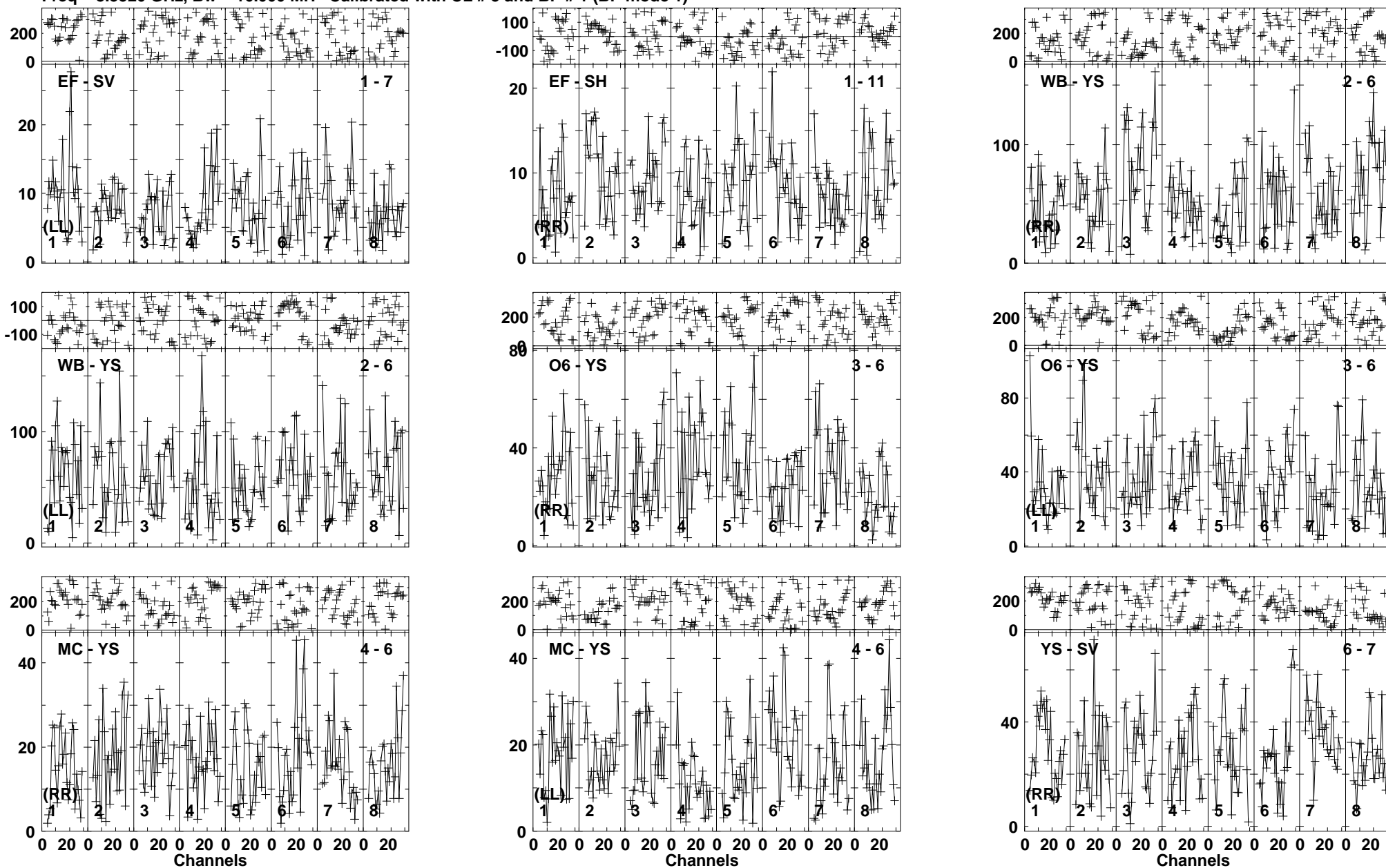
Lower frame: Milli Ampl Jy Top frame: Phas deg Vector averaged cross-power spectrum Baseline: EF (01) - SV (07) Timerange: 00/04:24:50 to 00/04:27:45
