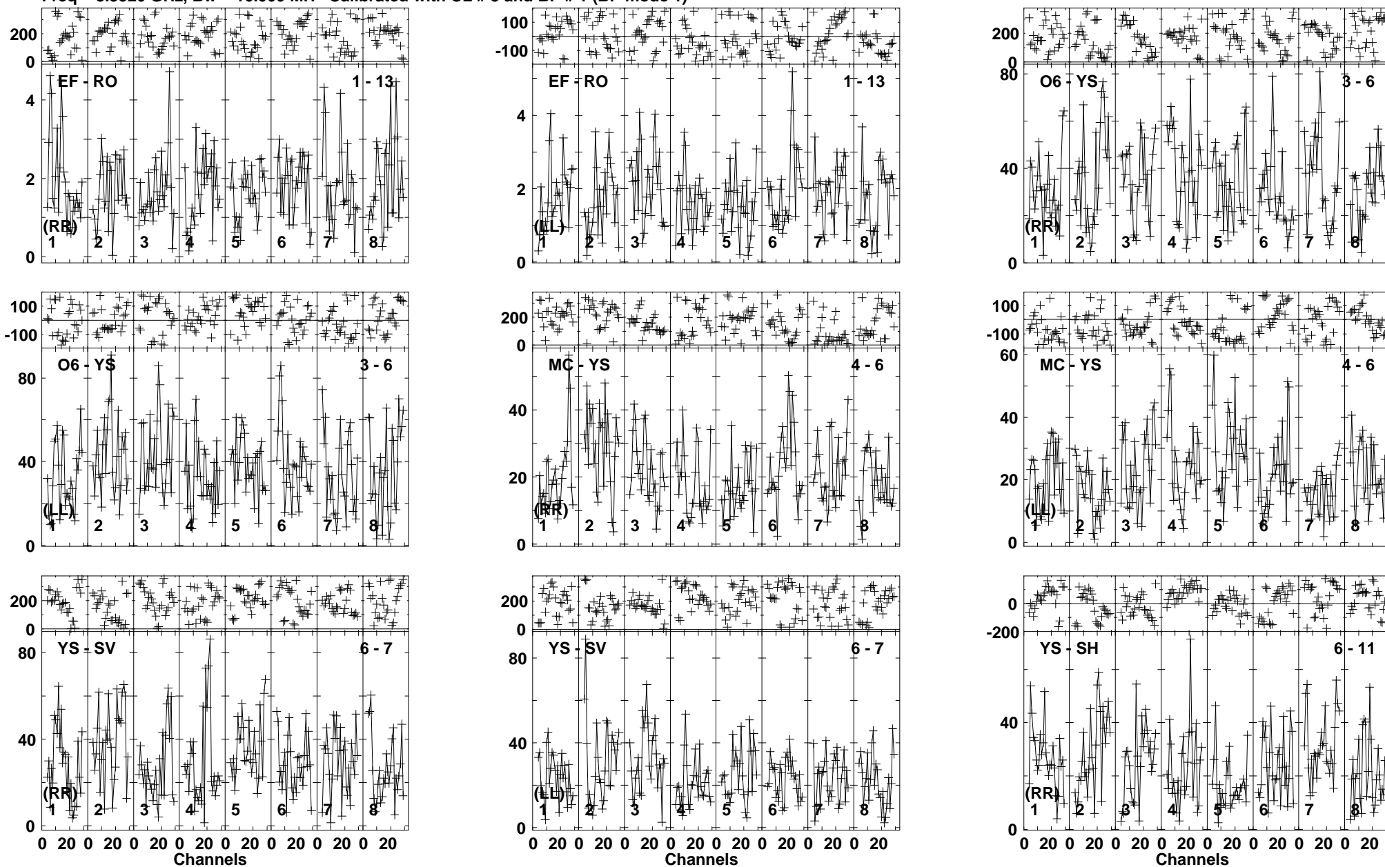
Lower frame: Milli Ampl Jy Top frame: Phas deg Vector averaged cross-power spectrum Baseline: EF (01) - RO (13) Timerange: 00/01:27:35 to 00/01:30:30
