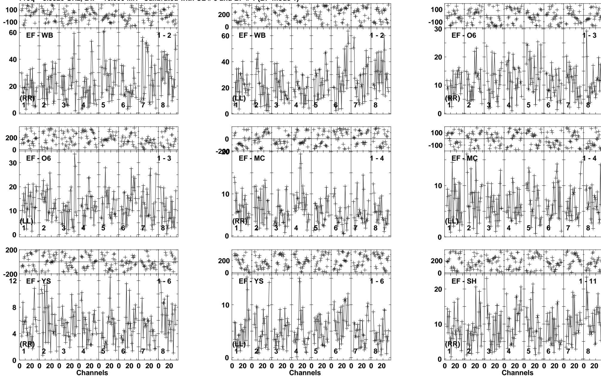
Lower frame: Milli Ampl Jy Top frame: Phas deg Vector averaged cross-power spectrum Baseline: EF (01) - WB (02) Timerange: 00/06:24:35 to 00/06:27:29
