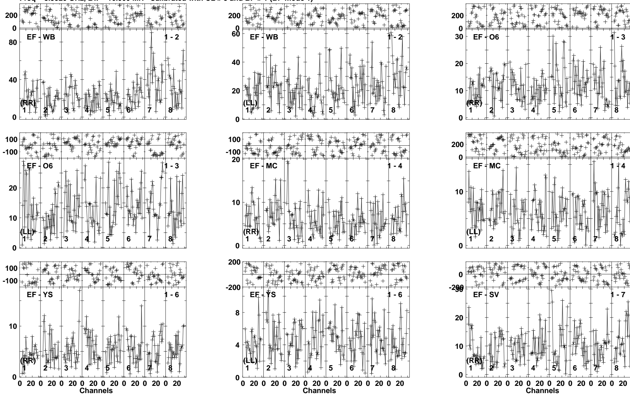
Lower frame: Milli Ampl Jy Top frame: Phas deg Vector averaged cross-power spectrum Baseline: EF (01) - WB (02) Timerange: 00/05:18:36 to 00/05:21:29
