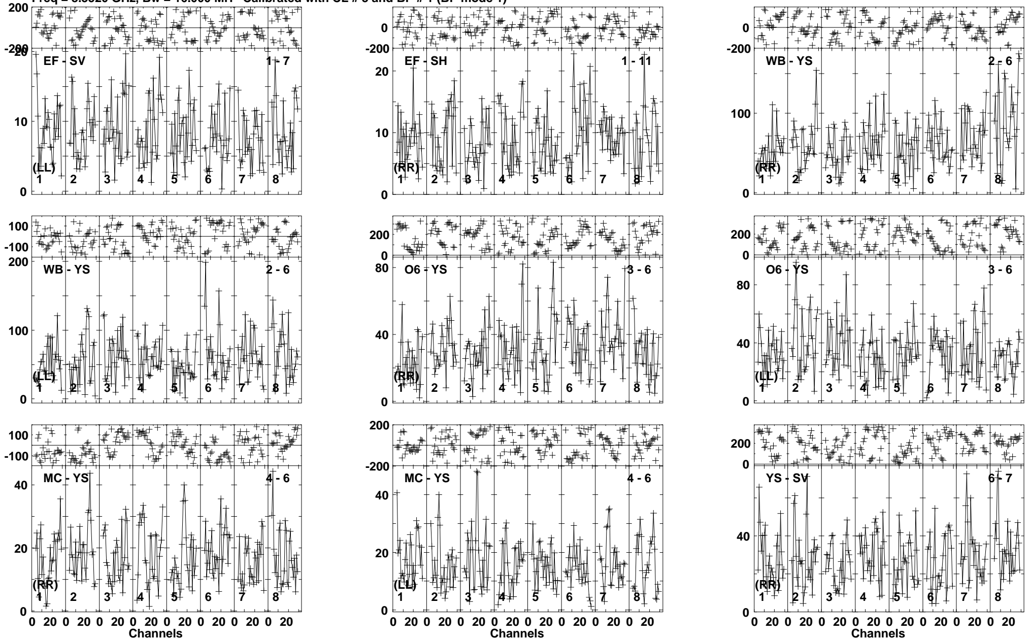
Lower frame: Milli Ampl Jy Top frame: Phas deg Vector averaged cross-power spectrum Baseline: EF (01) - SV (07) Timerange: 00/05:47:20 to 00/05:50:15
