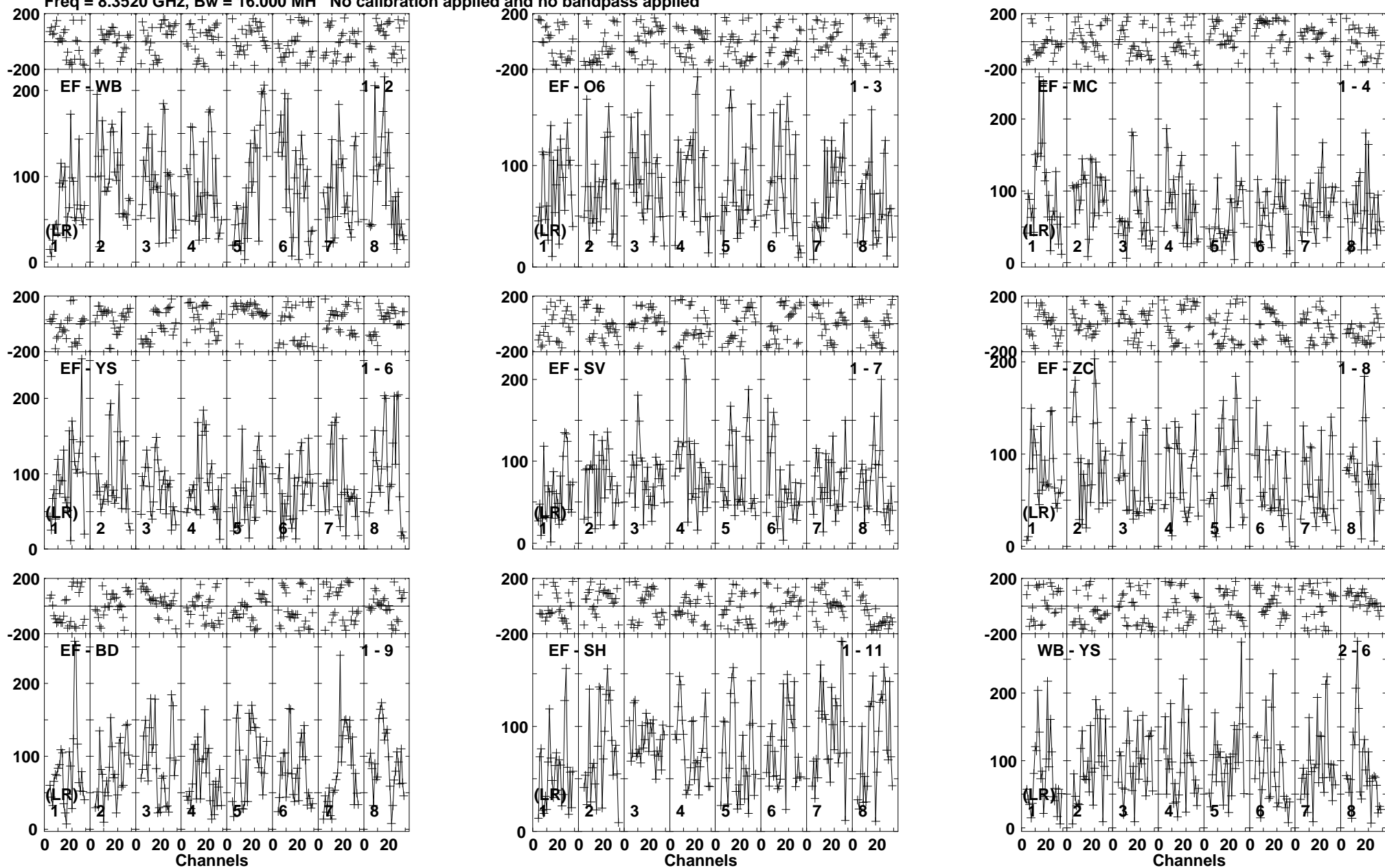
Lower frame: Micro Ampl Jy Top frame: Phas deg Vector averaged cross-power spectrum Baseline: EF (01) - WB (02) Timerange: 00/05:35:06 to 00/05:37:59
