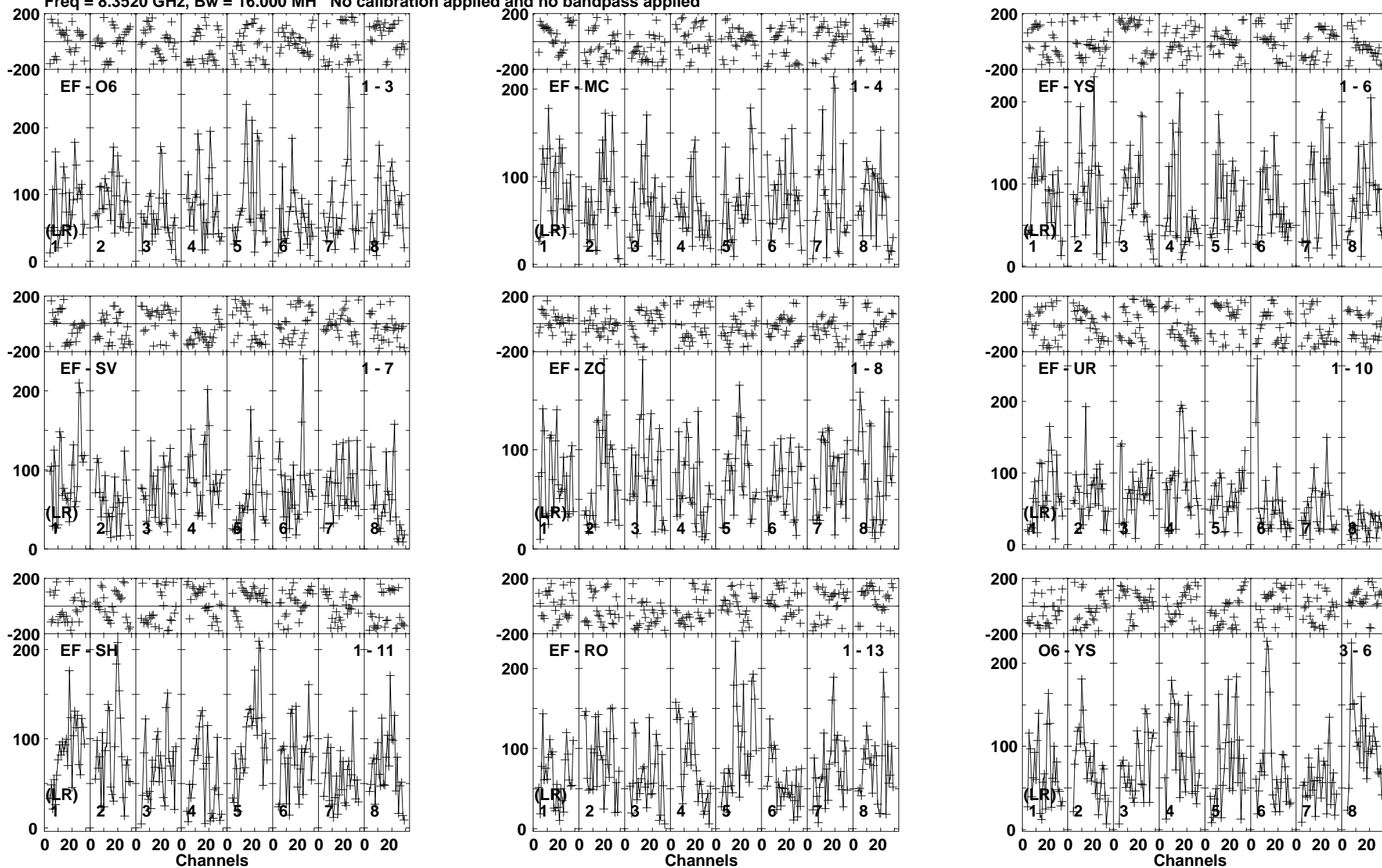
Lower frame: Micro Ampl Jy Top frame: Phas deg Vector averaged cross-power spectrum Baseline: EF (01) - O6 (03) Timerange: 00/01:48:06 to 00/01:51:00
