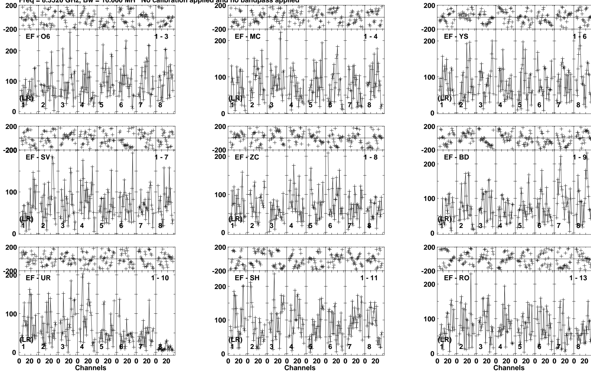
Lower frame: Micro Ampl Jy Top frame: Phas deg Vector averaged cross-power spectrum Baseline: EF (01) - O6 (03) Timerange: 00/01:31:35 to 00/01:34:30
