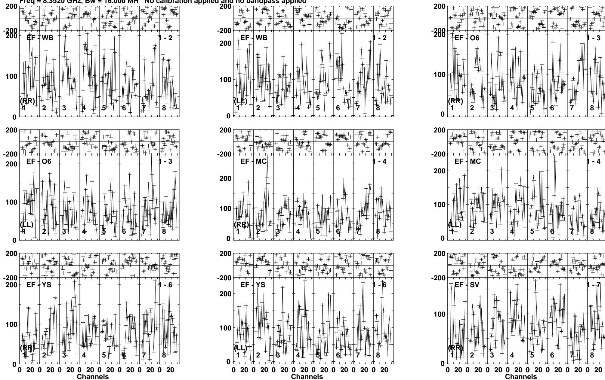
Lower frame: Micro Ampl Jy Top frame: Phas deg Vector averaged cross-power spectrum Baseline: EF (01) - WB (02) Timerange: 00/05:43:21 to 00/05:46:14
