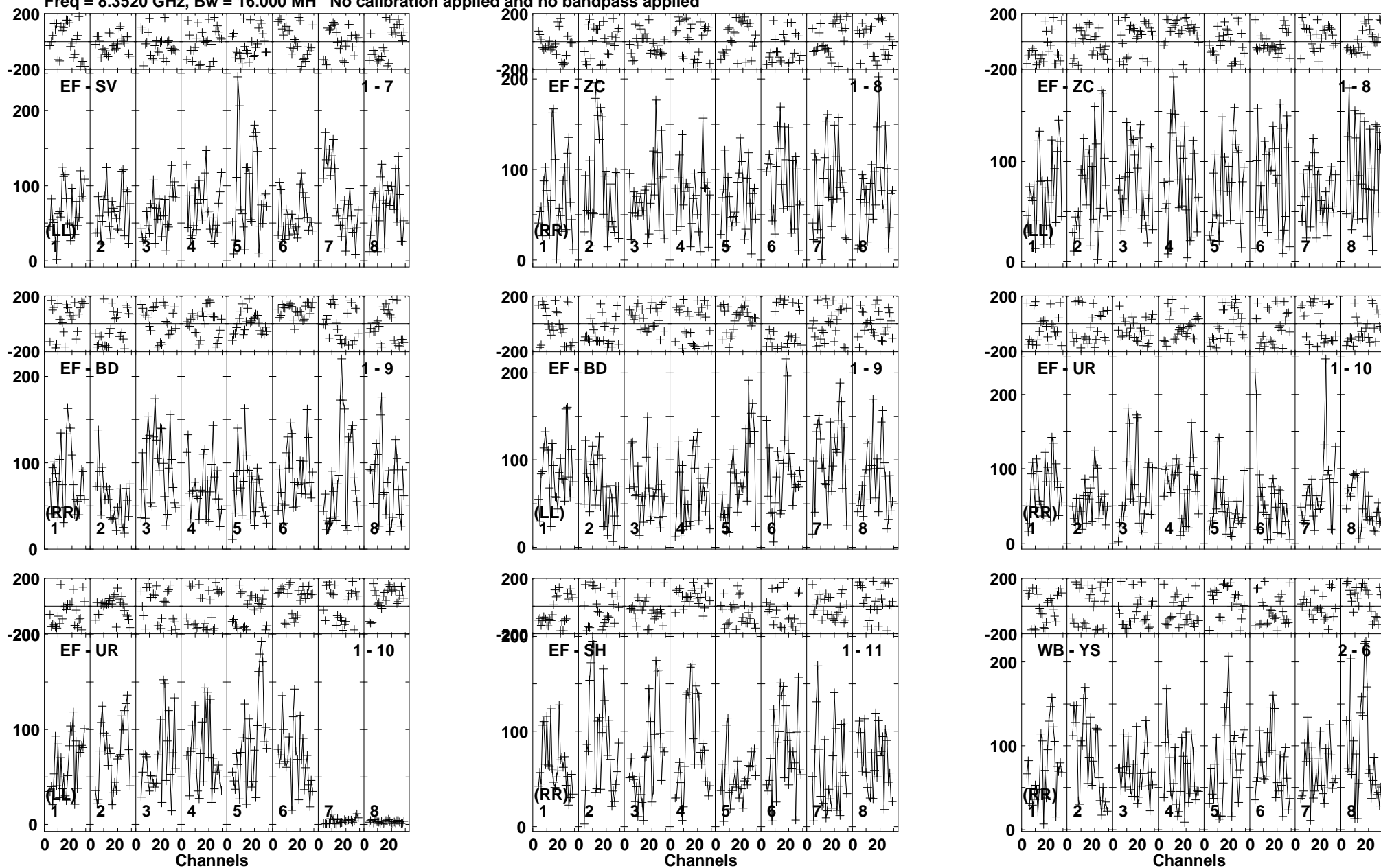
Lower frame: Micro Ampl Jy Top frame: Phas deg Vector averaged cross-power spectrum Baseline: EF (01) - SV (07) Timerange: 00/03:35:19 to 00/03:38:15
