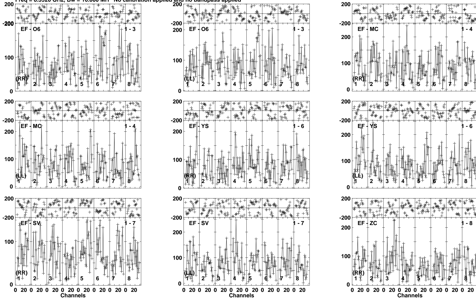
Lower frame: Micro Ampl Jy Top frame: Phas deg Vector averaged cross-power spectrum Baseline: EF (01) - O6 (03) Timerange: 00/00:54:36 to 00/00:57:30
