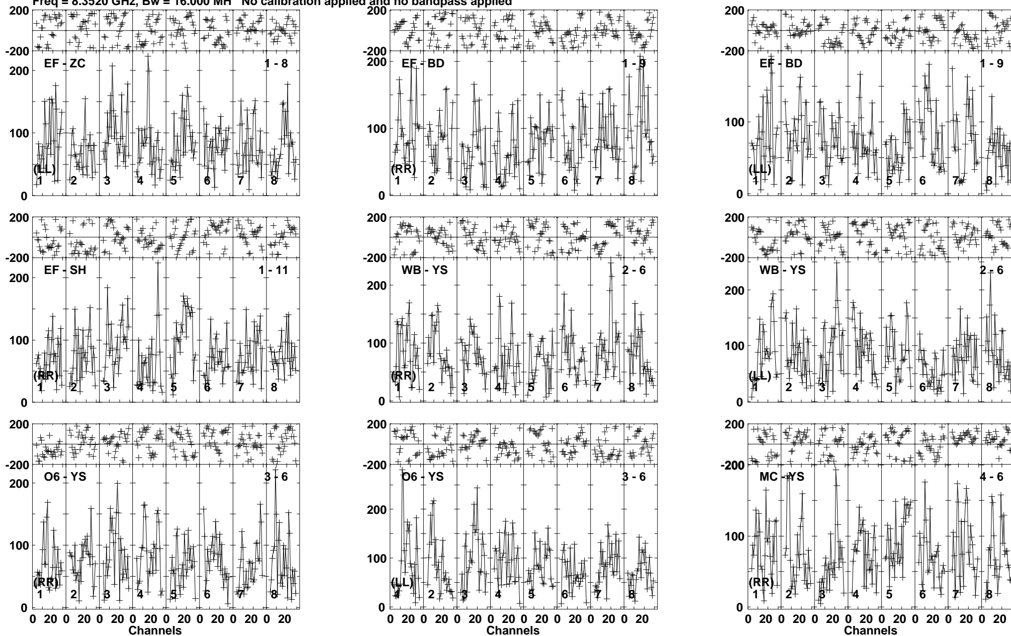
Lower frame: Micro Ampl Jy Top frame: Phas deg Vector averaged cross-power spectrum Baseline: EF (01) - ZC (08) Timerange: 00/05:59:51 to 00/06:02:44
