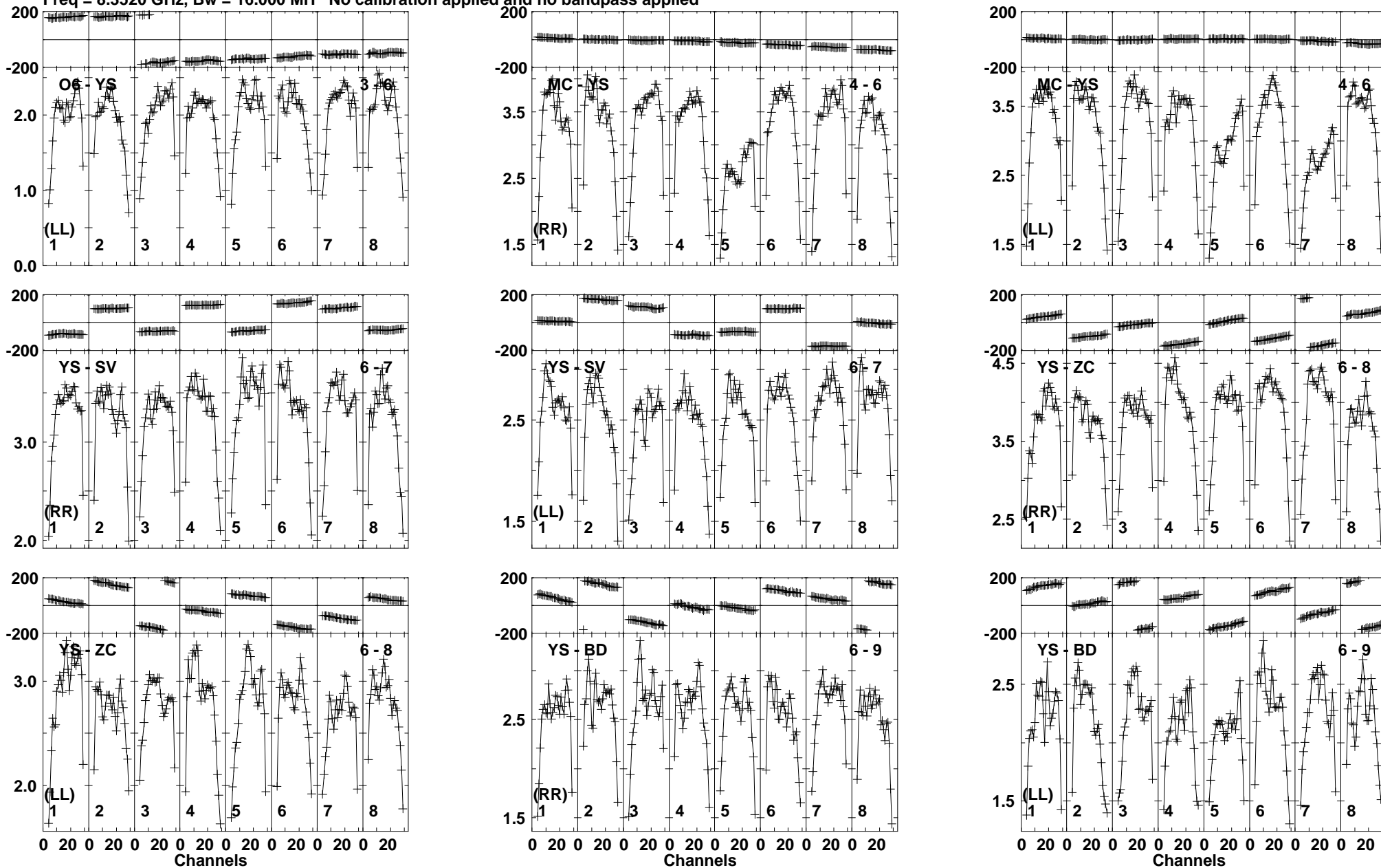
Lower frame: Milli Ampl Jy Top frame: Phas deg Vector averaged cross-power spectrum Baseline: O6 (03) - YS (06) Timerange: 00/01:22:20 to 00/01:23:14
