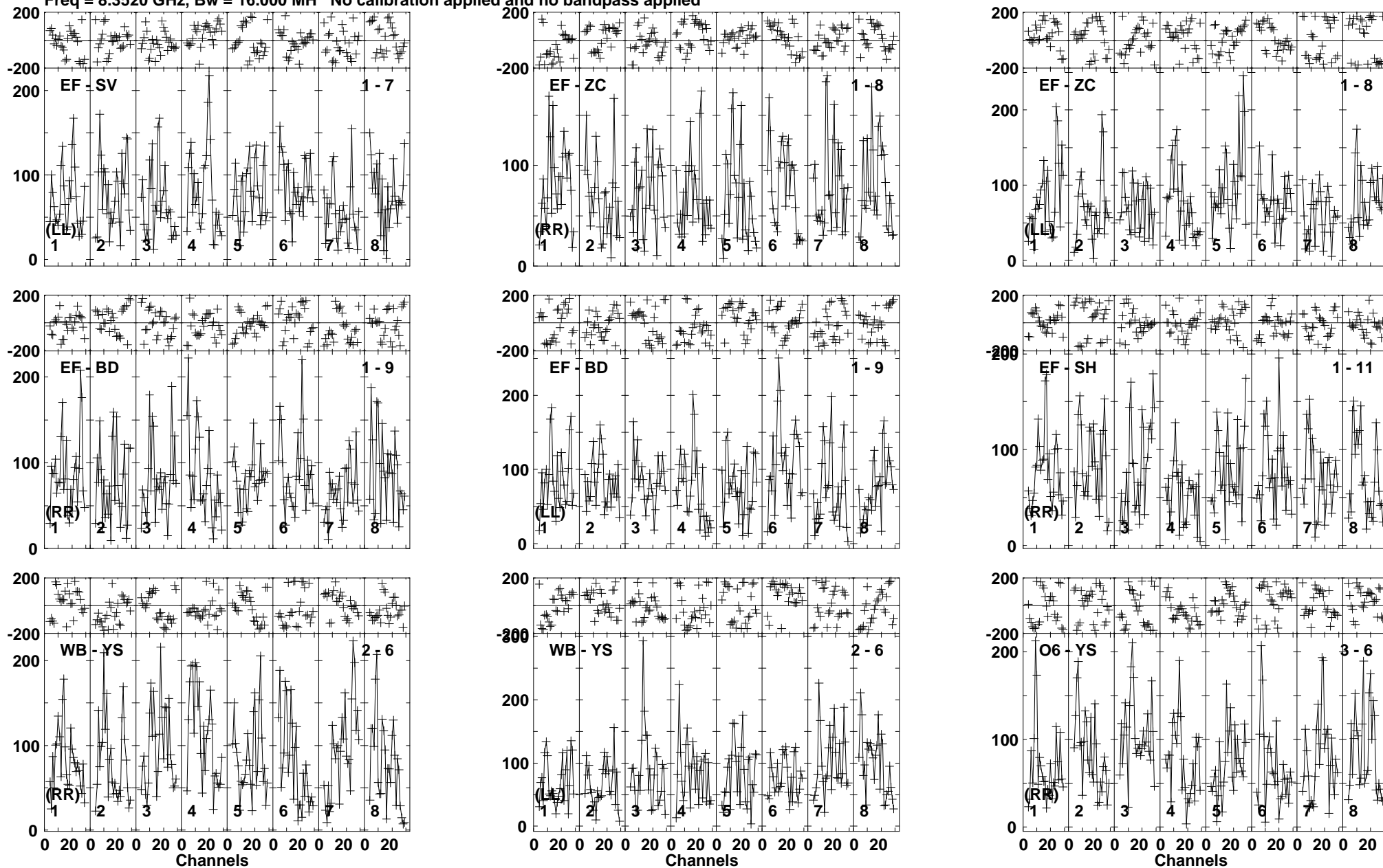
Lower frame: Micro Ampl Jy Top frame: Phas deg Vector averaged cross-power spectrum Baseline: EF (01) - SV (07) Timerange: 00/04:41:21 to 00/04:44:14
