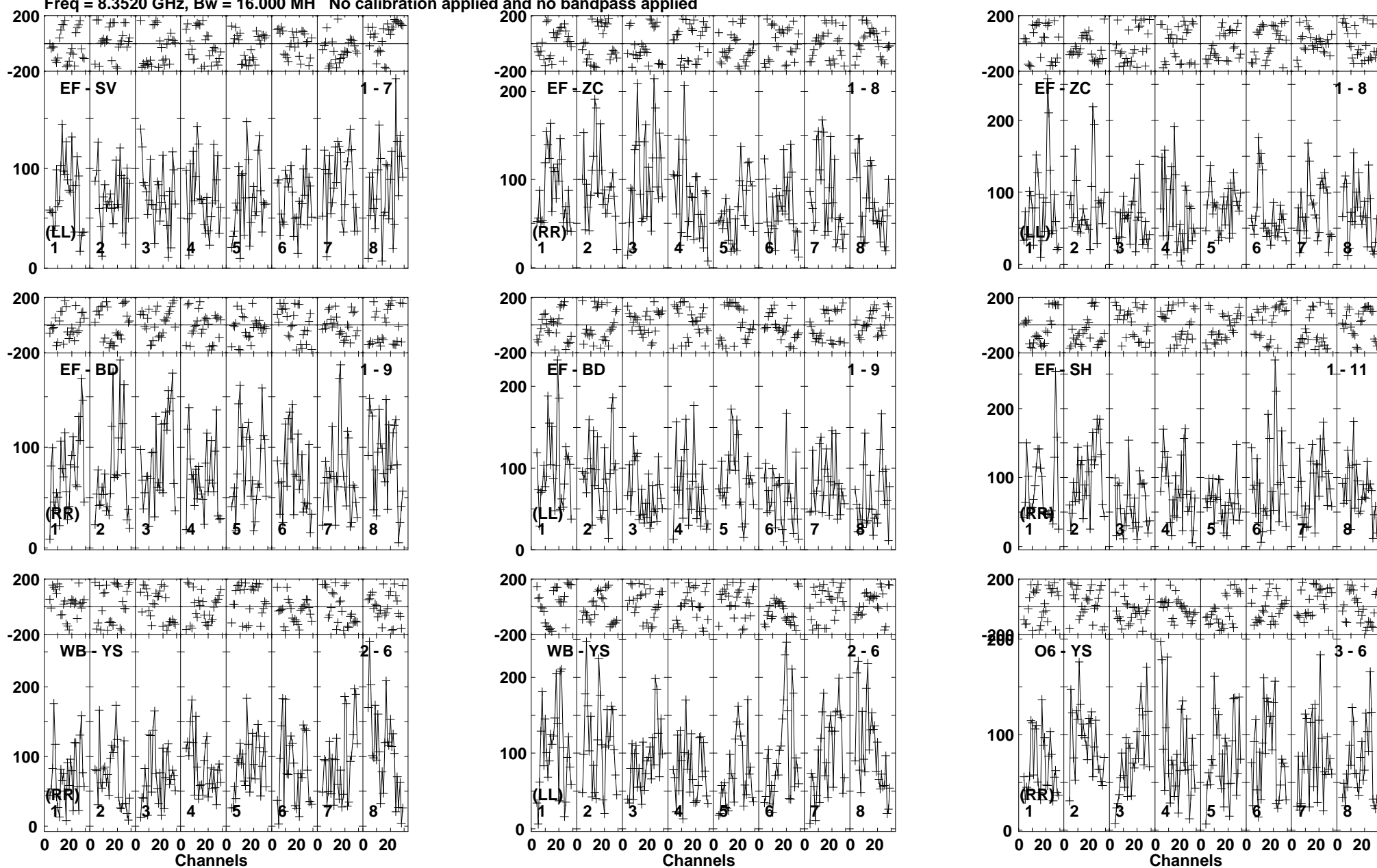
Lower frame: Micro Ampl Jy Top frame: Phas deg Vector averaged cross-power spectrum Baseline: EF (01) - SV (07) Timerange: 00/05:43:21 to 00/05:46:14
