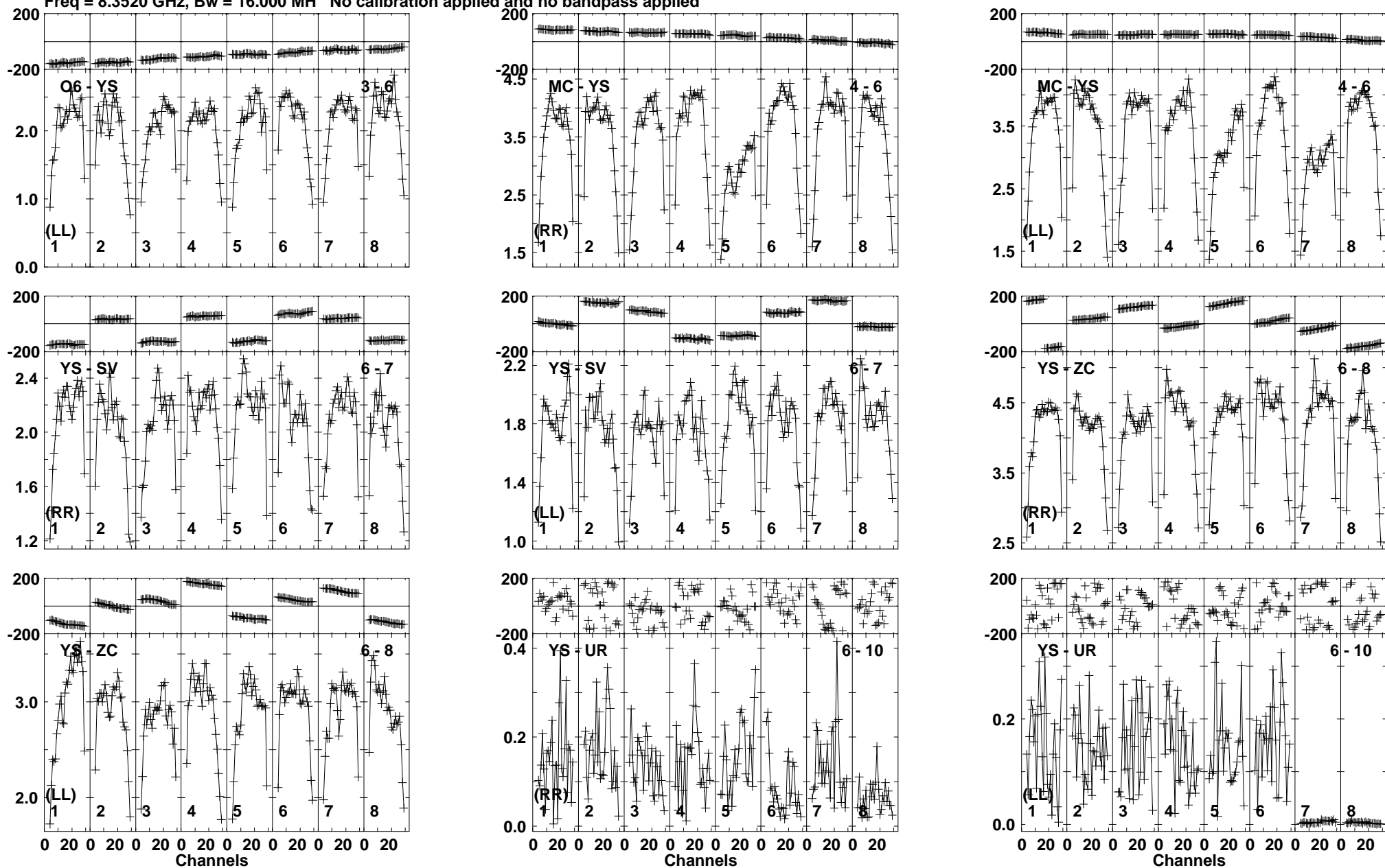
Lower frame: Milli Ampl Jy Top frame: Phas deg Vector averaged cross-power spectrum Baseline: O6 (03) - YS (06) Timerange: 00/03:05:56 to 00/03:06:30
