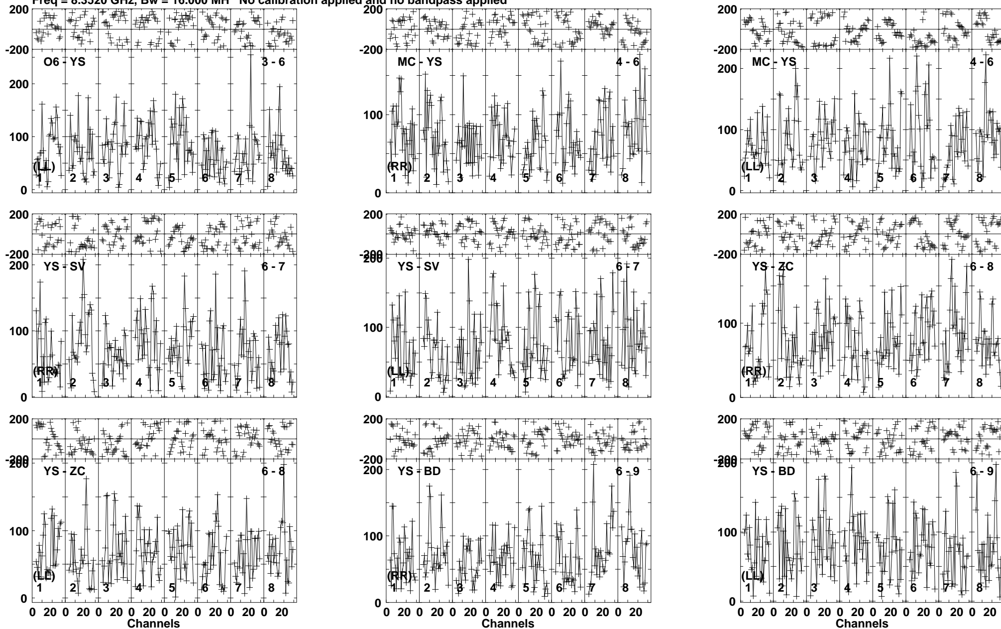
Lower frame: Micro Ampl Jy Top frame: Phas deg Vector averaged cross-power spectrum Baseline: O6 (03) - YS (06) Timerange: 00/01:31:35 to 00/01:34:30
