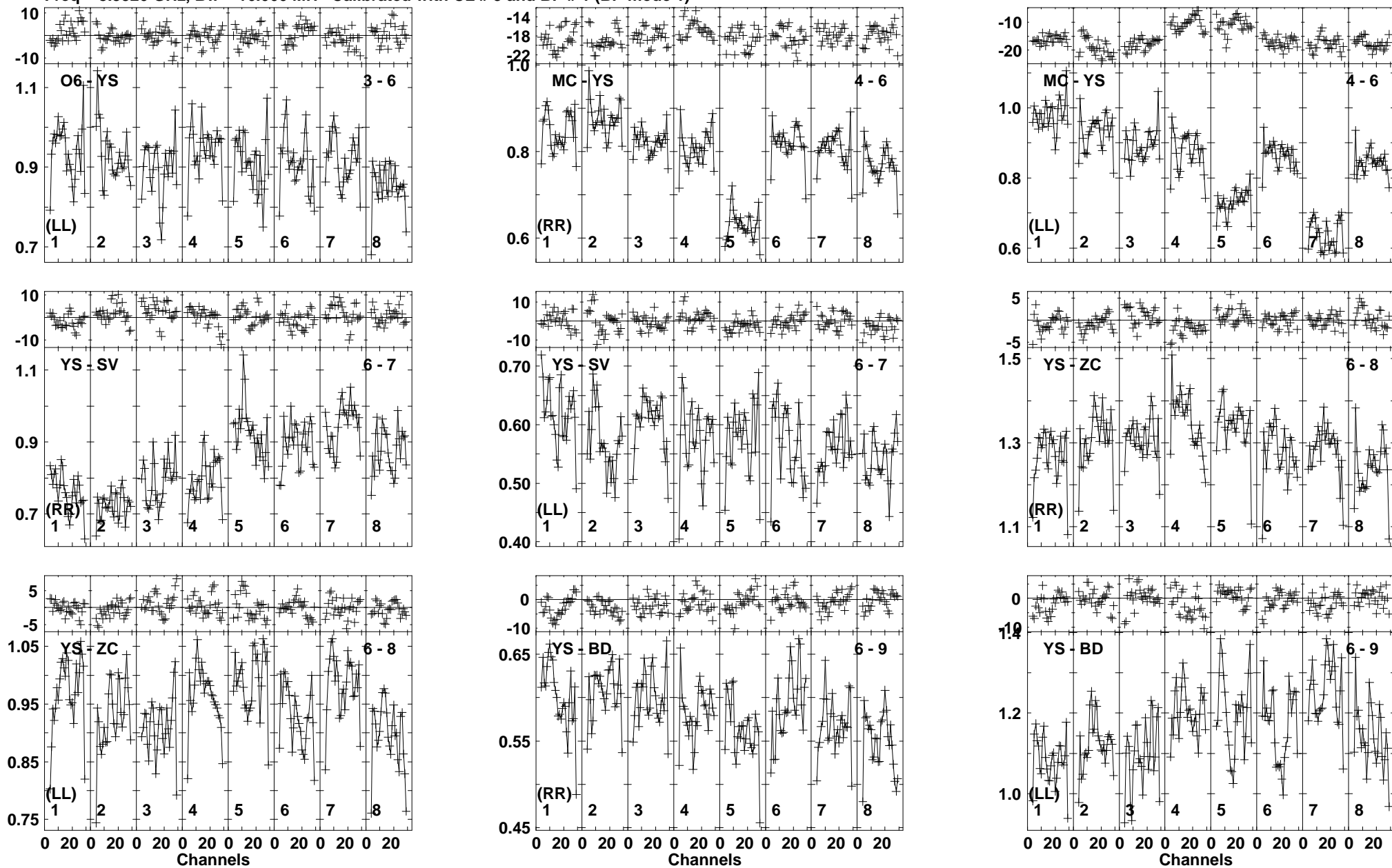
Lower frame: Ampl Jy Top frame: Phas deg Vector averaged cross-power spectrum Baseline: O6 (03) - YS (06) Timerange: 00/03:30:41 to 00/03:31:14
