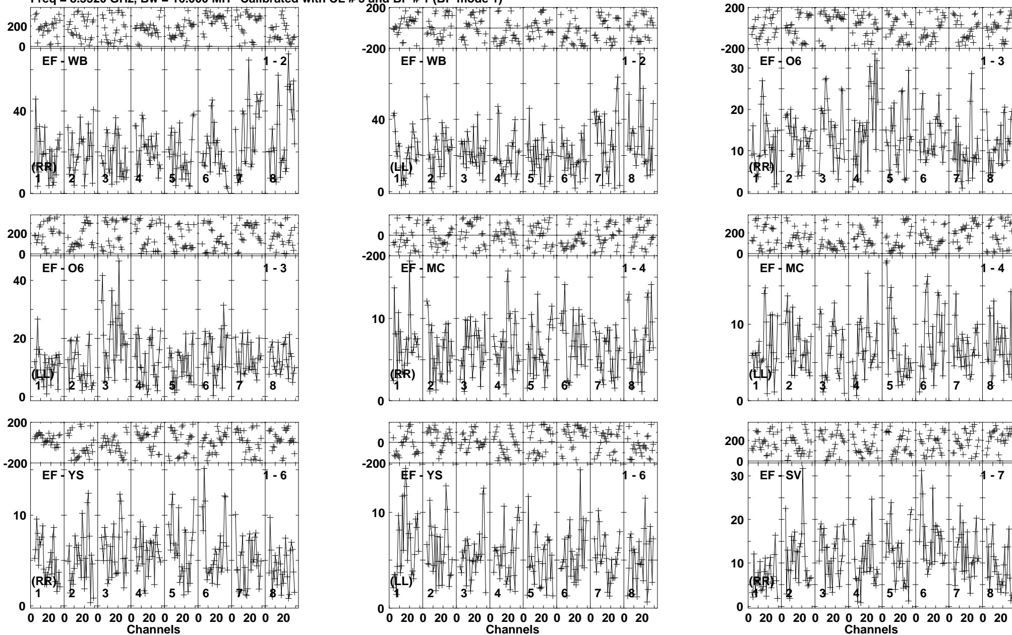
Lower frame: Milli Ampl Jy Top frame: Phas deg Vector averaged cross-power spectrum Baseline: EF (01) - WB (02) Timerange: 00/03:02:20 to 00/03:05:14
