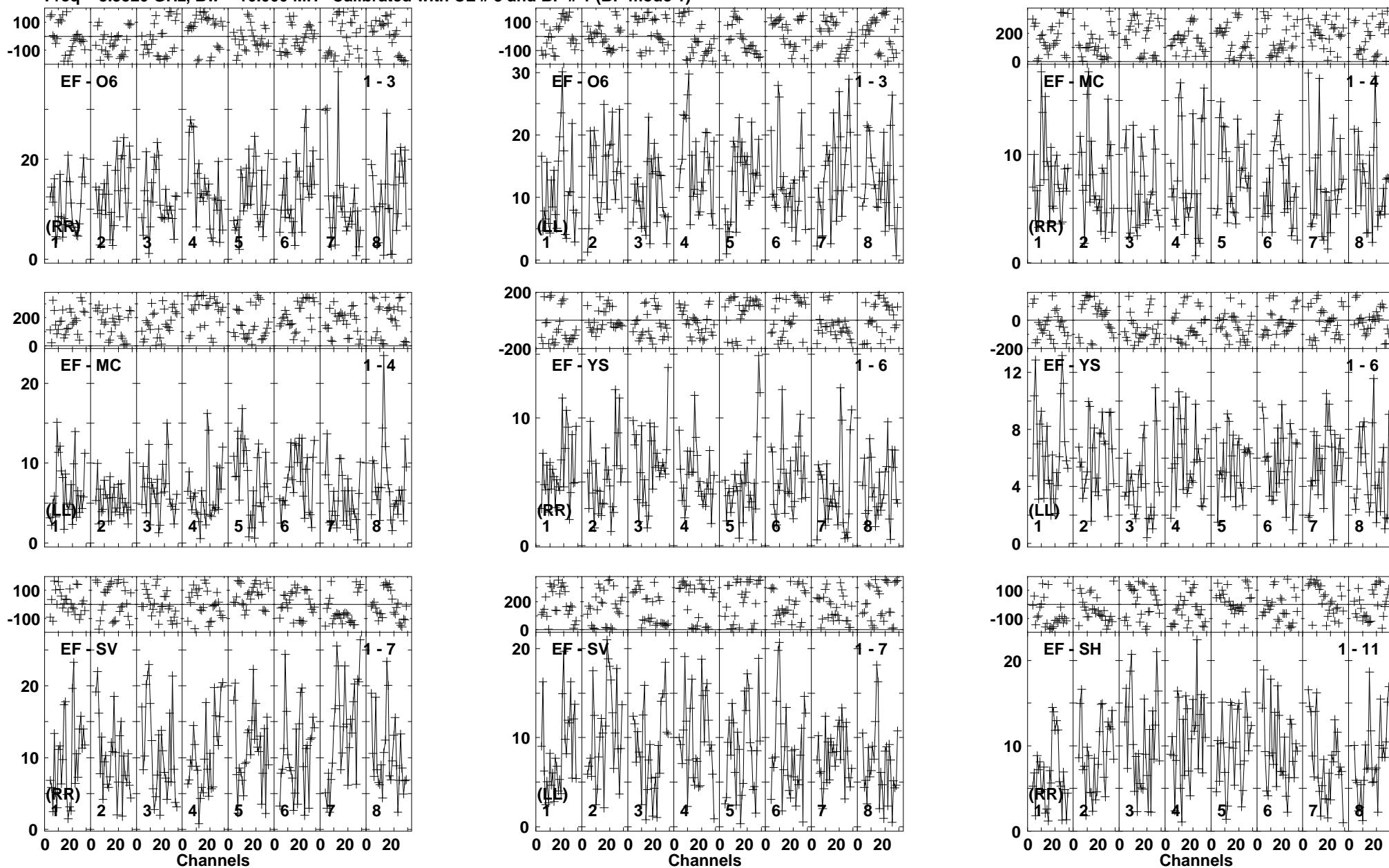
Lower frame: Milli Ampl Jy Top frame: Phas deg Vector averaged cross-power spectrum Baseline: EF (01) - O6 (03) Timerange: 00/01:52:20 to 00/01:55:15
