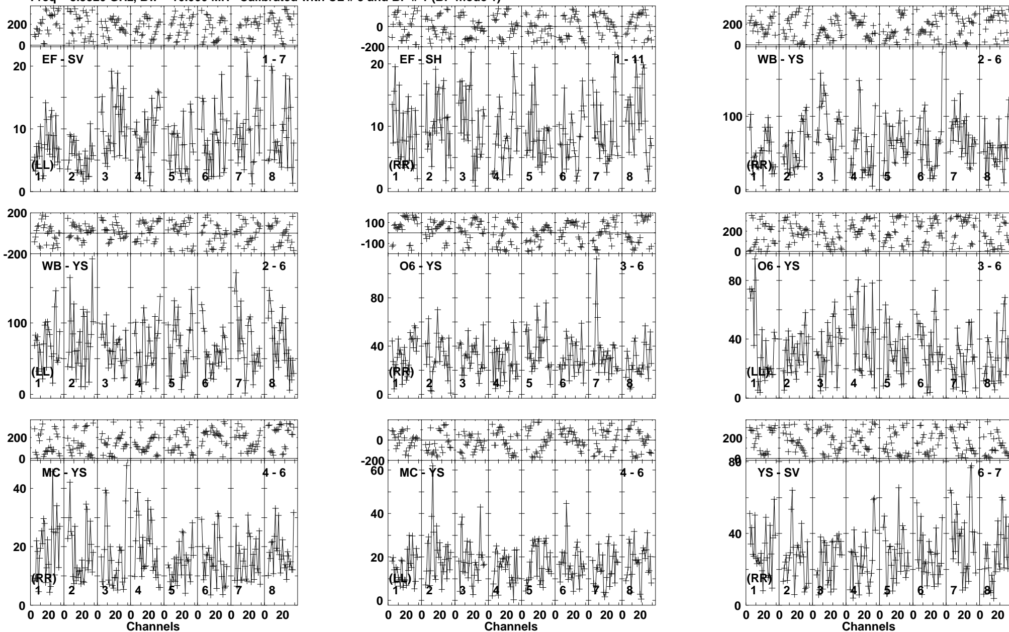
Lower frame: Milli Ampl Jy Top frame: Phas deg Vector averaged cross-power spectrum Baseline: EF (01) - SV (07) Timerange: 00/05:55:32 to 00/05:58:30
