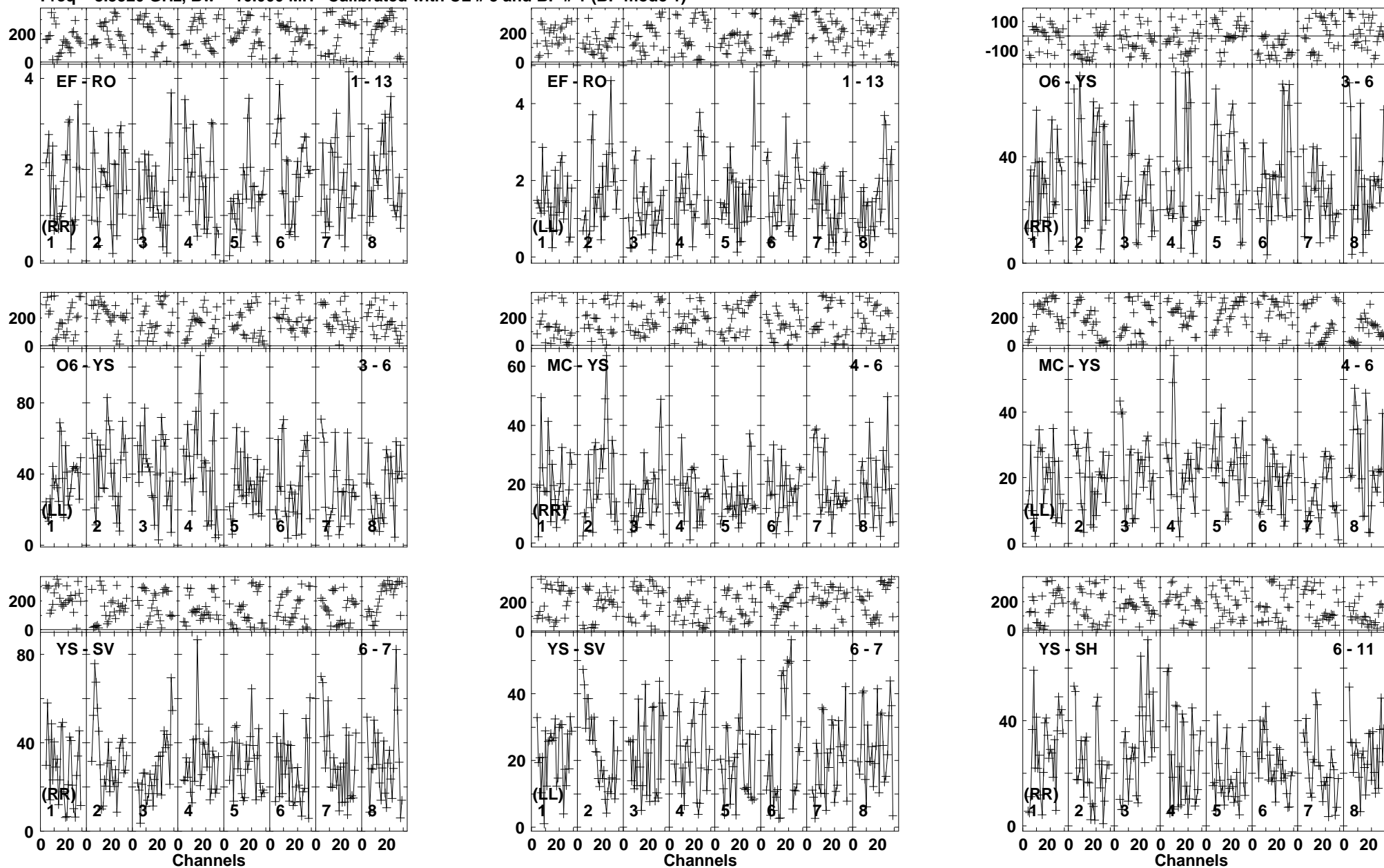
Lower frame: Milli Ampl Jy Top frame: Phas deg Vector averaged cross-power spectrum Baseline: EF (01) - RO (13) Timerange: 00/02:12:50 to 00/02:15:44
