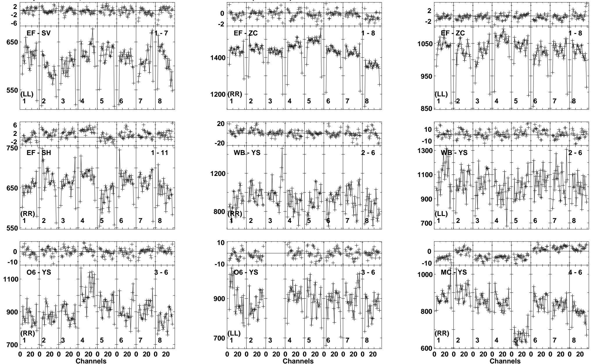
Lower frame: Milli Ampl Jy Top frame: Phas deg Vector averaged cross-power spectrum Baseline: EF (01) - SV (07) Timerange: 00/02:57:42 to 00/02:58:15
