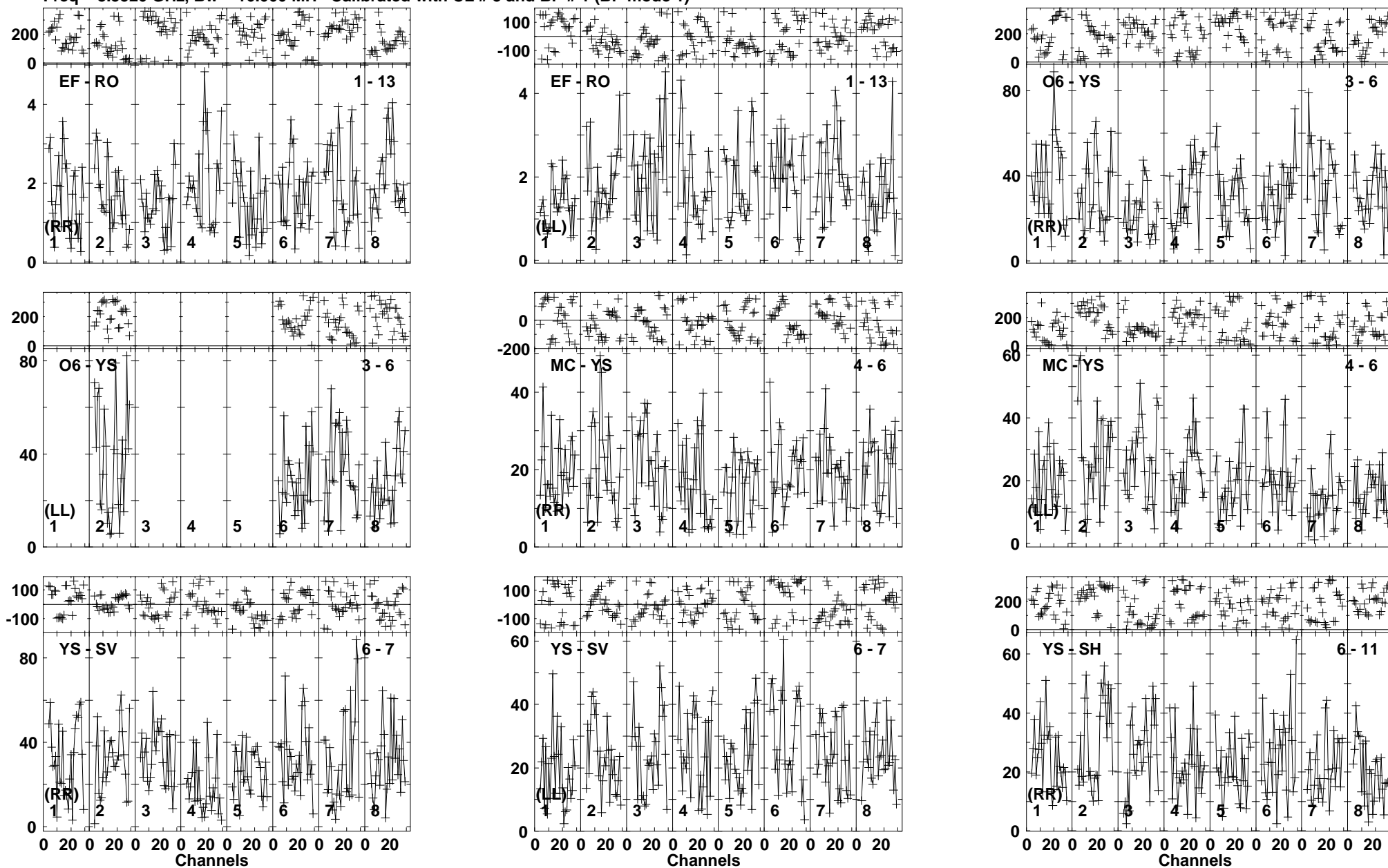
Lower frame: Milli Ampl Jy Top frame: Phas deg Vector averaged cross-power spectrum Baseline: EF (01) - RO (13) Timerange: 00/02:17:05 to 00/02:19:59
