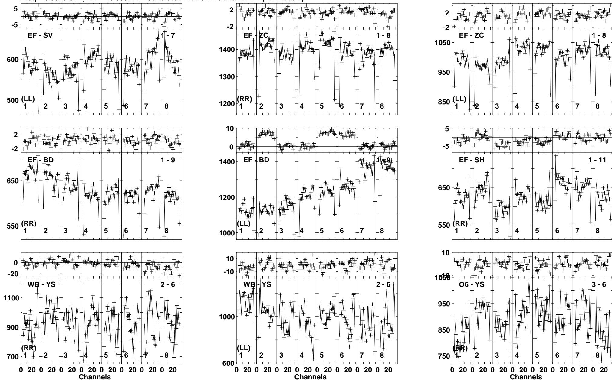
Lower frame: Milli Ampl Jy Top frame: Phas deg Vector averaged cross-power spectrum Baseline: EF (01) - SV (07) Timerange: 00/03:47:11 to 00/03:47:44
