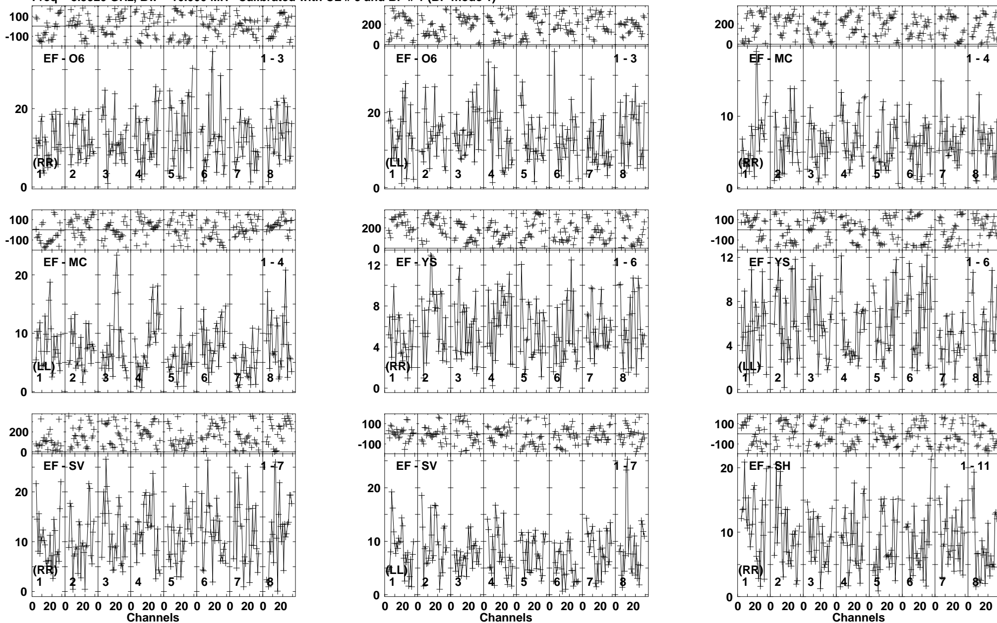
Lower frame: Milli Ampl Jy Top frame: Phas deg Vector averaged cross-power spectrum Baseline: EF (01) - O6 (03) Timerange: 00/01:48:06 to 00/01:51:00
