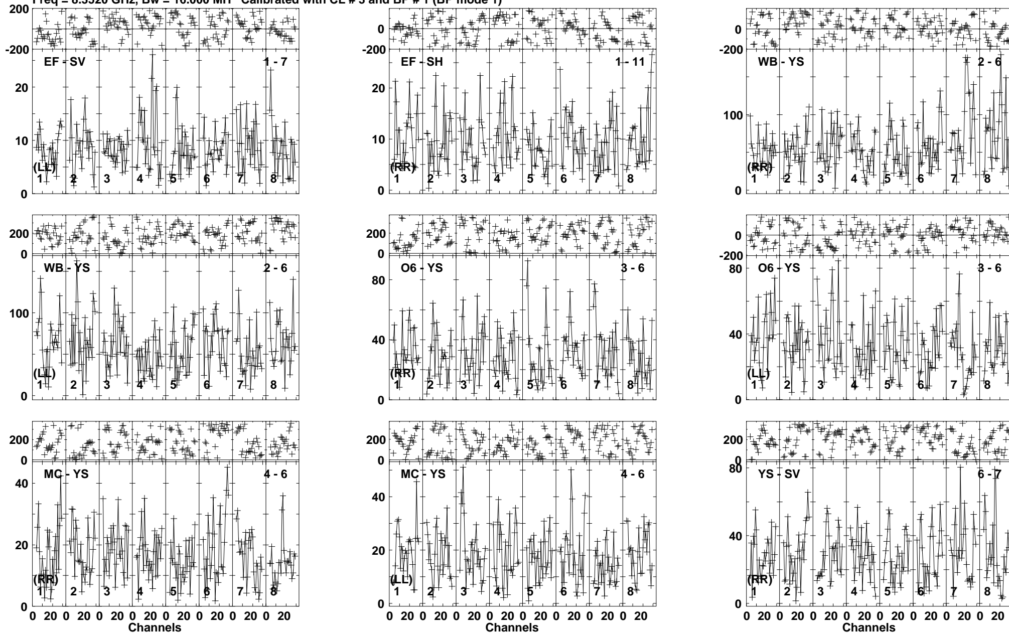
Lower frame: Milli Ampl Jy Top frame: Phas deg Vector averaged cross-power spectrum Baseline: EF (01) - SV (07) Timerange: 00/03:47:50 to 00/03:50:45
