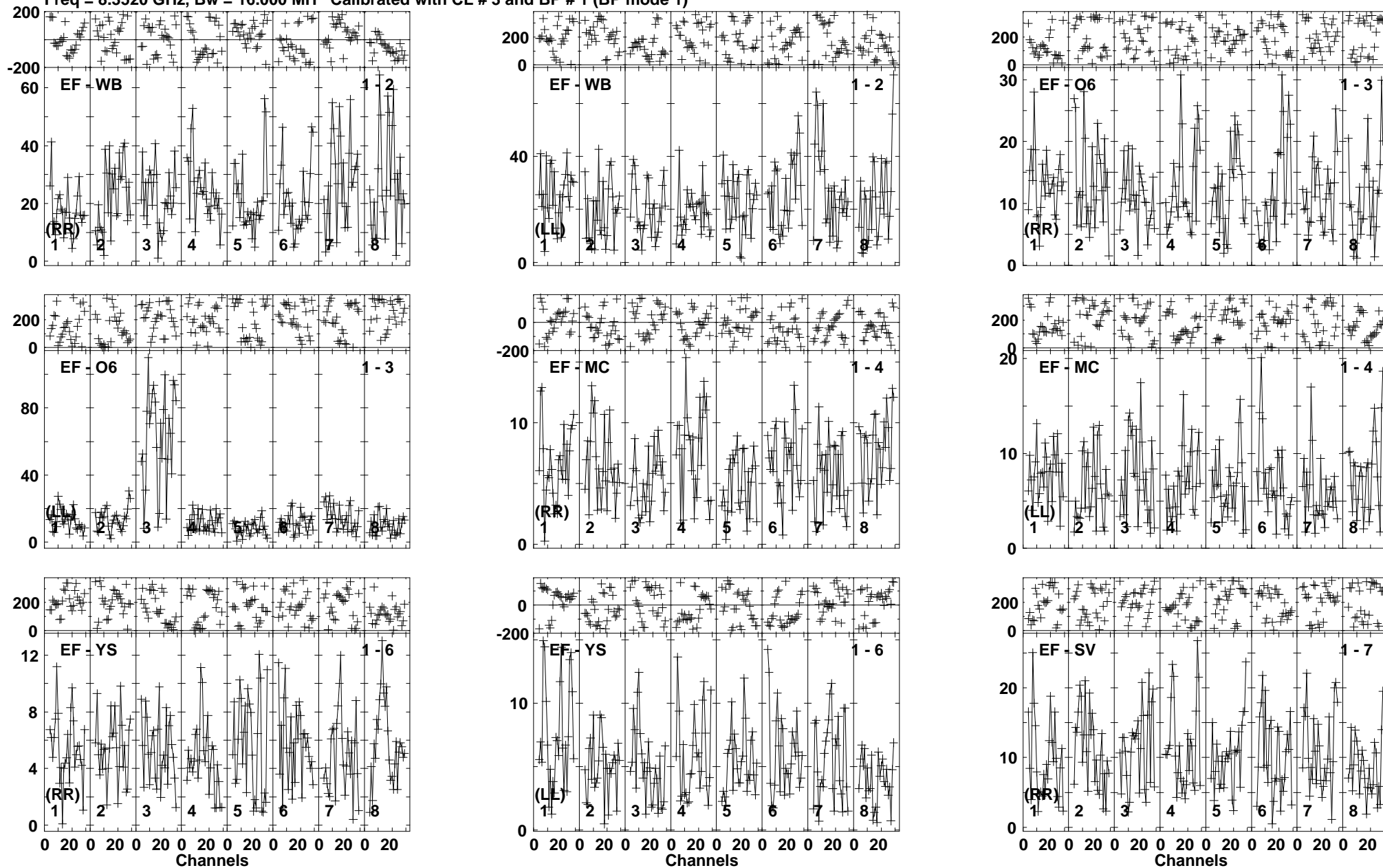
Lower frame: Milli Ampl Jy Top frame: Phas deg Vector averaged cross-power spectrum Baseline: EF (01) - WB (02) Timerange: 00/03:10:35 to 00/03:13:30
