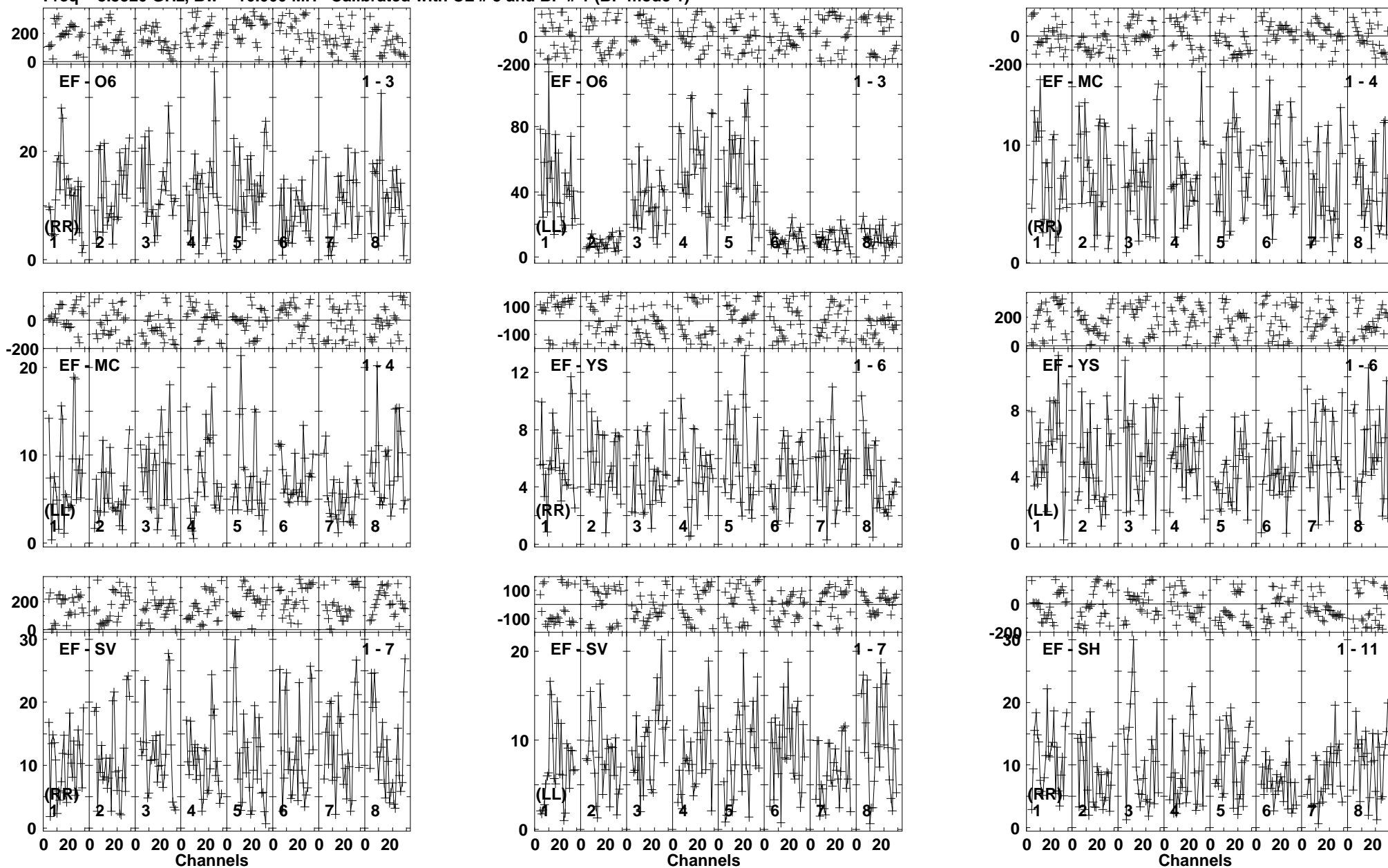
Lower frame: Milli Ampl Jy Top frame: Phas deg Vector averaged cross-power spectrum Baseline: EF (01) - O6 (03) Timerange: 00/02:37:36 to 00/02:40:30
