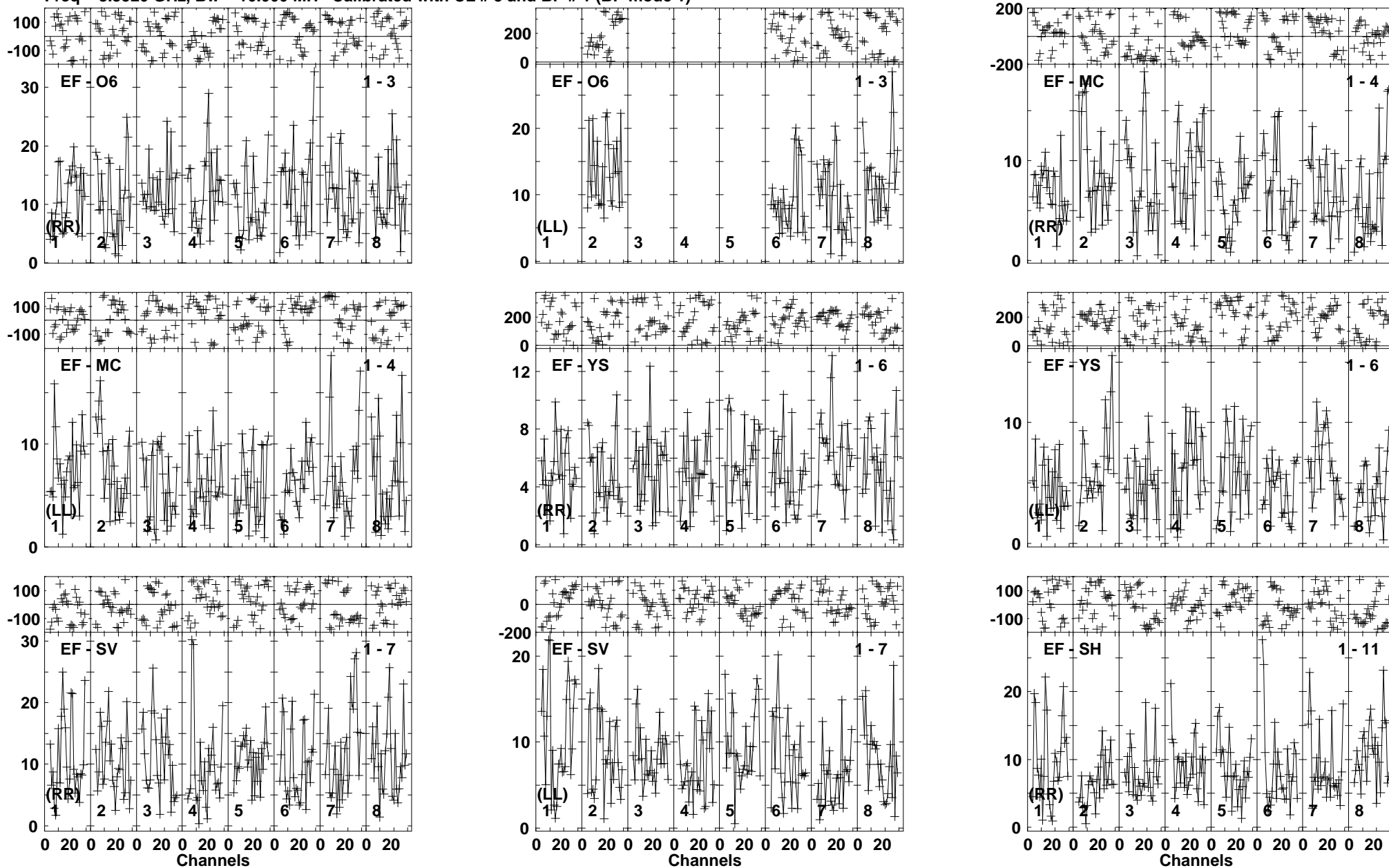
Lower frame: Milli Ampl Jy Top frame: Phas deg Vector averaged cross-power spectrum Baseline: EF (01) - O6 (03) Timerange: 00/02:21:05 to 00/02:23:59
