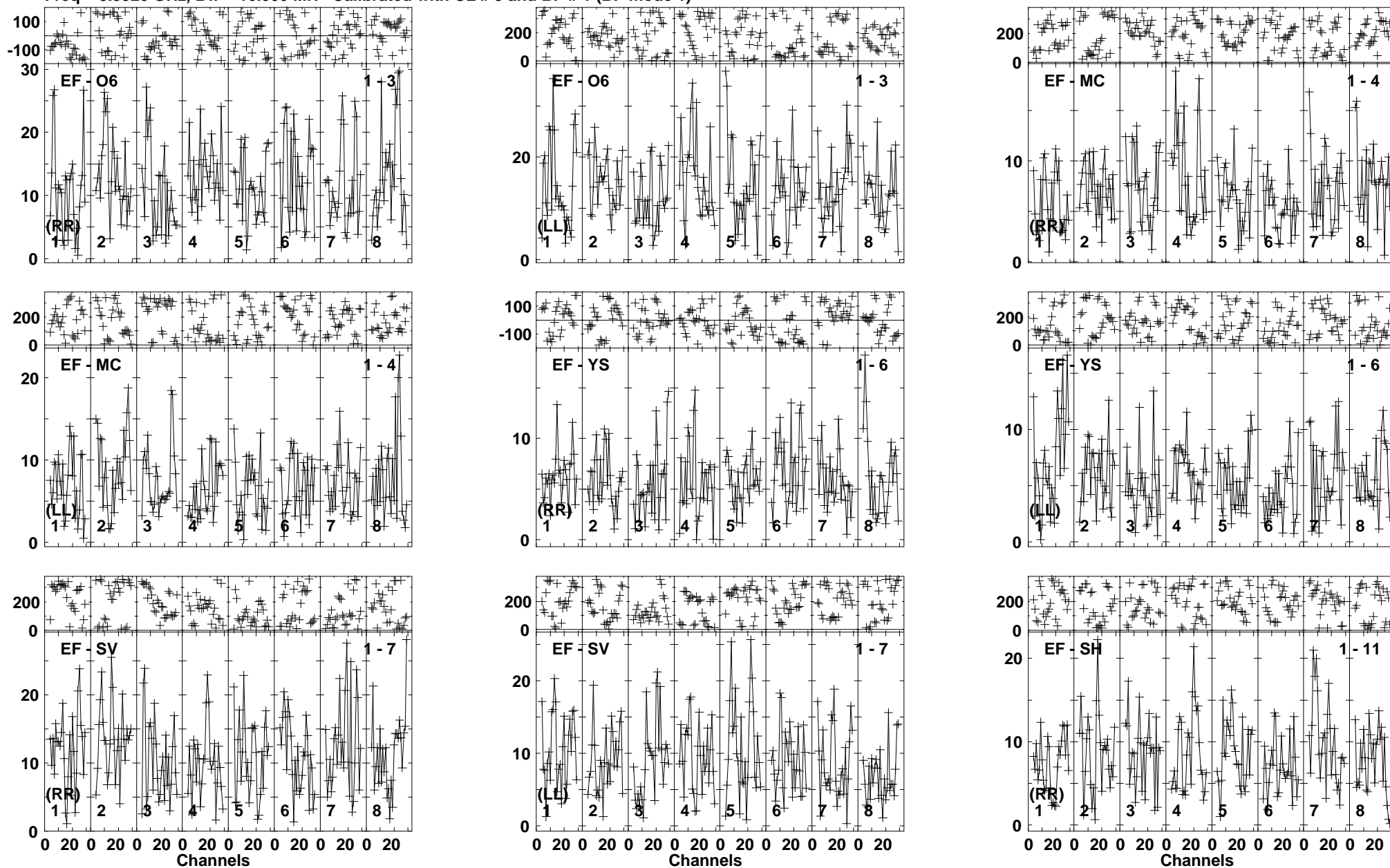
Lower frame: Milli Ampl Jy Top frame: Phas deg Vector averaged cross-power spectrum Baseline: EF (01) - O6 (03) Timerange: 00/01:19:20 to 00/01:22:14
