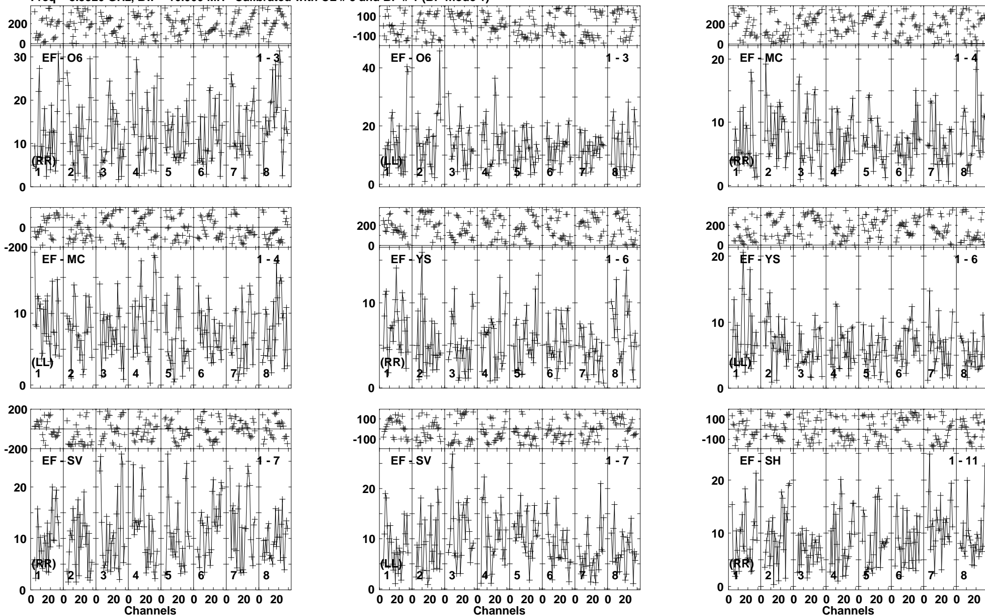
Lower frame: Milli Ampl Jy Top frame: Phas deg Vector averaged cross-power spectrum Baseline: EF (01) - O6 (03) Timerange: 00/01:23:20 to 00/01:26:15
