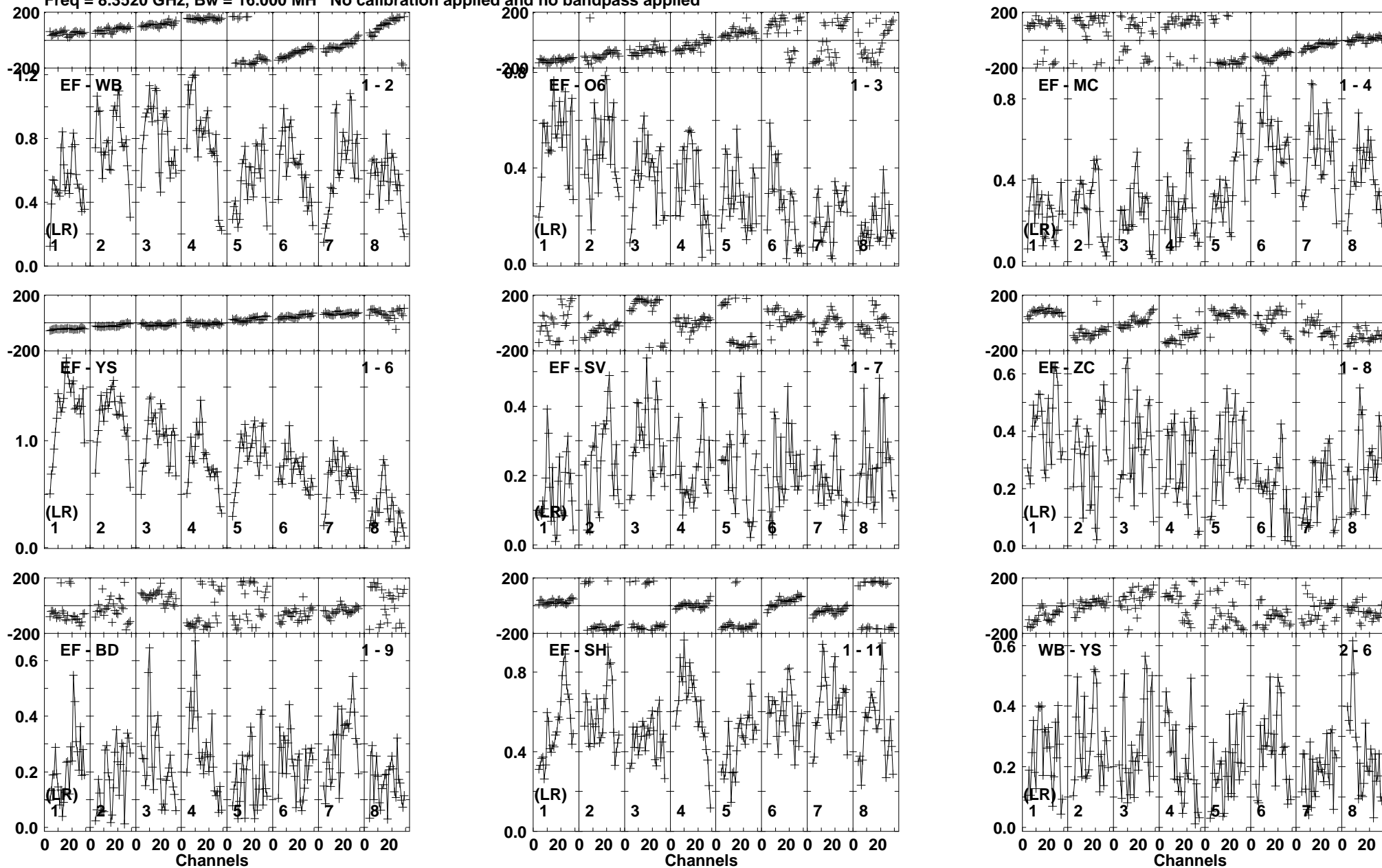
Lower frame: Milli Ampl Jy Top frame: Phas deg Vector averaged cross-power spectrum Baseline: EF (01) - WB (02) Timerange: 00/04:11:56 to 00/04:12:29
