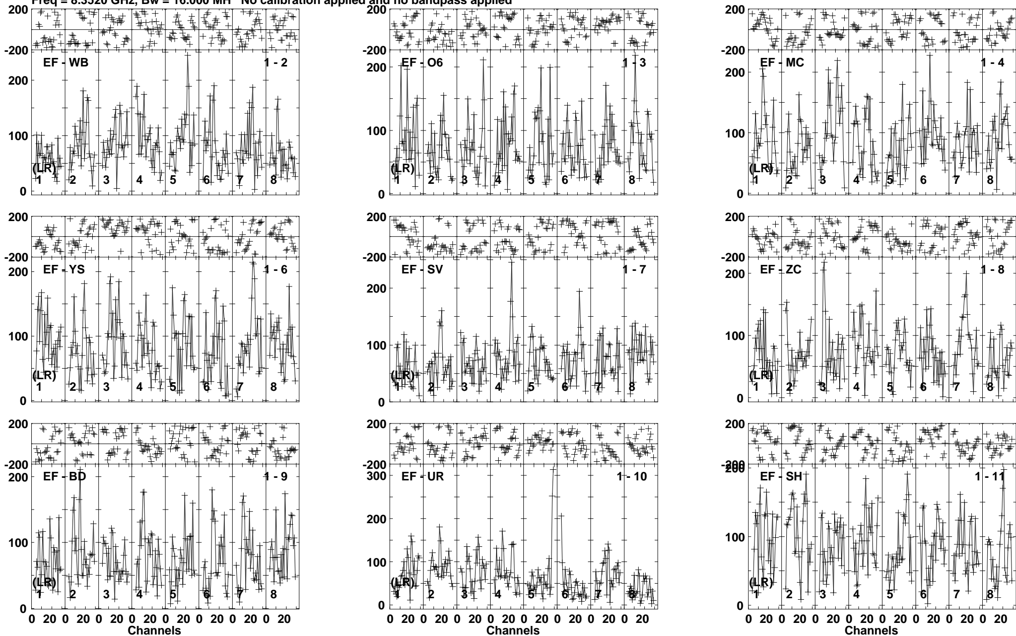
Lower frame: Micro Ampl Jy Top frame: Phas deg Vector averaged cross-power spectrum Baseline: EF (01) - WB (02) Timerange: 00/03:51:49 to 00/03:54:45
