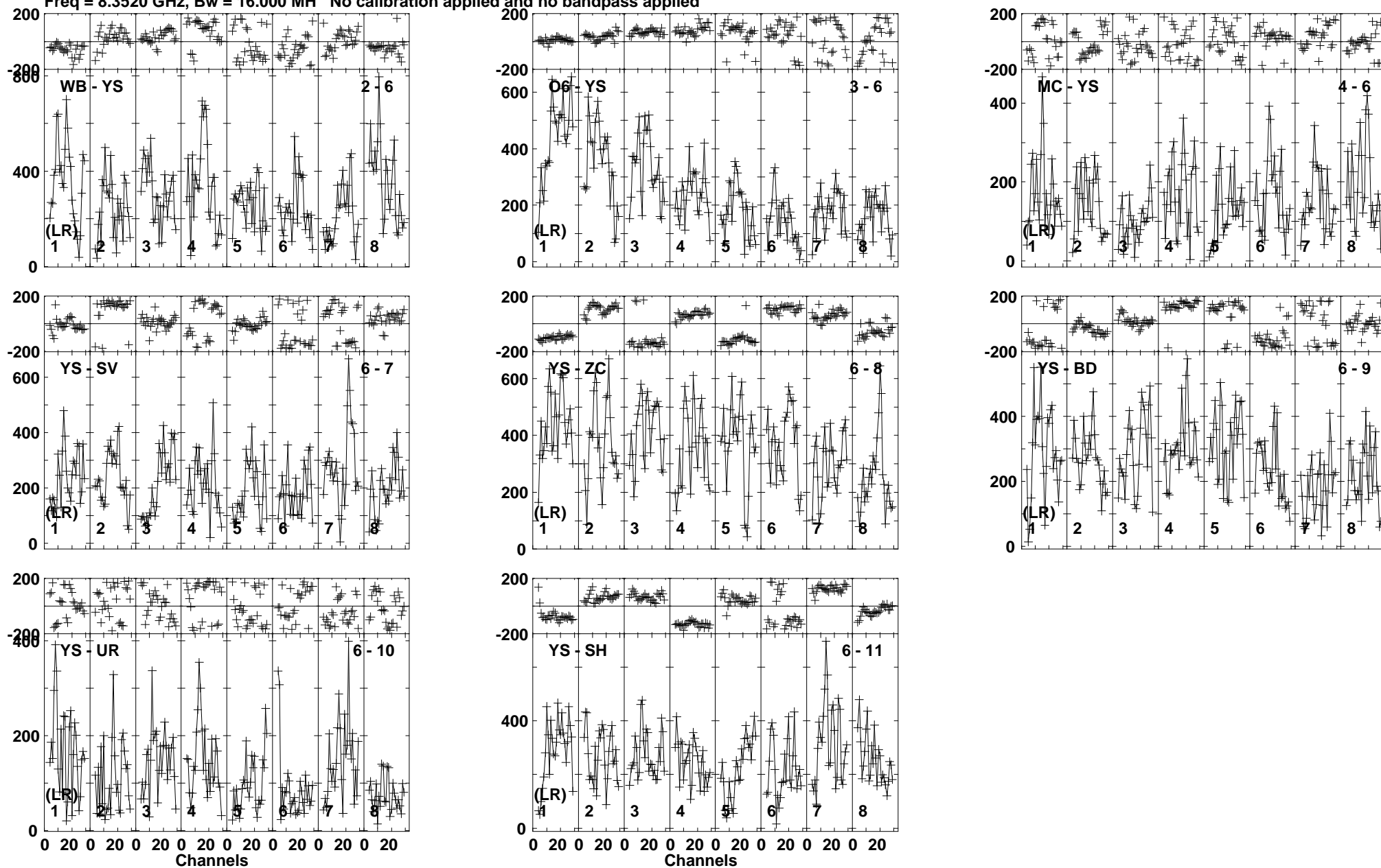
Lower frame: Micro Ampl Jy Top frame: Phas deg Vector averaged cross-power spectrum Baseline: WB (02) - YS (06) Timerange: 00/03:17:50 to 00/03:18:45
