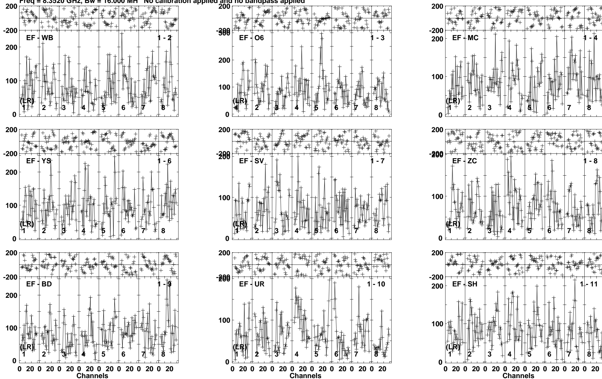
Lower frame: Micro Ampl Jy Top frame: Phas deg Vector averaged cross-power spectrum Baseline: EF (01) - WB (02) Timerange: 00/03:14:49 to 00/03:17:45
