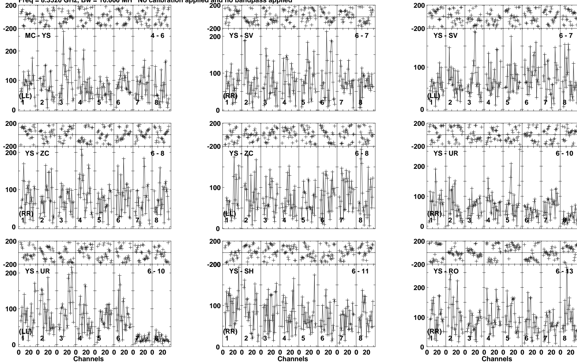
Lower frame: Micro Ampl Jy Top frame: Phas deg Vector averaged cross-power spectrum Baseline: MC (04) - YS (06) Timerange: 00/02:08:51 to 00/02:11:45
