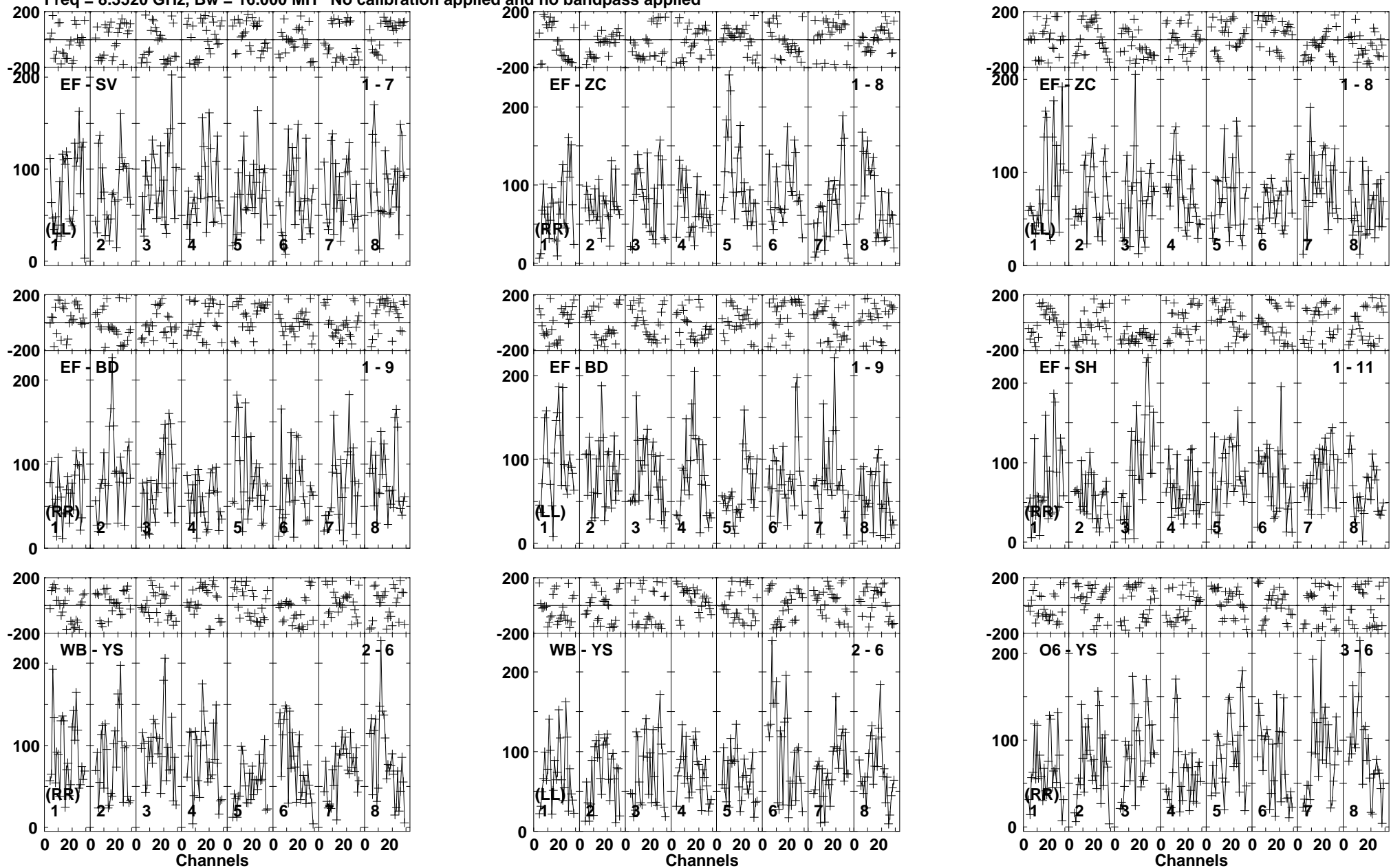
Lower frame: Micro Ampl Jy Top frame: Phas deg Vector averaged cross-power spectrum Baseline: EF (01) - SV (07) Timerange: 00/05:47:20 to 00/05:50:15
