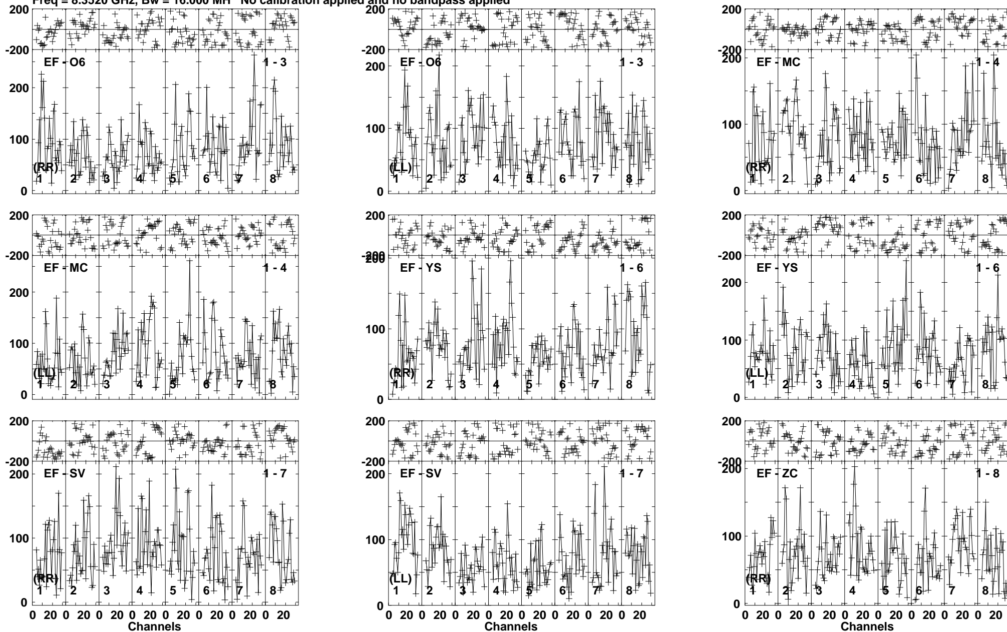
Lower frame: Micro Ampl Jy Top frame: Phas deg Vector averaged cross-power spectrum Baseline: EF (01) - O6 (03) Timerange: 00/02:33:36 to 00/02:36:30
