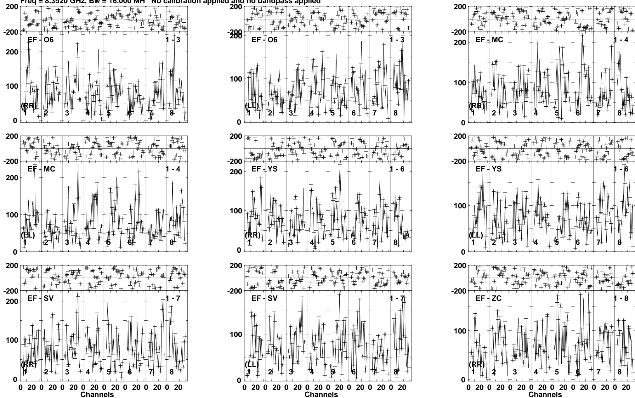
Lower frame: Micro Ampl Jy Top frame: Phas deg Vector averaged cross-power spectrum Baseline: EF (01) - O6 (03) Timerange: 00/02:37:36 to 00/02:40:30
