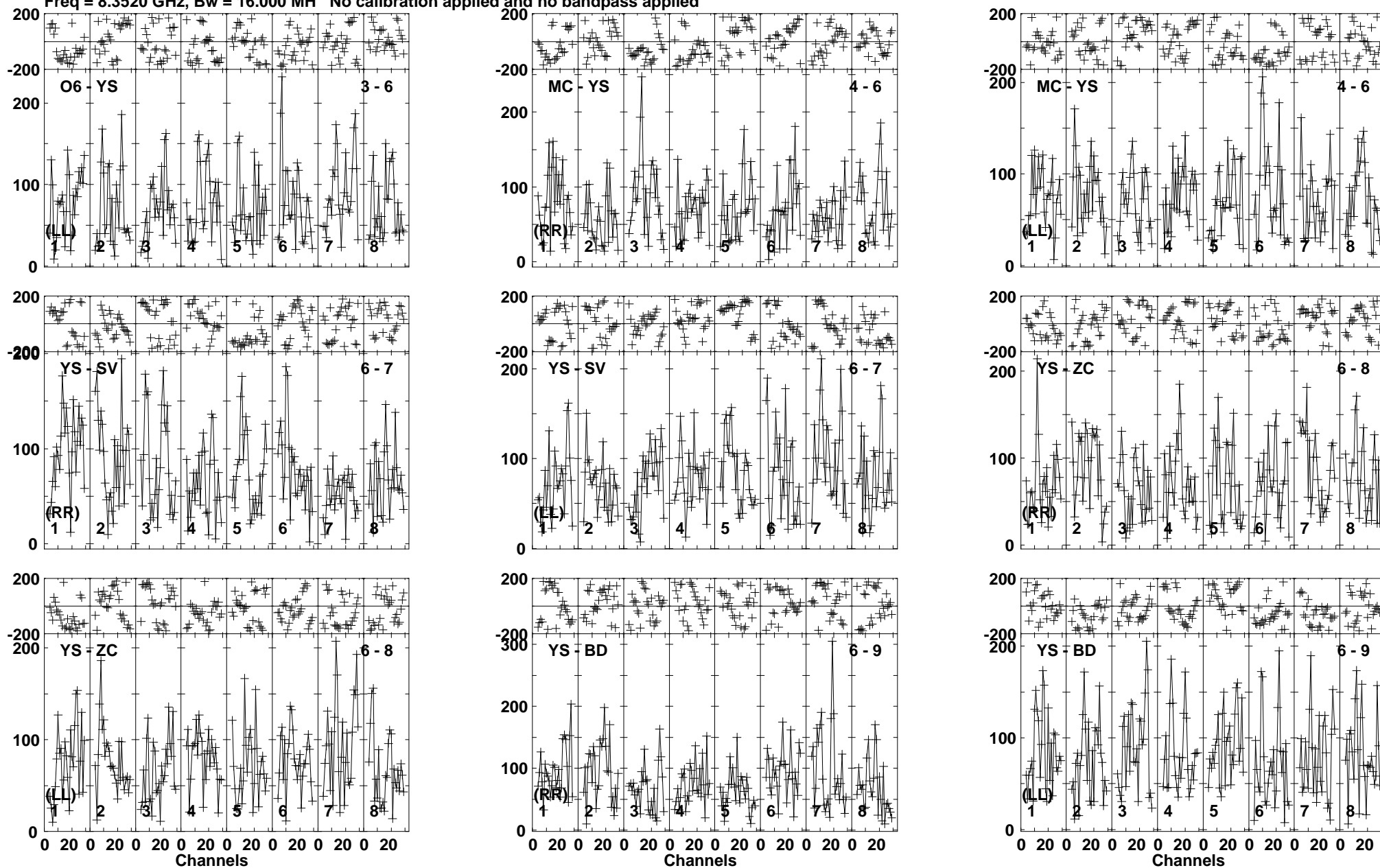
Lower frame: Micro Ampl Jy Top frame: Phas deg Vector averaged cross-power spectrum Baseline: O6 (03) - YS (06) Timerange: 00/05:14:20 to 00/05:17:15
