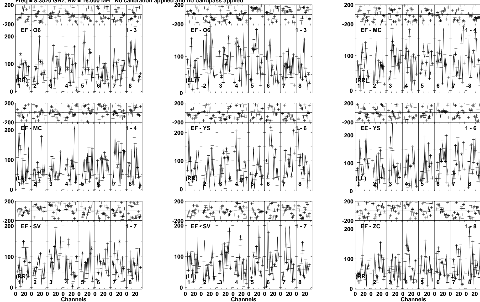
Lower frame: Micro Ampl Jy Top frame: Phas deg Vector averaged cross-power spectrum Baseline: EF (01) - O6 (03) Timerange: 00/01:06:50 to 00/01:09:45
