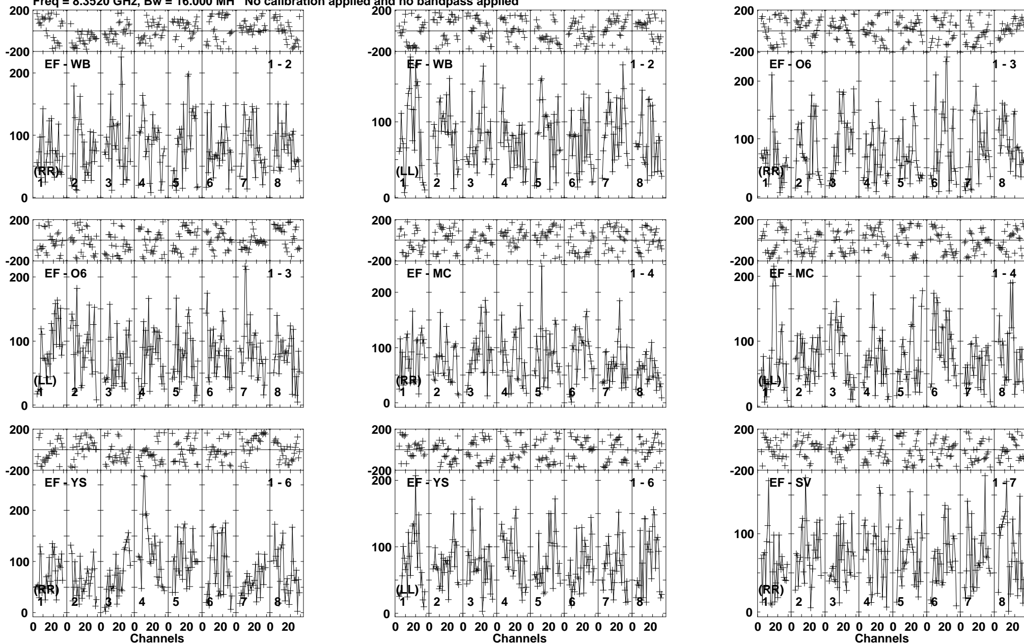
Lower frame: Micro Ampl Jy Top frame: Phas deg Vector averaged cross-power spectrum Baseline: EF (01) - WB (02) Timerange: 00/05:26:50 to 00/05:29:44
