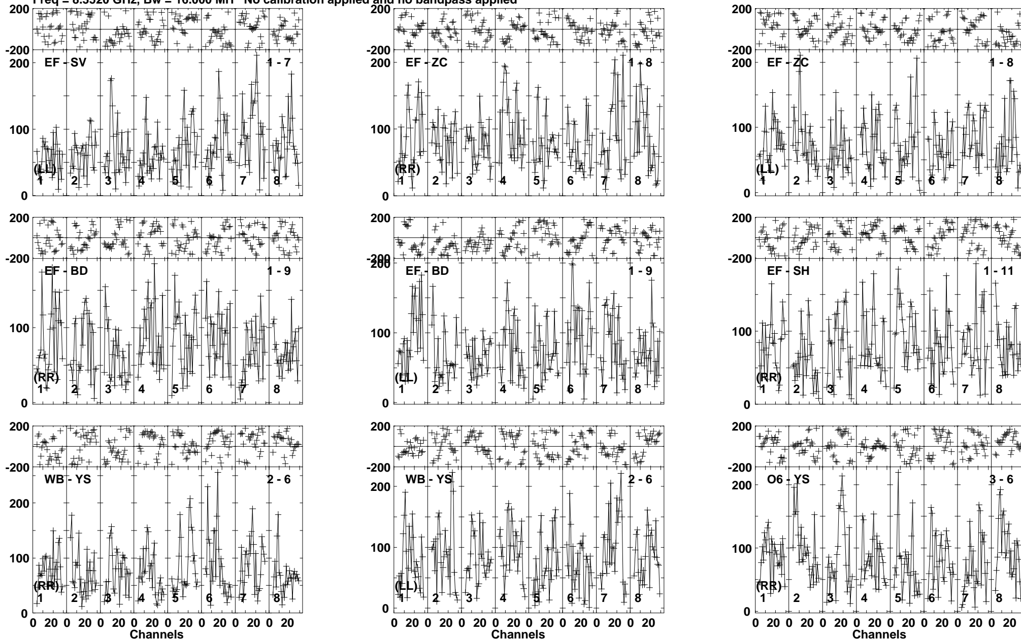
Lower frame: Micro Ampl Jy Top frame: Phas deg Vector averaged cross-power spectrum Baseline: EF (01) - SV (07) Timerange: 00/03:31:21 to 00/03:34:14
