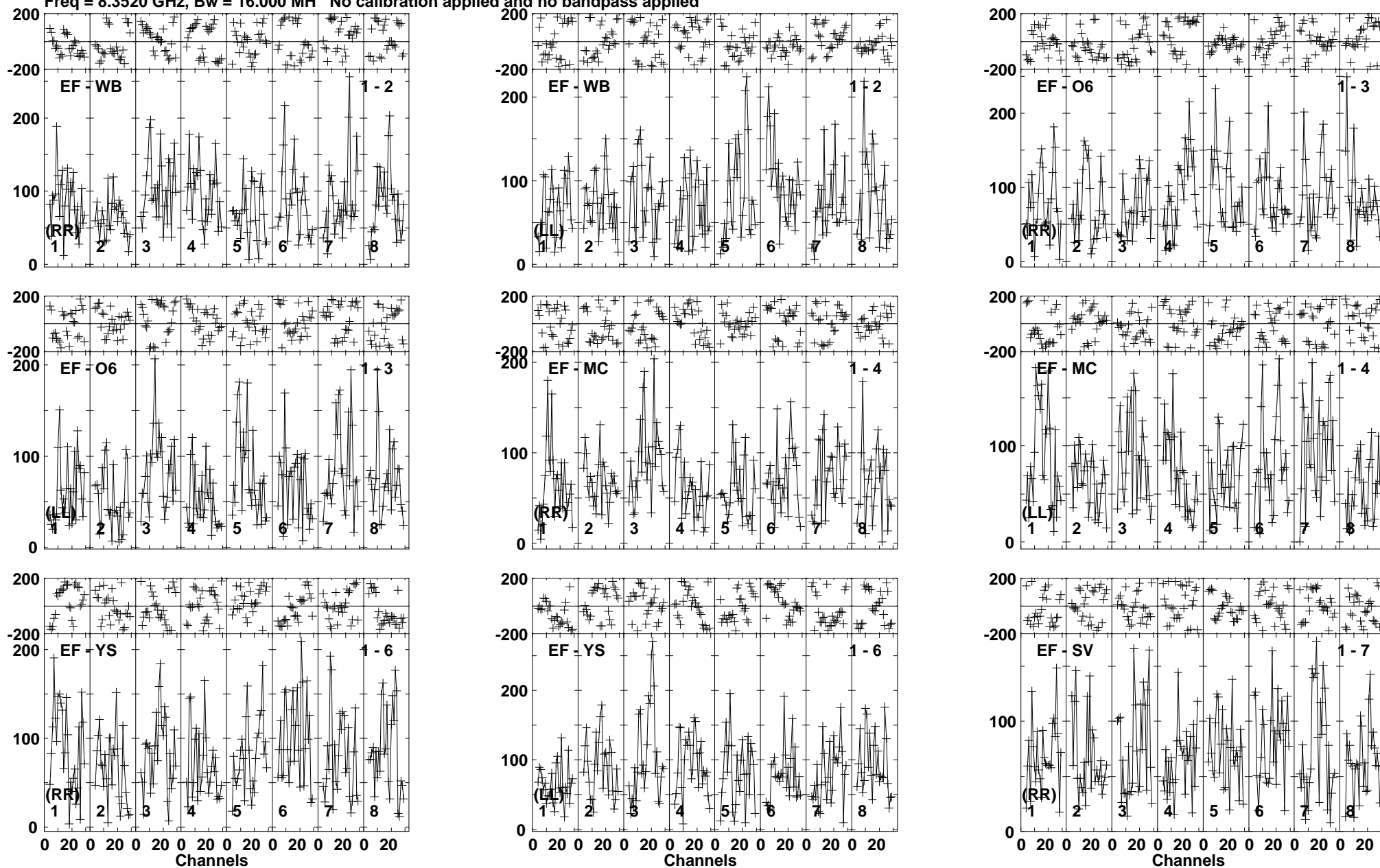
Lower frame: Micro Ampl Jy Top frame: Phas deg Vector averaged cross-power spectrum Baseline: EF (01) - WB (02) Timerange: 00/04:49:35 to 00/04:52:30
