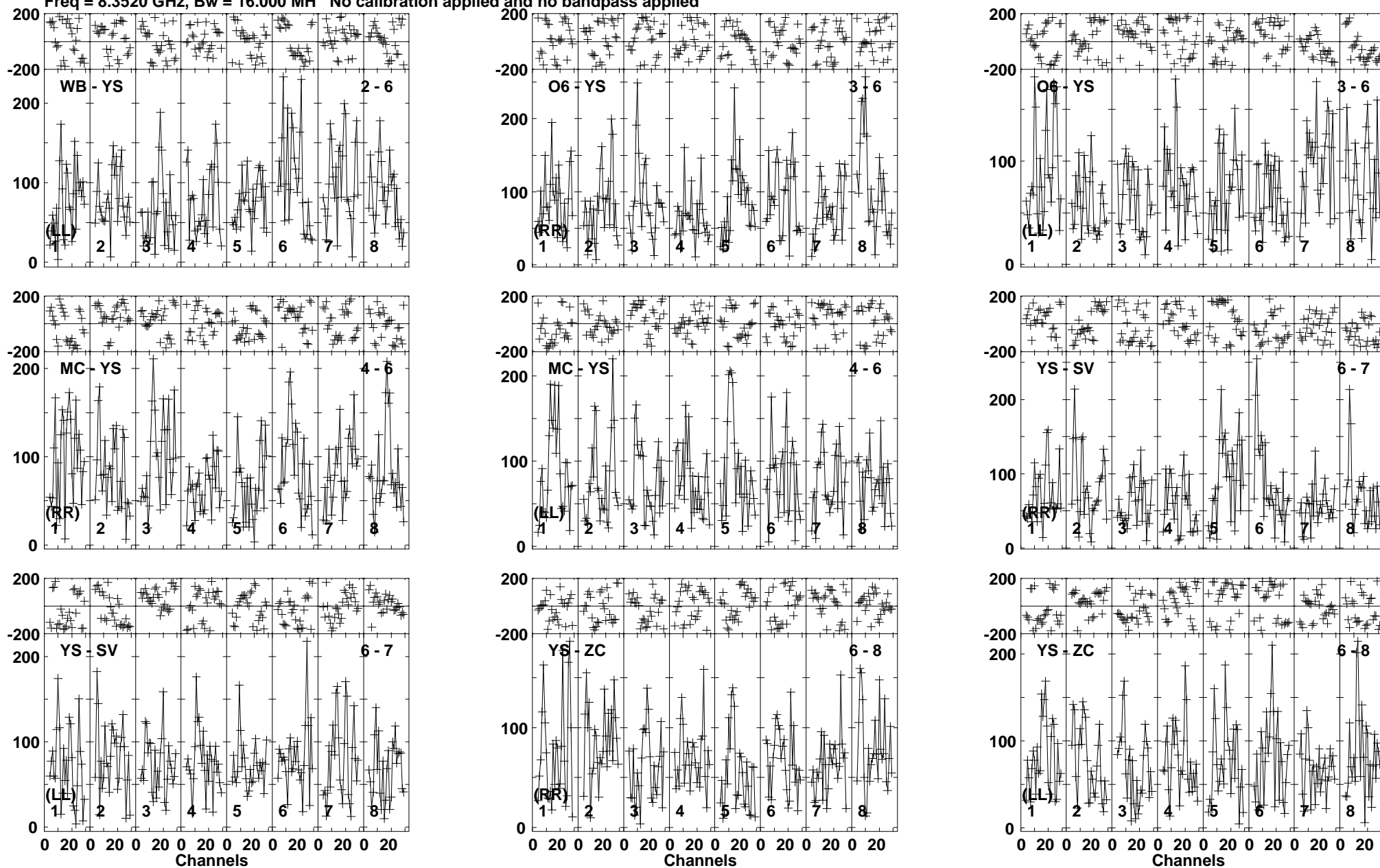
Lower frame: Micro Ampl Jy Top frame: Phas deg Vector average cross-power spectrum Baseline: WB (02) - YS (06) Timerange: 00/03:35:19 to 00/03:38:15
