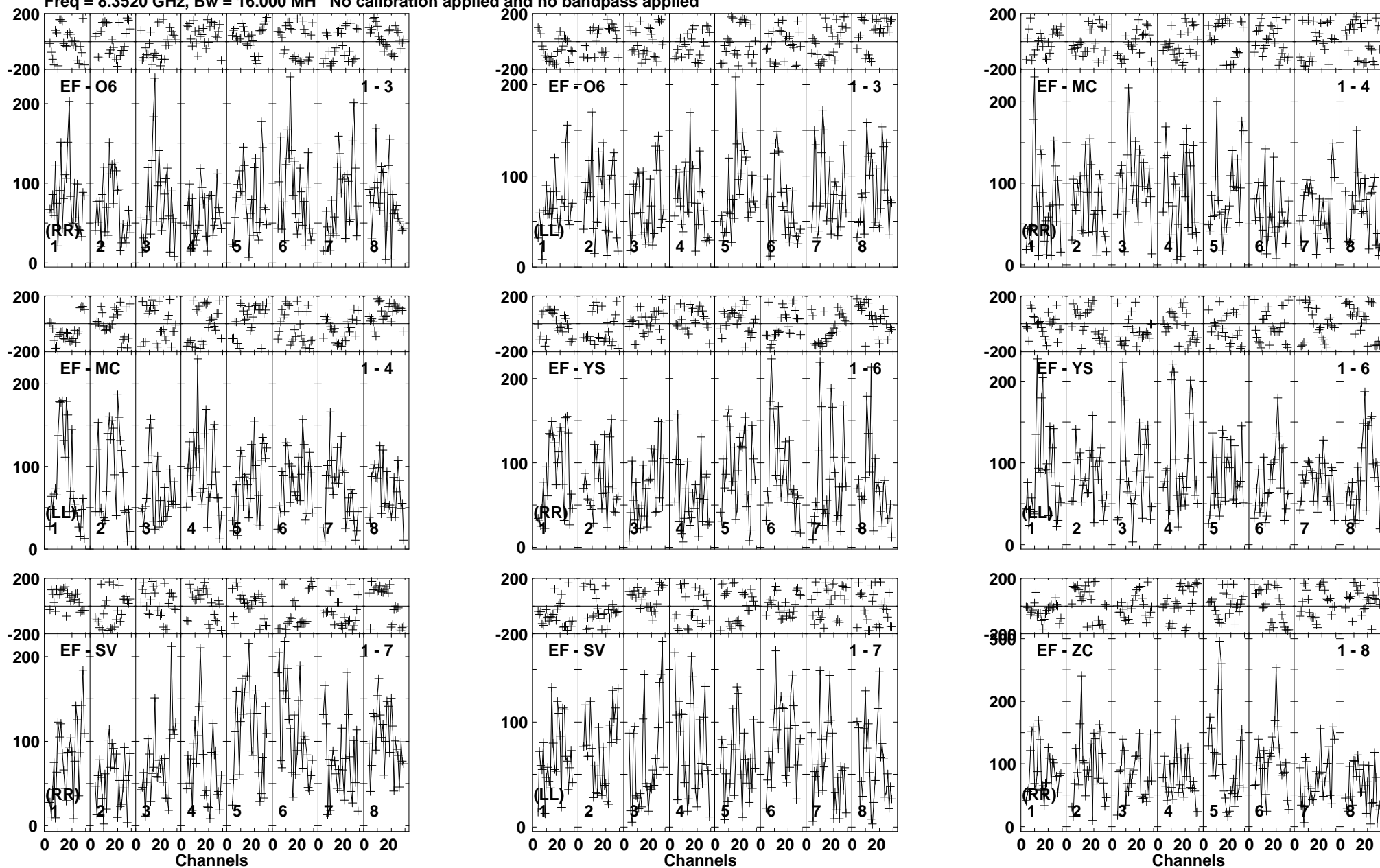
Lower frame: Micro Ampl Jy Top frame: Phas deg Vector averaged cross-power spectrum Baseline: EF (01) - O6 (03) Timerange: 00/02:41:50 to 00/02:44:44
