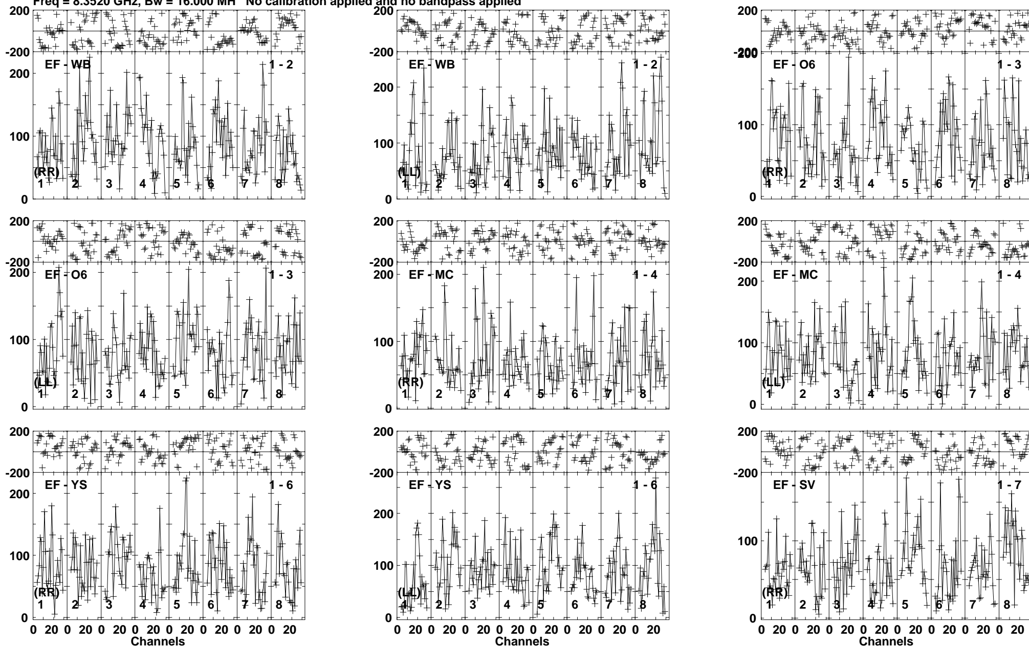
Lower frame: Micro Ampl Jy Top frame: Phas deg Vector averaged cross-power spectrum Baseline: EF (01) - WB (02) Timerange: 00/05:51:35 to 00/05:54:30
