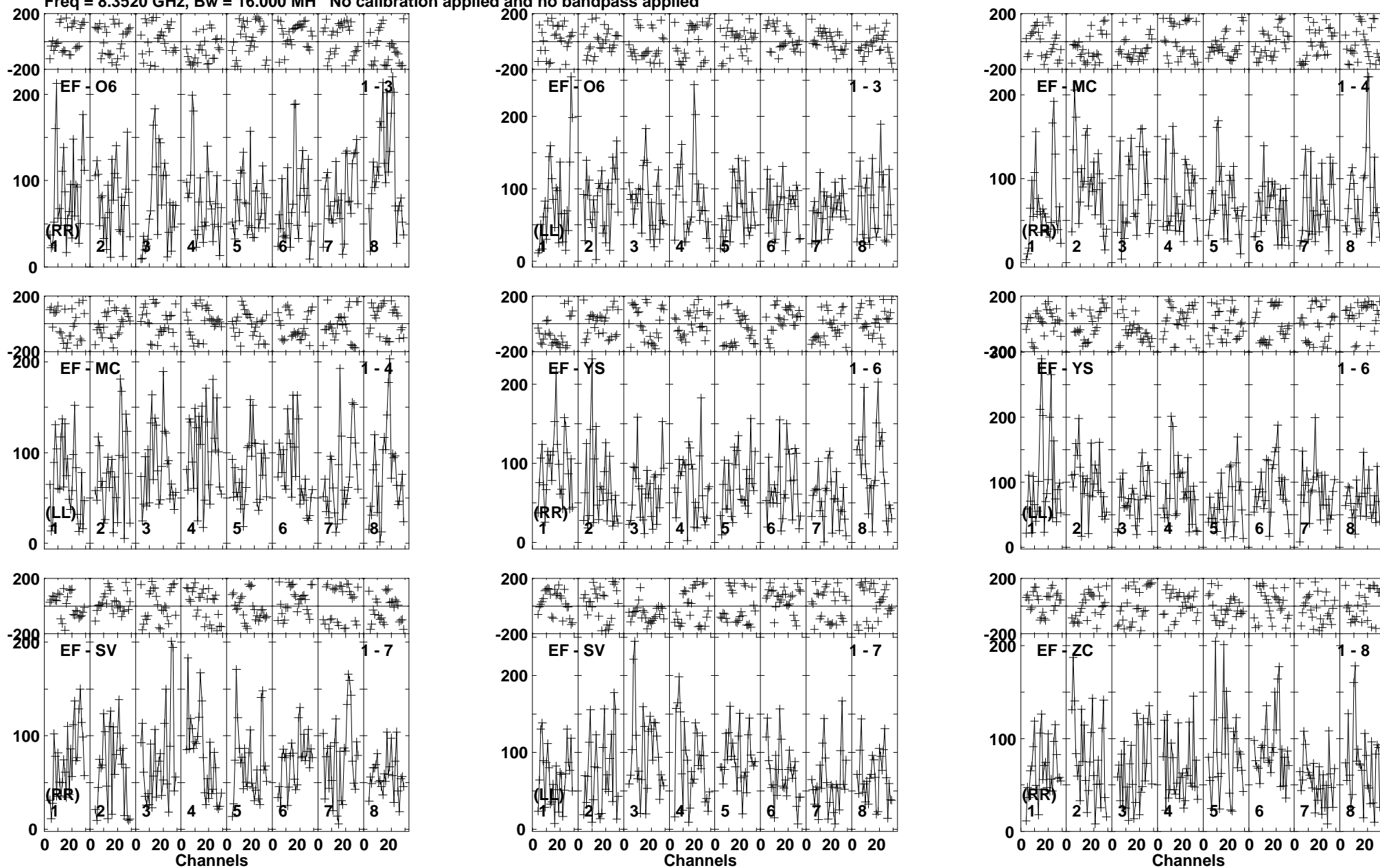
Lower frame: Micro Ampl Jy Top frame: Phas deg Vector averaged cross-power spectrum Baseline: EF (01) - O6 (03) Timerange: 00/01:23:20 to 00/01:26:15
