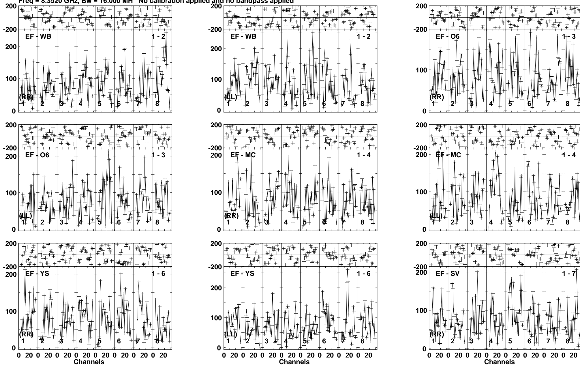
Lower frame: Micro Ampl Jy Top frame: Phas deg Vector averaged cross-power spectrum Baseline: EF (01) - WB (02) Timerange: 00/05:22:36 to 00/05:25:29
