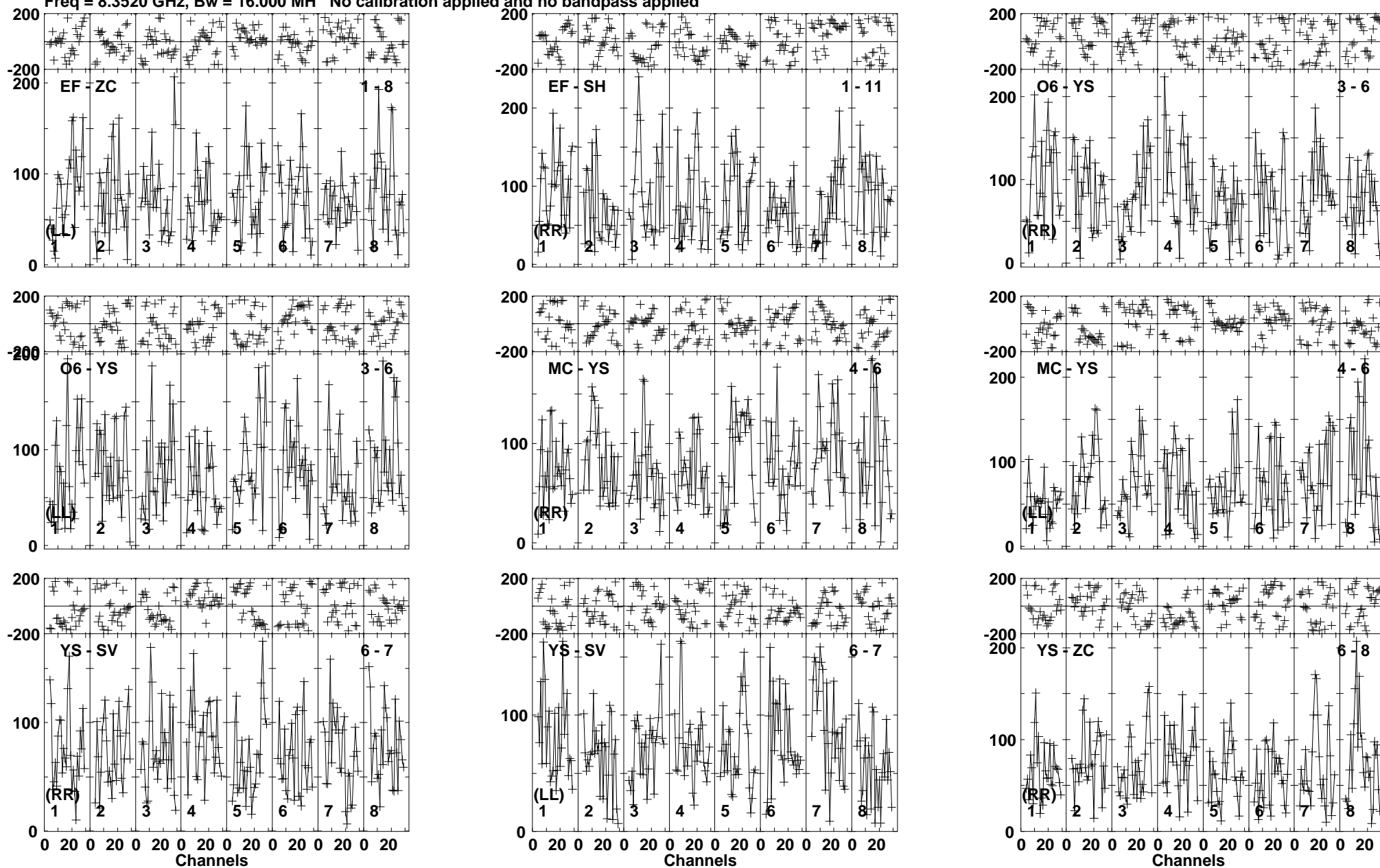
Lower frame: Micro Ampl Jy Top frame: Phas deg Vector averaged cross-power spectrum Baseline: EF (01) - ZC (08) Timerange: 00/02:37:36 to 00/02:40:30
