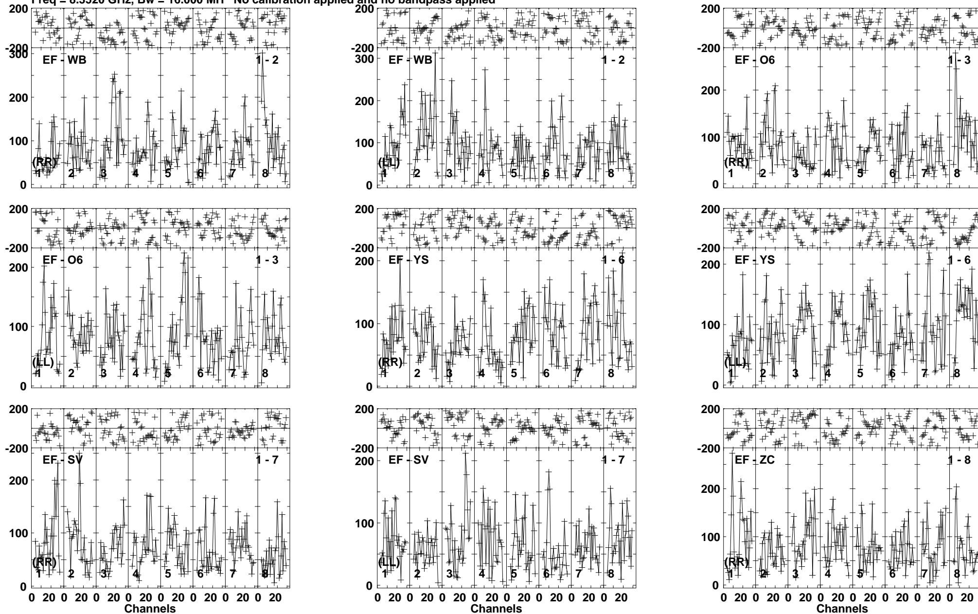
Lower frame: Micro Ampl Jy Top frame: Phas deg Vector averaged cross-power spectrum Baseline: EF (01) - WB (02) Timerange: 00/03:23:05 to 00/03:25:59
