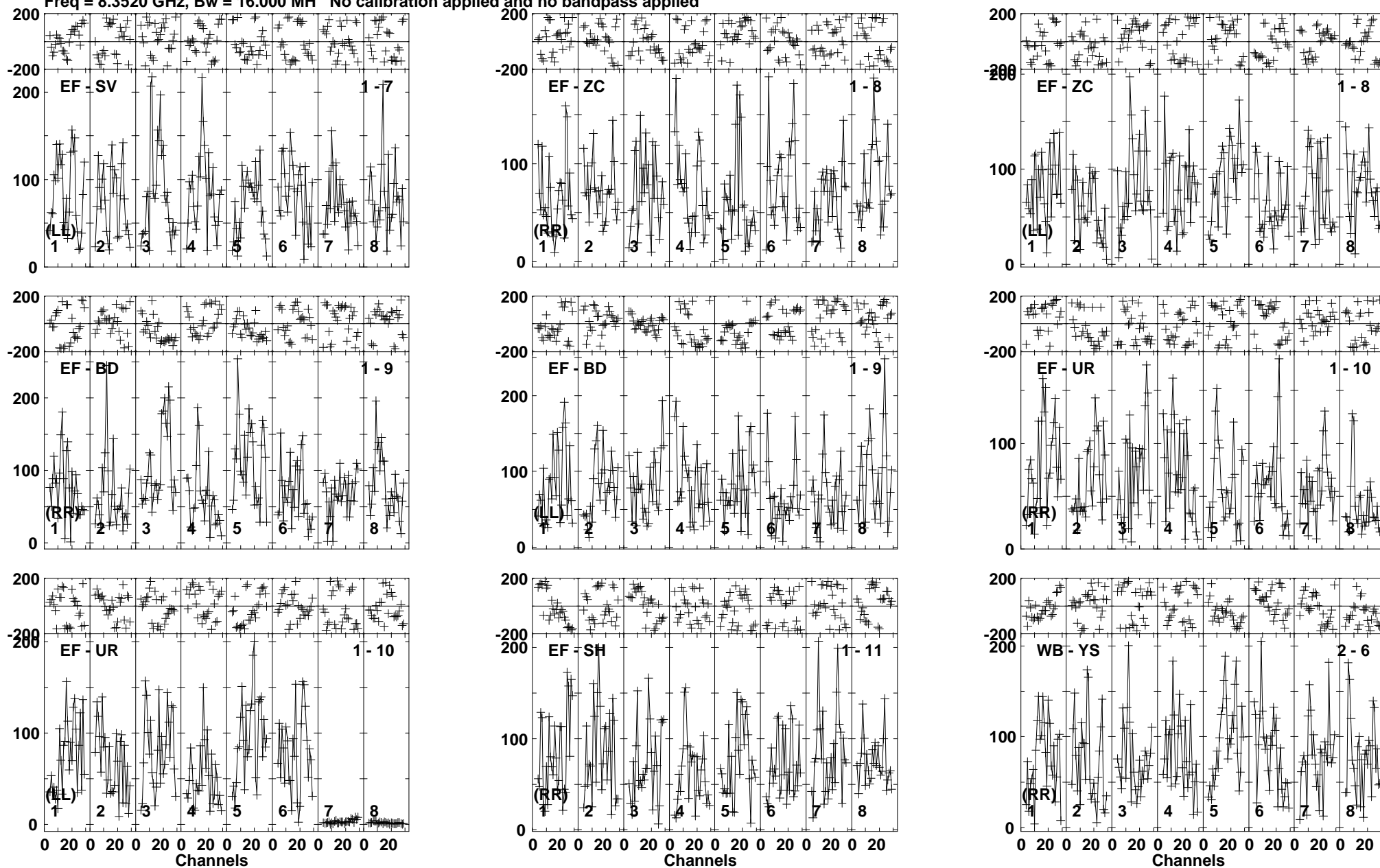
Lower frame: Micro Ampl Jy Top frame: Phas deg Vector averaged cross-power spectrum Baseline: EF (01) - SV (07) Timerange: 00/03:14:49 to 00/03:17:45
