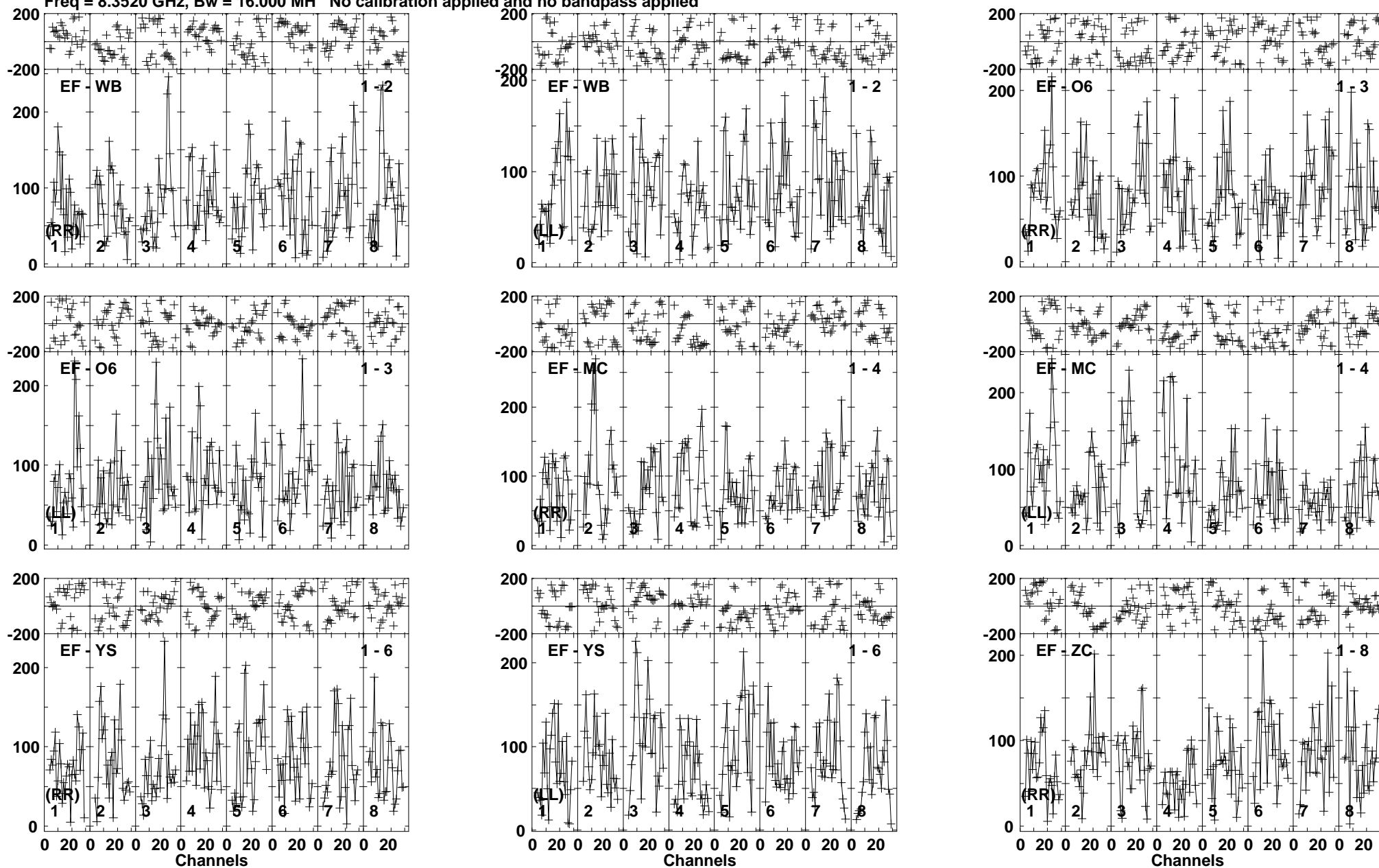
Lower frame: Micro Ampl Jy Top frame: Phas deg Vector averaged cross-power spectrum Baseline: EF (01) - WB (02) Timerange: 00/06:16:20 to 00/06:19:15
