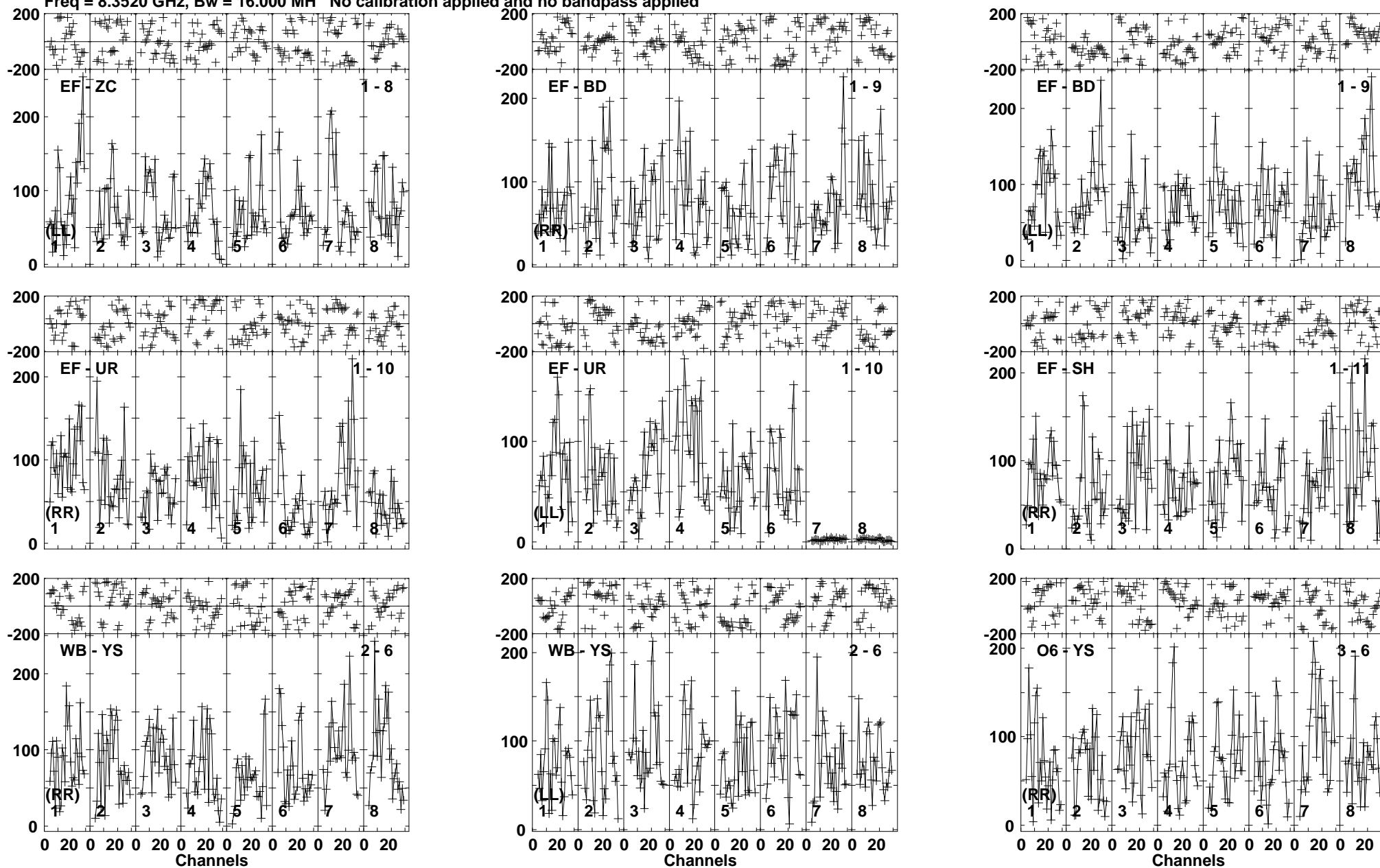
Lower frame: Micro Ampl Jy Top frame: Phas deg Vector averaged cross-power spectrum Baseline: EF (01) - ZC (08) Timerange: 00/03:23:05 to 00/03:25:59
