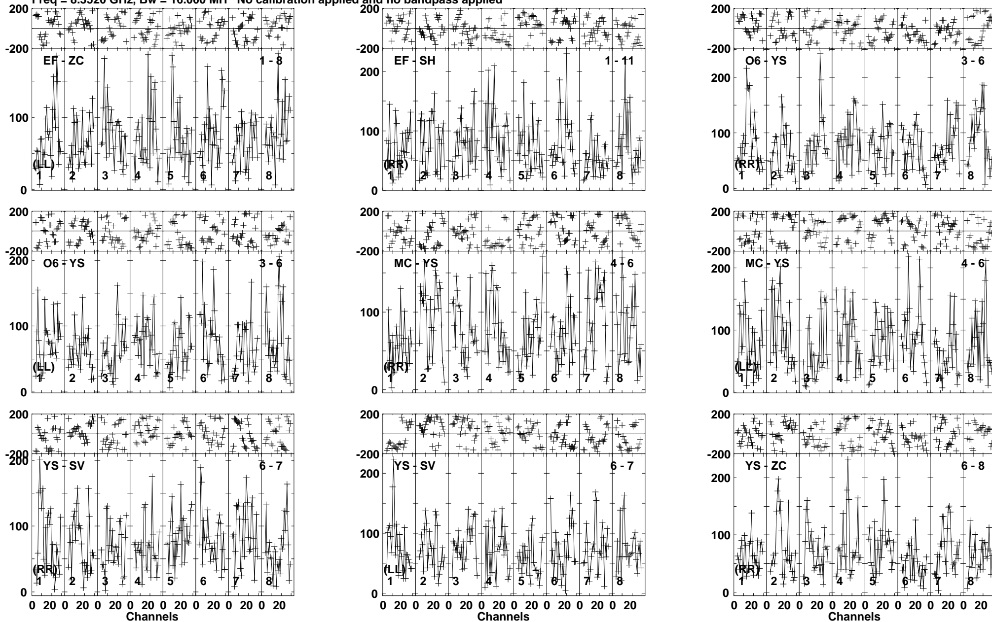
Lower frame: Micro Ampl Jy Top frame: Phas deg Vector averaged cross-power spectrum Baseline: EF (01) - ZC (08) Timerange: 00/02:29:20 to 00/02:32:15
