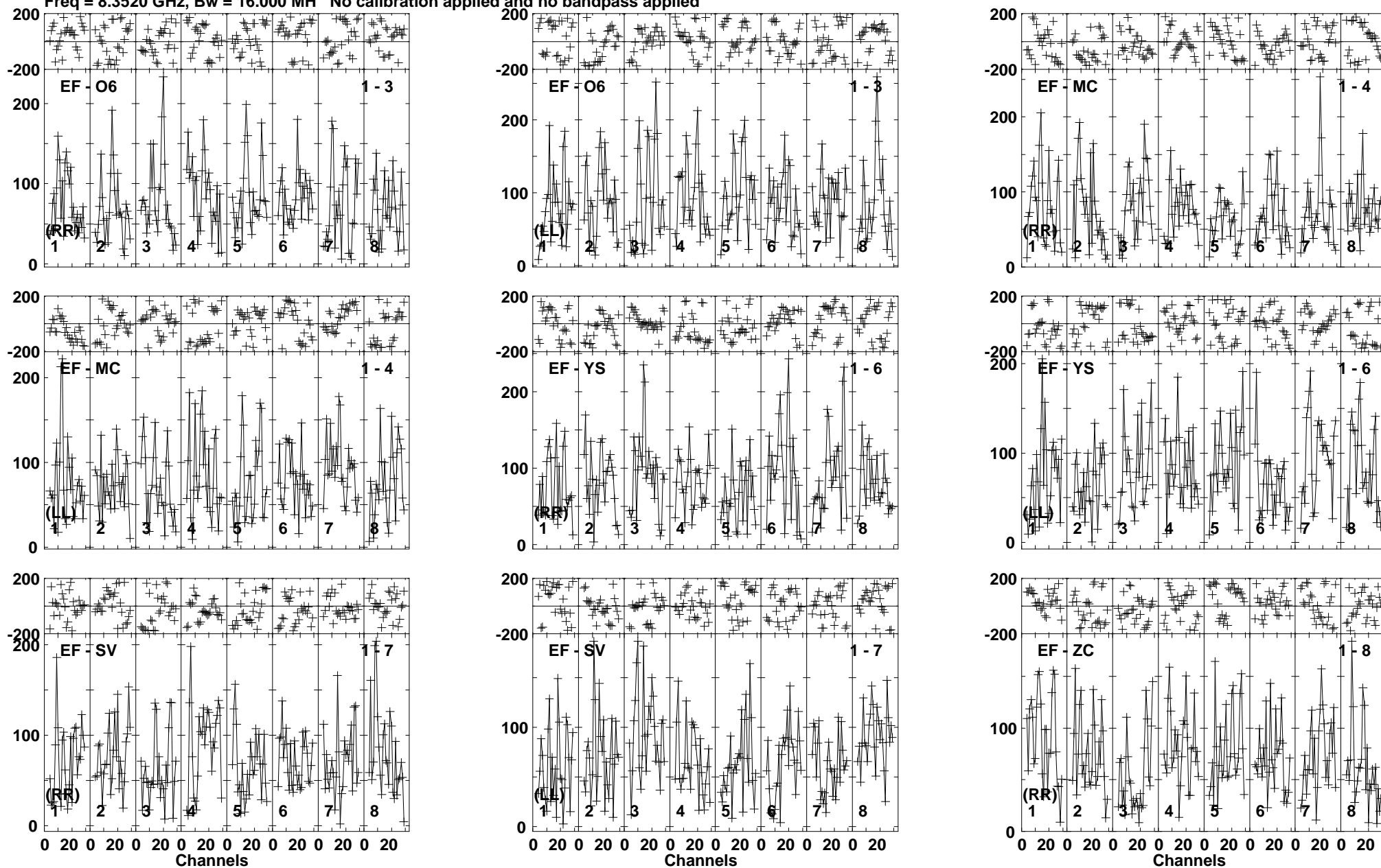
Lower frame: Micro Ampl Jy Top frame: Phas deg Vector averaged cross-power spectrum Baseline: EF (01) - O6 (03) Timerange: 00/01:11:05 to 00/01:13:59
