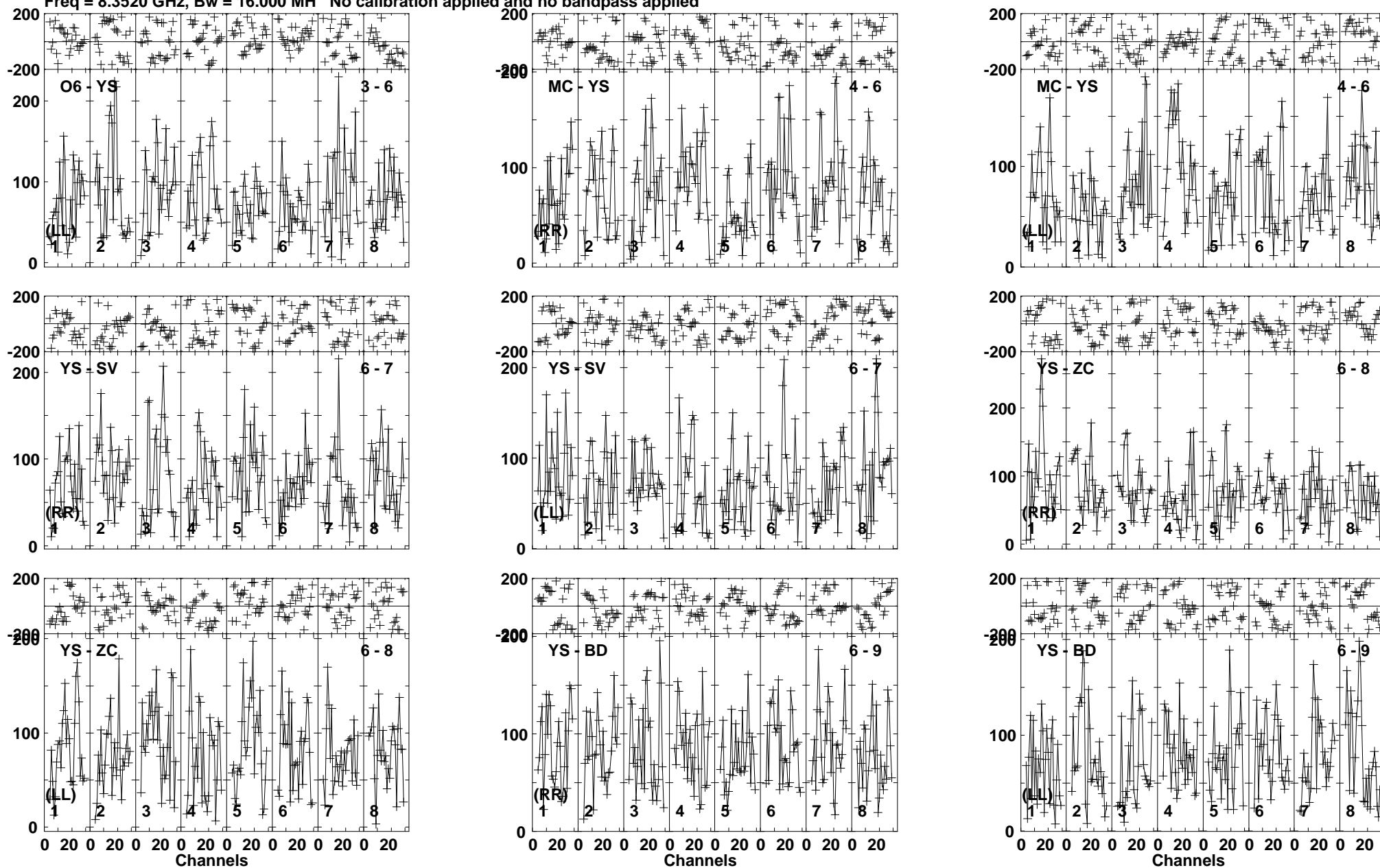
Lower frame: Micro Ampl Jy Top frame: Phas deg Vector averaged cross-power spectrum Baseline: O6 (03) - YS (06) Timerange: 00/05:10:21 to 00/05:13:15
