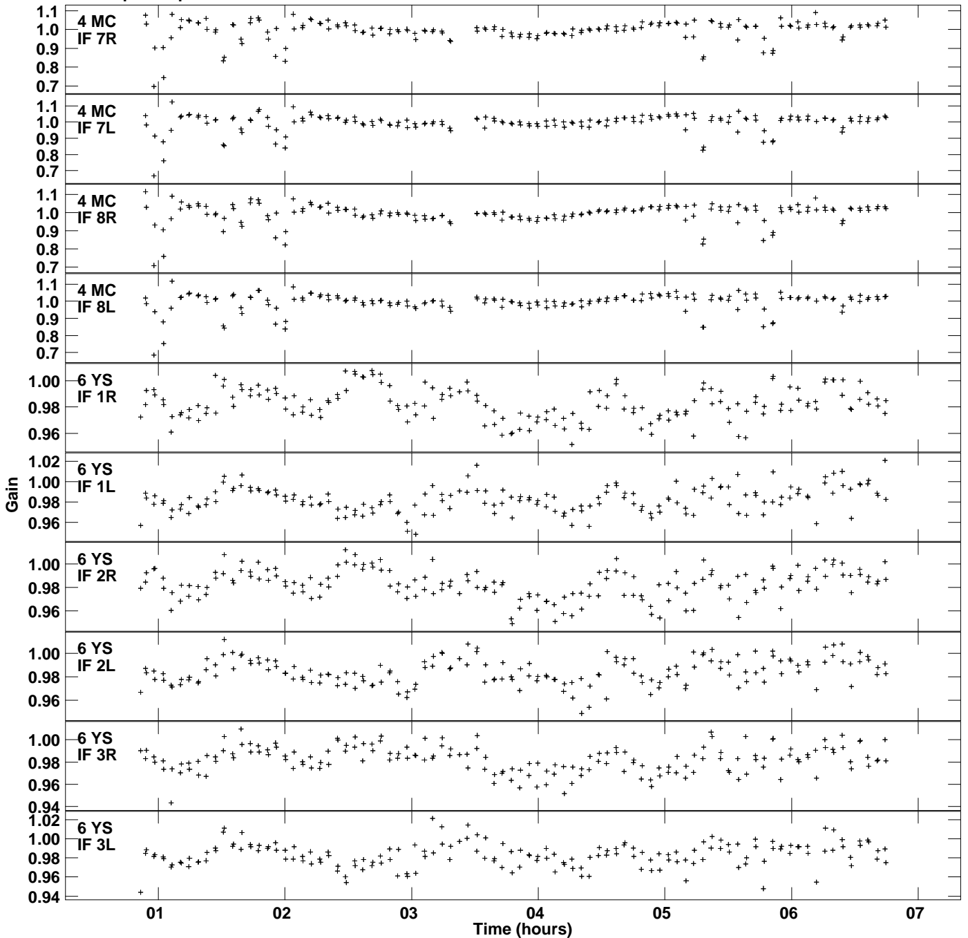
Plot file version 7 created 06-JUL-2016 19:50:46 Gain amp vs UTC time for J1128+5925.MULTI.1 SN 4 Rpol & Lpol IF 1 - 8
