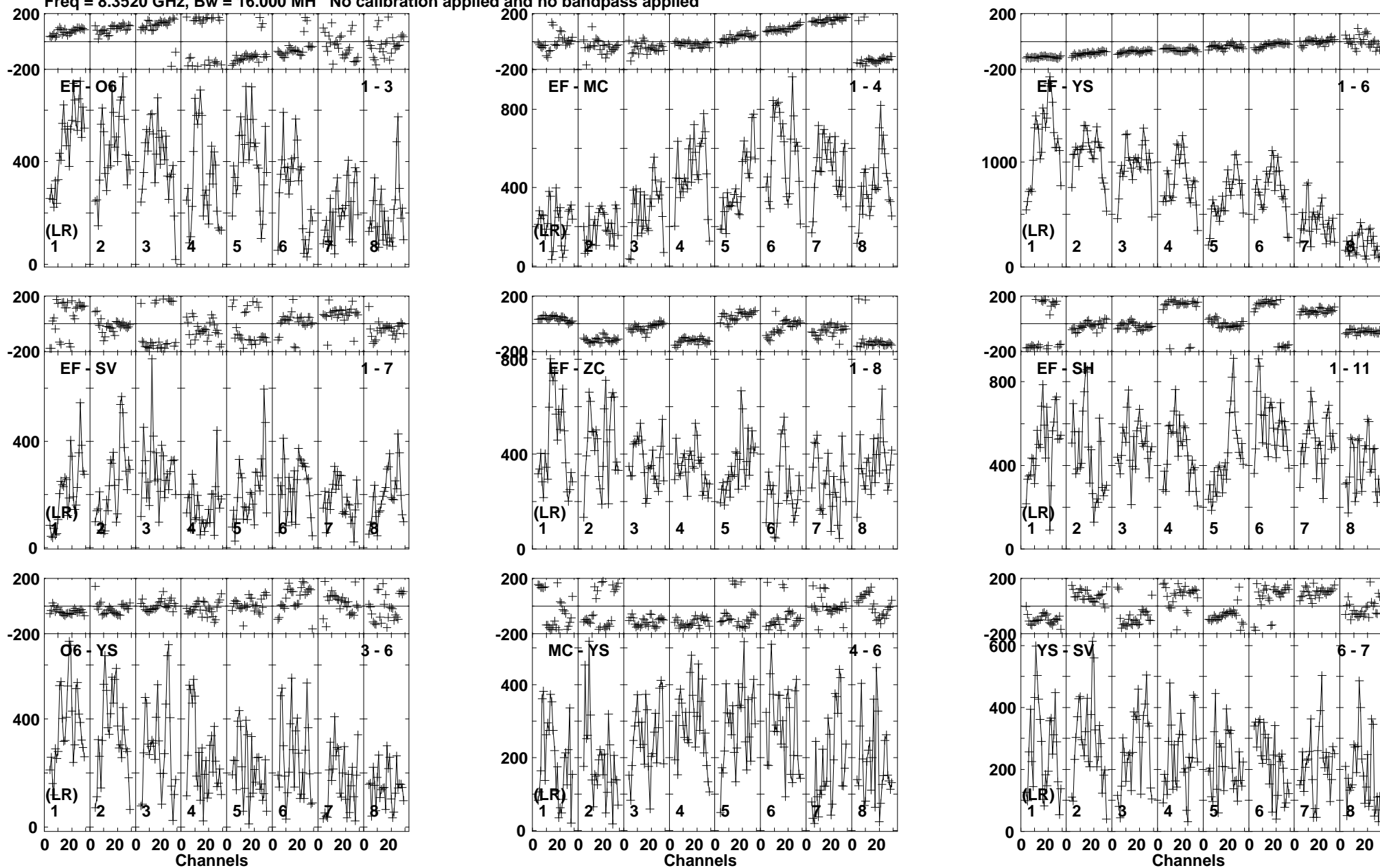
Lower frame: Micro Ampl Jy Top frame: Phas deg Vector averaged cross-power spectrum Baseline: EF (01) - O6 (03) Timerange: 00/02:32:56 to 00/02:33:29
