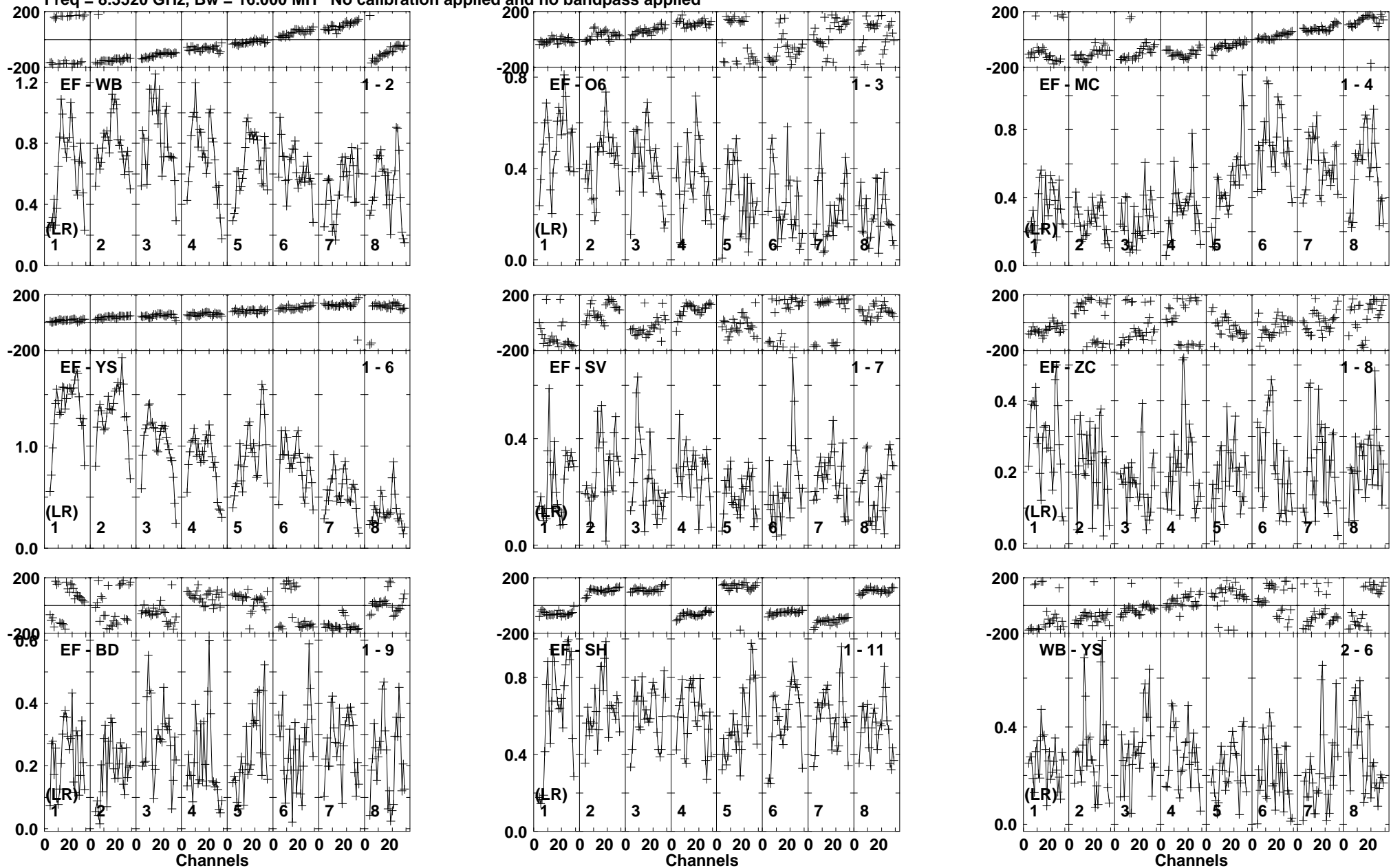
Lower frame: Milli Ampl Jy Top frame: Phas deg Vector averaged cross-power spectrum Baseline: EF (01) - WB (02) Timerange: 00/05:01:27 to 00/05:02:00
