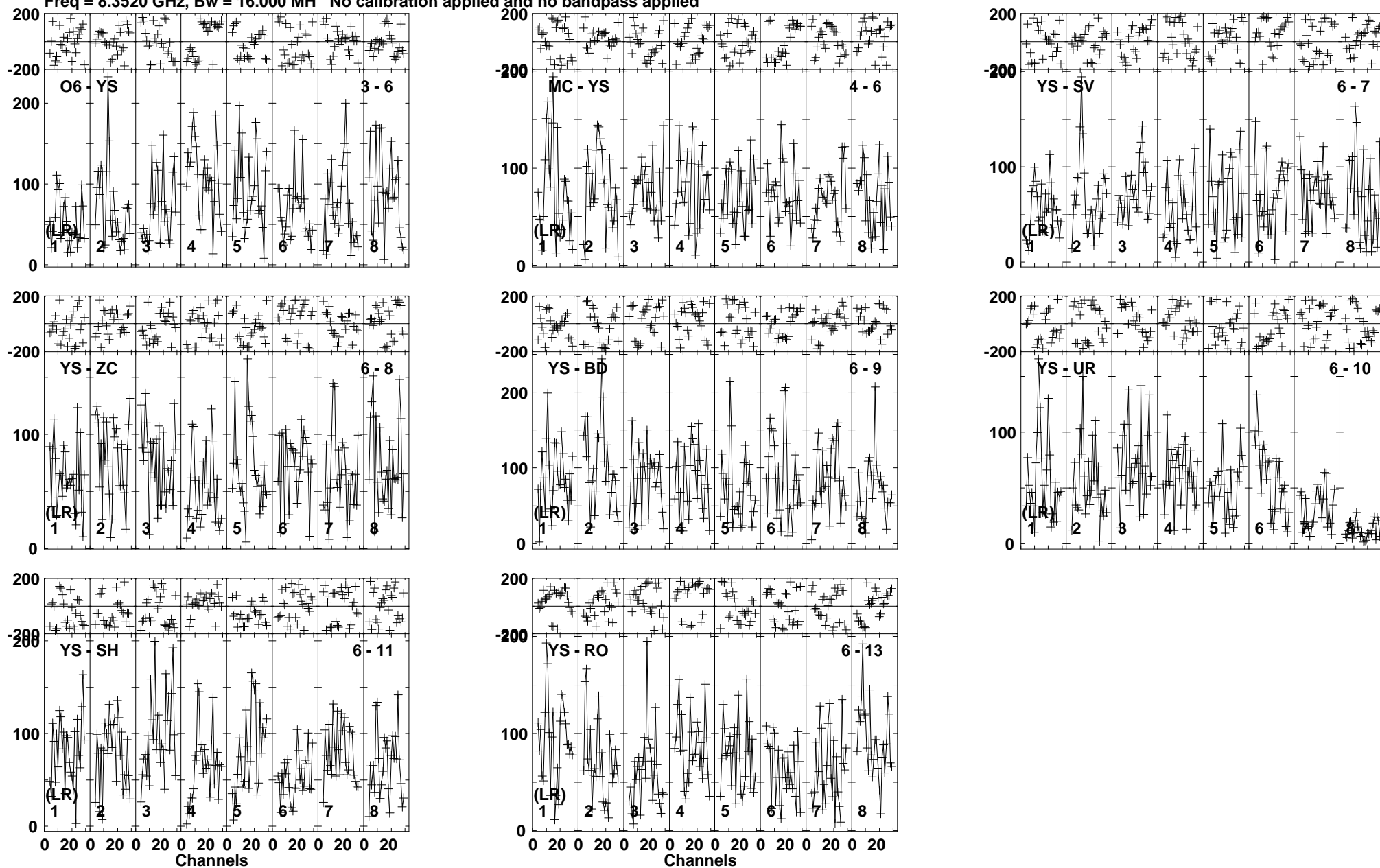
Lower frame: Micro Ampl Jy Top frame: Phas deg Vector averaged cross-power spectrum Baseline: O6 (03) - YS (06) Timerange: 00/01:27:35 to 00/01:30:30
