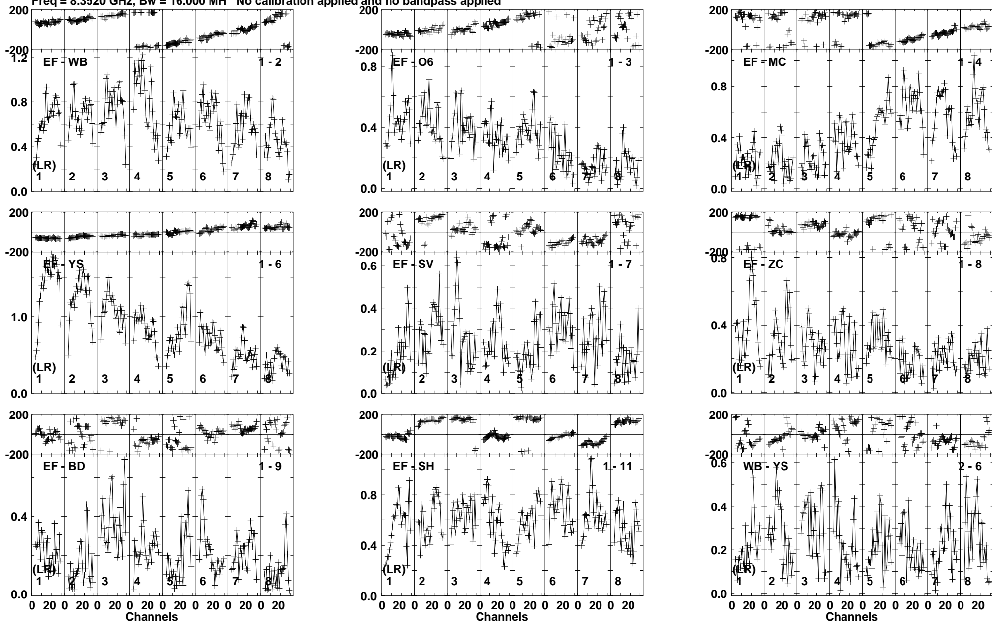
Lower frame: Milli Ampl Jy Top frame: Phas deg Vector averaged cross-power spectrum Baseline: EF (01) - WB (02) Timerange: 00/04:36:41 to 00/04:37:14
