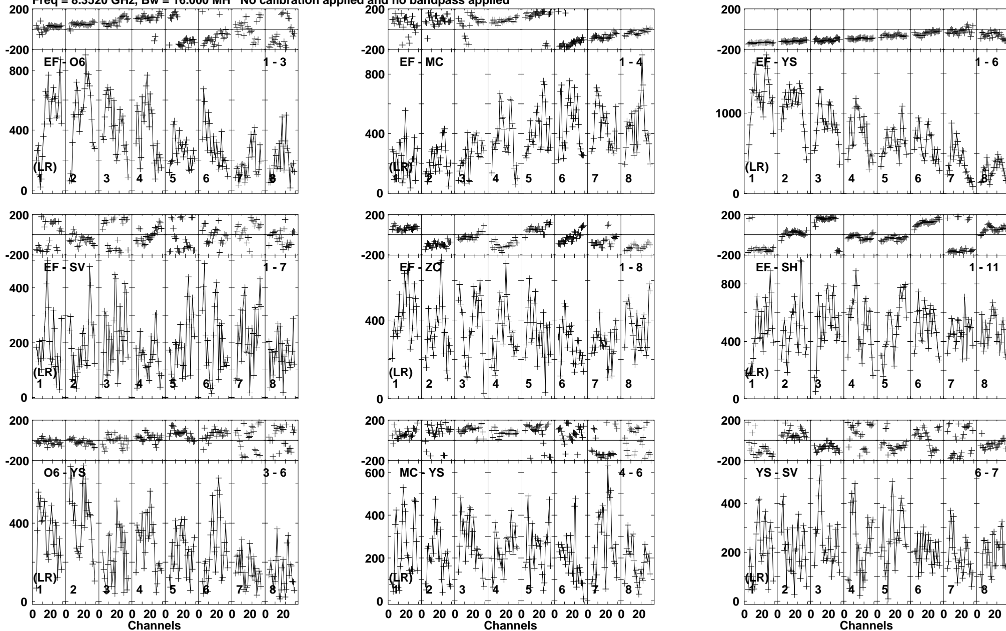
Lower frame: Micro Ampl Jy Top frame: Phas deg Vector averaged cross-power spectrum Baseline: EF (01) - O6 (03) Timerange: 00/02:24:42 to 00/02:25:15
