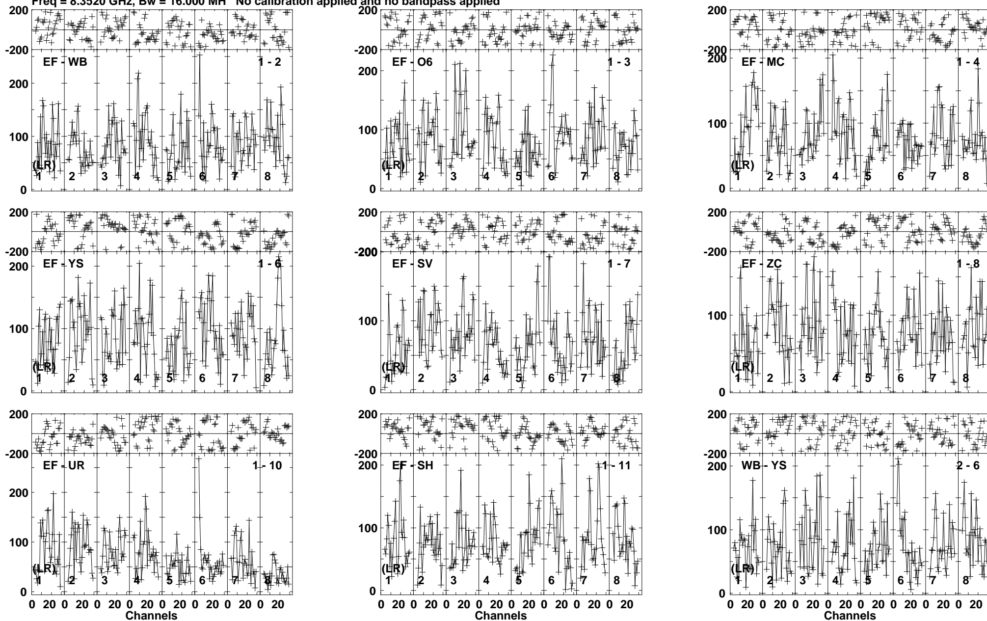
Lower frame: Micro Ampl Jy Top frame: Phas deg Vector averaged cross-power spectrum Baseline: EF (01) - WB (02) Timerange: 00/03:02:20 to 00/03:05:14
