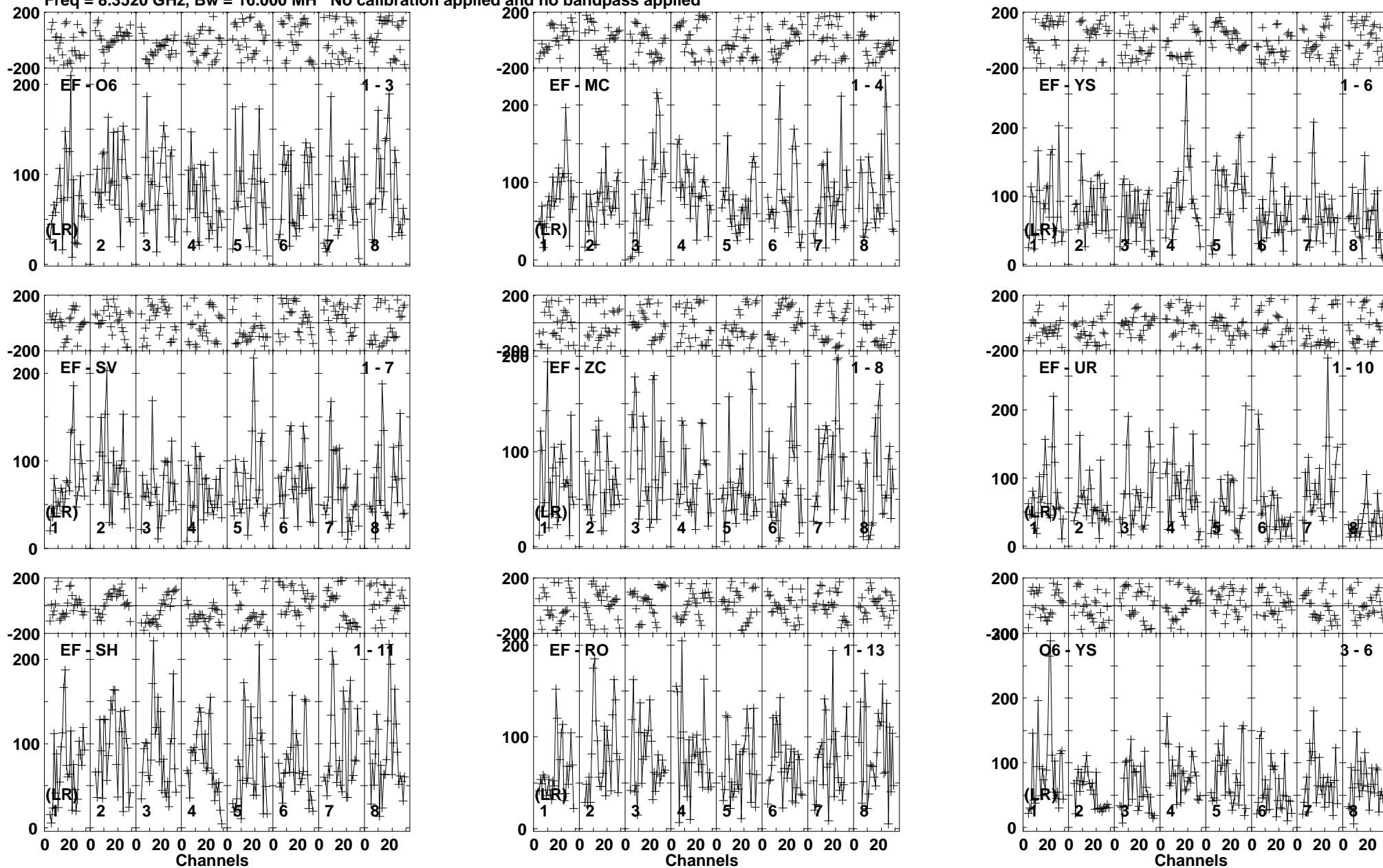
Lower frame: Micro Ampl Jy Top frame: Phas deg Vector averaged cross-power spectrum Baseline: EF (01) - O6 (03) Timerange: 00/02:17:05 to 00/02:19:59
