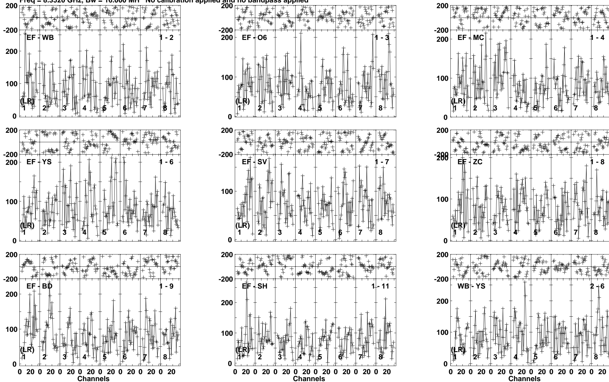
Lower frame: Micro Ampl Jy Top frame: Phas deg Vector averaged cross-power spectrum Baseline: EF (01) - WB (02) Timerange: 00/05:30:50 to 00/05:33:45
