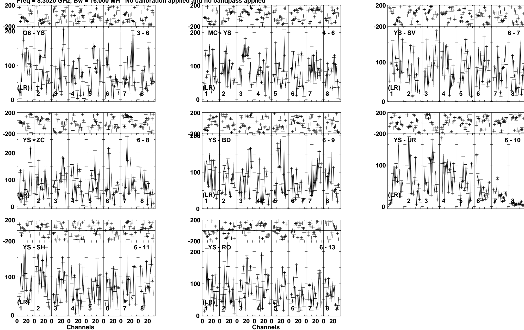
Lower frame: Micro Ampl Jy Top frame: Phas deg Vector averaged cross-power spectrum Baseline: O6 (03) - YS (06) Timerange: 00/01:23:20 to 00/01:26:15
