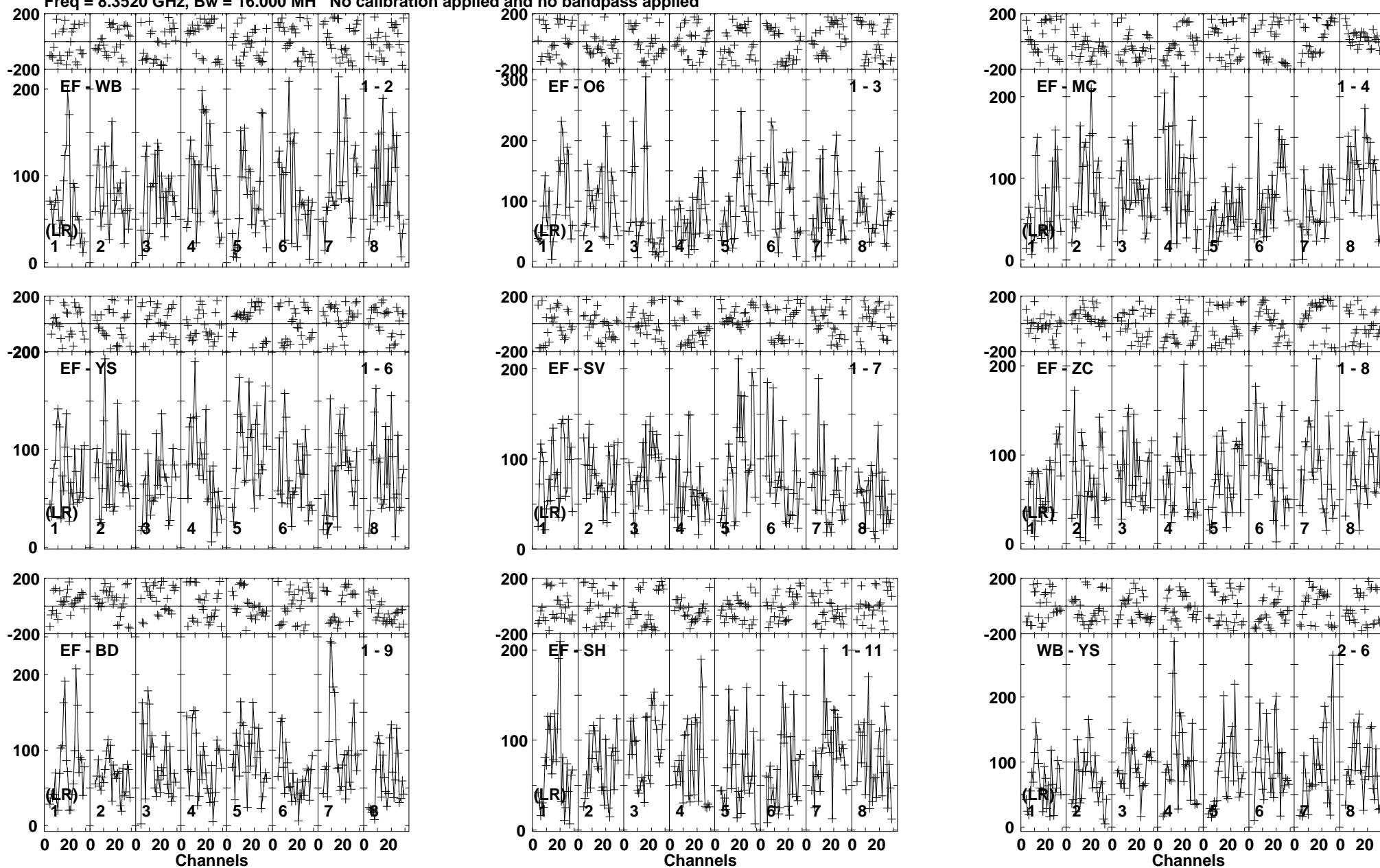
Lower frame: Micro Ampl Jy Top frame: Phas deg Vector averaged cross-power spectrum Baseline: EF (01) - WB (02) Timerange: 00/04:08:21 to 00/04:11:14
