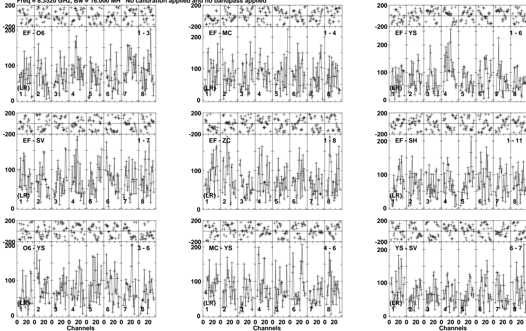
Lower frame: Micro Ampl Jy Top frame: Phas deg Vector average cross-power spectrum Baseline: EF (01) - O6 (03) Timerange: 00/02:25:21 to 00/02:28:15
