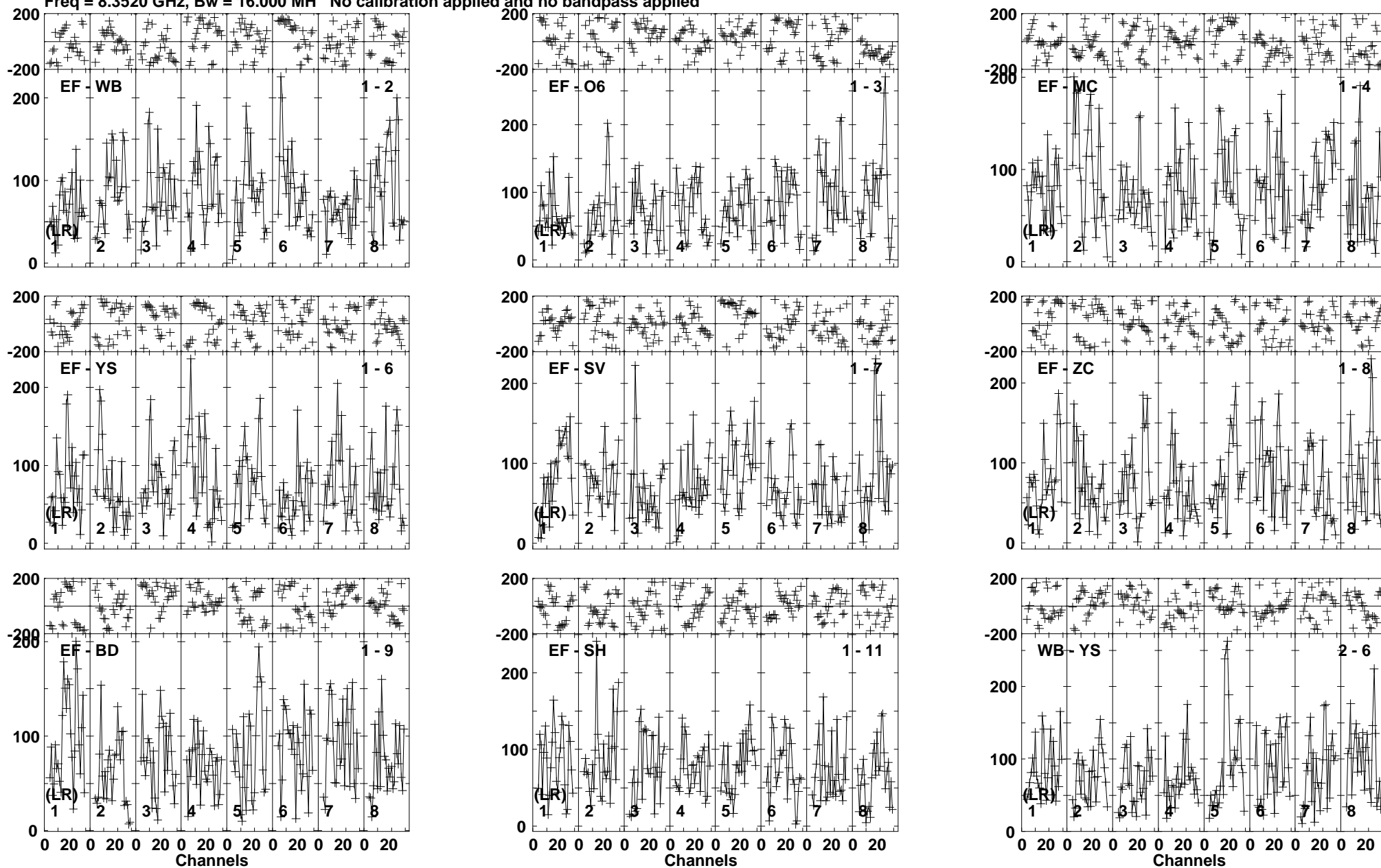
Lower frame: Micro Ampl Jy Top frame: Phas deg Vector averaged cross-power spectrum Baseline: EF (01) - WB (02) Timerange: 00/03:31:21 to 00/03:34:14
