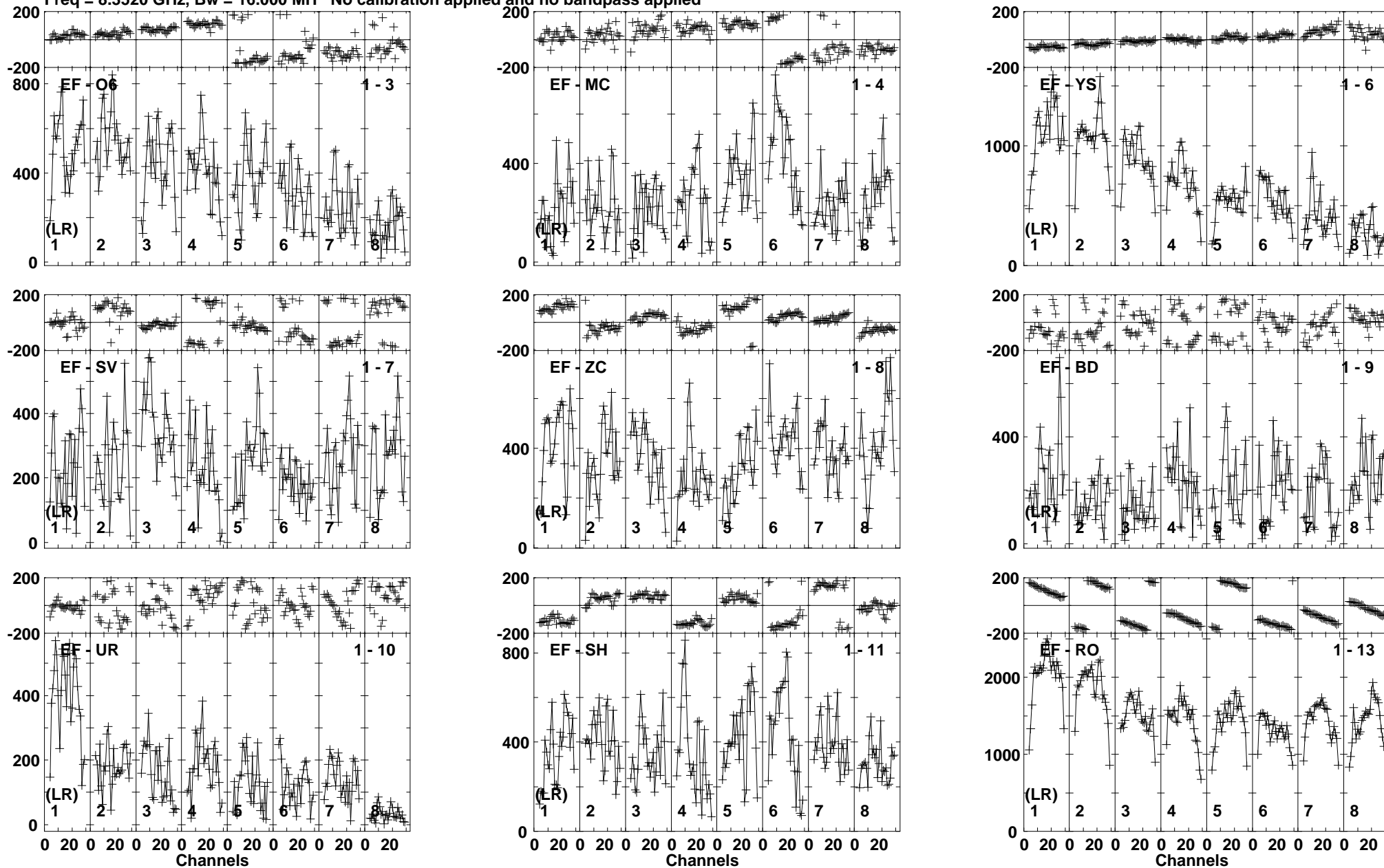
Lower frame: Micro Ampl Jy Top frame: Phas deg Vector averaged cross-power spectrum Baseline: EF (01) - O6 (03) Timerange: 00/01:30:35 to 00/01:31:29
