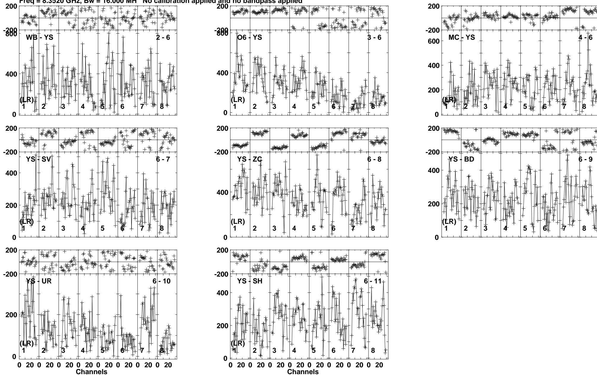
Lower frame: Micro Ampl Jy Top frame: Phas deg Vector averaged cross-power spectrum Baseline: WB (02) - YS (06) Timerange: 00/03:09:32 to 00/03:10:29
