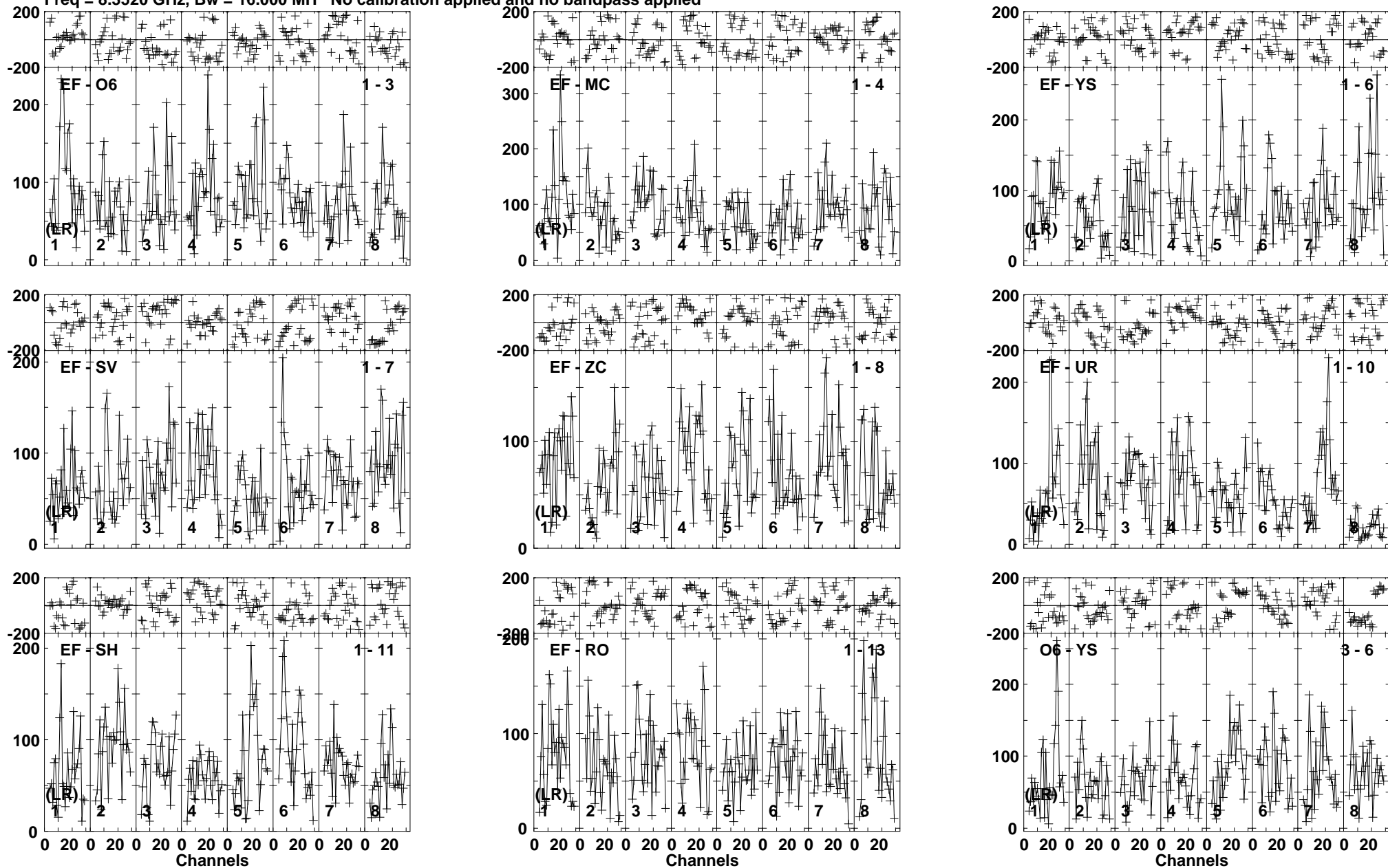
Lower frame: Micro Ampl Jy Top frame: Phas deg Vector averaged cross-power spectrum Baseline: EF (01) - O6 (03) Timerange: 00/01:44:05 to 00/01:46:59
