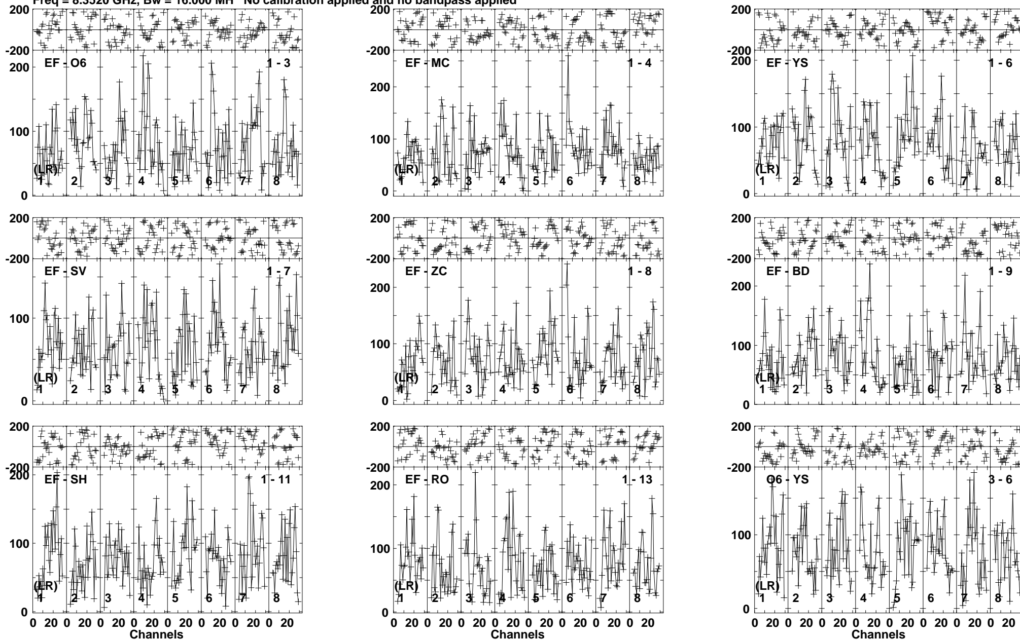
Lower frame: Micro Ampl Jy Top frame: Phas deg Vector averaged cross-power spectrum Baseline: EF (01) - O6 (03) Timerange: 00/01:02:51 to 00/01:05:45
